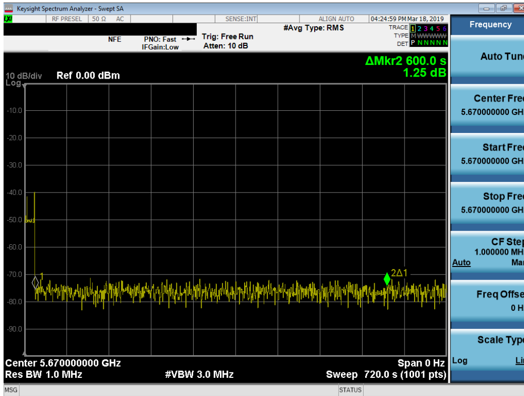
Figure 5-3. Band 2C Client Beacon Test – Monitoring live spectrum – Elapse time 10 minutes
