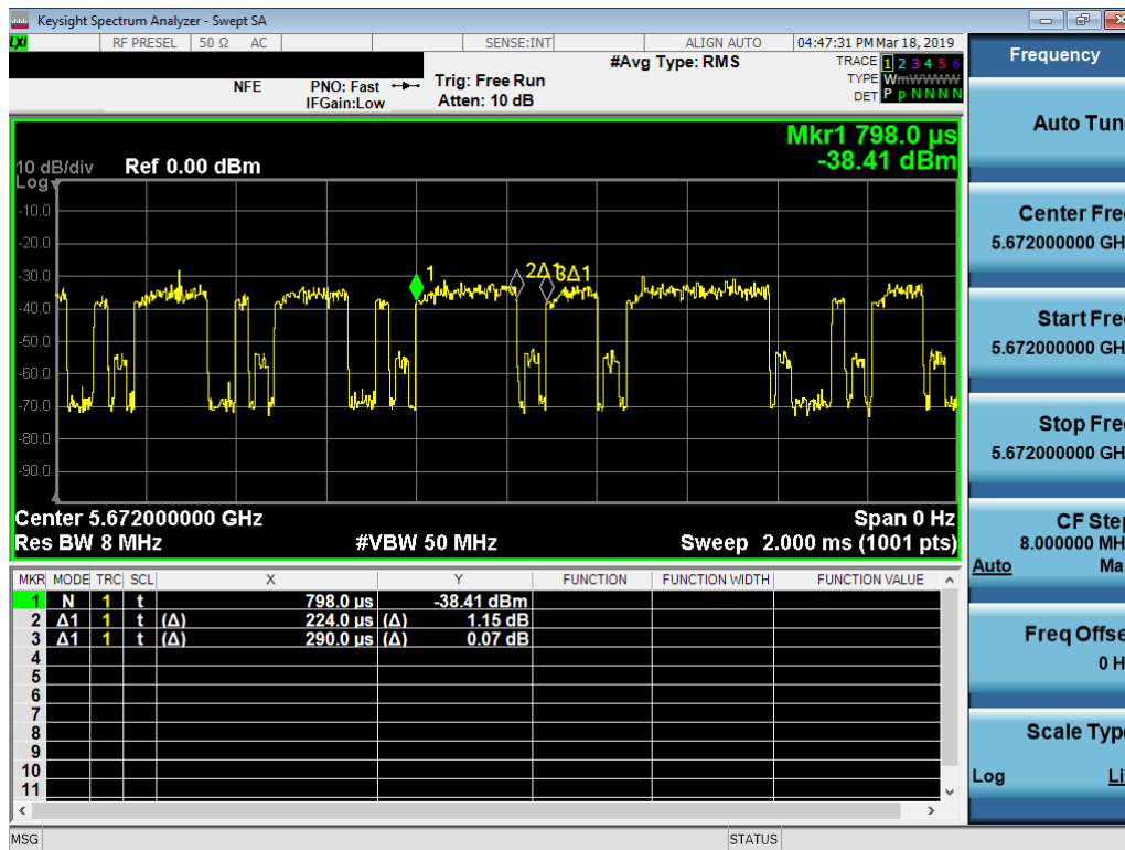
Figure 5-1. Band 2C Pulse Width and Period
