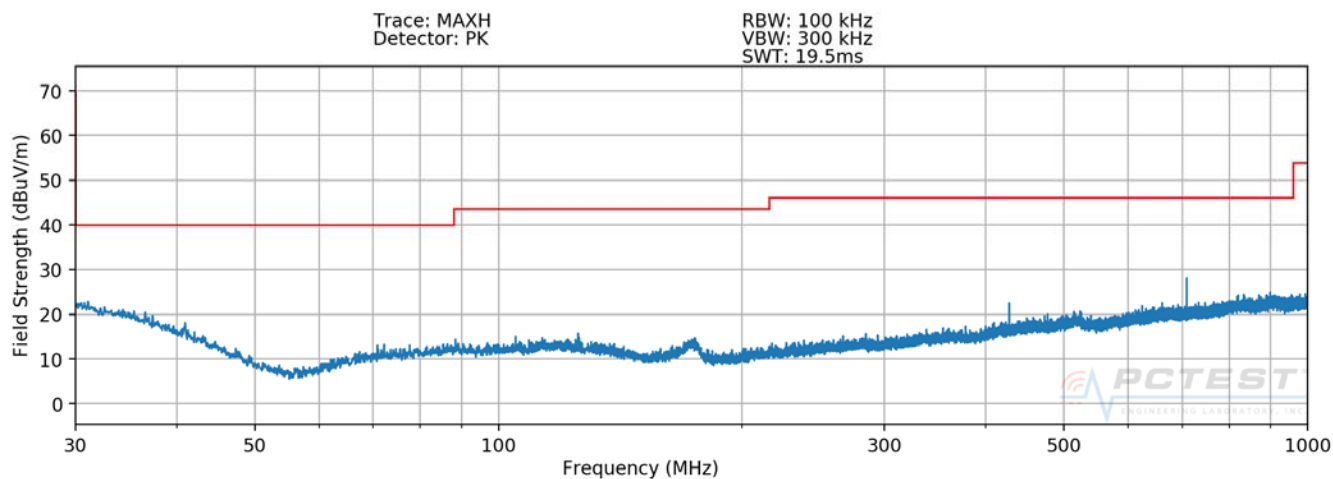
Plot 7-8. Radiated Spurious Plot 30MHz – 1GHz (Pol. V)
