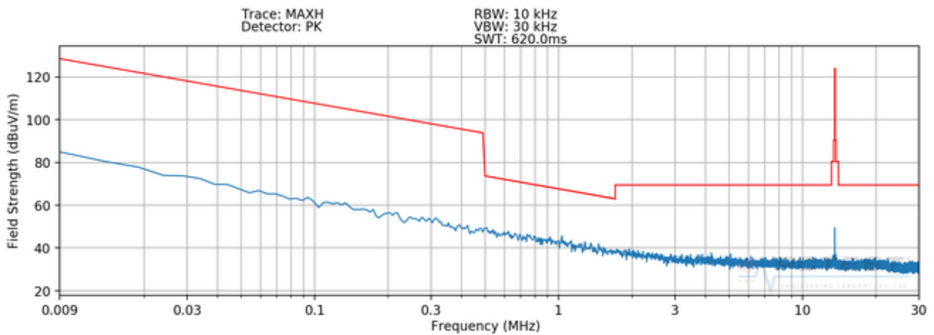
Plot 7-5. Radiated Spurious Plot 9kHz – 30MHz (Pol. Z - CLOSED)
