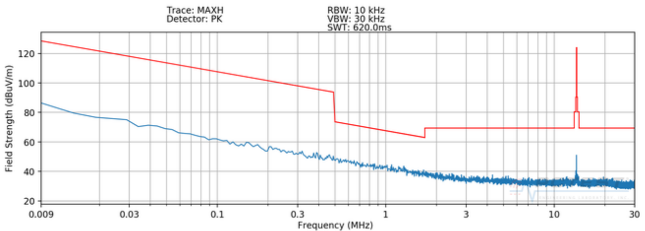
Plot 7-6. Radiated Spurious Plot 9kHz – 30MHz (Pol. Z - OPEN)
