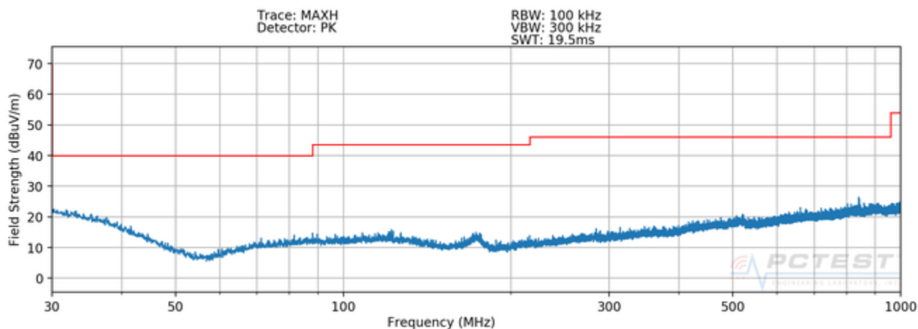
Plot 7-7. Radiated Spurious Plot 30MHz – 1GHz (Pol. H)
