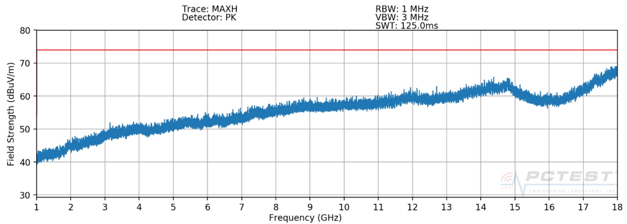
Plot 7-2. Radiated Spurious Plot above 1GHz [Radiated Test Config. 1 - H]
