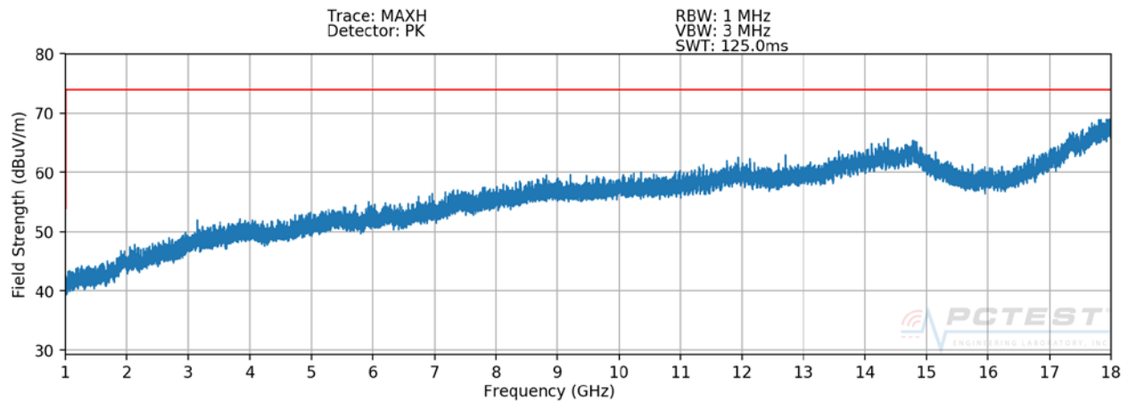
Plot 7-6. Radiated Spurious Plot above 1GHz [Radiated Test Config. 2 - V]
