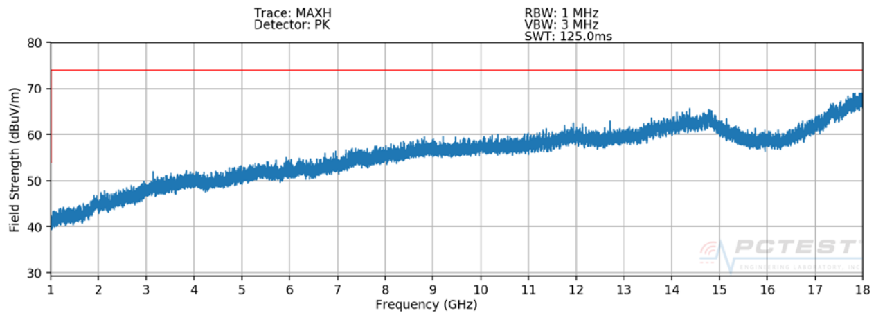
Plot 7-12. Radiated Spurious Plot above 1GHz [Radiated Test Config. 4 - V]
