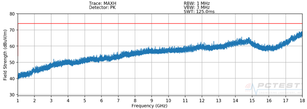
Plot 7-5. Radiated Spurious Plot above 1GHz [Radiated Test Config. 2 - H]
