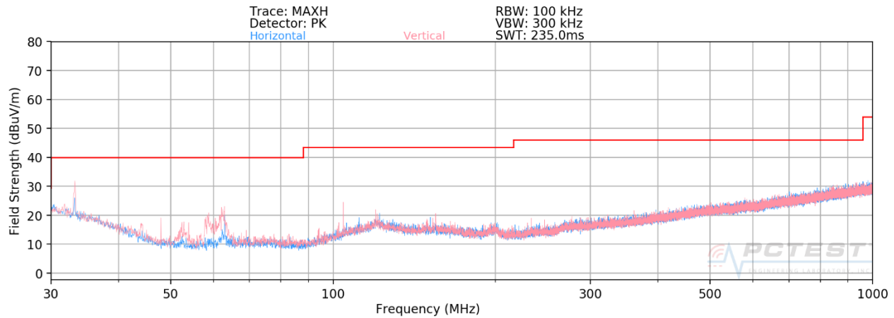
Plot 7-4. Radiated Spurious Plot below 1GHz [Radiated Test Config. 2]
