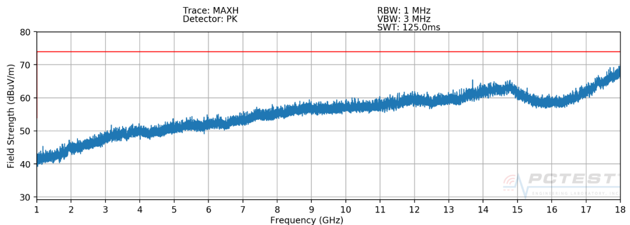
Plot 7-3. Radiated Spurious Plot above 1GHz [Radiated Test Config. 1 - V]
