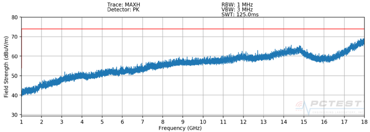
Plot 7-8. Radiated Spurious Plot above 1GHz [Radiated Test Config. 3 - H]
