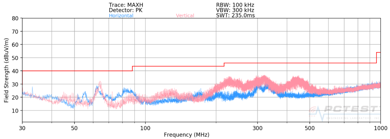
Plot 7-10. Radiated Spurious Plot below 1GHz [Radiated Test Config. 4]
