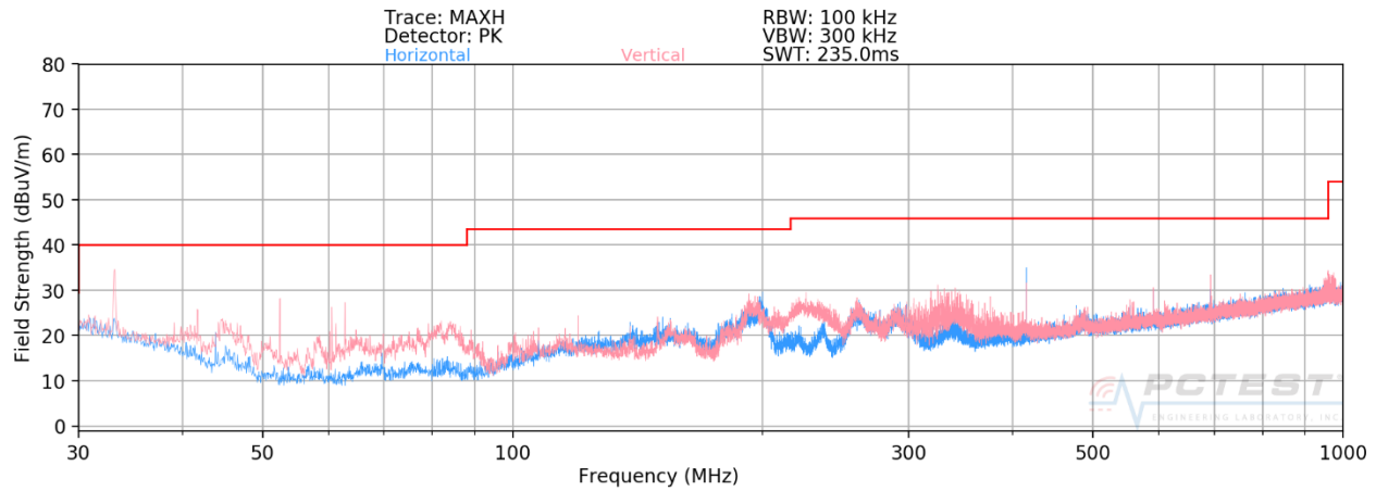
Plot 7-7. Radiated Spurious Plot below 1GHz [Radiated Test Config. 3]
