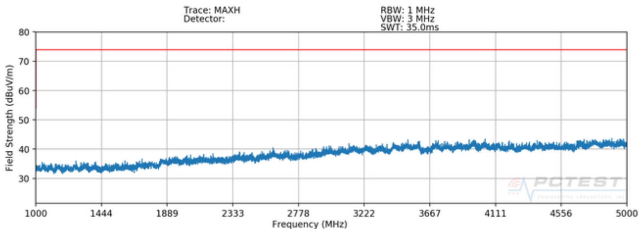
Plot 7-2. Radiated Spurious Plot above 1GHz – H - OPEN
