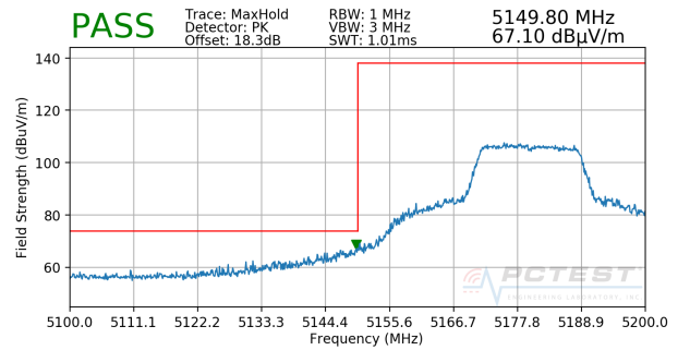
Plot 7-23. Radiated Lower Band Edge Plot MIMO (Peak – UNII Band 1)
