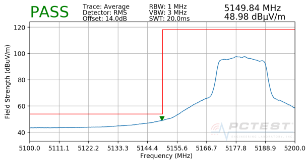
Plot 7-22. Radiated Lower Band Edge Plot MIMO (Average – UNII Band 1)
