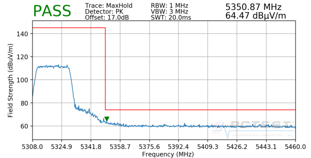
Plot 7-25. Radiated Upper Band Edge Plot MIMO (Peak – UNII Band 2A)
