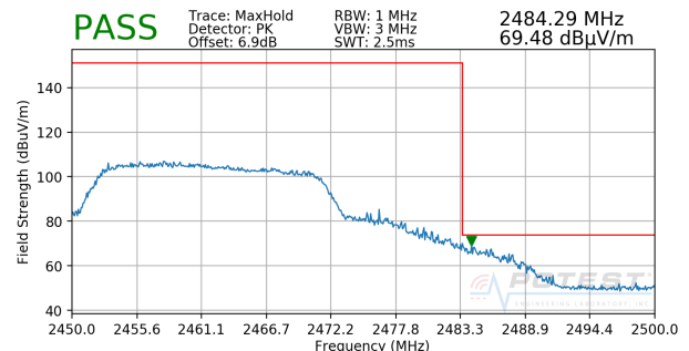
Plot 7-20. Radiated Restricted Upper Band Edge Measurement MIMO (Peak)
