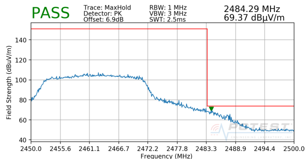
Plot 7-4. Radiated Restricted Upper Band Edge Measurement SISO ANT2 (Peak)
