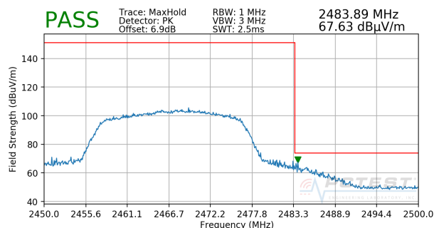
Plot 7-6. Radiated Restricted Upper Band Edge Measurement SISO ANT2 (Peak)
