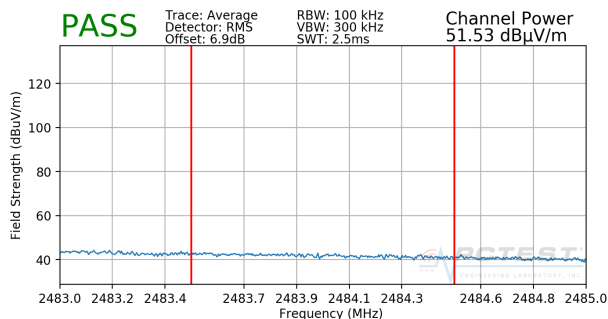
Plot 7-3. Radiated Restricted Upper Band Edge Measurement SISO ANT2 (Average)
