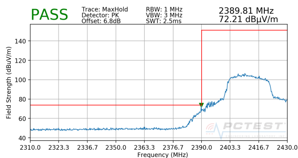
Plot 7-2. Radiated Restricted Lower Band Edge Measurement SISO ANT2 (Peak)
