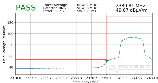
Plot 7-9. Radiated Restricted Lower Band Edge Measurement MIMO (Average)
