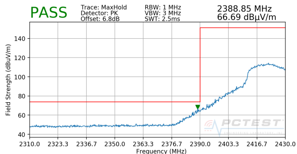
Plot 7-14. Radiated Restricted Lower Band Edge Measurement MIMO (Peak)
