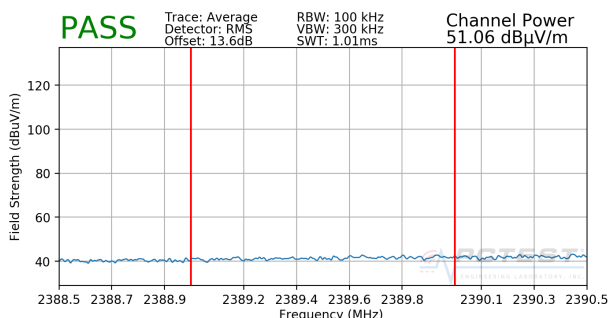
Plot 7-11. Radiated Restricted Lower Band Edge Measurement MIMO (Average)
