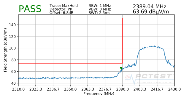
Plot 7-10. Radiated Restricted Lower Band Edge Measurement MIMO (Peak)
