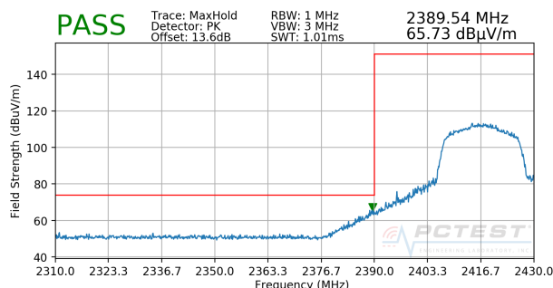
Plot 7-12. Radiated Restricted Lower Band Edge Measurement MIMO (Peak)
