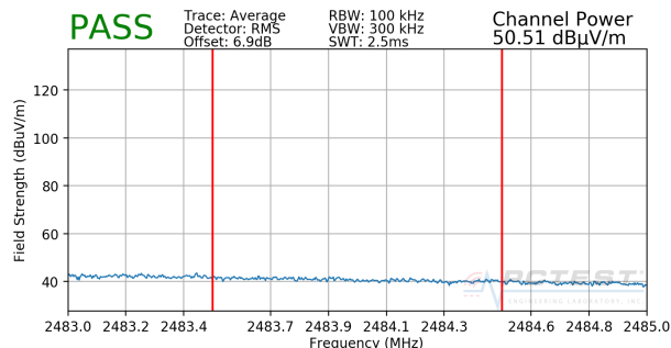
Plot 7-19. Radiated Restricted Upper Band Edge Measurement MIMO (Average)
