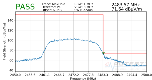
Plot 7-8. Radiated Restricted Upper Band Edge Measurement SISO ANT2 (Peak)
