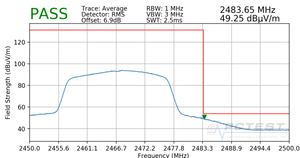
Plot 7-5. Radiated Restricted Upper Band Edge Measurement SISO ANT2 (Average)
