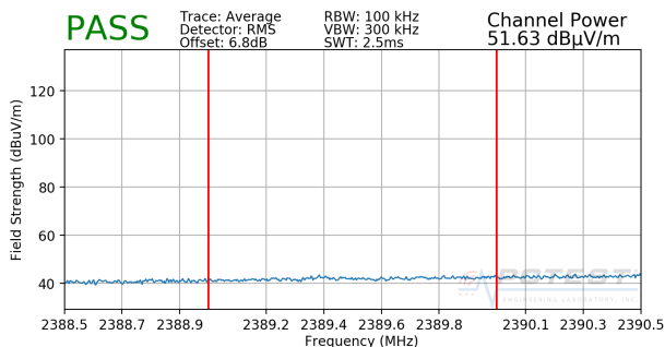
Plot 7-13. Radiated Restricted Lower Band Edge Measurement MIMO (Average)
