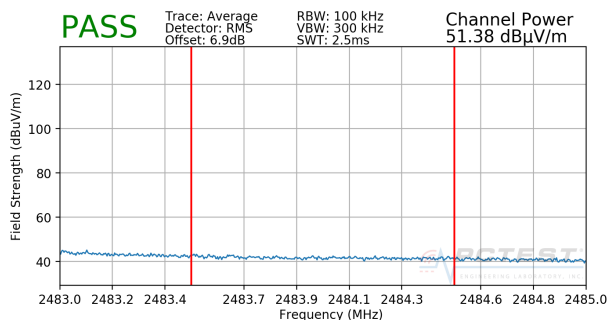
Plot 7-7. Radiated Restricted Upper Band Edge Measurement SISO ANT2 (Average)
