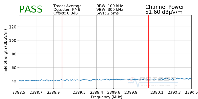
Plot 7-1. Radiated Restricted Lower Band Edge Measurement SISO ANT2 (Average)
