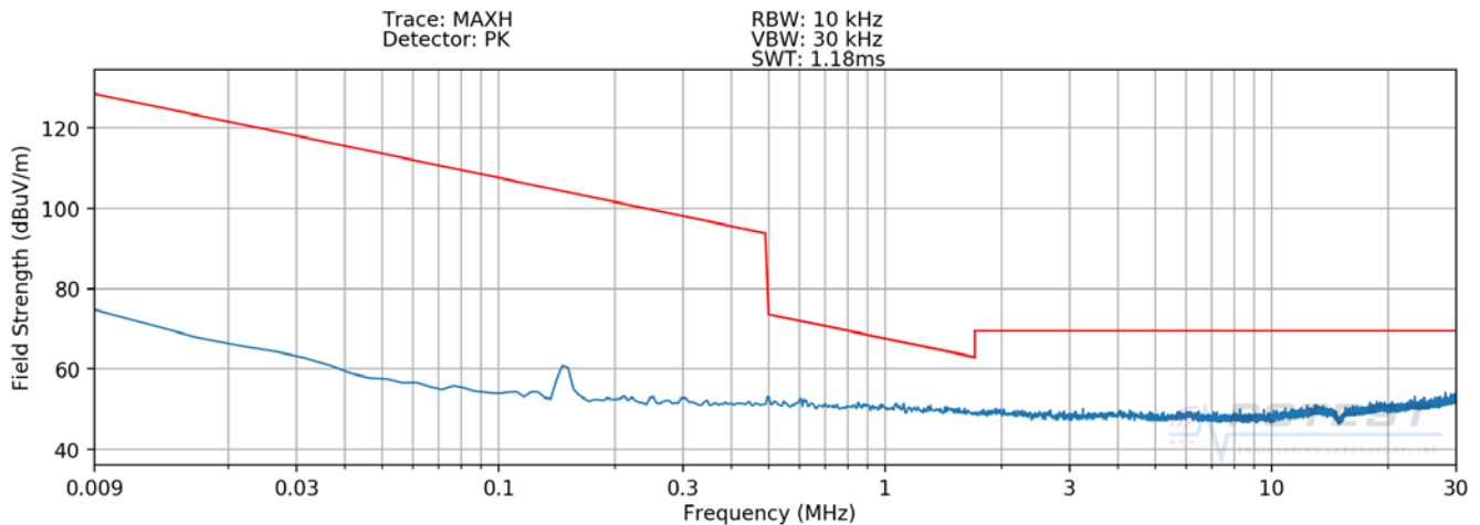
Plot 7-5. Radiated Spurious Plot 9kHz – 30MHz (Pol. Y – WPT with Earbuds)
