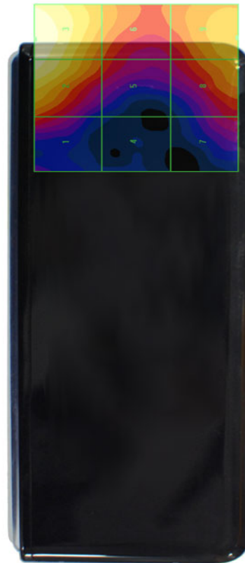
Figure 18-4 E-Field WD Scan overlay
