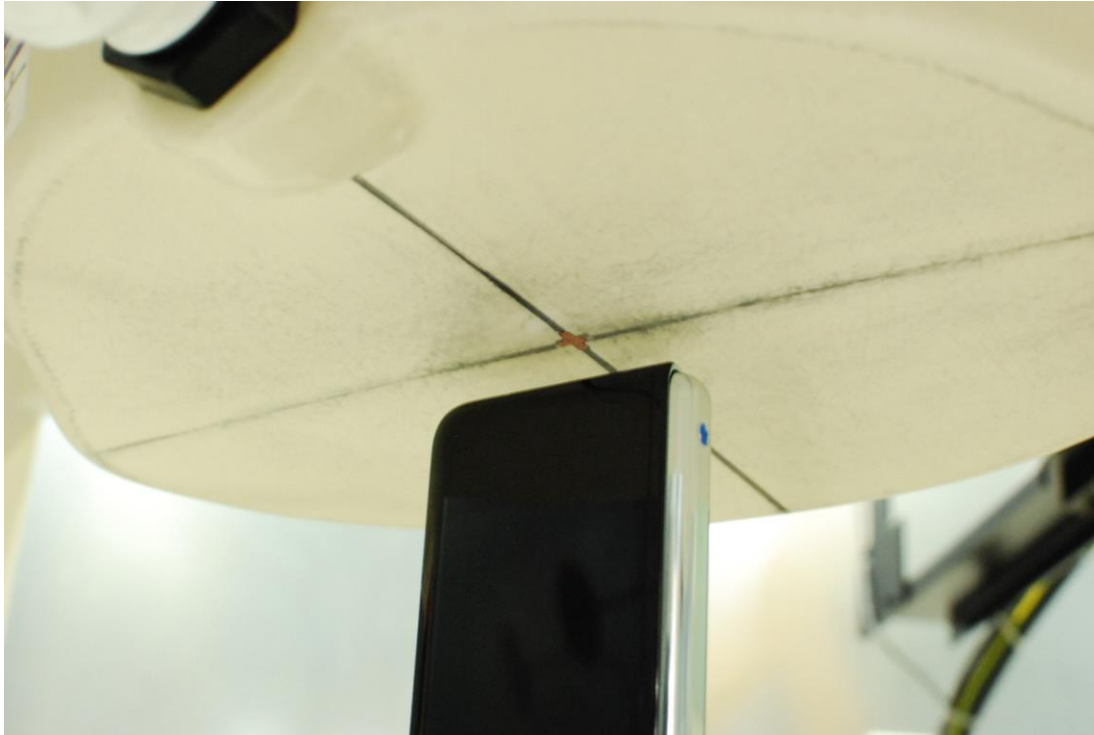
SAR Test Setup Photo 13 – Closed Configuration Bottom Edge at 1.1cm
