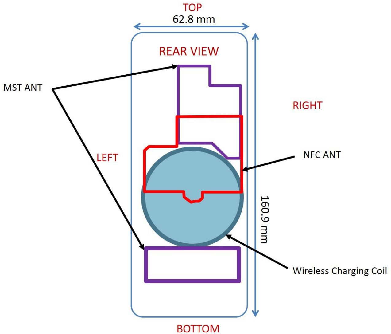
Figure F-2 NFC Antenna Locations
