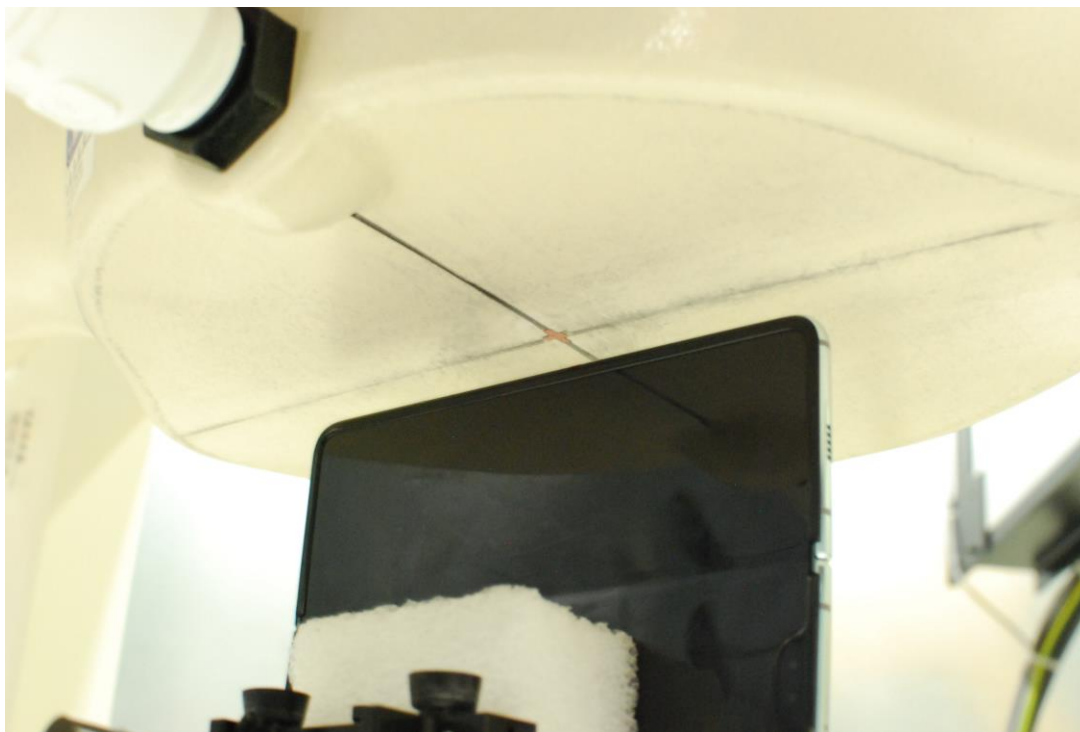
SAR Test Setup Photo 31 – Open Configuration Right Edge at 1.0cm
