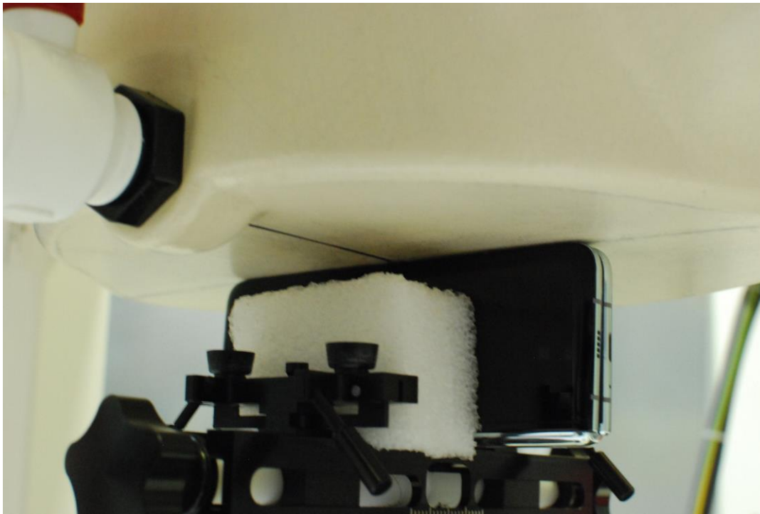
SAR Test Setup Photo 17 – Closed Configuration Right Edge at 0.0cm
