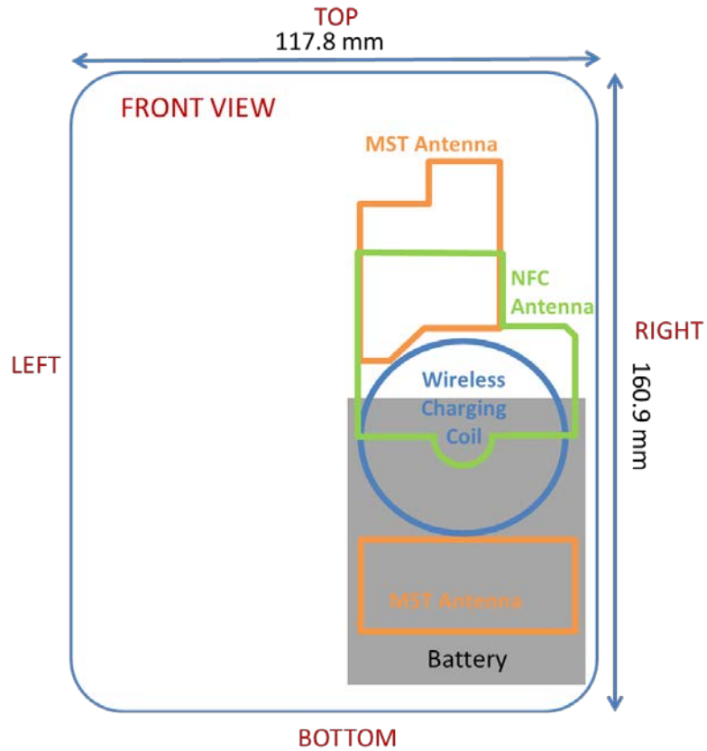
Figure F-3 MST/NFC Antenna and WPC Locations Open Configuration
