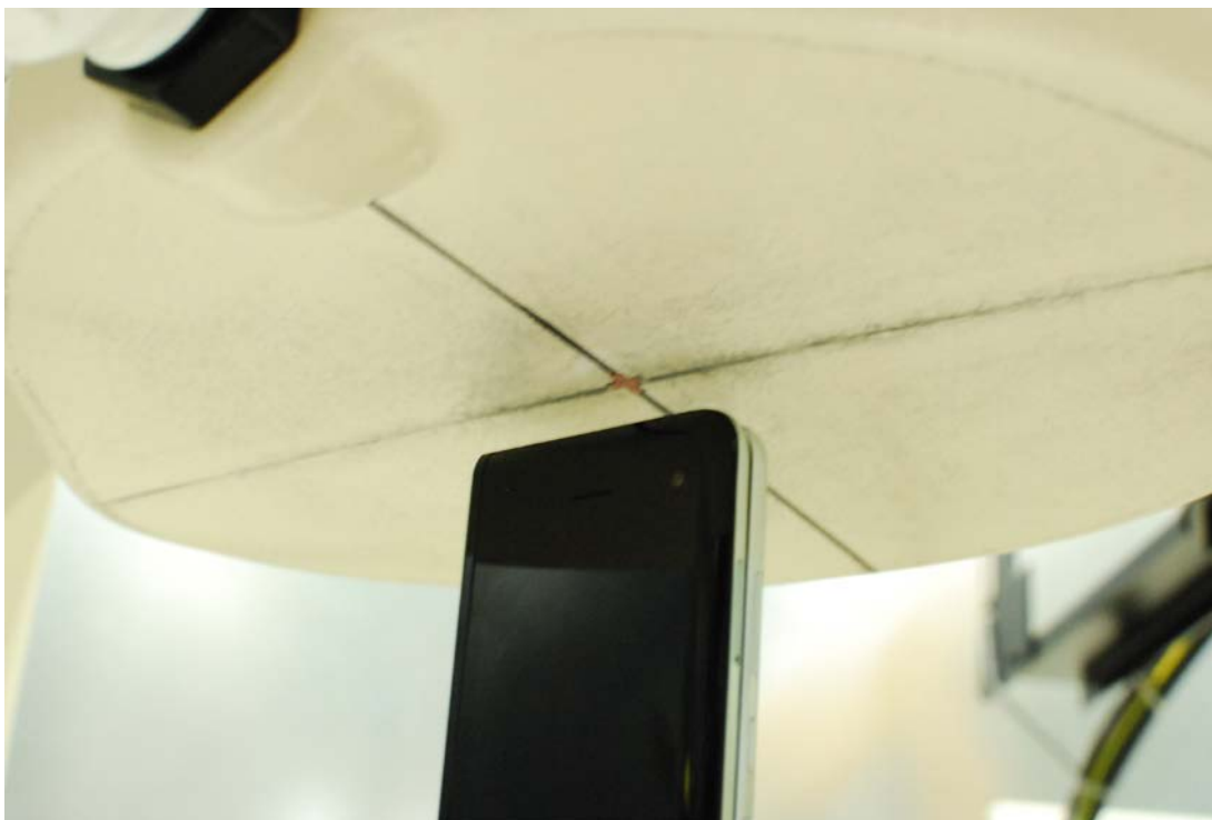
SAR Test Setup Photo 11 – Closed Configuration Top Edge at 1.0cm
