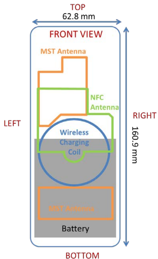
Figure F-2 MST/NFC Antenna and WPC Locations Closed Configuration
