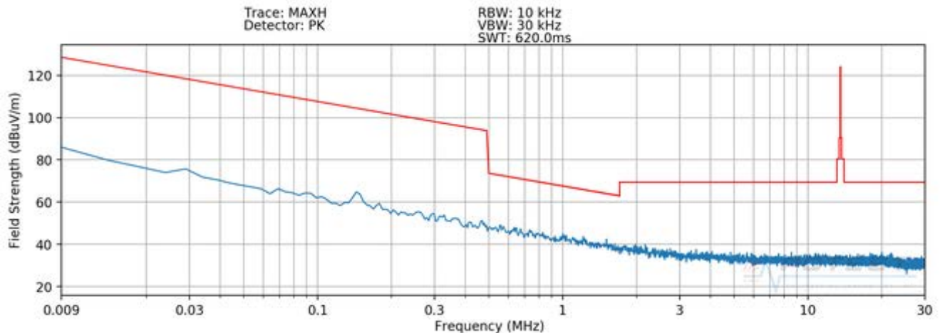
Plot 7-3. Radiated Spurious Plot 9kHz – 30MHz (Pol. Z - WPT)
