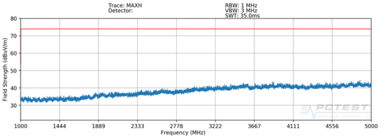
Plot 7-5. Radiated Spurious Plot above 1GHz – H – CLOSED
