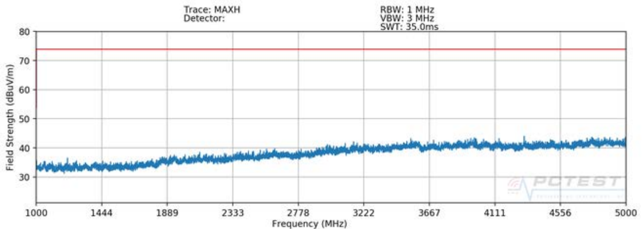
Plot 7-6. Radiated Spurious Plot above 1GHz – V – CLOSED
