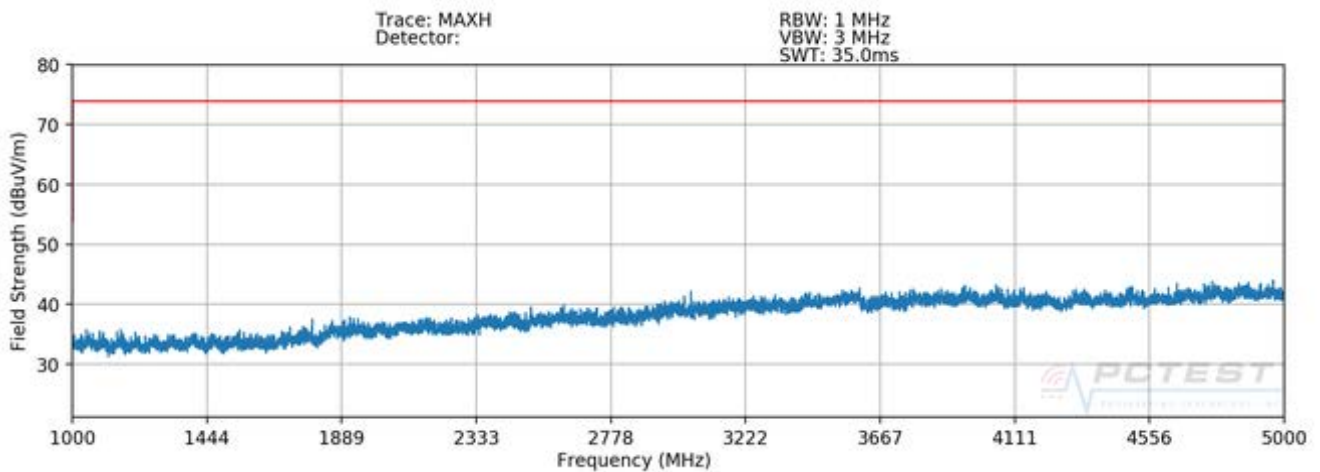
Plot 7-3. Radiated Spurious Plot above 1GHz – H - OPEN
