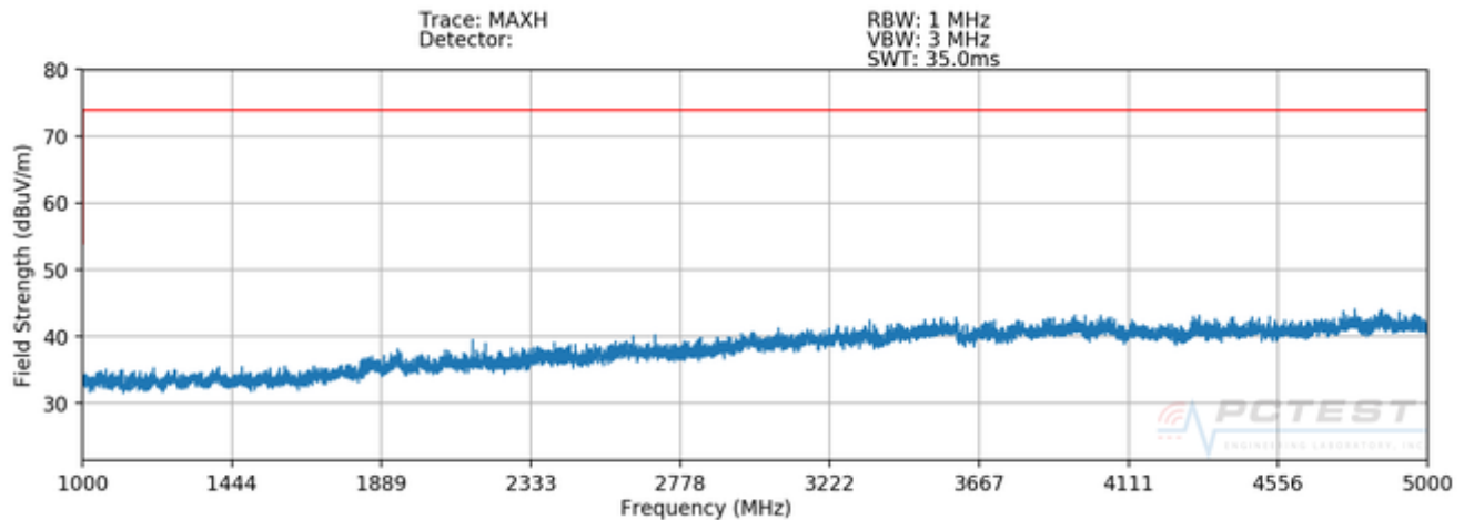
Plot 7-4. Radiated Spurious Plot above 1GHz – V – OPEN
