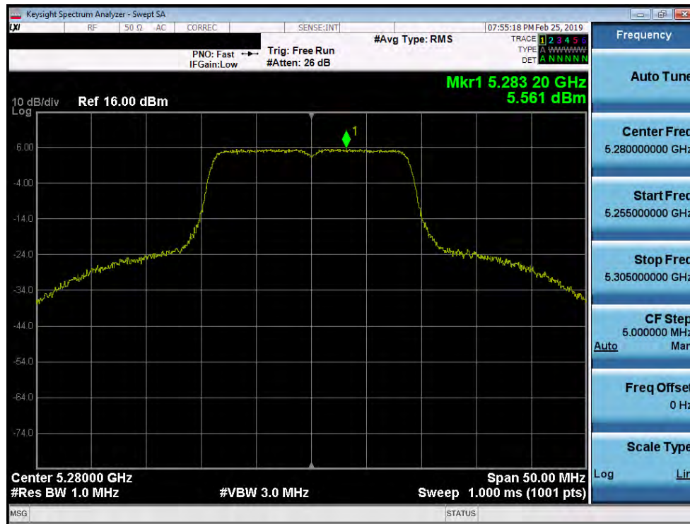
Plot 7-152. Power Spectral Density Plot SISO ANT1 (20MHz BW 802.11n (UNII Band 2A) – Ch. 56)
