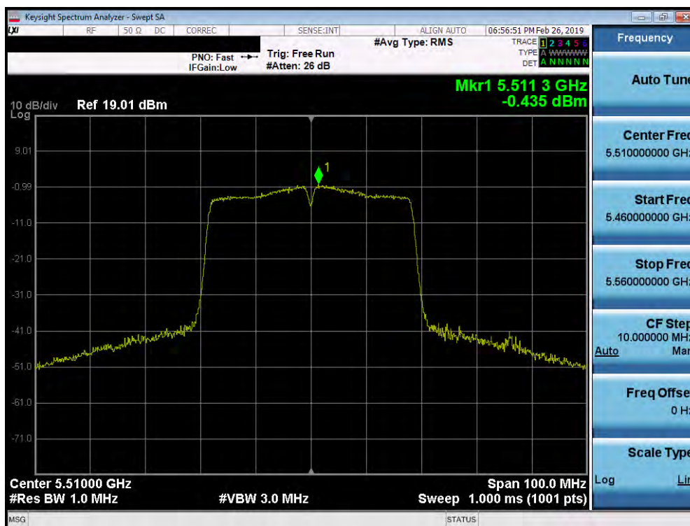
Plot 7-175. Power Spectral Density Plot SISO ANT1 (40MHz BW 802.11ax (UNII Band 2C) – Ch. 102)
