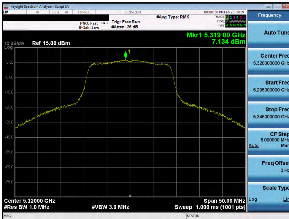
Plot 7-150. Power Spectral Density Plot SISO ANT1 (802.11a (UNII Band 2A) – Ch. 64)
