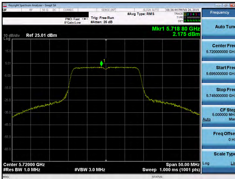
Plot 7-171. Power Spectral Density Plot SISO ANT1 (20MHz BW 802.11ax (UNII Band 2C) – Ch. 144)
