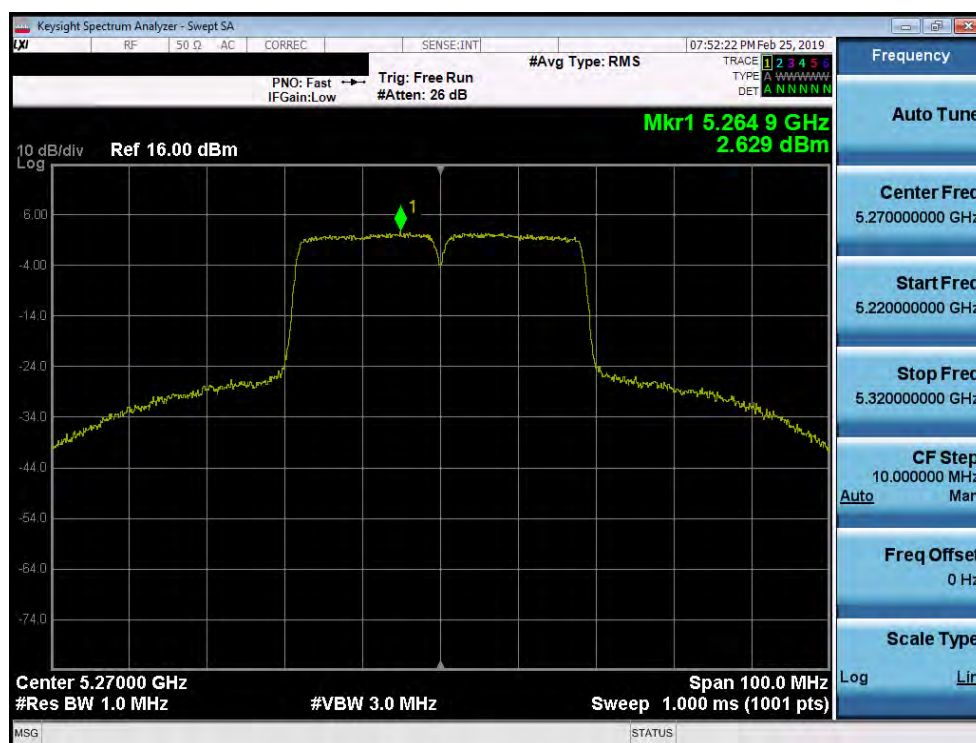
Plot 7-157. Power Spectral Density Plot SISO ANT1 (40MHz BW 802.11n (UNII Band 2A) – Ch. 54)
