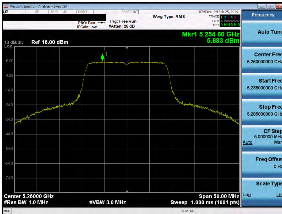
Plot 7-151. Power Spectral Density Plot SISO ANT1 (20MHz BW 802.11n (UNII Band 2A) – Ch. 52)
