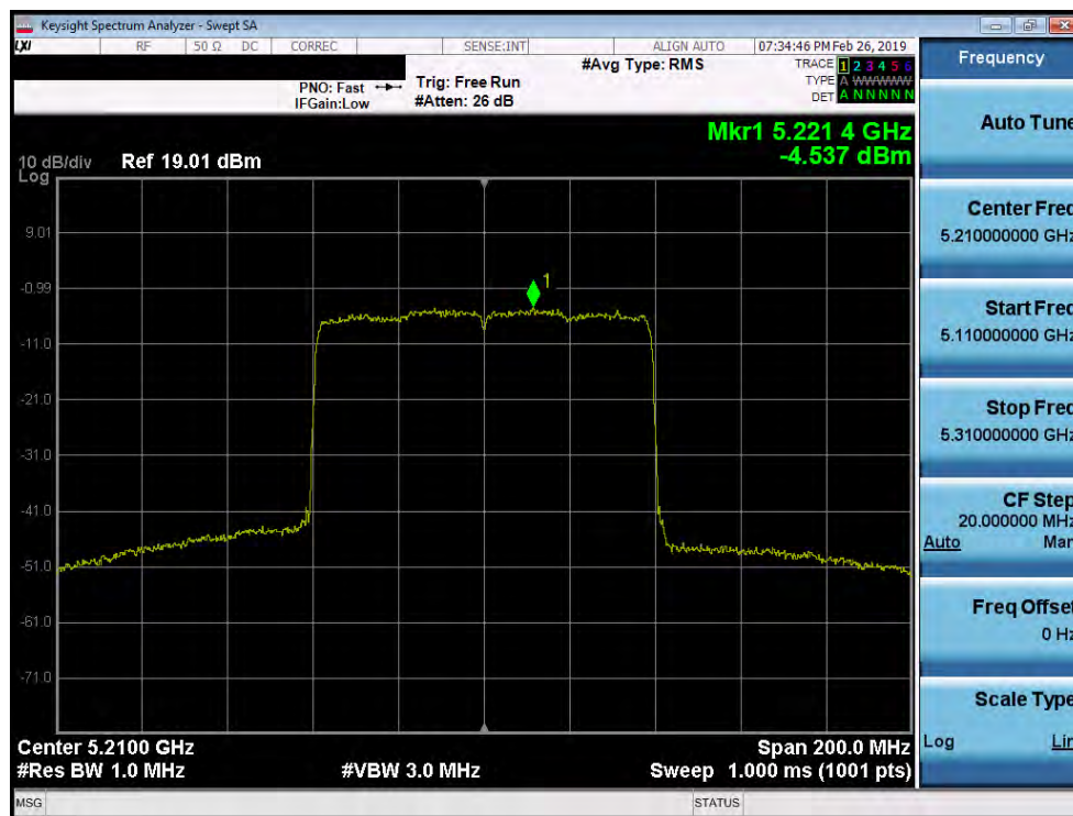
Plot 7-147. Power Spectral Density Plot SISO ANT1 (80MHz BW 802.11ax (UNII Band 1) – Ch. 42)
