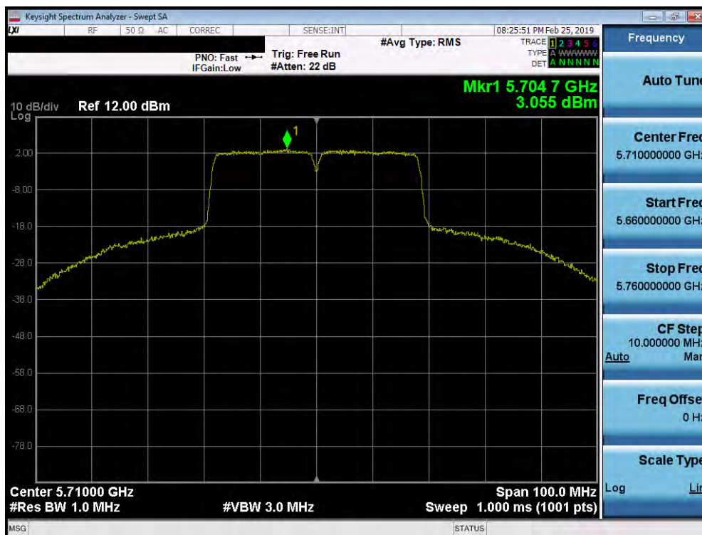
Plot 7-174. Power Spectral Density Plot SISO ANT1 (40MHz BW 802.11n (UNII Band 2C) – Ch. 142)
