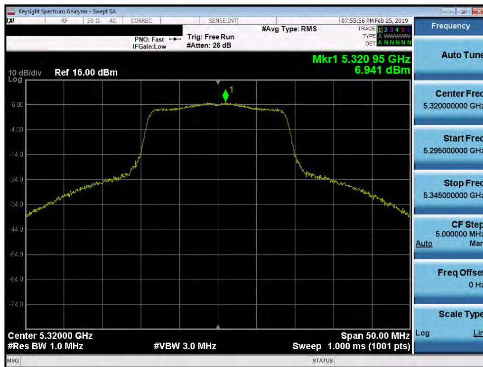
Plot 7-153. Power Spectral Density Plot SISO ANT1 (20MHz BW 802.11n (UNII Band 2A) – Ch. 64)
