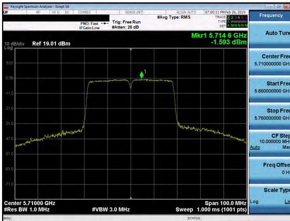
Plot 7-177. Power Spectral Density Plot SISO ANT1 (40MHz BW 802.11ax (UNII Band 2C) – Ch. 142)
