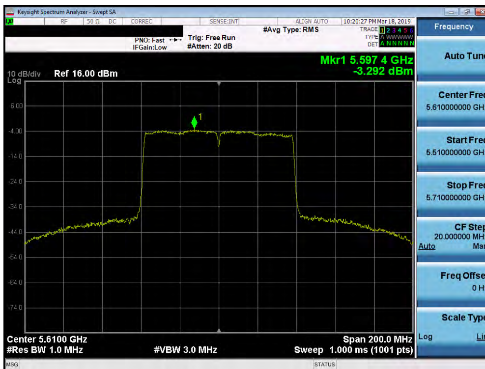
Plot 7-179. Power Spectral Density Plot SISO ANT1 (80MHz BW 802.11ac (UNII Band 2C) – Ch. 122)
