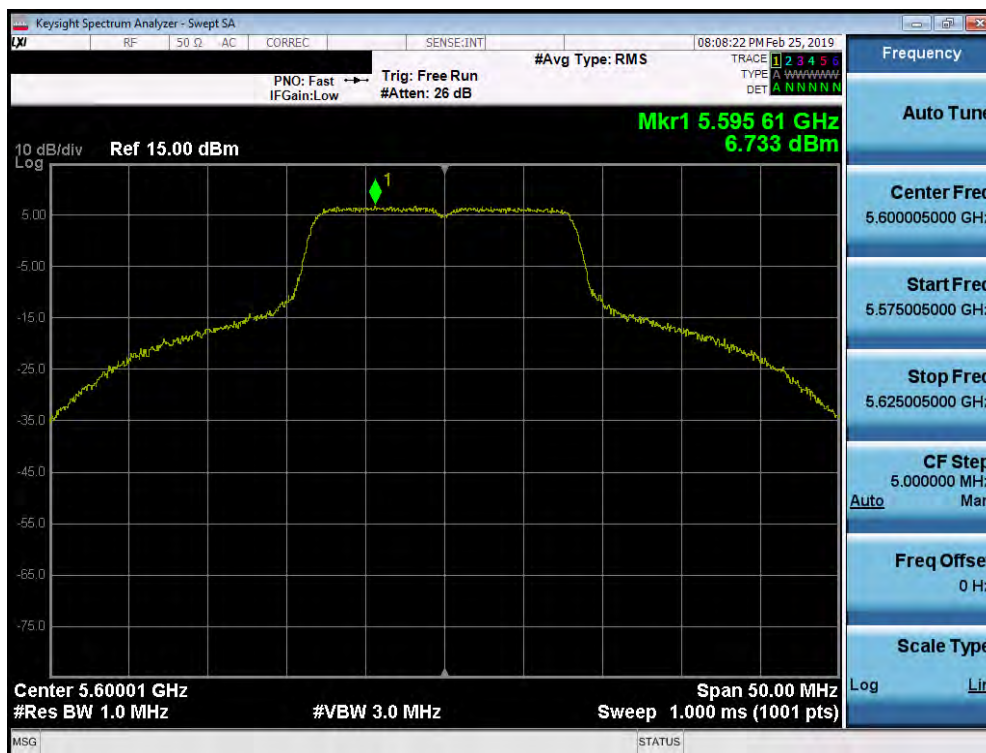
Plot 7-164. Power Spectral Density Plot SISO ANT1 (802.11a (UNII Band 2C) – Ch. 120)
