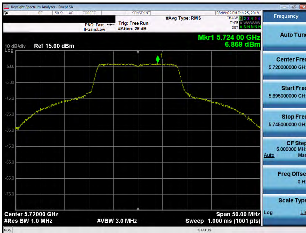
Plot 7-165. Power Spectral Density Plot SISO ANT1 (802.11a (UNII Band 2C) – Ch. 144)
