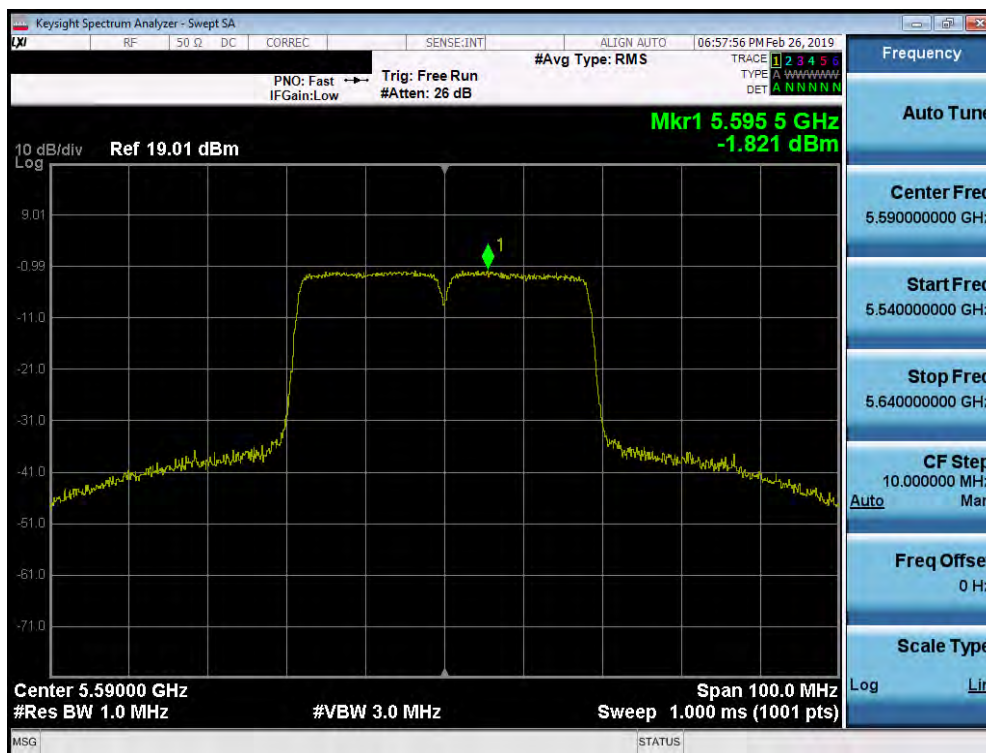
Plot 7-176. Power Spectral Density Plot SISO ANT1 (40MHz BW 802.11ax (UNII Band 2C) – Ch. 118)
