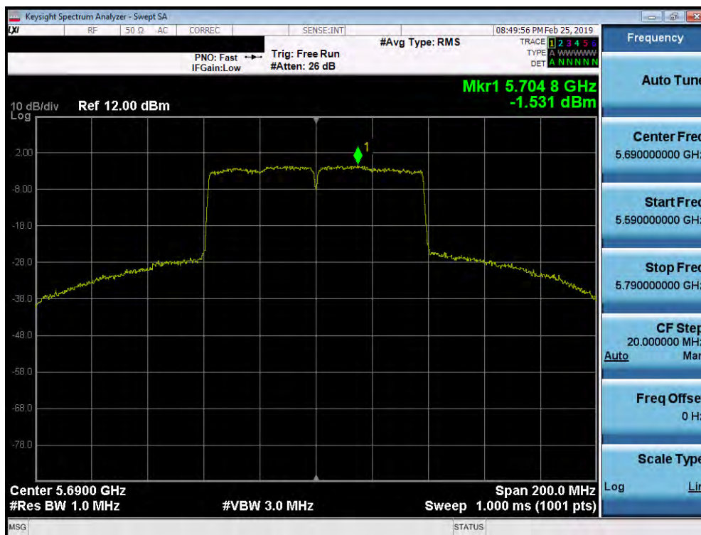
Plot 7-180. Power Spectral Density Plot SISO ANT1 (80MHz BW 802.11ac (UNII Band 2C) – Ch. 138)
