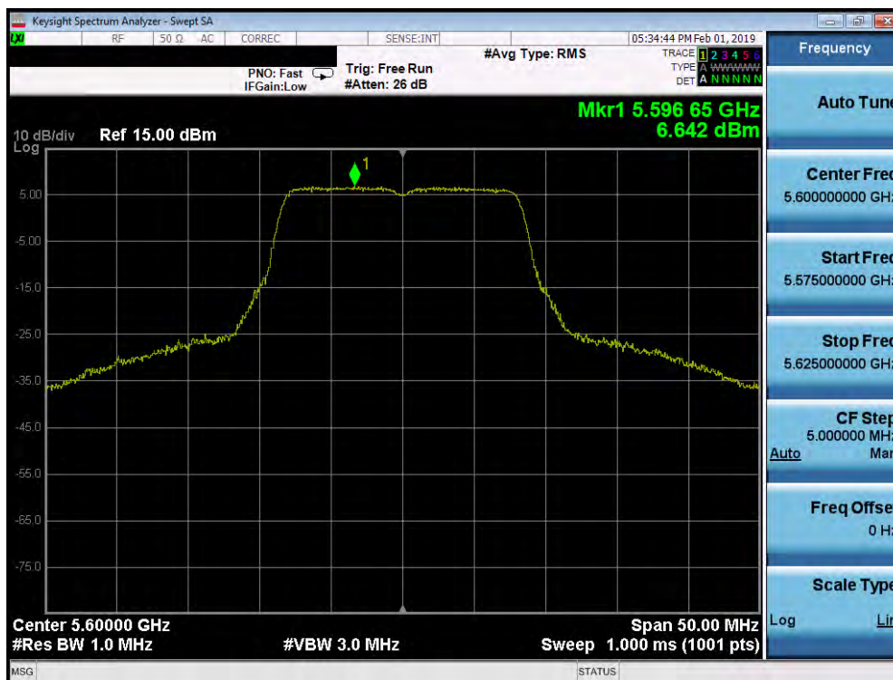
Plot 7-230. Power Spectral Density Plot SISO ANT2 (802.11a (UNII Band 2C) – Ch. 120)
