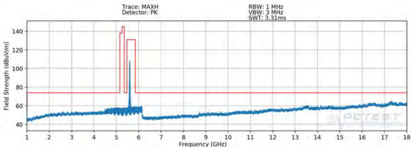
Plot 7-270. Radiated Spurious Plot above 1GHz SISO ANT1 (802.11a – U2C Ch. 120 - OPEN)
