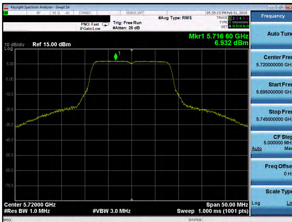
Plot 7-231. Power Spectral Density Plot SISO ANT2 (802.11a (UNII Band 2C) – Ch. 144)
