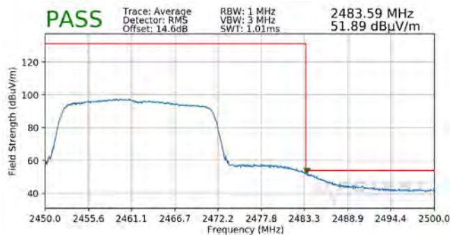
Plot 7-157. Radiated Restricted Band Edge Measurement MIMO with WCP (Average – 242 Tones)
