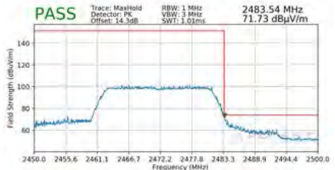
Plot 7-132. Radiated Restricted Upper Band Edge Measurement SISO ANT2 (Peak - 242 Tones)
