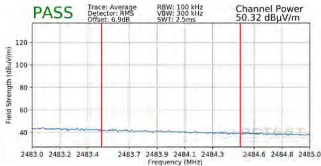
Plot 7-149. Radiated Restricted Upper Band Edge Measurement MIMO (Average – 242 Tones)
