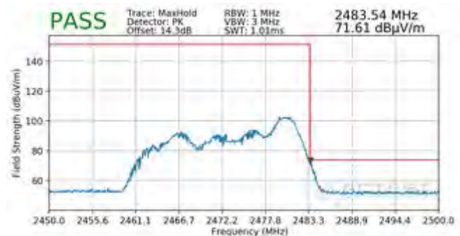
Plot 7-144. Radiated Restricted Upper Band Edge Measurement MIMO (Peak – 26 Tones)
