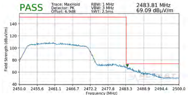
Plot 7-152. Radiated Restricted Upper Band Edge Measurement MIMO (Peak – 242 Tones)
