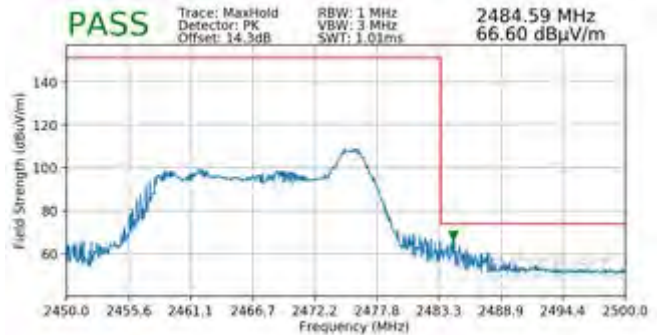
Plot 7-120. Radiated Restricted Upper Band Edge Measurement SISO ANT2 (Peak – 26 Tones)
