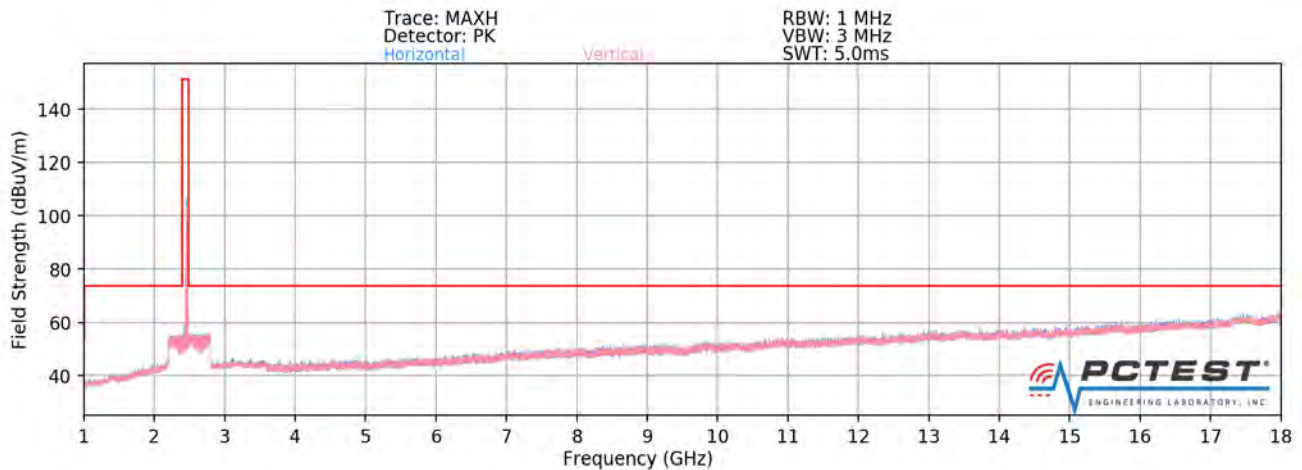
Plot 7-75. Radiated Spurious Plot above 1GHz SISO ANT2 (802.11ax OFDMA - 106 Tones - Ch. 11 - CLOSED)
