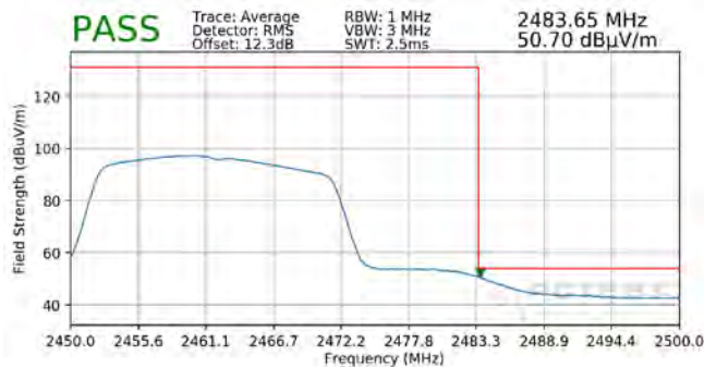
Plot 7-107. Radiated Restricted Upper Band Edge Measurement SISO ANT1 (Average – 242 Tones)
