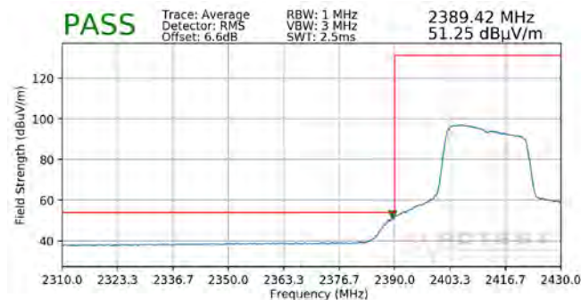
Plot 7-123. Radiated Restricted Lower Band Edge Measurement SISO ANT2 (Average – 242 Tones)
