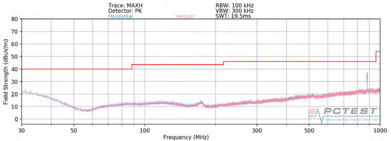
Plot 7-164. Radiated Spurious Plot below 1GHz MIMO (242 Tones - CLOSED)
