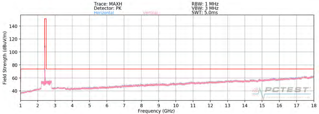
Plot 7-65. Radiated Spurious Plot above 1GHz SISO ANT1 (802.11ax OFDMA - 106 Tones - Ch. 1 - CLOSED)
