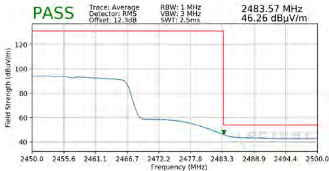
Plot 7-125. Radiated Restricted Upper Band Edge Measurement SISO ANT2 (Average – 242 Tones)
