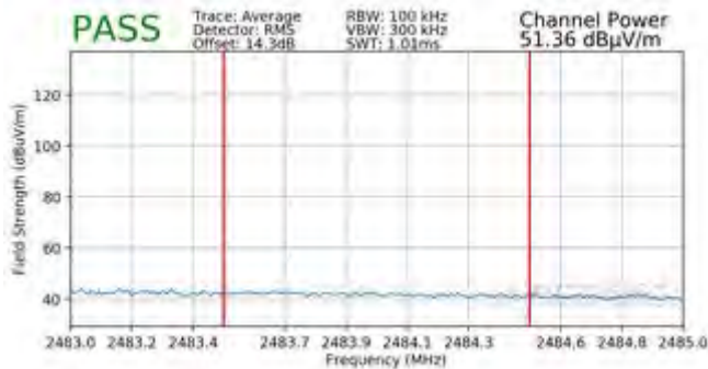
Plot 7-129. Radiated Restricted Upper Band Edge Measurement SISO ANT2 (Average - 242 Tones)
