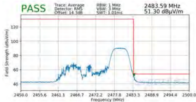
Plot 7-121. Radiated Restricted Upper Band Edge Measurement SISO ANT2 (Average – 52 Tones)
