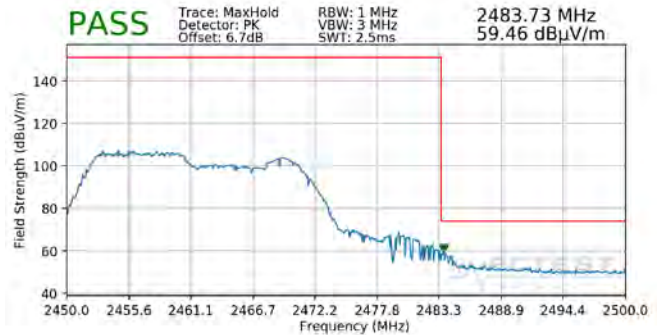
Plot 7-118. Radiated Restricted Upper Band Edge Measurement SISO ANT2 (Peak – 106 Tones)
