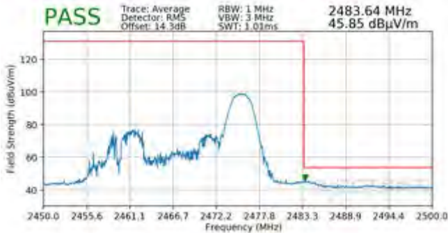
Plot 7-119. Radiated Restricted Upper Band Edge Measurement SISO ANT2 (Average – 26 Tones)
