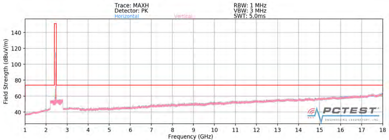
Plot 7-67. Radiated Spurious Plot above 1GHz SISO ANT1 (802.11ax OFDMA - 106 Tones - Ch. 11 - CLOSED)
