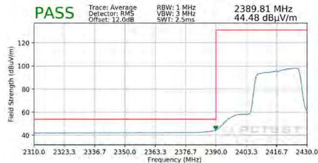
Plot 7-147. Radiated Restricted Lower Band Edge Measurement MIMO (Average – 242 Tones)
