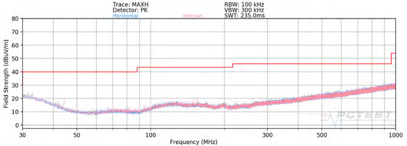
Plot 7-161. Radiated Spurious Plot below 1GHz SISO ANT2 (106 Tones - CLOSED)
