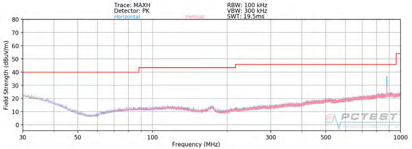
Plot 7-163. Radiated Spurious Plot below 1GHz MIMO (106 Tones - CLOSED)
