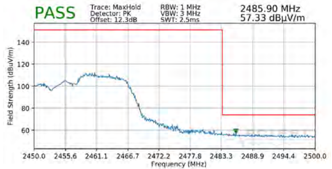
Plot 7-138. Radiated Restricted Upper Band Edge Measurement MIMO (Peak – 106 Tones)
