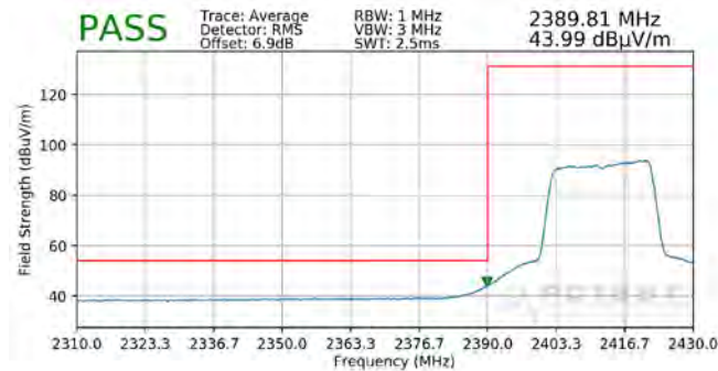
Plot 7-145. Radiated Restricted Lower Band Edge Measurement MIMO (Average – 242 Tones)
