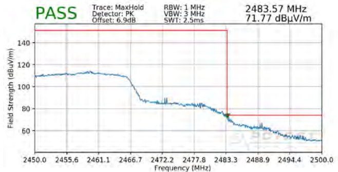
Plot 7-150. Radiated Restricted Upper Band Edge Measurement MIMO (Peak – 242 Tones)
