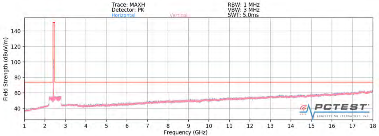
Plot 7-73. Radiated Spurious Plot above 1GHz SISO ANT2 (802.11ax OFDMA - 106 Tones - Ch. 1 - CLOSED)
