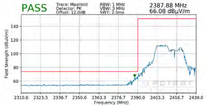
Plot 7-90. Radiated Restricted Lower Band Edge Measurement SISO ANT1 (Peak – 106 Tones)
