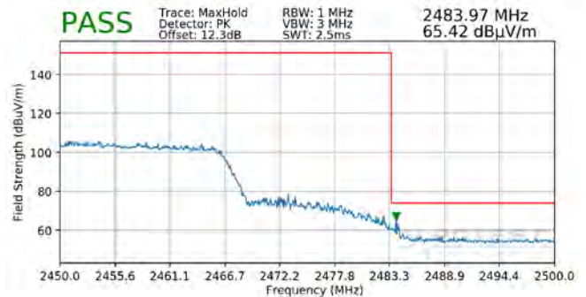
Plot 7-126. Radiated Restricted Upper Band Edge Measurement SISO ANT2 (Peak – 242 Tones)
