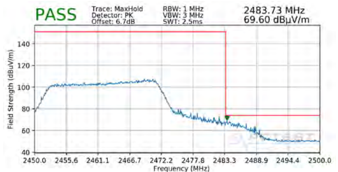
Plot 7-128. Radiated Restricted Upper Band Edge Measurement SISO ANT2 (Peak – 242 Tones)
