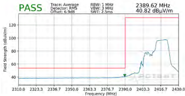
Plot 7-133. Radiated Restricted Lower Band Edge Measurement MIMO (Average – 106 Tones)
