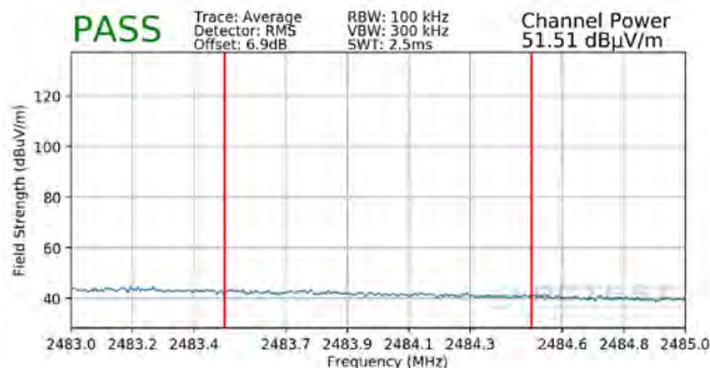
Plot 7-151. Radiated Restricted Upper Band Edge Measurement MIMO (Average – 242 Tones)
