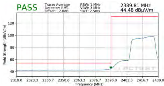
Plot 7-135. Radiated Restricted Lower Band Edge Measurement MIMO (Average – 106 Tones)
