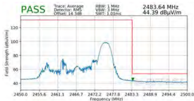
Plot 7-141. Radiated Restricted Upper Band Edge Measurement MIMO (Average – 26 Tones)
