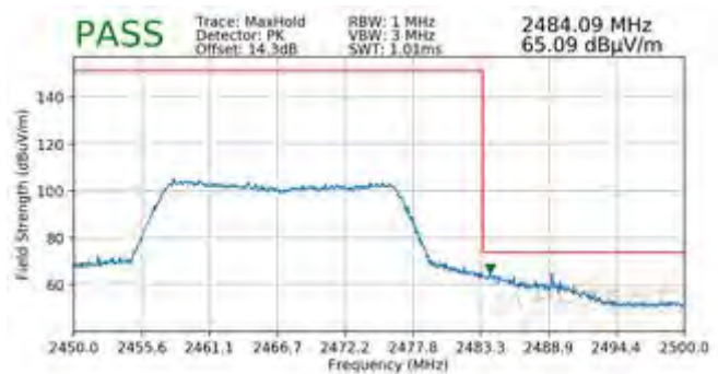
Plot 7-154. Radiated Restricted Upper Band Edge Measurement MIMO (Peak - 242 Tones)
