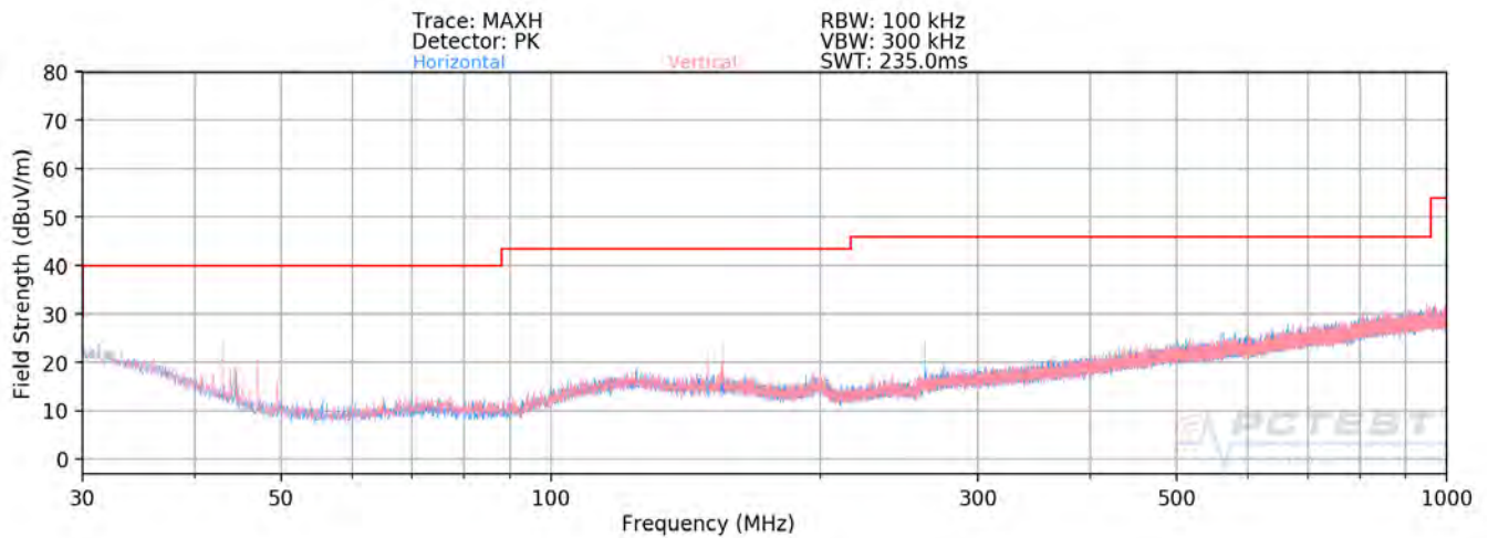
Plot 7-160. Radiated Spurious Plot below 1GHz SISO ANT1 (242 Tones - CLOSED)
