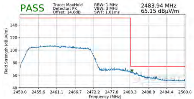
Plot 7-158. Radiated Restricted Band Edge Measurement MIMO with WCP (Peak – 242 Tones)
