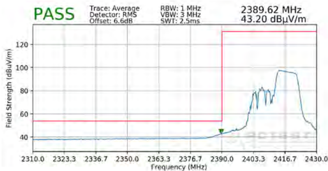
Plot 7-113. Radiated Restricted Lower Band Edge Measurement SISO ANT2 (Average – 106 Tones)
