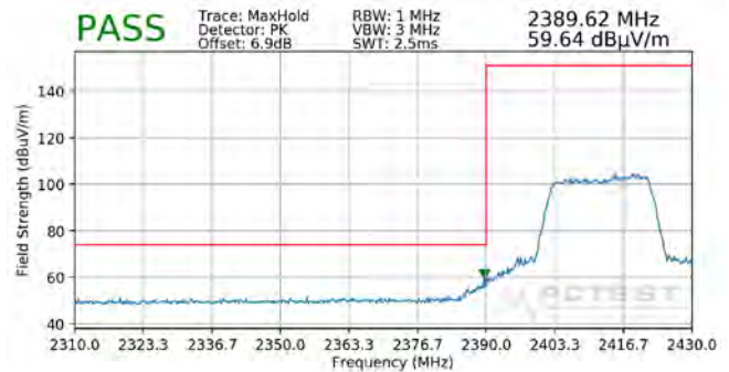
Plot 7-146. Radiated Restricted Lower Band Edge Measurement MIMO (Peak – 242 Tones)
