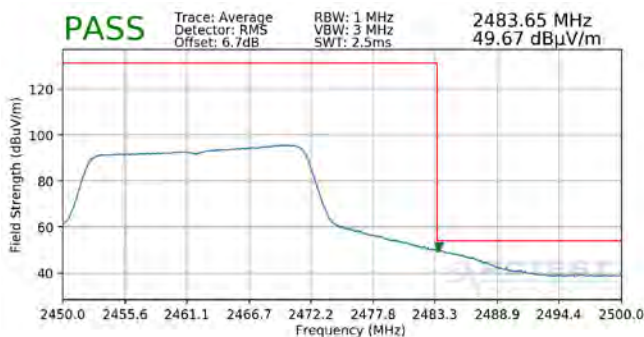
Plot 7-127. Radiated Restricted Upper Band Edge Measurement SISO ANT2 (Average – 242 Tones)
