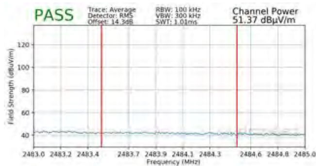
Plot 7-153. Radiated Restricted Upper Band Edge Measurement MIMO (Average - 242 Tones)
