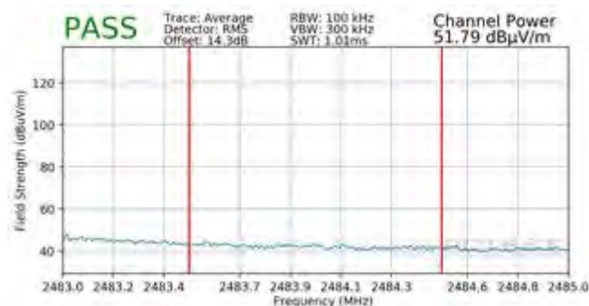
Plot 7-155. Radiated Restricted Upper Band Edge Measurement MIMO (Average - 242 Tones)
