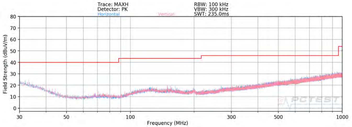
Plot 7-162. Radiated Spurious Plot below 1GHz SISO ANT2 (242 Tones - CLOSED)
