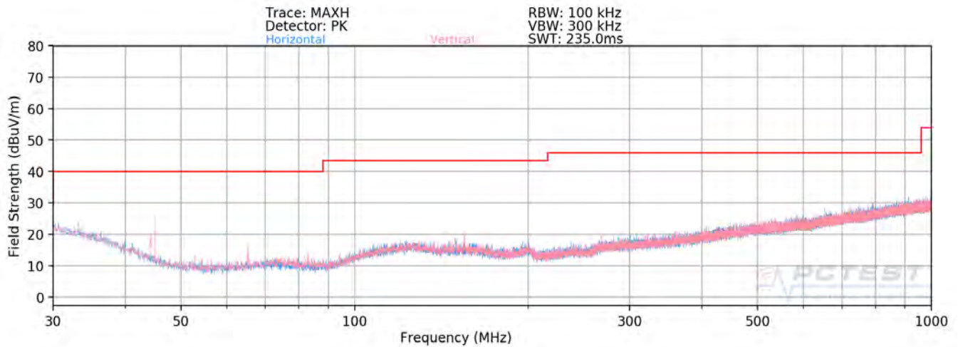
Plot 7-159. Radiated Spurious Plot below 1GHz SISO ANT1 (106 Tones - CLOSED)
