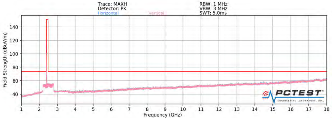
Plot 7-81. Radiated Spurious Plot above 1GHz MIMO (802.11ax OFDMA – 106 Tones – Ch. 1 – CLOSED)
