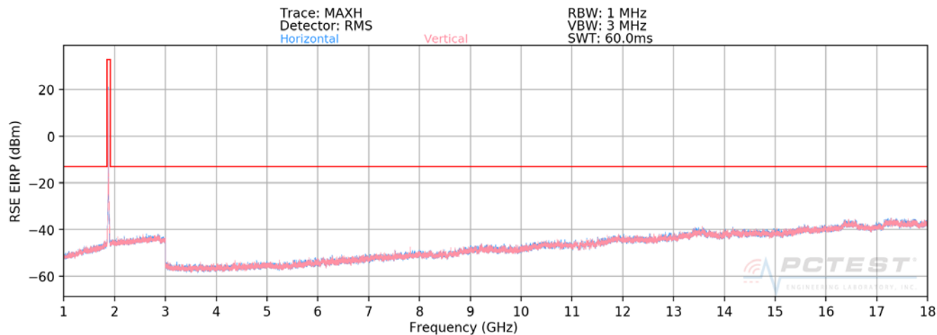
Plot 7-85. Radiated Spurious Plot above 1GHz (PCS WCDMA Mode - OPEN)
