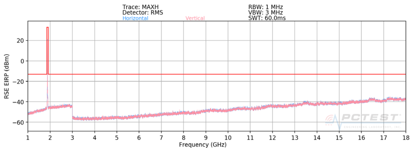
Plot 7-83. Radiated Spurious Plot above 1GHz (PCS GPRS Mode - OPEN)
