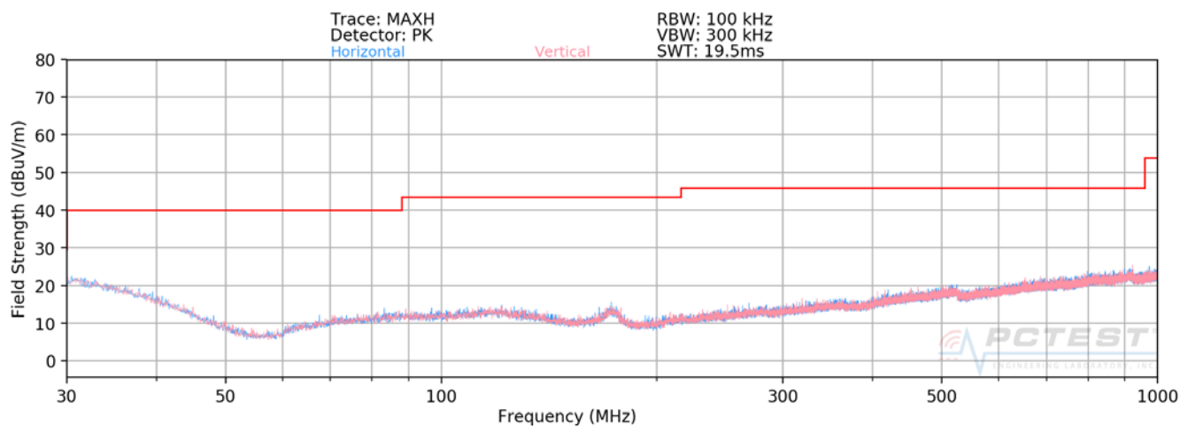
Plot 7-57. Radiated Spurious Plot below 1GHz - CLOSED
