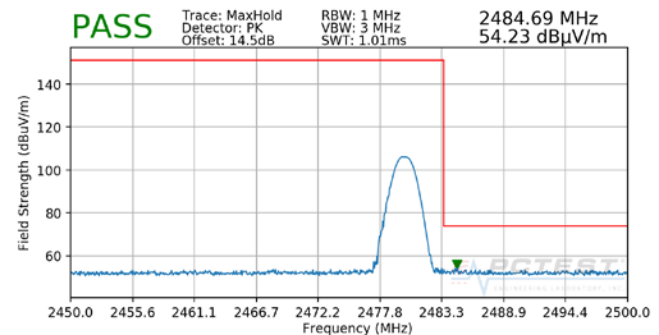
Plot 7-53. Radiated Restricted Upper Band Edge Measurement (Peak - CLOSED)
