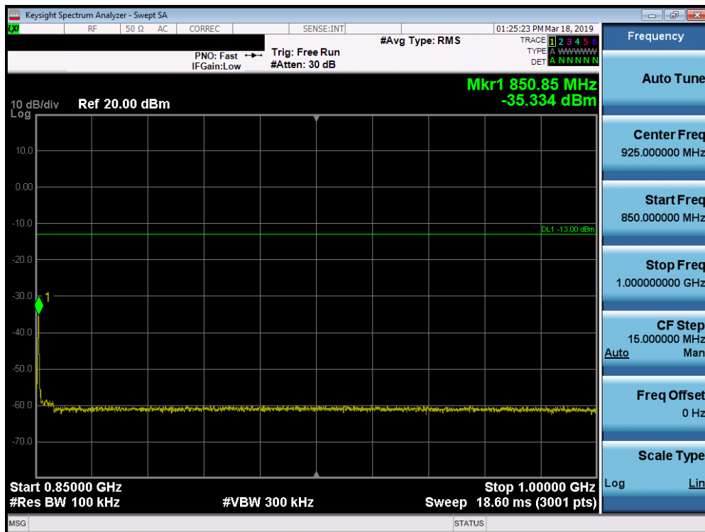
Plot 7-20. Conducted Spurious Plot (LTE Band 26, 5.0MHz QPSK – RB Size 1, RB Offset 0 – High Channel)
