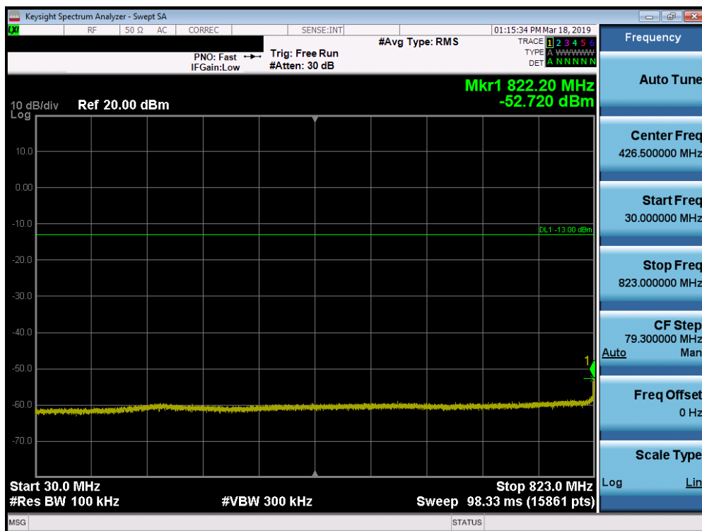
Plot 7-16. Conducted Spurious Plot (LTE Band 26, 5.0MHz QPSK – RB Size 1, RB Offset 0 – Low Channel)
