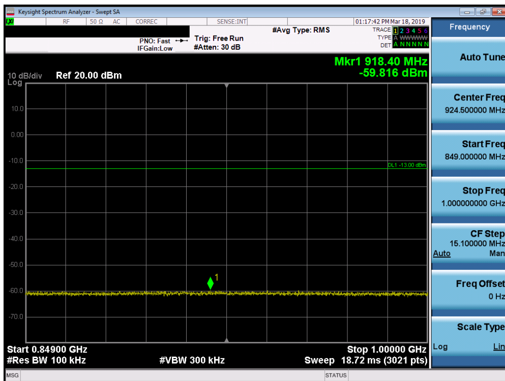
Plot 7-17. Conducted Spurious Plot (LTE Band 26, 5.0MHz QPSK – RB Size 1, RB Offset 0 – Low Channel)
