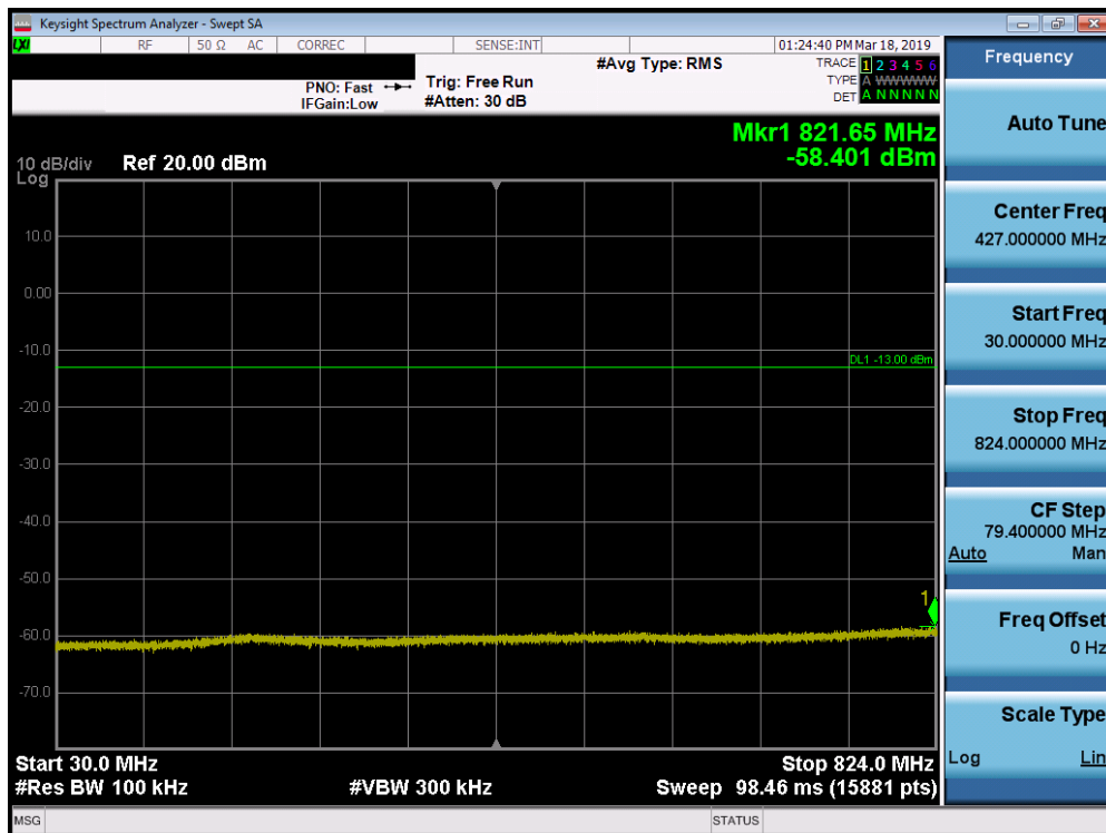
Plot 7-19. Conducted Spurious Plot (LTE Band 26, 5.0MHz QPSK – RB Size 1, RB Offset 0 – High Channel)
