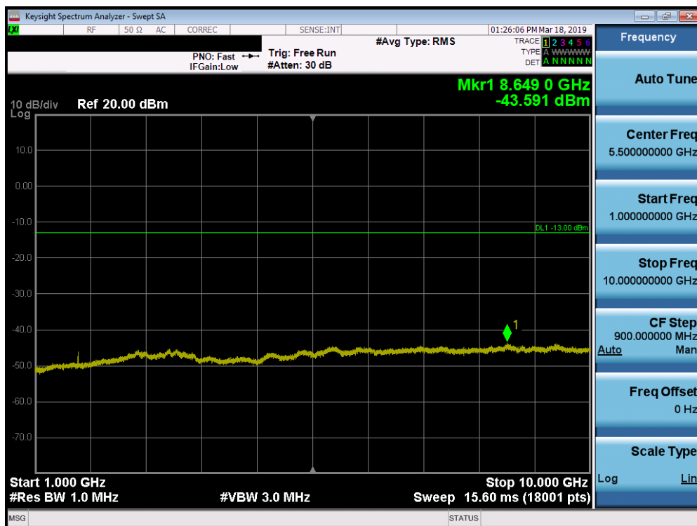
Plot 7-21. Conducted Spurious Plot (LTE Band 26, 5.0MHz QPSK – RB Size 1, RB Offset 0 – High Channel)
