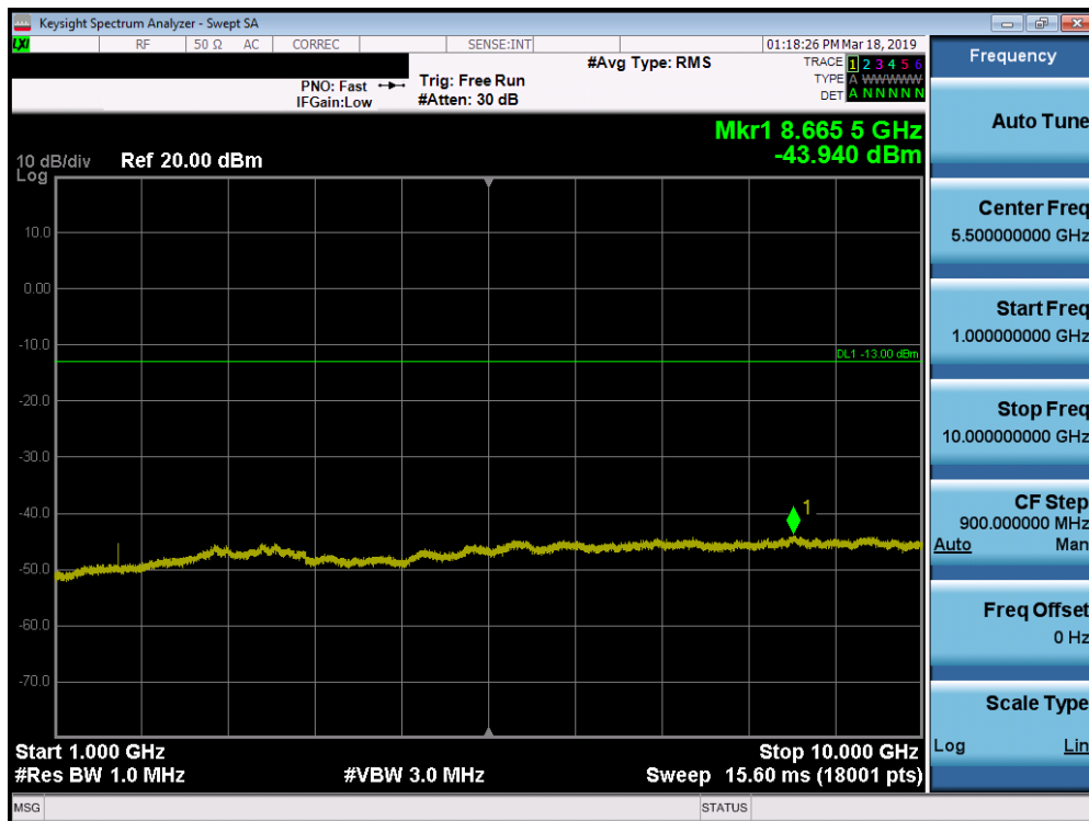
Plot 7-18. Conducted Spurious Plot (LTE Band 26, 5.0MHz QPSK – RB Size 1, RB Offset 0 – Low Channel)
