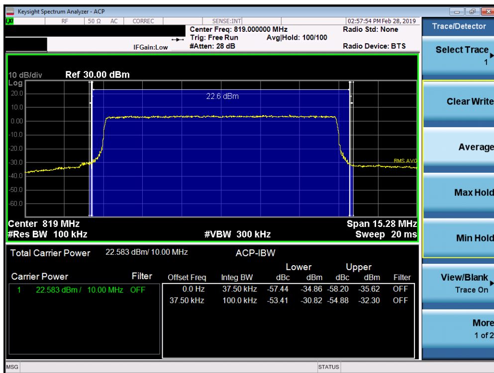
Plot 7-28. Channel Edge Plot (LTE Band 26, 10MHz QPSK – RB Size 50)
