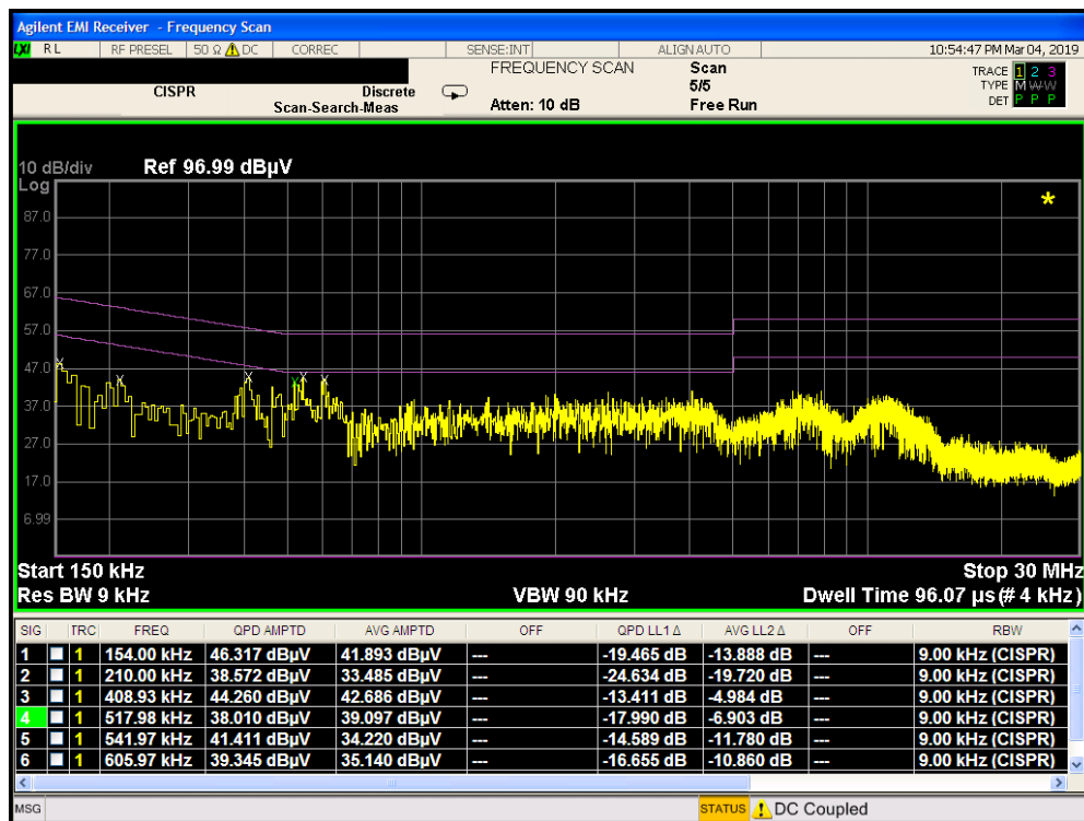
Plot 7-8. Line-Conducted Test Plot Terminated at 50 Ohms(L1)
