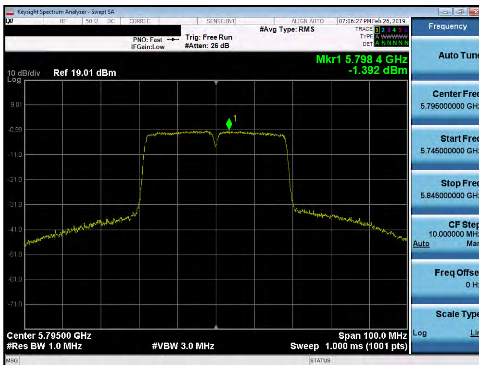
Plot 7-196. Power Spectral Density Plot SISO ANT1 (40MHz BW 802.11ax (UNII Band 3) – Ch. 159)
