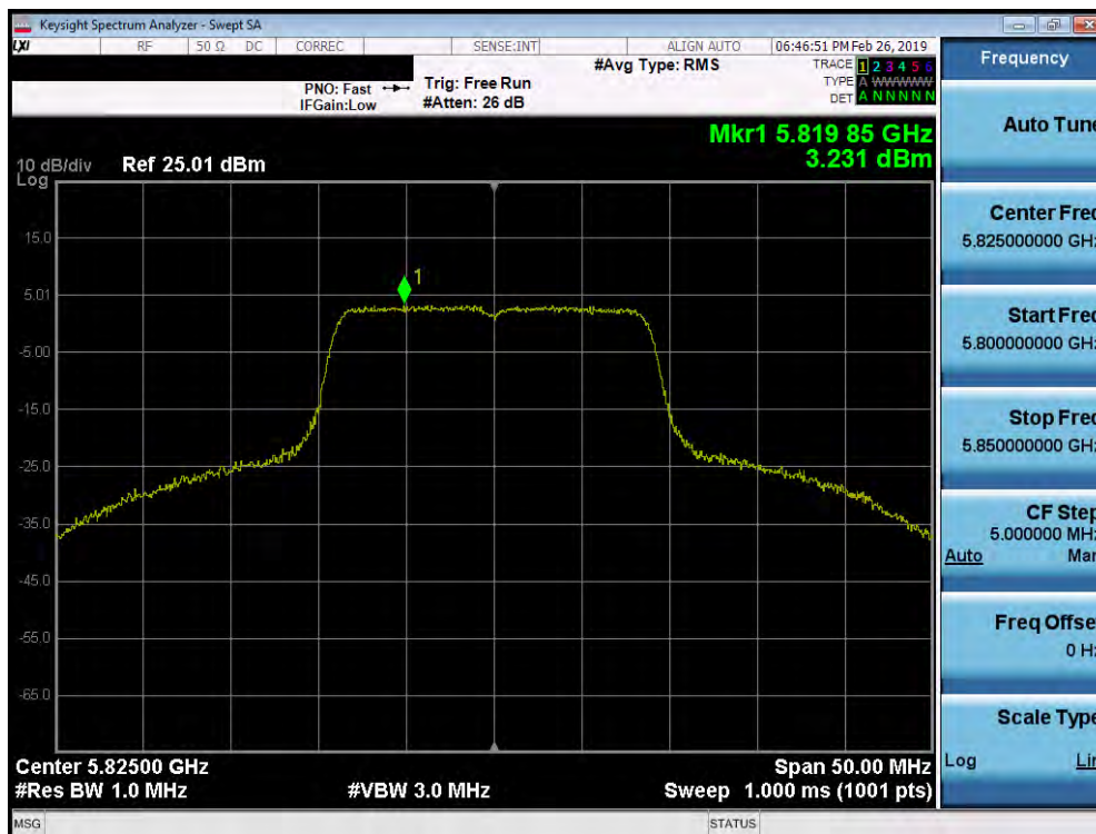
Plot 7-192. Power Spectral Density Plot SISO ANT1 (20MHz BW 802.11ax (UNII Band 3) – Ch. 165)
