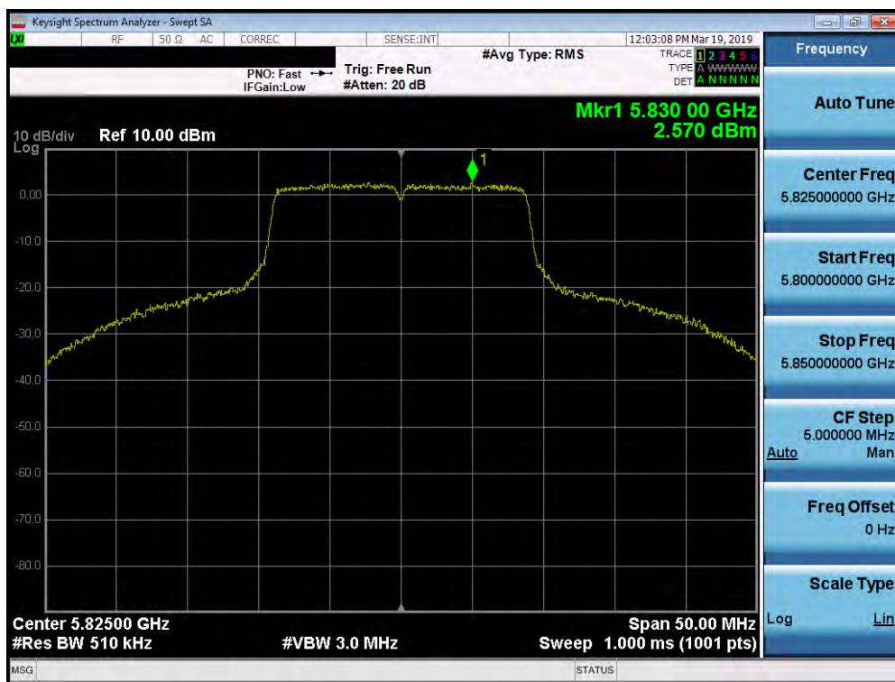
Plot 7-186. Power Spectral Density Plot SISO ANT1 (802.11a (UNII Band 3) – Ch. 165)
