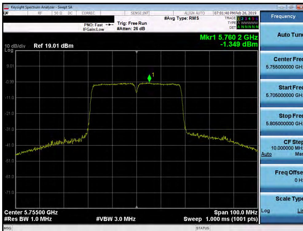
Plot 7-195. Power Spectral Density Plot SISO ANT1 (40MHz BW 802.11ax (UNII Band 3) – Ch. 151)
