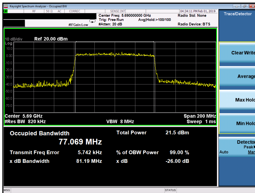
Plot 7-102. 26dB Bandwidth Plot SISO ANT2 (80MHz BW 802.11ax (UNII Band 2C) – Ch. 138)
