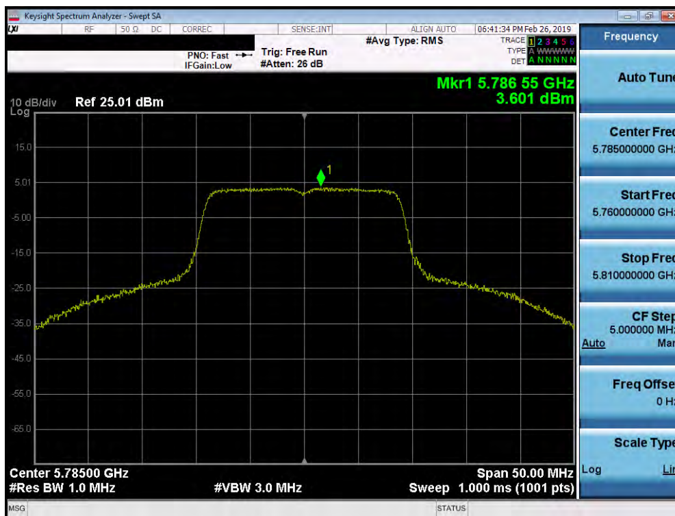
Plot 7-191. Power Spectral Density Plot SISO ANT1 (20MHz BW 802.11ax (UNII Band 3) – Ch. 157)
