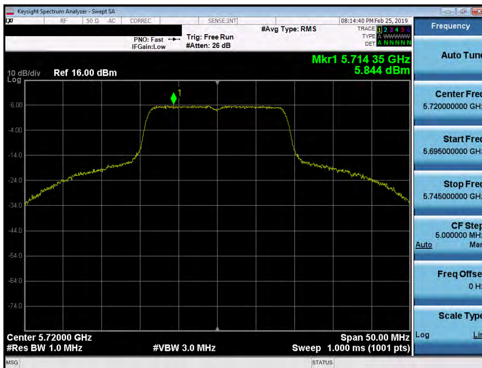
Plot 7-168. Power Spectral Density Plot SISO ANT1 (20MHz BW 802.11n (UNII Band 2C) – Ch. 144)
