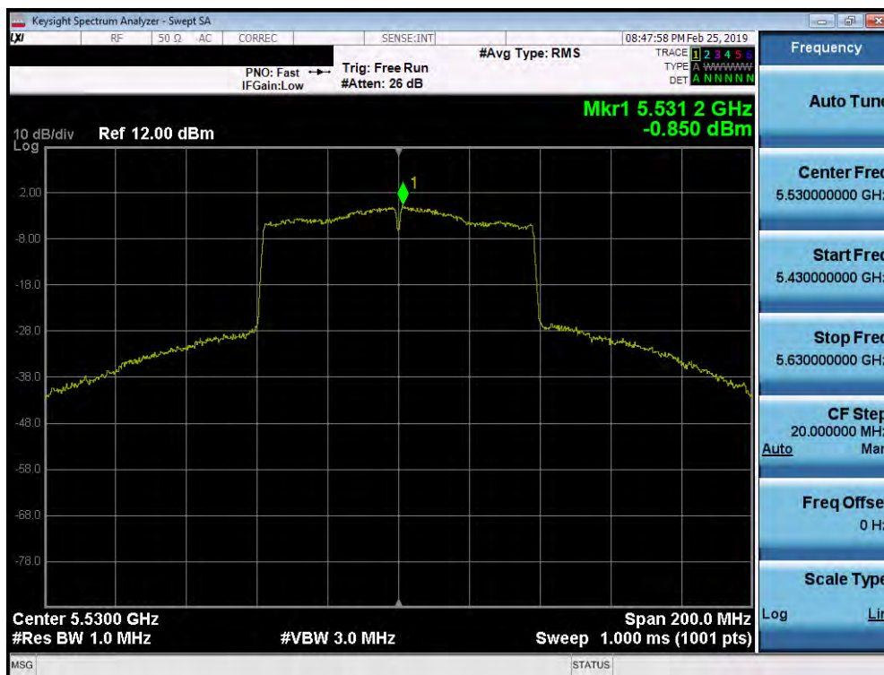
Plot 7-178. Power Spectral Density Plot SISO ANT1 (80MHz BW 802.11ac (UNII Band 2C) – Ch. 106)
