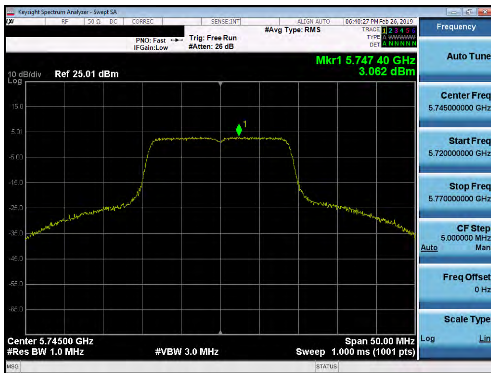
Plot 7-190. Power Spectral Density Plot SISO ANT1 (20MHz BW 802.11ax (UNII Band 3) – Ch. 149)
