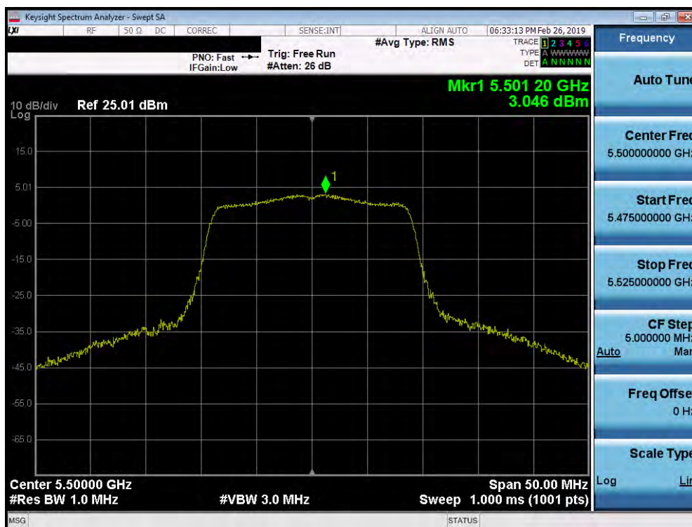
Plot 7-169. Power Spectral Density Plot SISO ANT1 (20MHz BW 802.11ax (UNII Band 2C) – Ch. 100)
