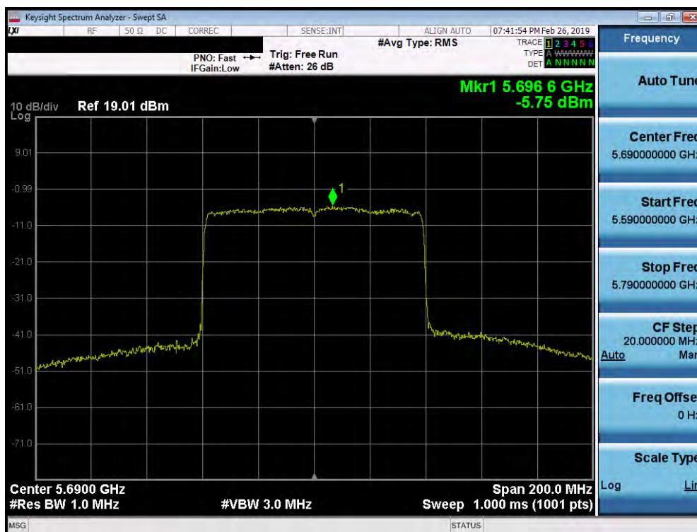
Plot 7-183. Power Spectral Density Plot SISO ANT1 (80MHz BW 802.11ax (UNII Band 2C) – Ch. 138)
