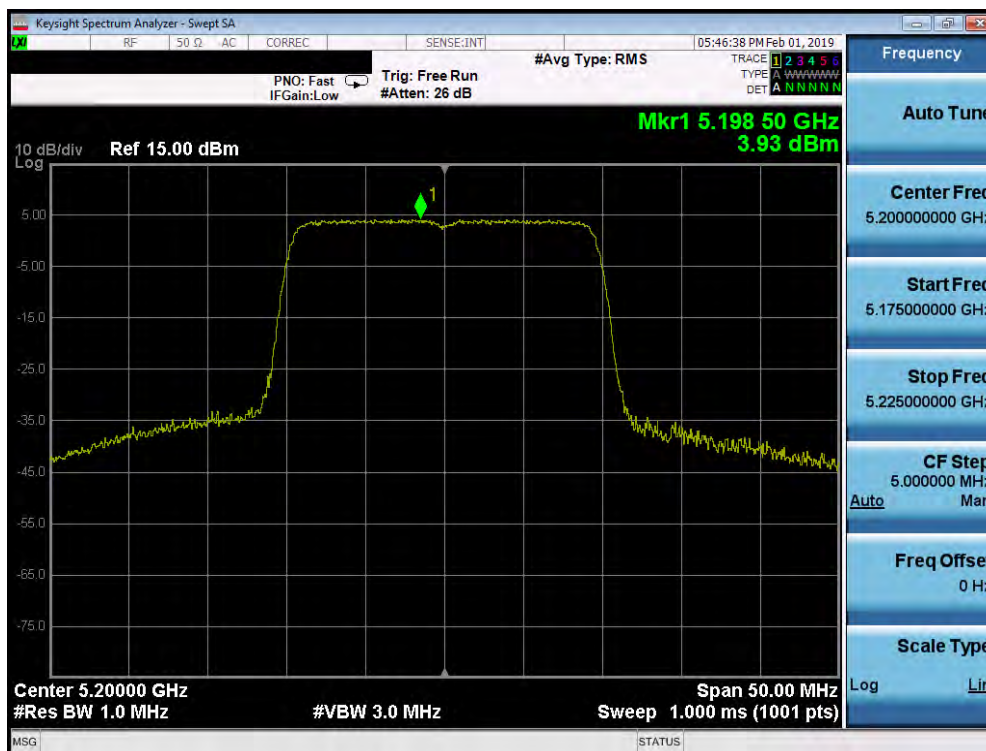
Plot 7-206. Power Spectral Density Plot SISO ANT2 (20MHz BW 802.11ax (UNII Band 1) – Ch. 40)
