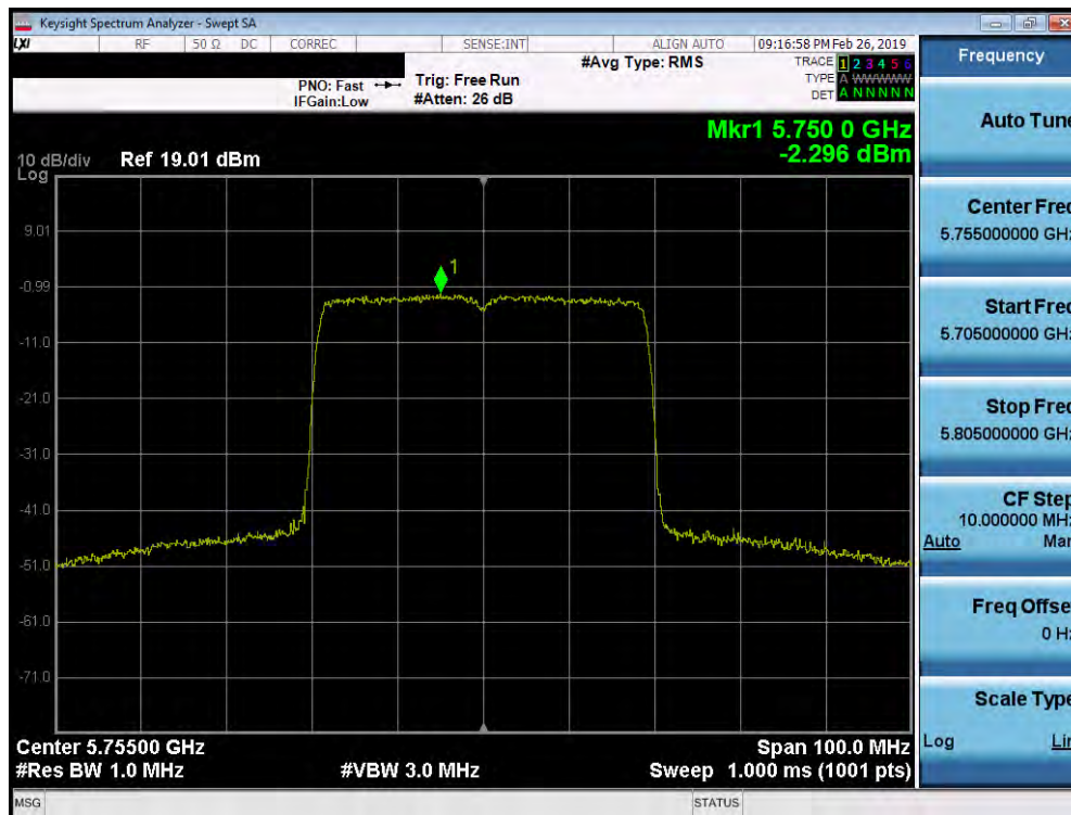
Plot 7-261. Power Spectral Density Plot SISO ANT2 (40MHz BW 802.11ax (UNII Band 3) – Ch. 151)
