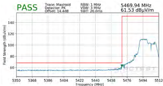
Plot 7-310. Radiated Lower Band Edge Plot SISO ANT1 (Peak - UNII Band 2C)
