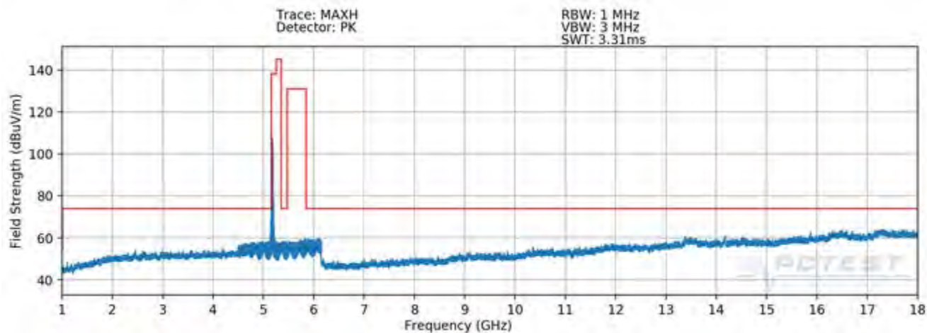
Plot 7-266. Radiated Spurious Plot above 1GHz SISO ANT1 (802.11a – U1 Ch. 40 - OPEN)
