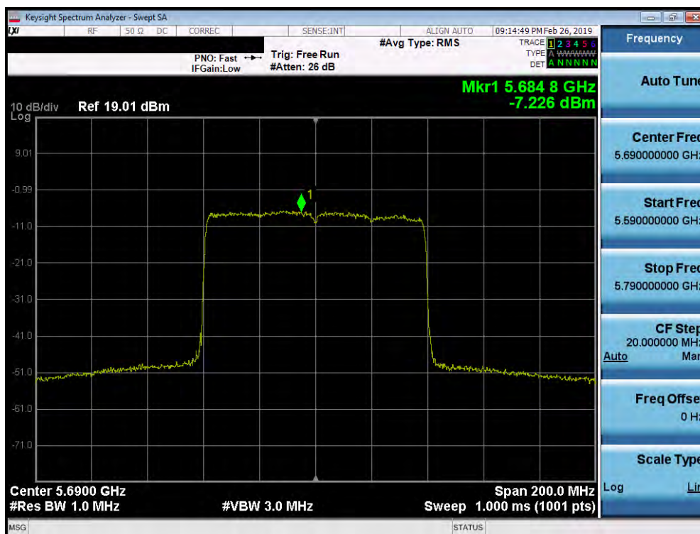
Plot 7-249. Power Spectral Density Plot SISO ANT2 (80MHz BW 802.11ax (UNII Band 2C) – Ch. 138)
