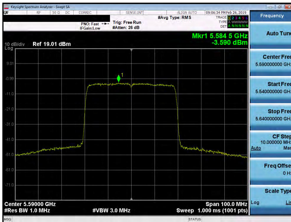
Plot 7-242. Power Spectral Density Plot SISO ANT2 (40MHz BW 802.11ax (UNII Band 2C) – Ch. 118)
