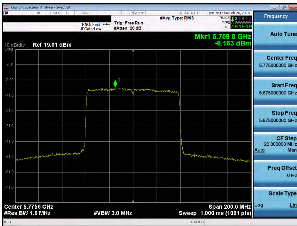
Plot 7-264. Power Spectral Density Plot SISO ANT2 (80MHz BW 802.11ax (UNII Band 3) – Ch. 155)
