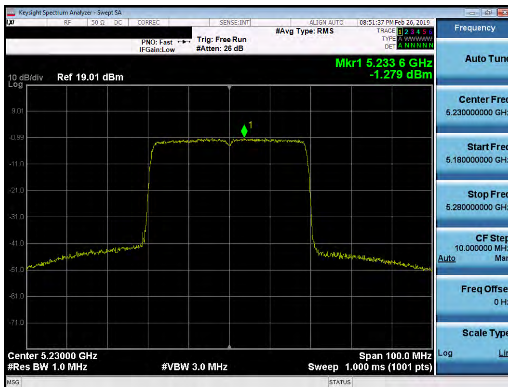
Plot 7-211. Power Spectral Density Plot SISO ANT2 (40MHz BW 802.11ax (UNII Band 1) – Ch. 46)
