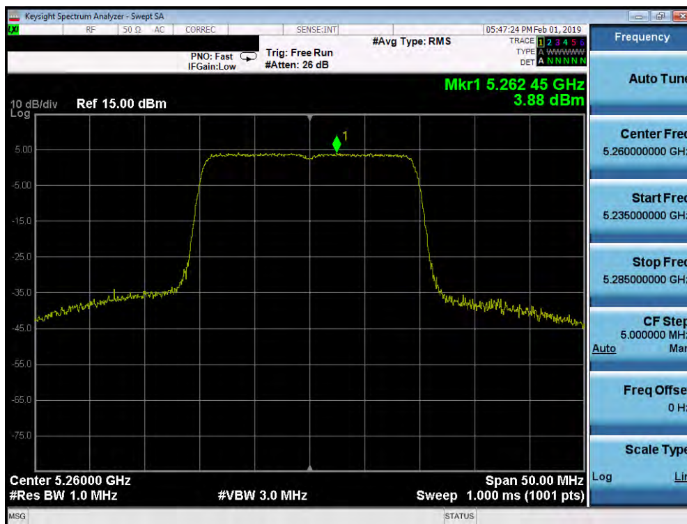
Plot 7-220. Power Spectral Density Plot SISO ANT2 (20MHz BW 802.11ax (UNII Band 2A) – Ch. 52)
