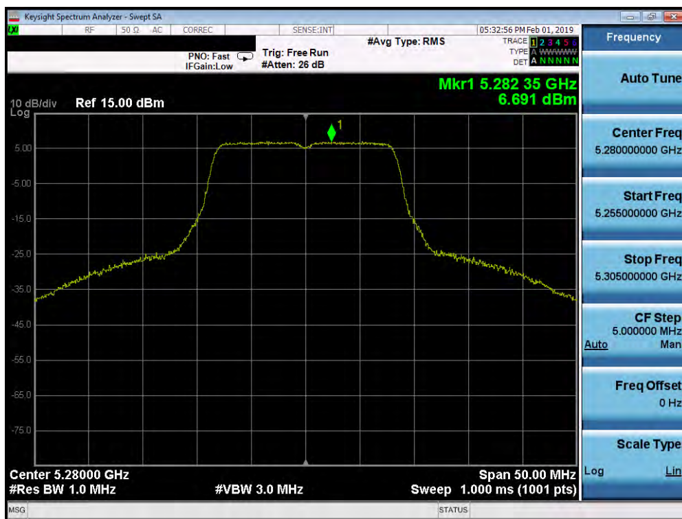
Plot 7-215. Power Spectral Density Plot SISO ANT2 (802.11a (UNII Band 2A) – Ch. 56)
