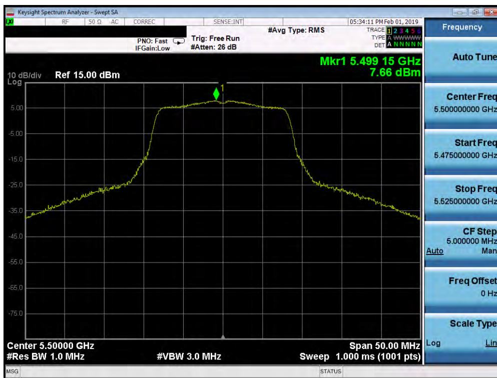
Plot 7-229. Power Spectral Density Plot SISO ANT2 (802.11a (UNII Band 2C) – Ch. 100)
