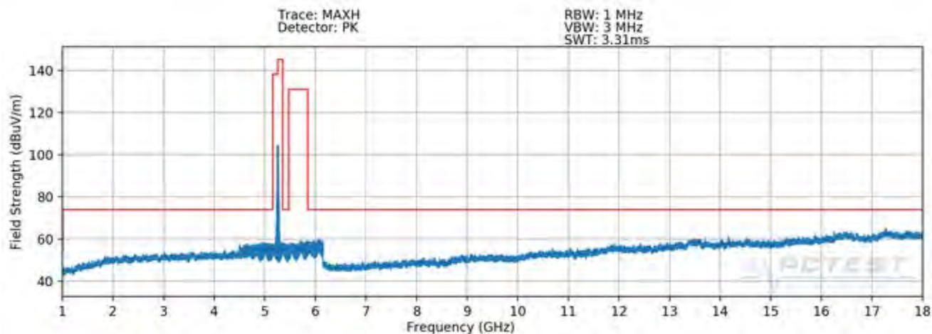
Plot 7-267. Radiated Spurious Plot above 1GHz SISO ANT1 (802.11a – U2A Ch. 56 - CLOSED)
