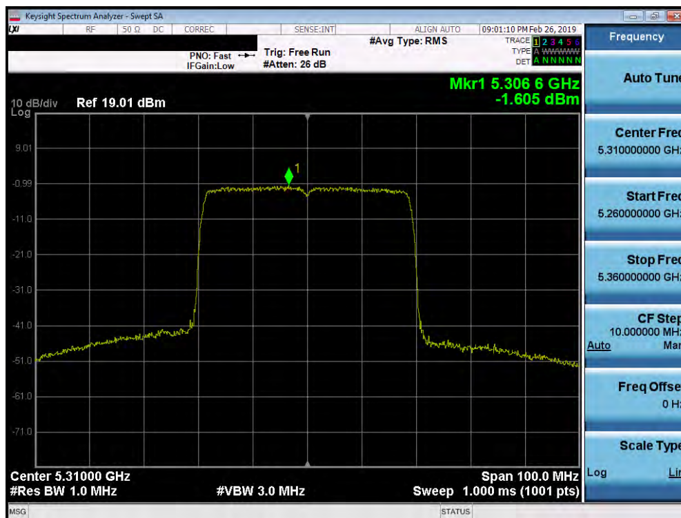
Plot 7-226. Power Spectral Density Plot SISO ANT2 (40MHz BW 802.11ax (UNII Band 2A) – Ch. 62)
