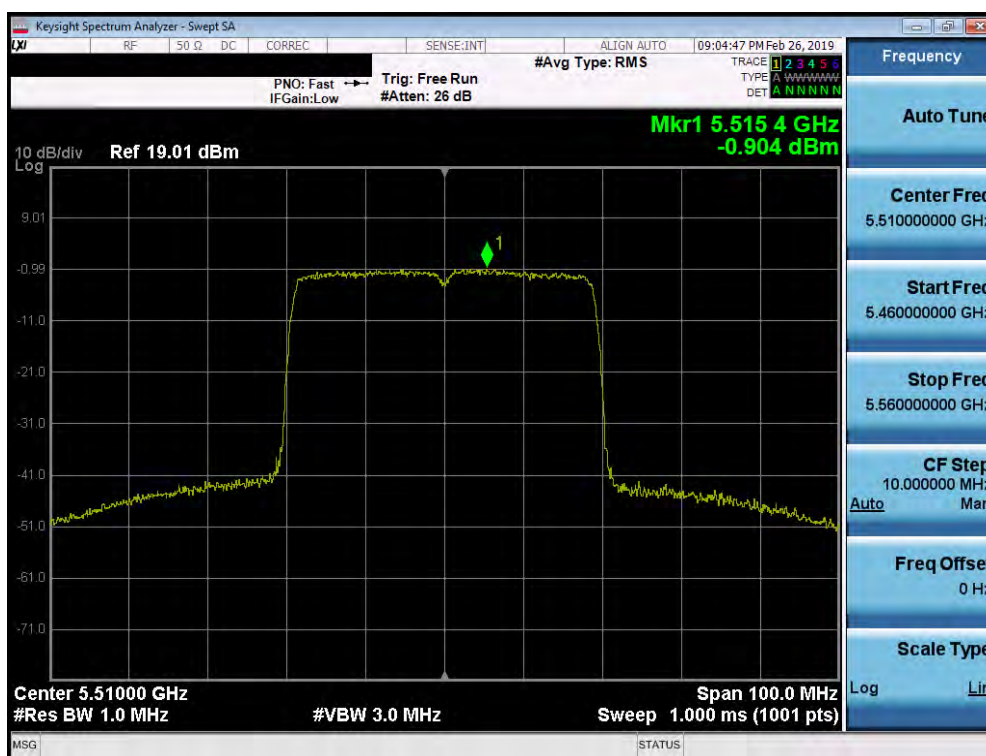
Plot 7-241. Power Spectral Density Plot SISO ANT2 (40MHz BW 802.11ax (UNII Band 2C) – Ch. 102)
