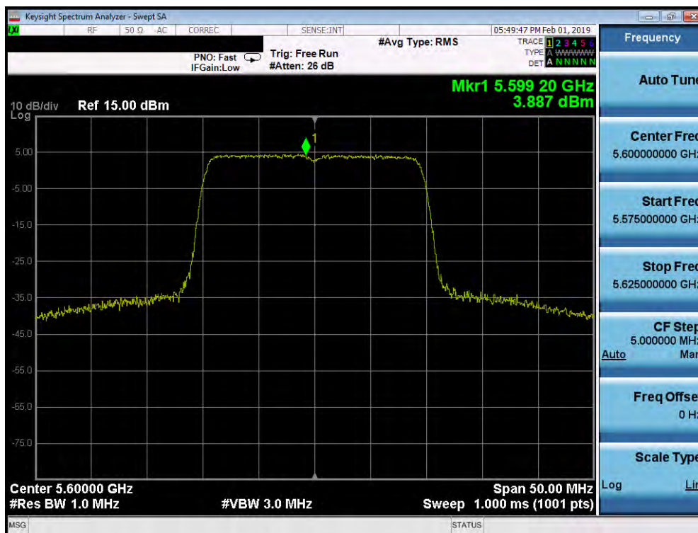
Plot 7-236. Power Spectral Density Plot SISO ANT2 (20MHz BW 802.11n (UNII Band 2C) – Ch. 120)
