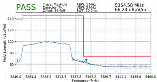
Plot 7-324. Radiated Upper Band Edge Plot SISO ANT1 (Peak - UNII Band 2A)
