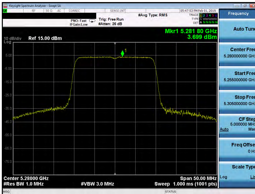
Plot 7-221. Power Spectral Density Plot SISO ANT2 (20MHz BW 802.11ax (UNII Band 2A) – Ch. 56)
