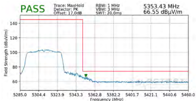
Plot 7-363. Radiated Upper Band Edge Plot MIMO (Peak – UNII Band 2A)
