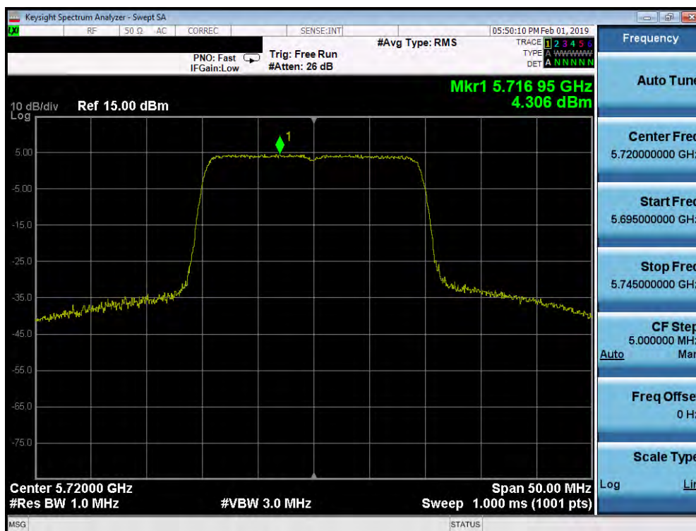
Plot 7-237. Power Spectral Density Plot SISO ANT2 (20MHz BW 802.11n (UNII Band 2C) – Ch. 144)
