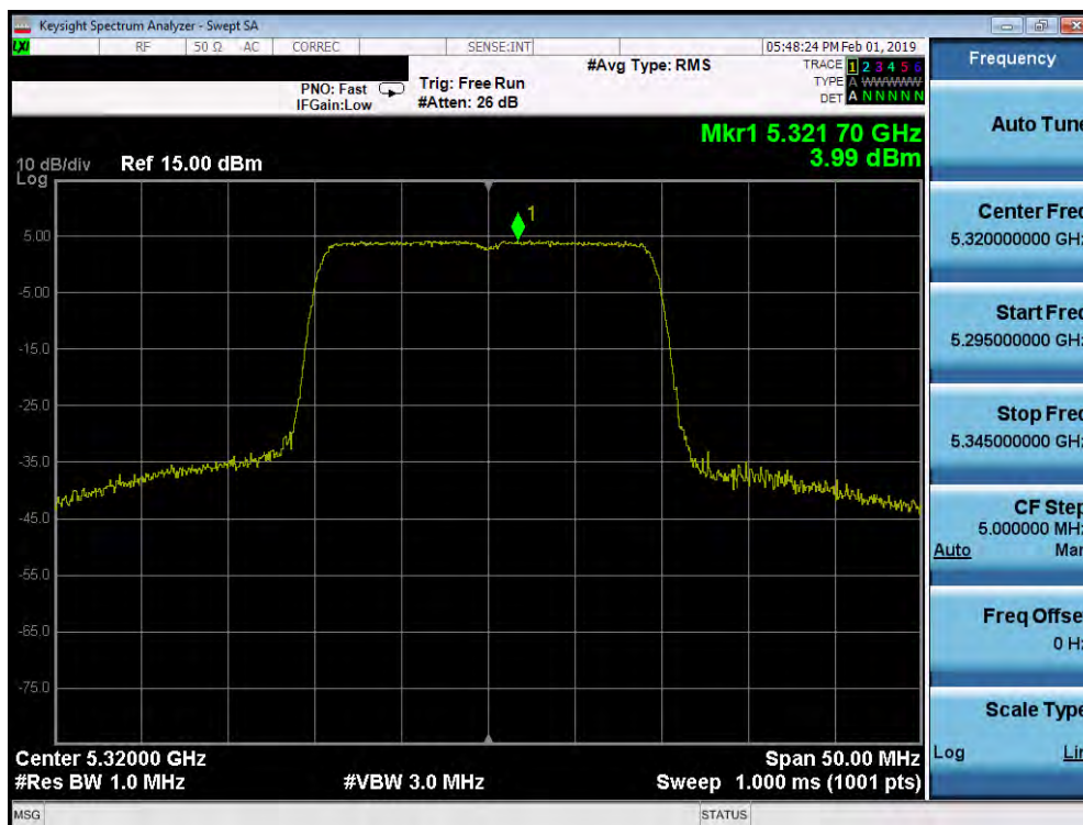
Plot 7-222. Power Spectral Density Plot SISO ANT2 (20MHz BW 802.11ax (UNII Band 2A) – Ch. 64)
