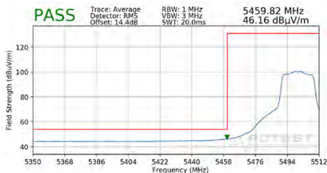
Plot 7-309. Radiated Lower Band Edge Plot SISO ANT1 (Average - UNII Band 2C)
