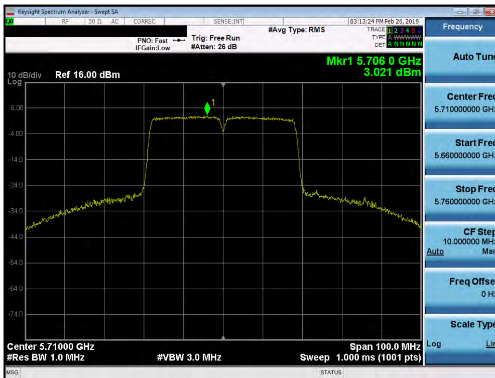
Plot 7-240. Power Spectral Density Plot SISO ANT2 (40MHz BW 802.11n (UNII Band 2C) – Ch. 142)
