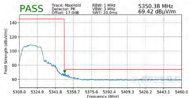
Plot 7-354. Radiated Upper Band Edge Plot MIMO (Peak – UNII Band 2A)
