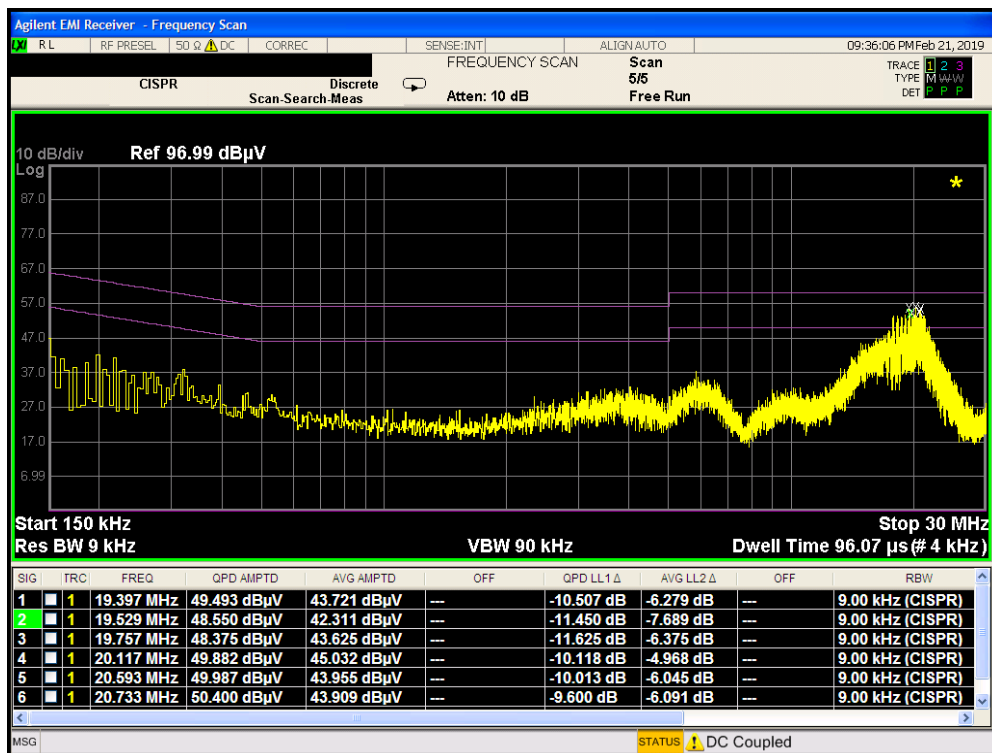
Plot 7-383. Line Conducted Plot with 802.11a UNII Band 3 (L1)
