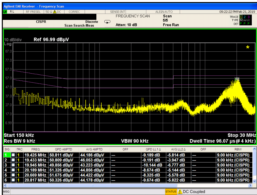
Plot 7-379. Line Conducted Plot with 802.11a UNII Band 2A (L1)
