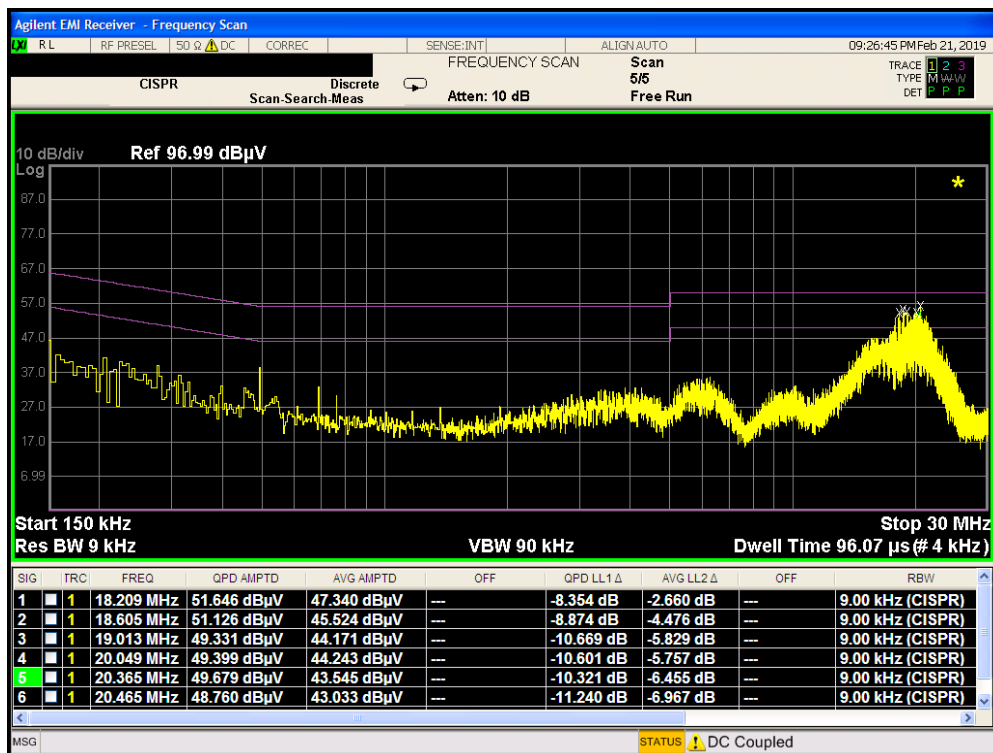
Plot 7-381. Line Conducted Plot with 802.11a UNII Band 2C (L1)
