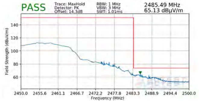
Plot 7-114. Radiated Restricted Upper Band Edge Measurement SISO ANT1 (Peak)
