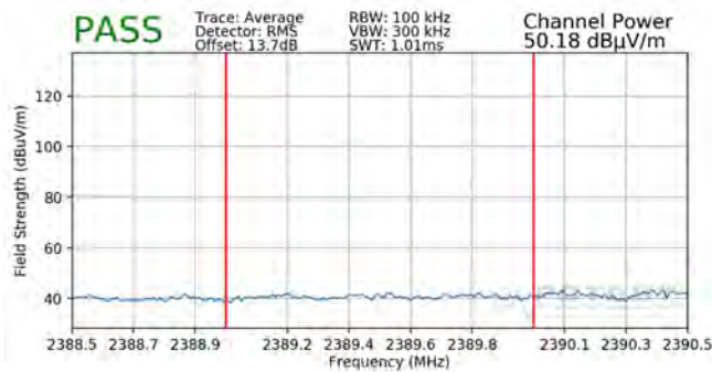
Plot 7-137. Radiated Restricted Band Edge Measurement SISO ANT2 with WCP (Average)
