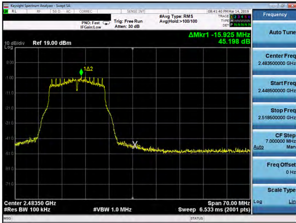
Plot 7-77. Band Edge Plot SISO ANT2 (802.11g – Ch. 12)
