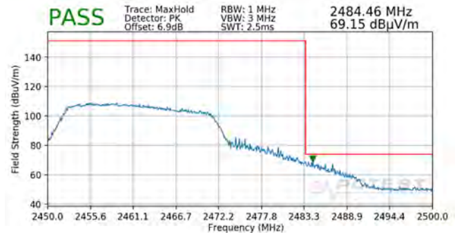
Plot 7-148. Radiated Restricted Upper Band Edge Measurement MIMO (Peak)
