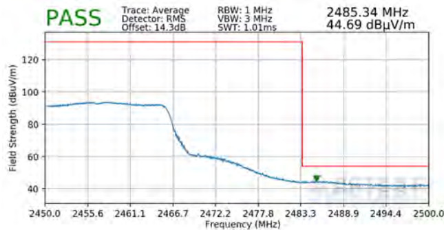
Plot 7-129. Radiated Restricted Upper Band Edge Measurement SISO ANT2 (Average)
