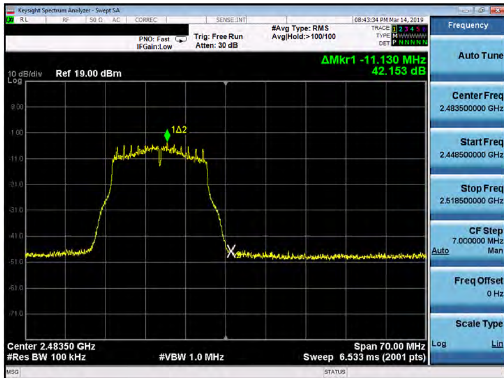
Plot 7-78. Band Edge Plot SISO ANT2 (802.11g – Ch. 13)
