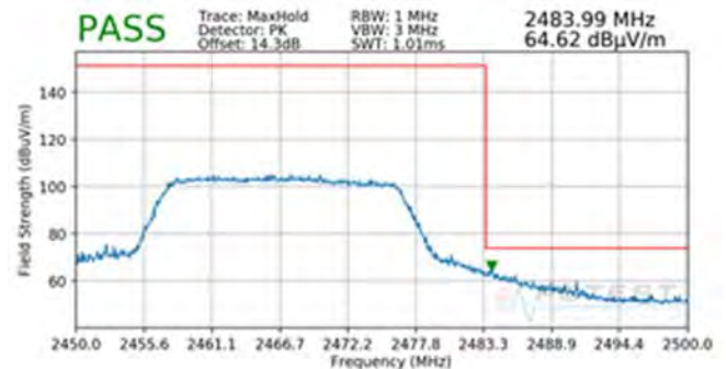
Plot 7-150. Radiated Restricted Upper Band Edge Measurement MIMO (Peak)
