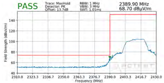
Plot 7-122. Radiated Restricted Band Edge Measurement SISO ANT1 with WCP (Peak)
