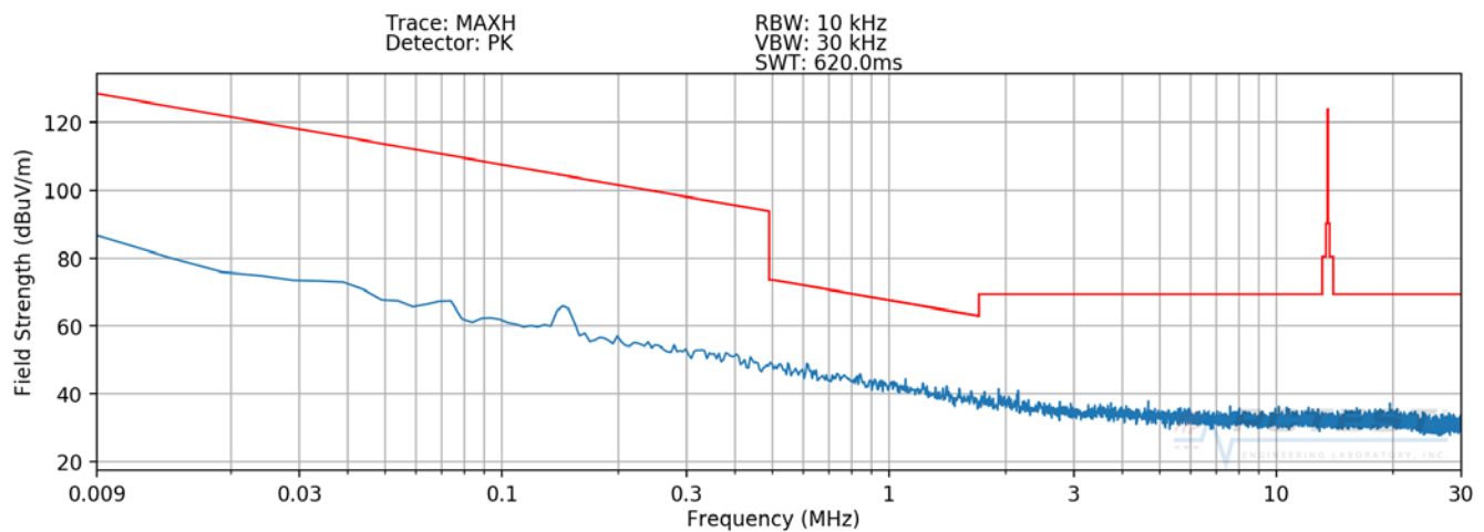
Plot 7-5. Radiated Spurious Plot 9kHz – 30MHz (Pol. Y – WPT with Earbuds)
