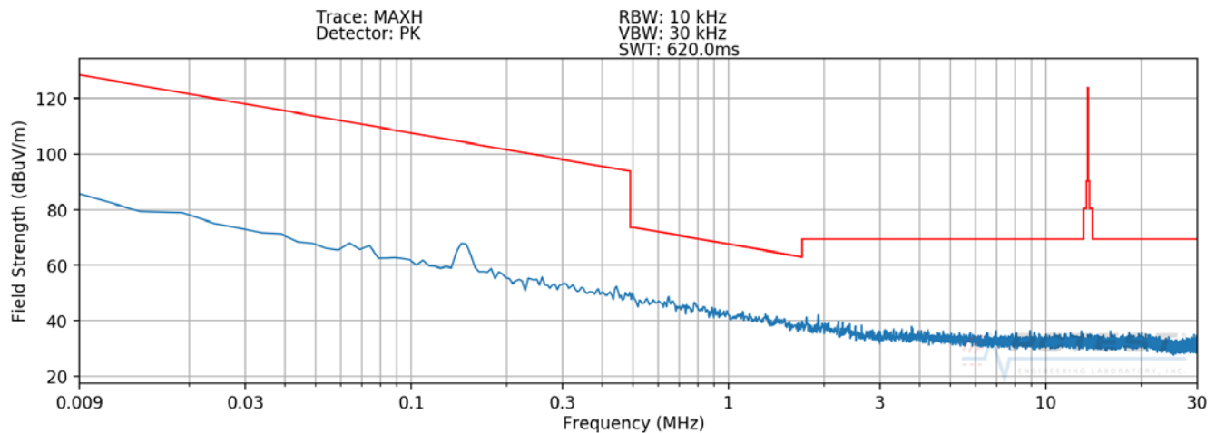
Plot 7-4. Radiated Spurious Plot 9kHz – 30MHz (Pol. X – WPT with Earbuds)
