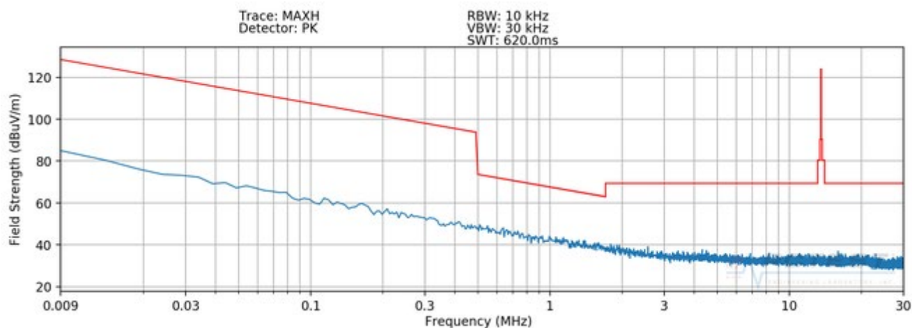
Plot 7-2 Radiated Spurious Plot 9kHz – 30MHz (Pol. Y - WPT)
