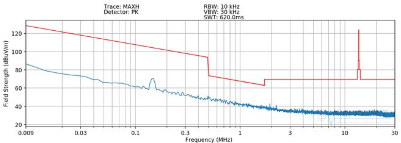
Plot 7-6. Radiated Spurious Plot 9kHz – 30MHz (Pol. Z – WPT with Earbuds)
