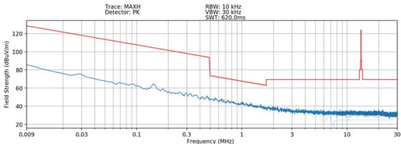
Plot 7-3. Radiated Spurious Plot 9kHz – 30MHz (Pol. Z - WPT)
