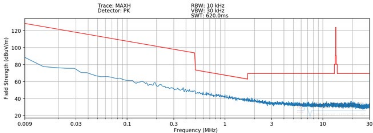
Plot 7-1. Radiated Spurious Plot 9kHz – 30MHz (Pol. X - WPT)
