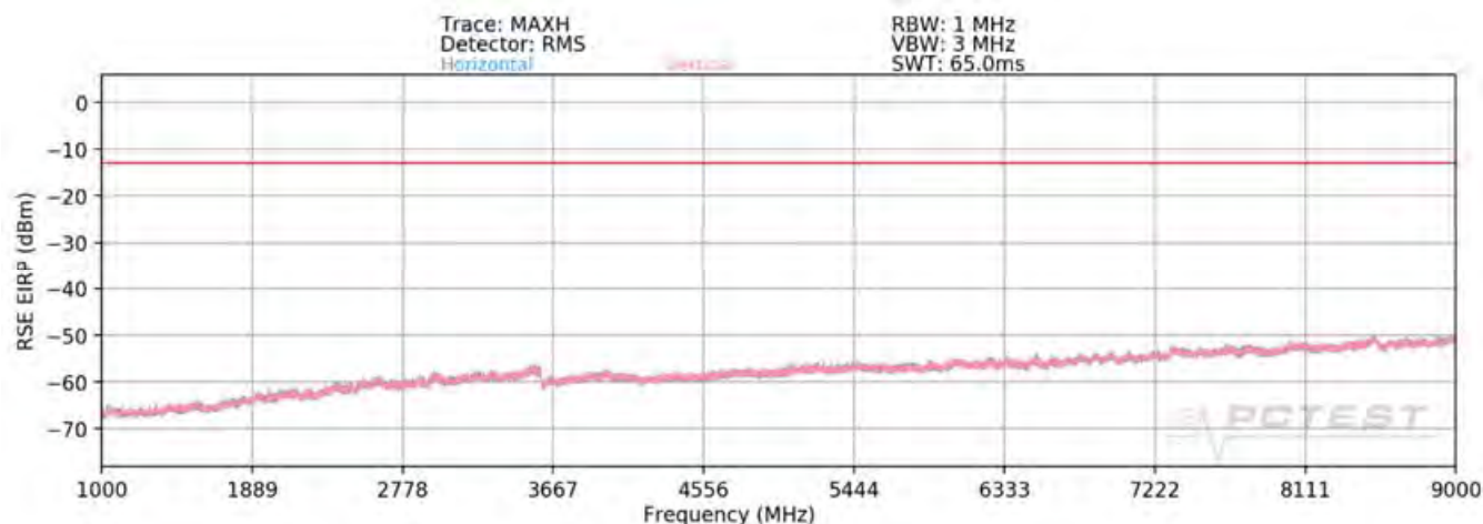
Plot 7-136. Radiated Spurious Plot above 1GHz (Band 5)
