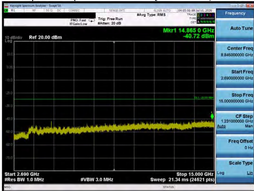
Plot 7-79. Conducted Spurious Plot (Band 41 PC3 - 20.0MHz QPSK - RB Size 1, RB Offset 0 - Low Channel)
