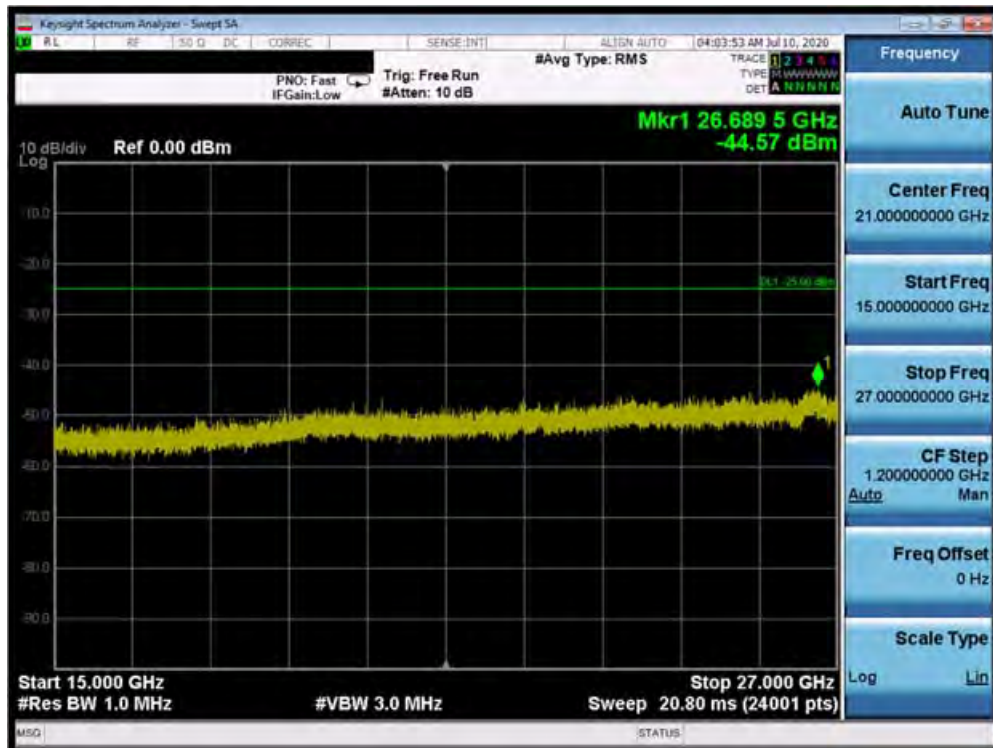
Plot 7-83. Conducted Spurious Plot (Band 41 PC3 - 20.0MHz QPSK - RB Size 1, RB Offset 0 - Mid Channel)
