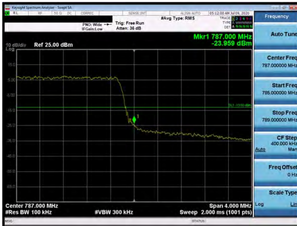
Plot 7-97. Upper Band Edge Plot (Band 13 - 5.0MHz QPSK - Full RB Configuration)
