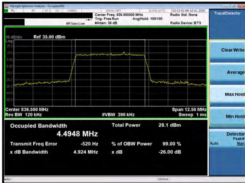
Plot 7-32. Occupied Bandwidth Plot (Band 5 - 5.0MHz 256-QAM - Full RB Configuration)
