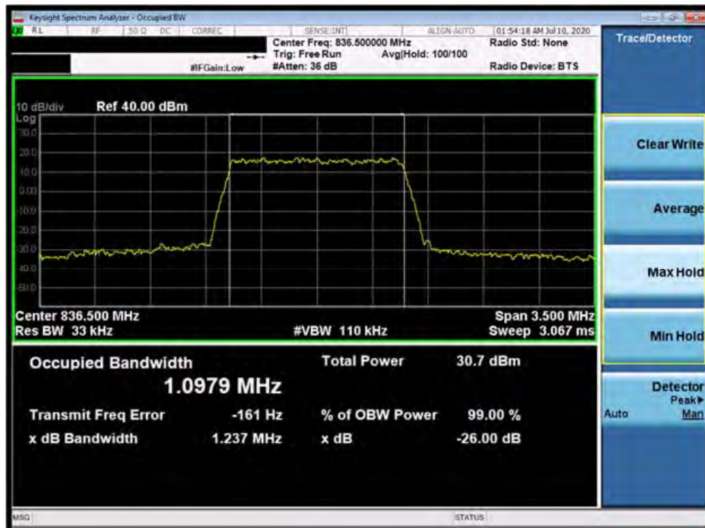
Plot 7-38. Occupied Bandwidth Plot (Band 5 - 1.4MHz 16-QAM - Full RB Configuration)
