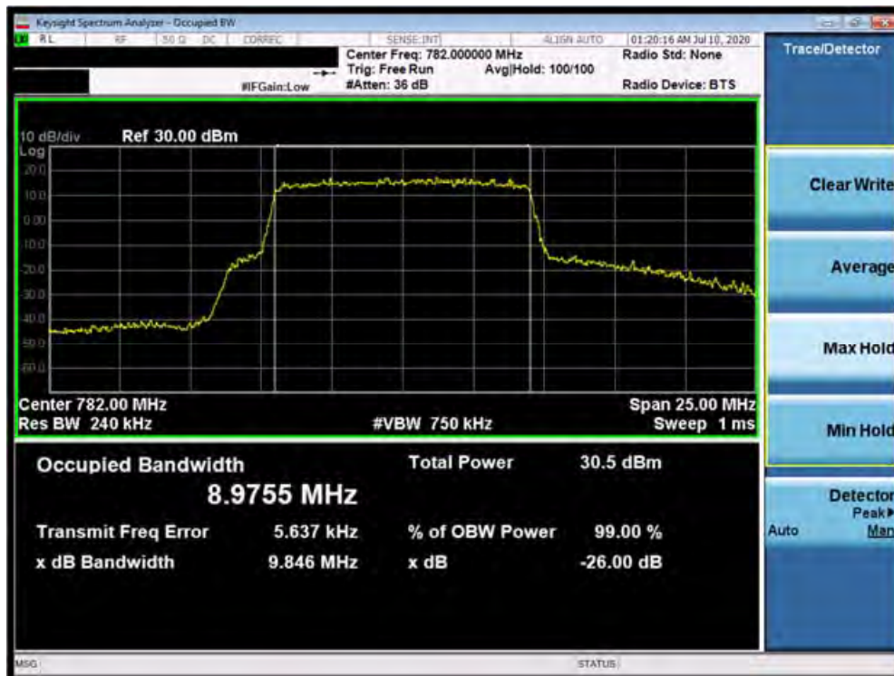
Plot 7-18. Occupied Bandwidth Plot (Band 13 - 10.0MHz 16-QAM - Full RB Configuration)
