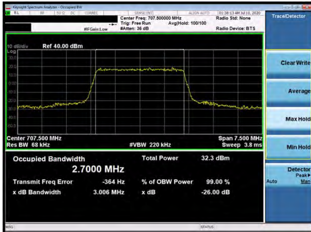
Plot 7-9. Occupied Bandwidth Plot (Band 12 - 3.0MHz QPSK - Full RB Configuration)
