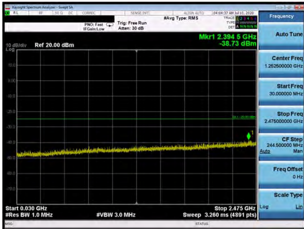
Plot 7-78. Conducted Spurious Plot (Band 41 PC3 - 20.0MHz QPSK - RB Size 1, RB Offset 0 - Low Channel)
