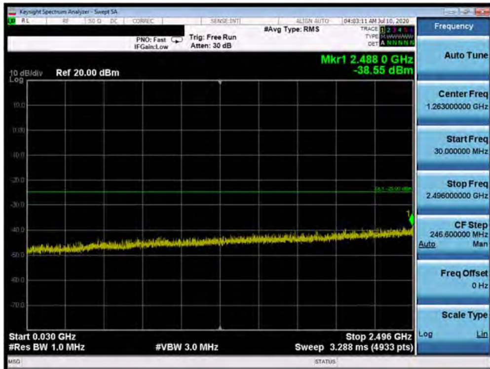
Plot 7-81. Conducted Spurious Plot (Band 41 PC3 - 20.0MHz QPSK - RB Size 1, RB Offset 0 - Mid Channel)
