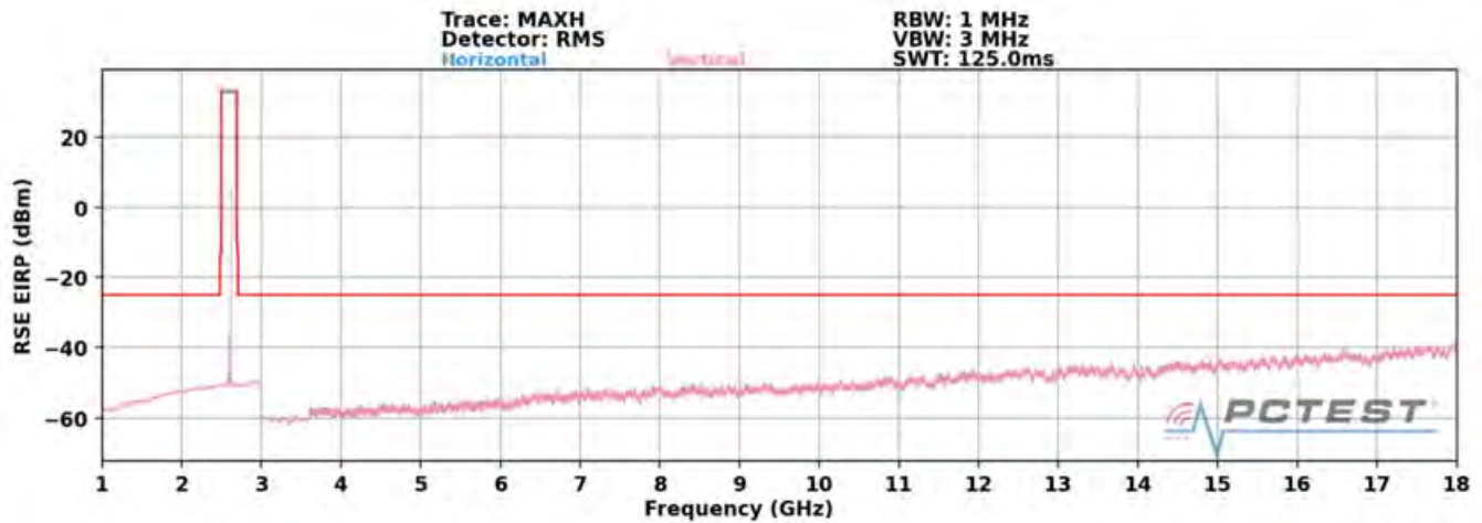
Plot 7-134. Radiated Spurious Plot above 1GHz (Band 41)
