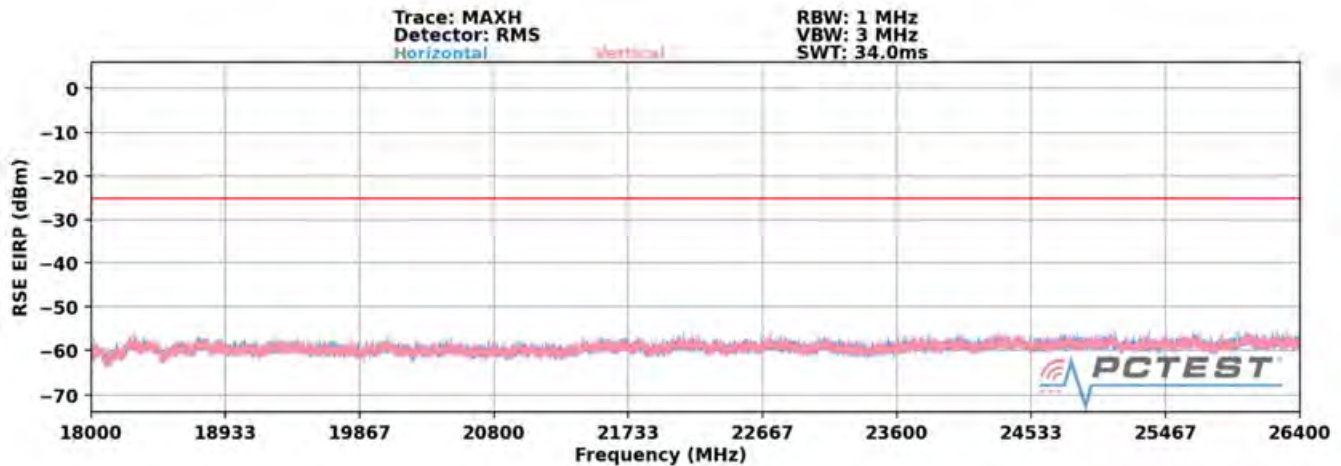
Plot 7-135. Radiated Spurious Plot 18GHz – 26.5GHz (Band 41)
