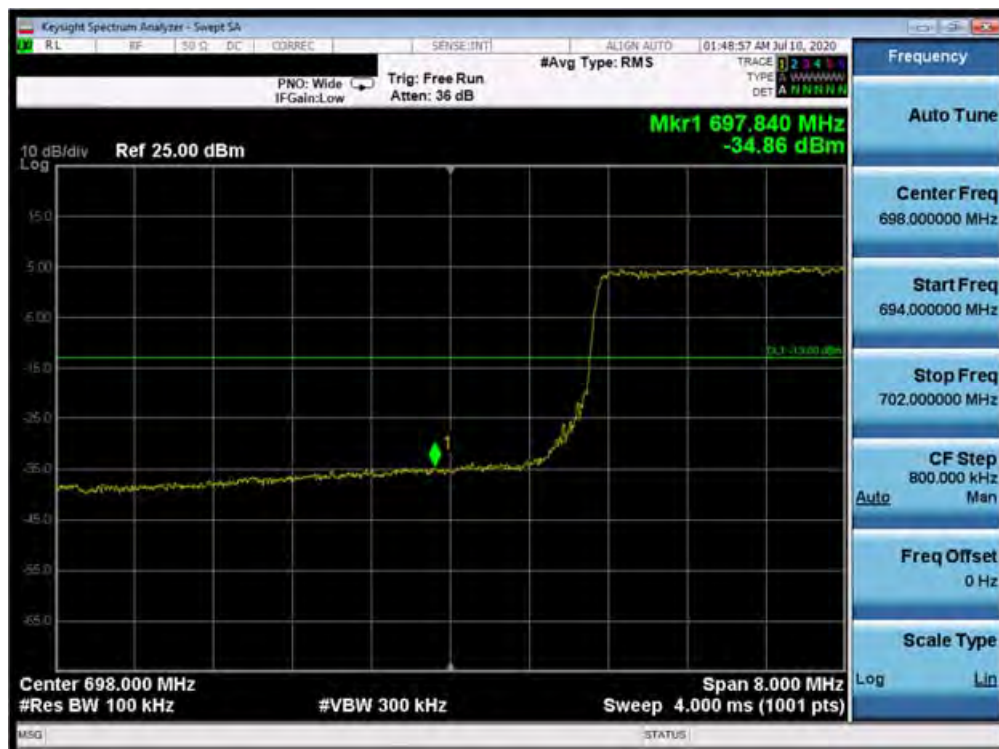
Plot 7-93. Lower Band Edge Plot (Band 12 - 10.0MHz QPSK - Full RB Configuration)
