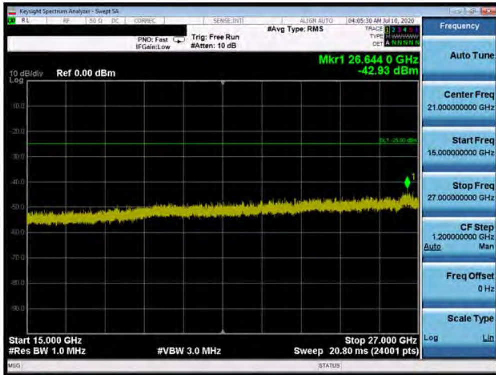
Plot 7-80. Conducted Spurious Plot (Band 41 PC3 - 20.0MHz QPSK - RB Size 1, RB Offset 0 - Low Channel)
