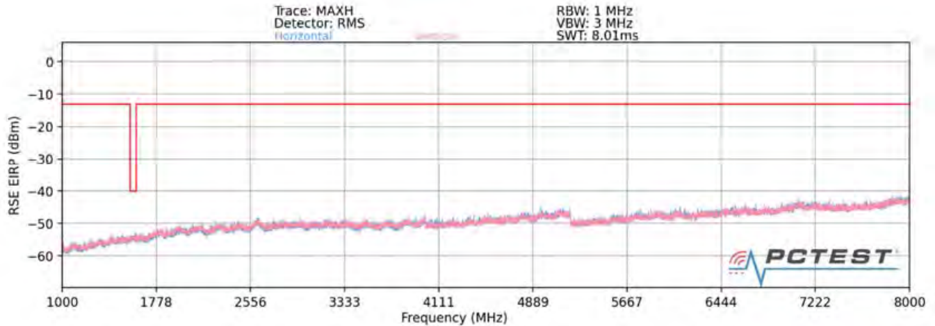
Plot 7-132. Radiated Spurious Plot above 1GHz (Band 13)
