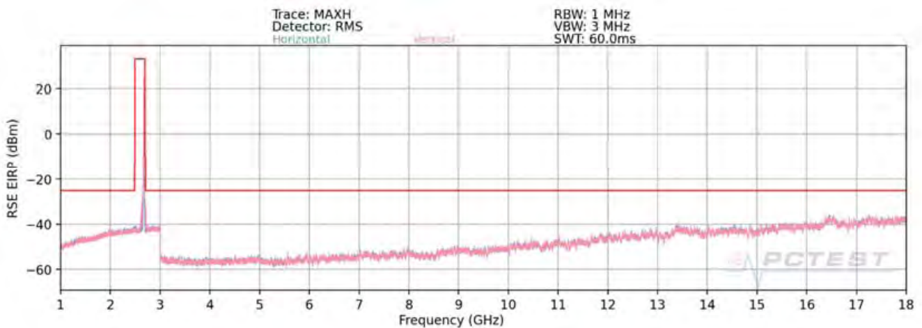
Plot 7-139. Radiated Spurious Plot 1GHz - 18GHz (ULCA Band 41 High Channel – PCC/SCC: 1RB)
