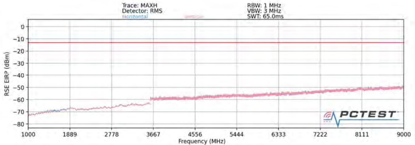
Plot 7-133. Radiated Spurious Plot above 1GHz (Band 5)
