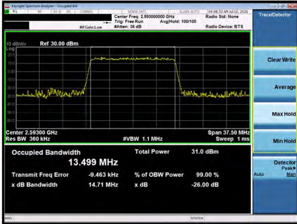
Plot 7-45. Occupied Bandwidth Plot (Band 41 (PC3) - 15.0MHz QPSK - Full RB Configuration)
