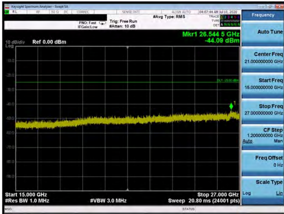
Plot 7-86. Conducted Spurious Plot (Band 41 PC3 - 20.0MHz QPSK - RB Size 1, RB Offset 99 - High Channel)
