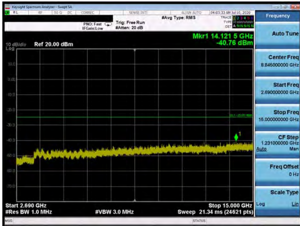
Plot 7-82. Conducted Spurious Plot (Band 41 PC3 - 20.0MHz QPSK - RB Size 1, RB Offset 0 - Mid Channel)
