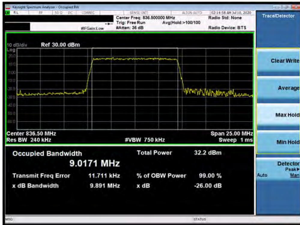
Plot 7-25. Occupied Bandwidth Plot (Band 5 - 10.0MHz QPSK - Full RB Configuration)
