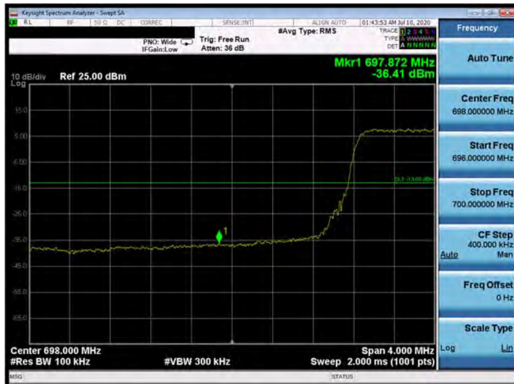
Plot 7-91. Lower Band Edge Plot (Band 12 - 5.0MHz QPSK - Full RB Configuration)
