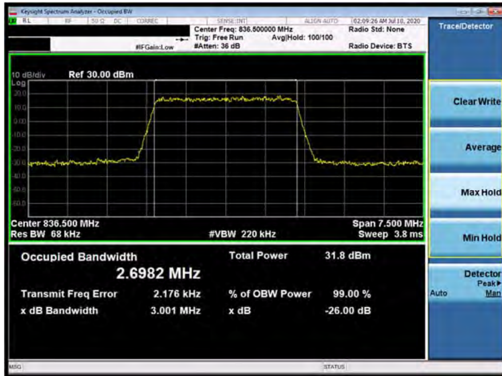
Plot 7-33. Occupied Bandwidth Plot (Band 5 - 3.0MHz QPSK - Full RB Configuration)
