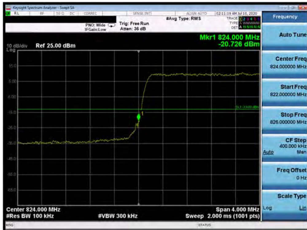
Plot 7-105. Lower Band Edge Plot (Band 5 - 3.0MHz QPSK - Full RB Configuration)
