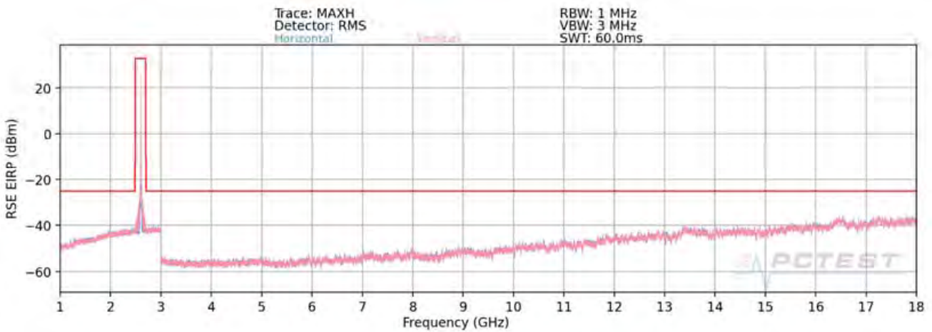
Plot 7-138. Radiated Spurious Plot 1GHz - 18GHz (ULCA Band 41 Mid Channel – PCC/SCC: 1RB)
