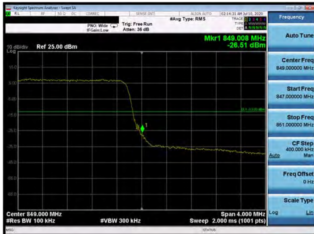
Plot 7-108. Upper Band Edge Plot (Band 5 - 5.0MHz QPSK - Full RB Configuration)
