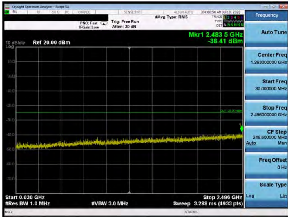
Plot 7-84. Conducted Spurious Plot (Band 41 PC3 - 20.0MHz QPSK - RB Size 1, RB Offset 99 - High Channel)
