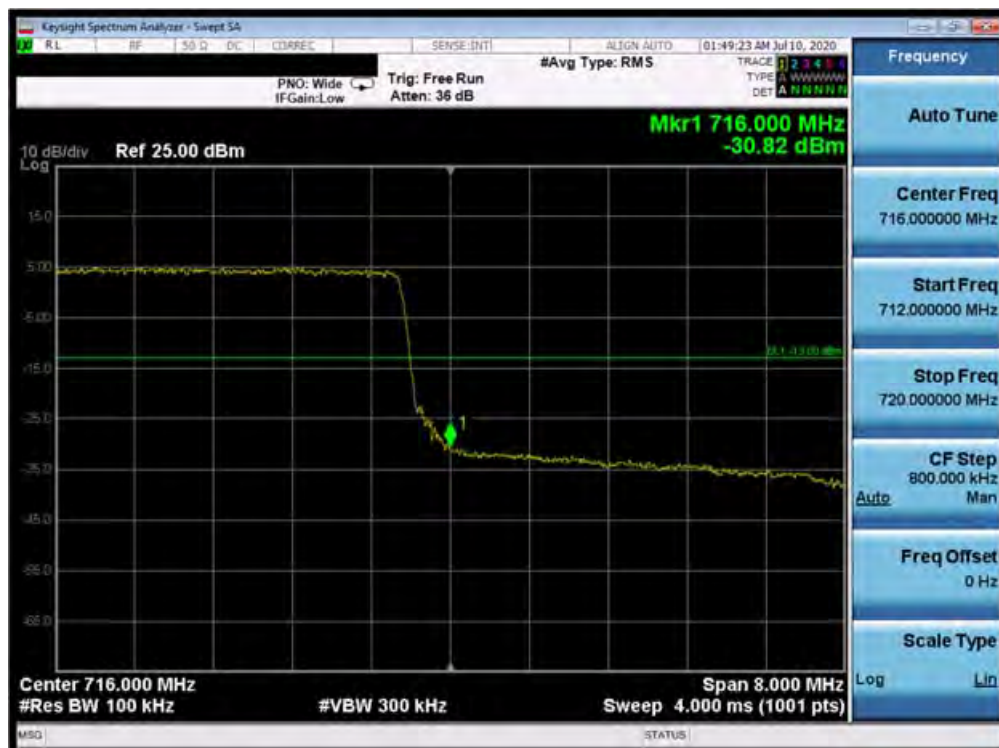
Plot 7-94. Upper Band Edge Plot (Band 12 - 10.0MHz QPSK - Full RB Configuration)
