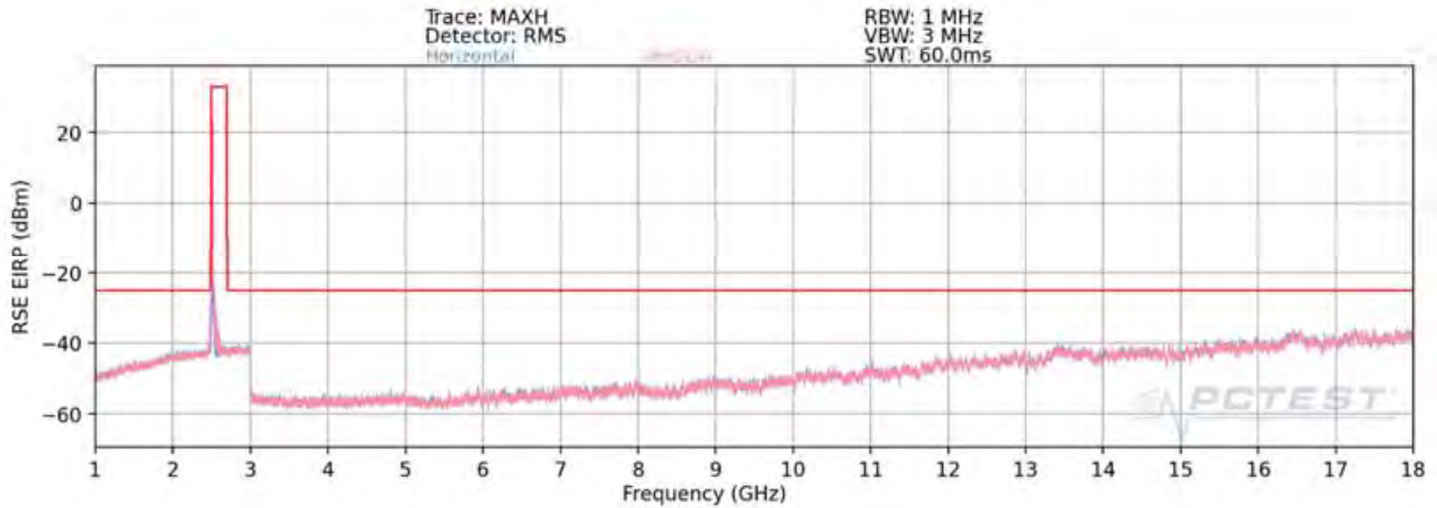
Plot 7-137. Radiated Spurious Plot 1GHz - 18GHz (ULCA Band 41 Low Channel – PCC/SCC: 1RB)
