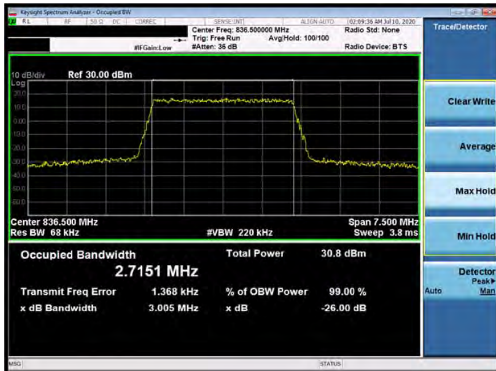
Plot 7-34. Occupied Bandwidth Plot (Band 5 - 3.0MHz 16-QAM - Full RB Configuration)
