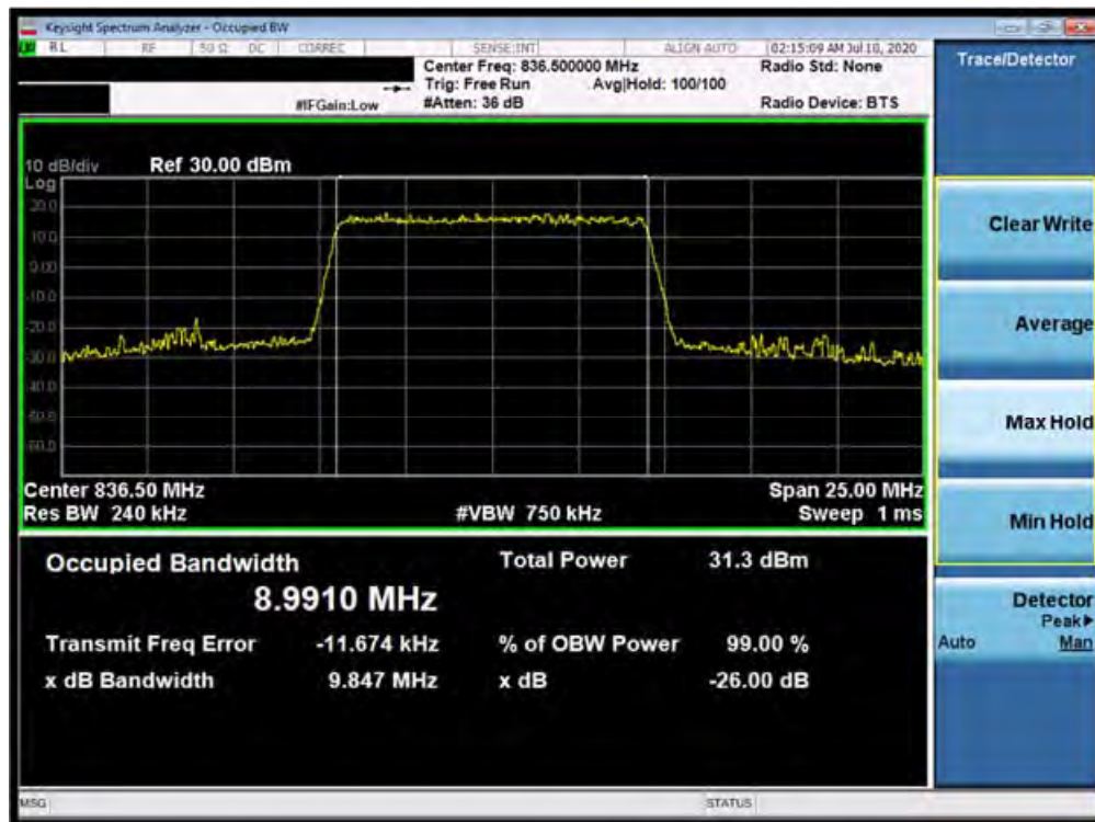
Plot 7-26. Occupied Bandwidth Plot (Band 5 - 10.0MHz 16-QAM - Full RB Configuration)
