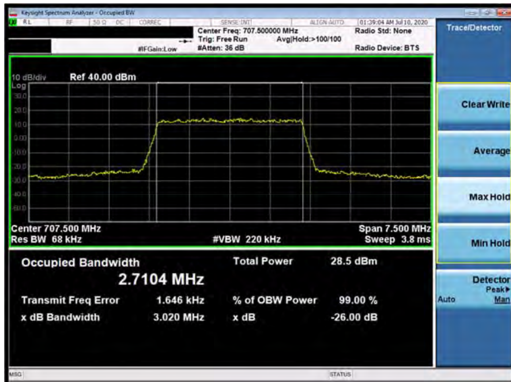
Plot 7-12. Occupied Bandwidth Plot (Band 12 - 3.0MHz 256-QAM - Full RB Configuration)
