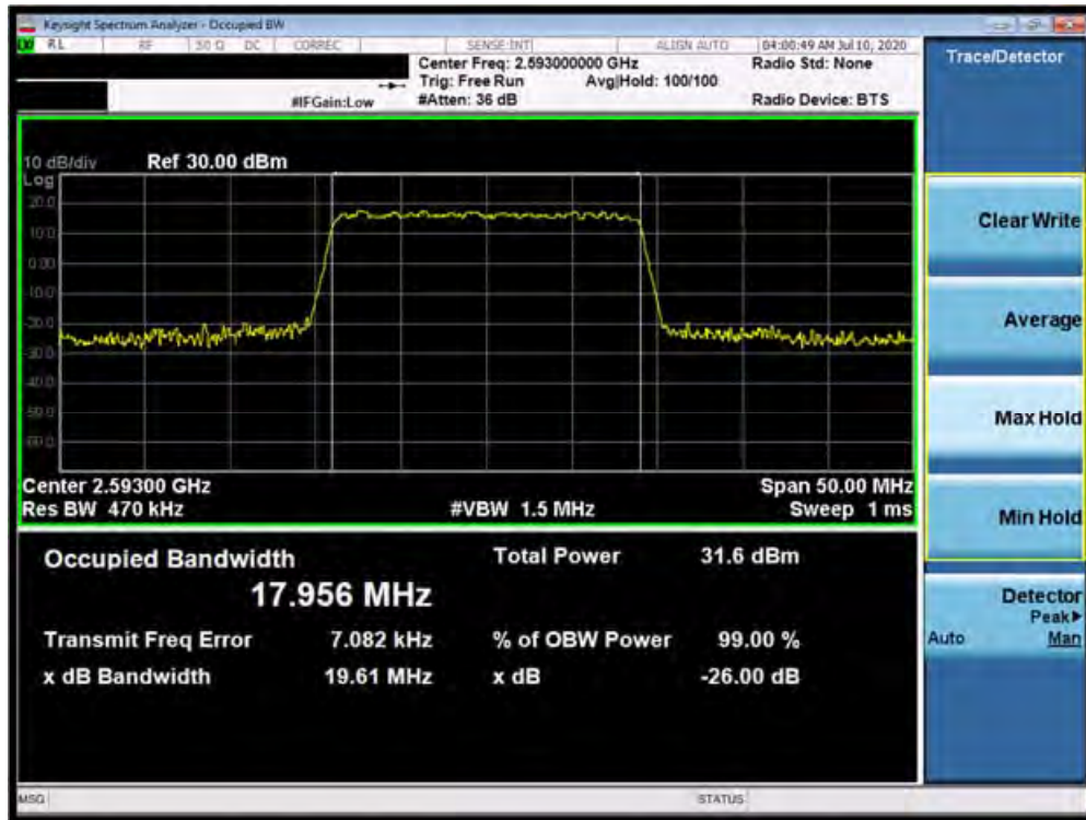
Plot 7-41. Occupied Bandwidth Plot (Band 41 (PC3) - 20.0MHz QPSK - Full RB Configuration)
