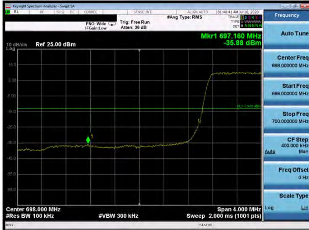
Plot 7-89. Lower Band Edge Plot (Band 12 - 3.0MHz QPSK - Full RB Configuration)
