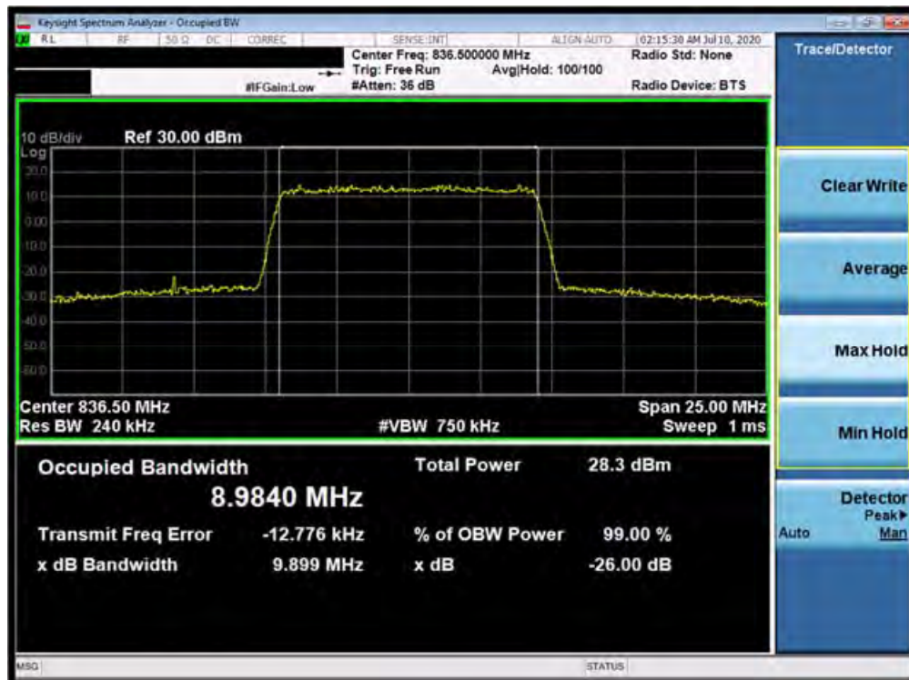
Plot 7-28. Occupied Bandwidth Plot (Band 5 - 10.0MHz 256-QAM - Full RB Configuration)
