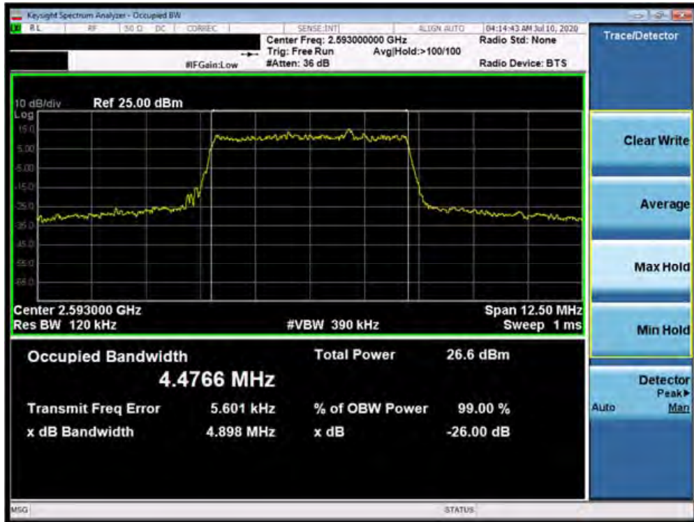
Plot 7-56. Occupied Bandwidth Plot (Band 41 (PC3) - 5.0MHz 256-QAM - Full RB Configuration)
