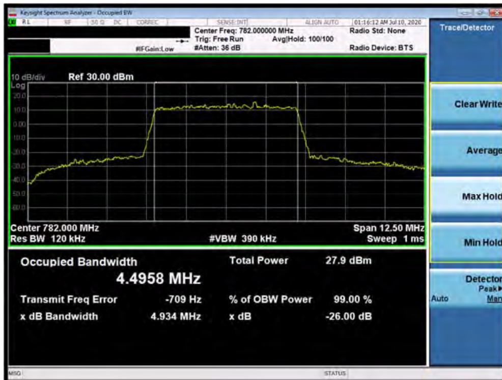
Plot 7-24. Occupied Bandwidth Plot (Band 13 - 5.0MHz 256-QAM - Full RB Configuration)
