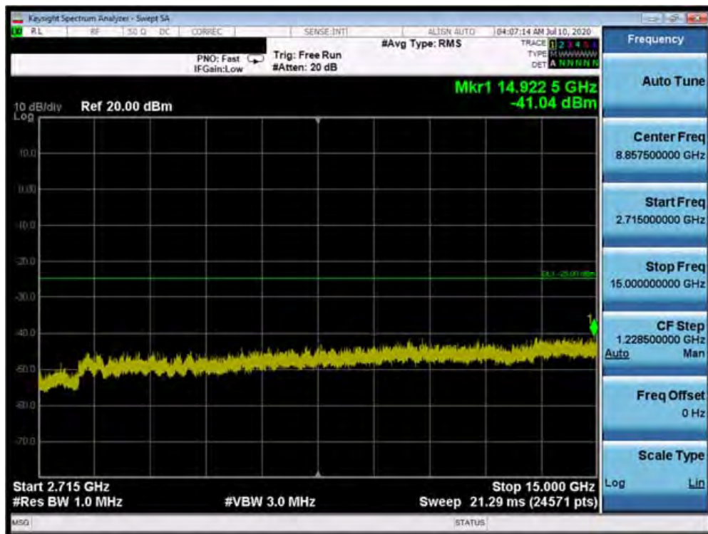
Plot 7-85. Conducted Spurious Plot (Band 41 PC3 - 20.0MHz QPSK - RB Size 1, RB Offset 99 – High Channel)
