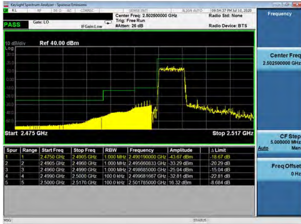
Plot 7-109. Lower ACP Plot at 2500 MHz (Band 41 PC3- 5.0MHz QPSK - Full RB Configuration)
