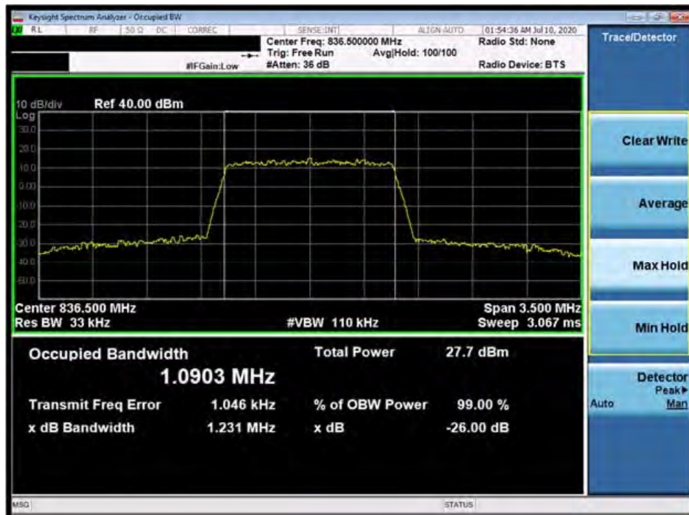
Plot 7-40. Occupied Bandwidth Plot (Band 5 - 1.4MHz 256-QAM - Full RB Configuration)
