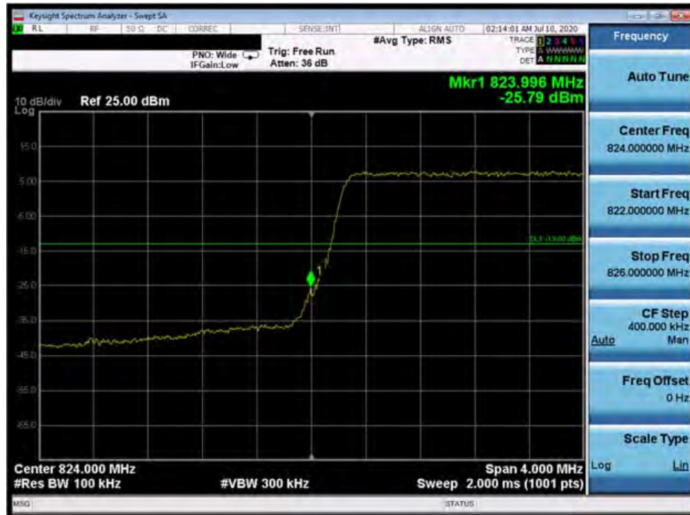
Plot 7-107. Lower Band Edge Plot (Band 5 - 5.0MHz QPSK - Full RB Configuration)
