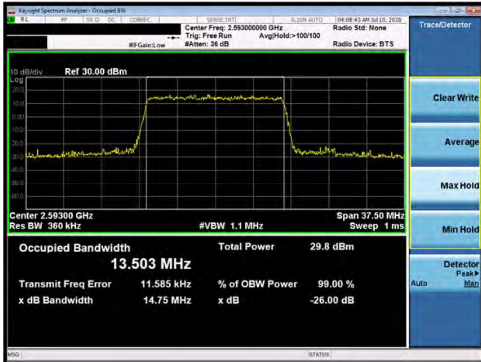
Plot 7-46. Occupied Bandwidth Plot (Band 41 (PC3) - 15.0MHz 16-QAM - Full RB Configuration)
