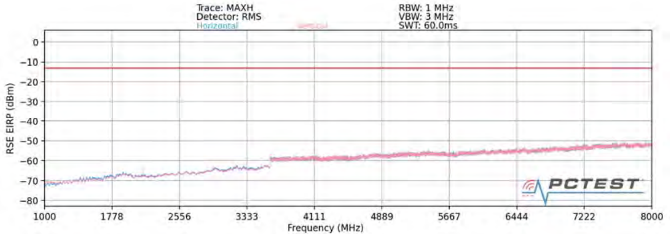
Plot 7-131. Radiated Spurious Plot above 1GHz (Band 12)
