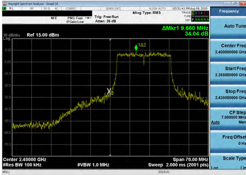
Plot 7-37. Band Edge Plot SISO ANT2 (802.11ax OFDMA - 242 Tones - Ch. 1)
