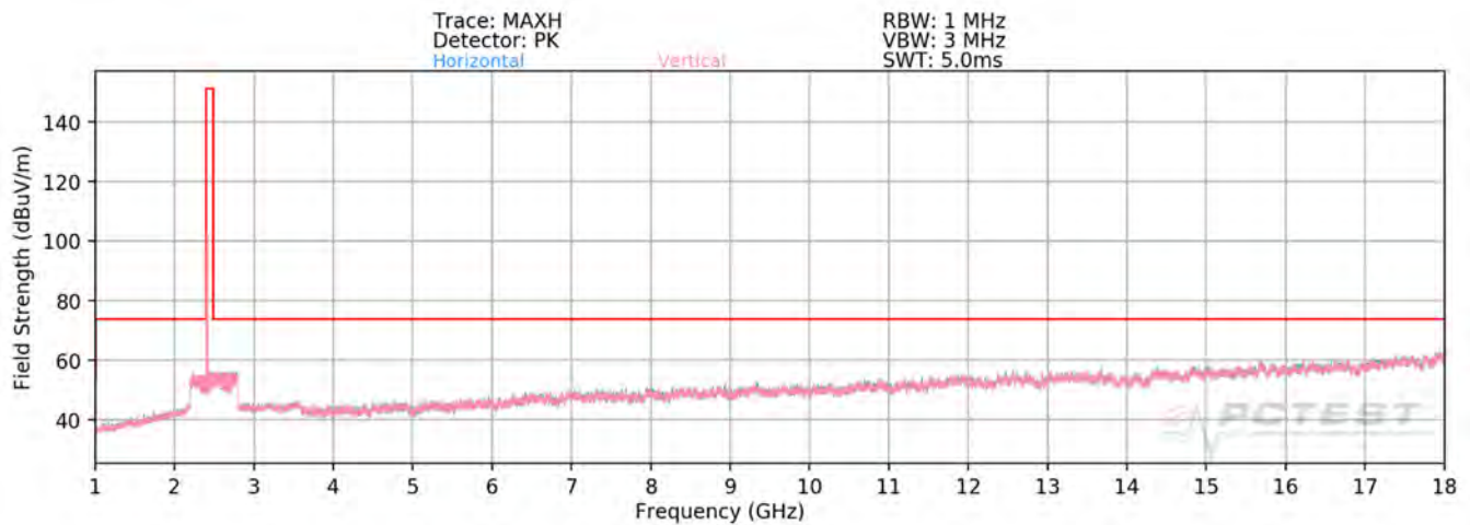
Plot 7-84. Radiated Spurious Plot above 1GHz MIMO (802.11ax OFDMA – 242 Tones – Ch. 1)
