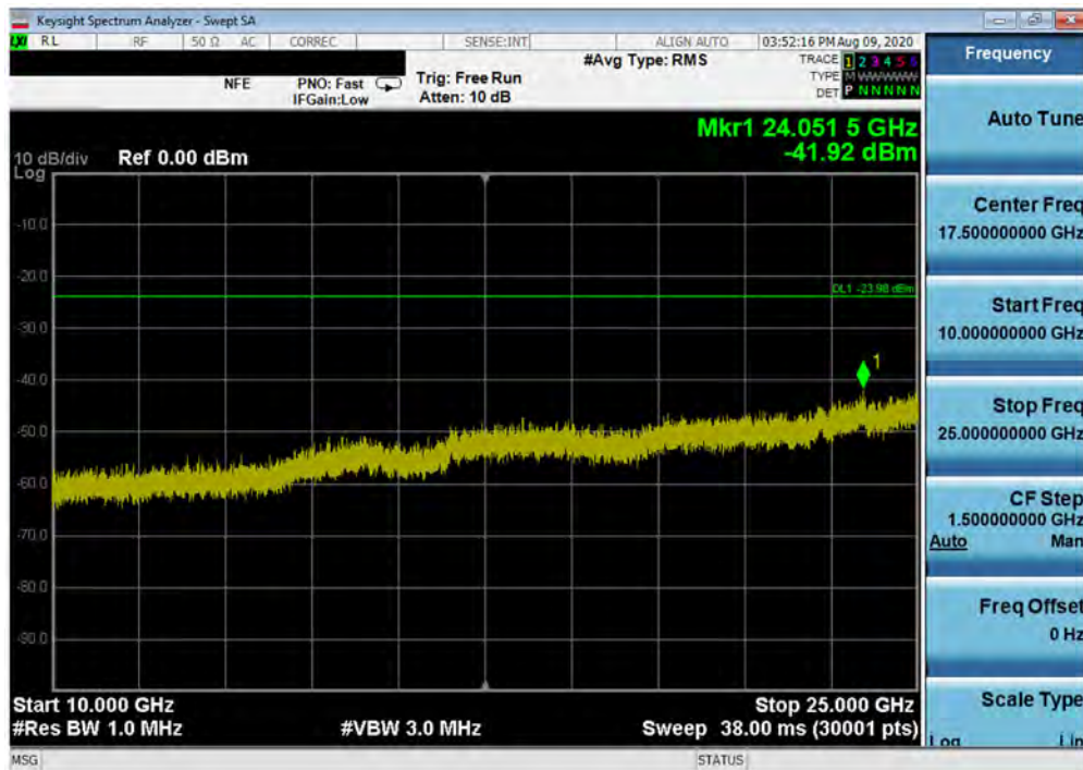
Plot 7-60. Conducted Spurious Plot SISO ANT2 (802.11ax OFDMA – 242 Tones – Ch. 1)
