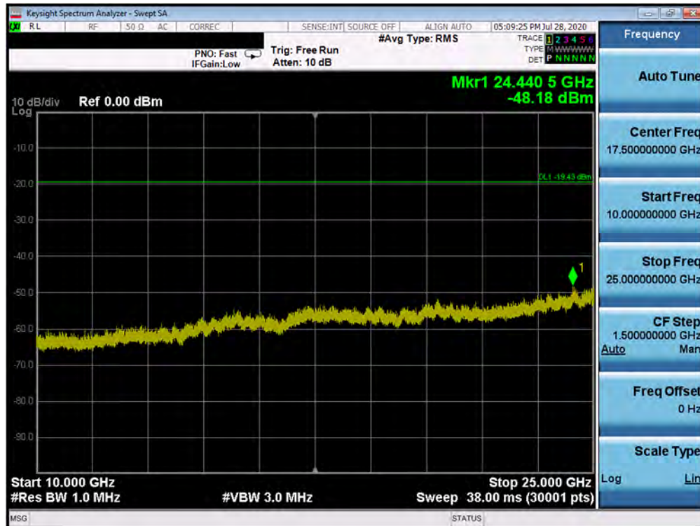
Plot 7-58. Conducted Spurious Plot SISO ANT2 (802.11ax OFDMA – 26 Tones – Ch. 11)
