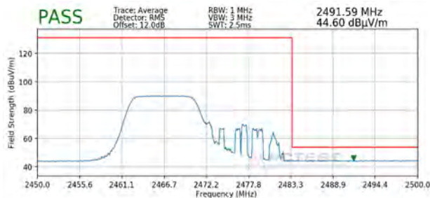
Plot 7-111. Radiated Restricted Upper Band Edge Measurement SISO ANT2 (Average – 106 Tones)
