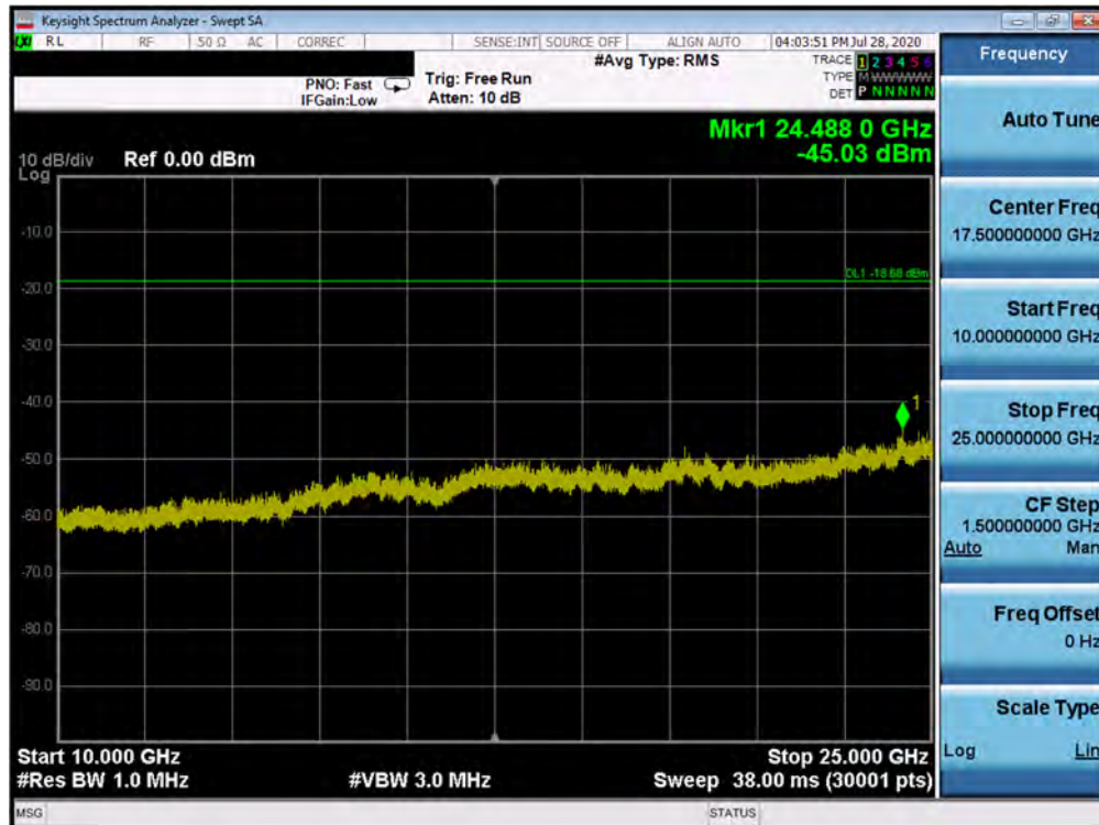
Plot 7-46. Conducted Spurious Plot SISO ANT1 (802.11ax OFDMA – 26 Tones – Ch. 11)
