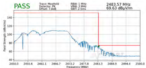
Plot 7-124. Radiated Restricted Upper Band Edge Measurement MIMO (Peak – 106 Tones)
