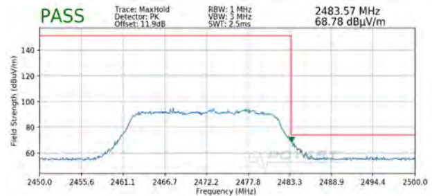
Plot 7-136. Radiated Restricted Upper Band Edge Measurement MIMO (Peak – 242 Tones)
