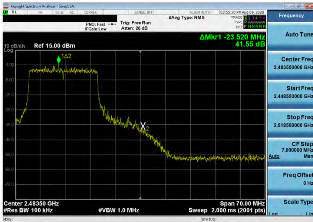
Plot 7-38. Band Edge Plot SISO ANT2 (802.11ax OFDMA - 242 Tones - Ch. 11)
