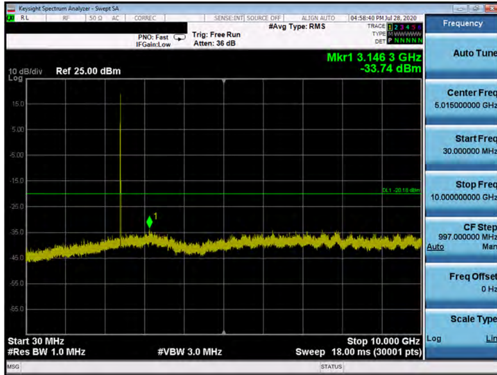
Plot 7-53. Conducted Spurious Plot SISO ANT2 (802.11ax OFDMA – 26 Tones – Ch. 1)
