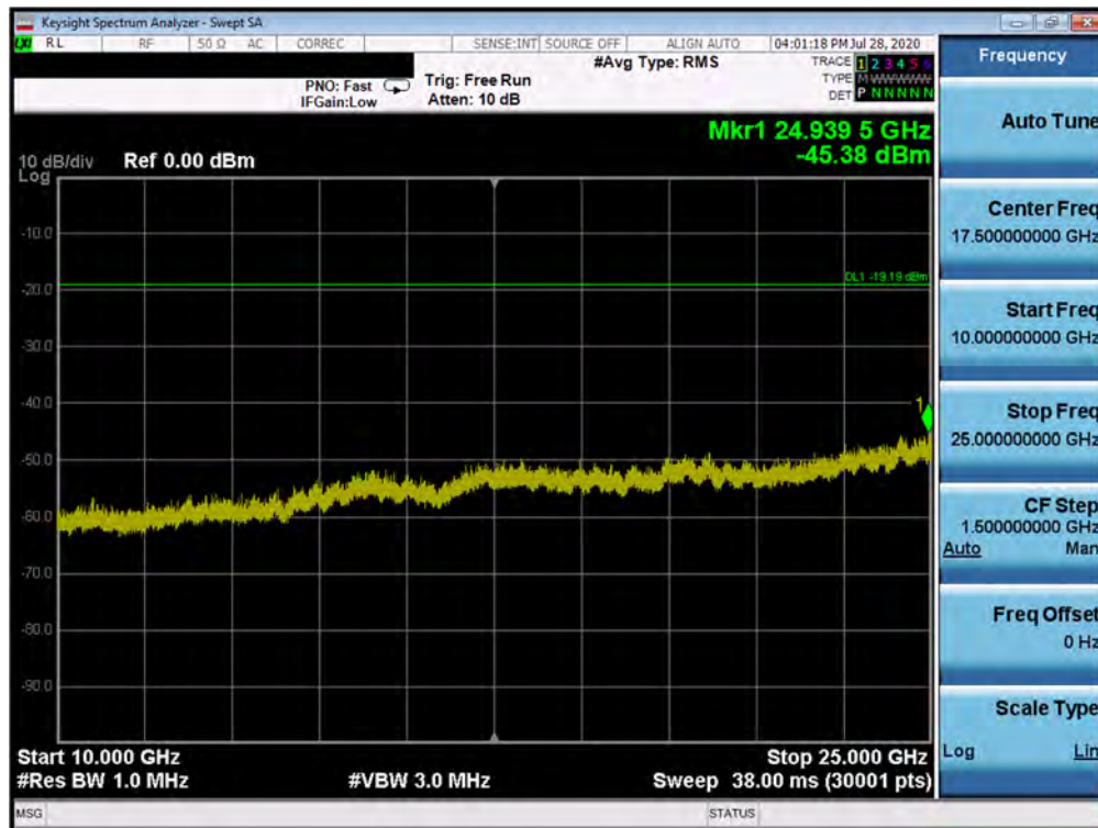
Plot 7-44. Conducted Spurious Plot SISO ANT1 (802.11ax OFDMA – 26 Tones – Ch. 6)
