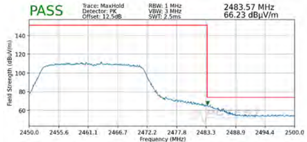
Plot 7-132. Radiated Restricted Upper Band Edge Measurement MIMO (Peak - 242 Tones)
