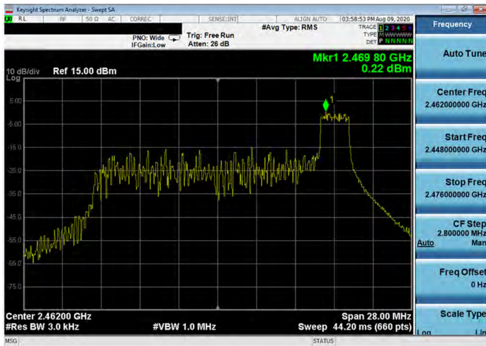
Plot 7-21. Power Spectral Density Plot SISO ANT2 (802.11ax OFDMA – 26 Tones – Ch. 11)
