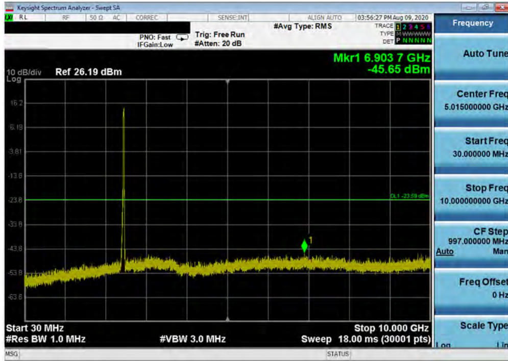
Plot 7-63. Conducted Spurious Plot SISO ANT2 (802.11ax OFDMA – 242 Tones – Ch. 11)
