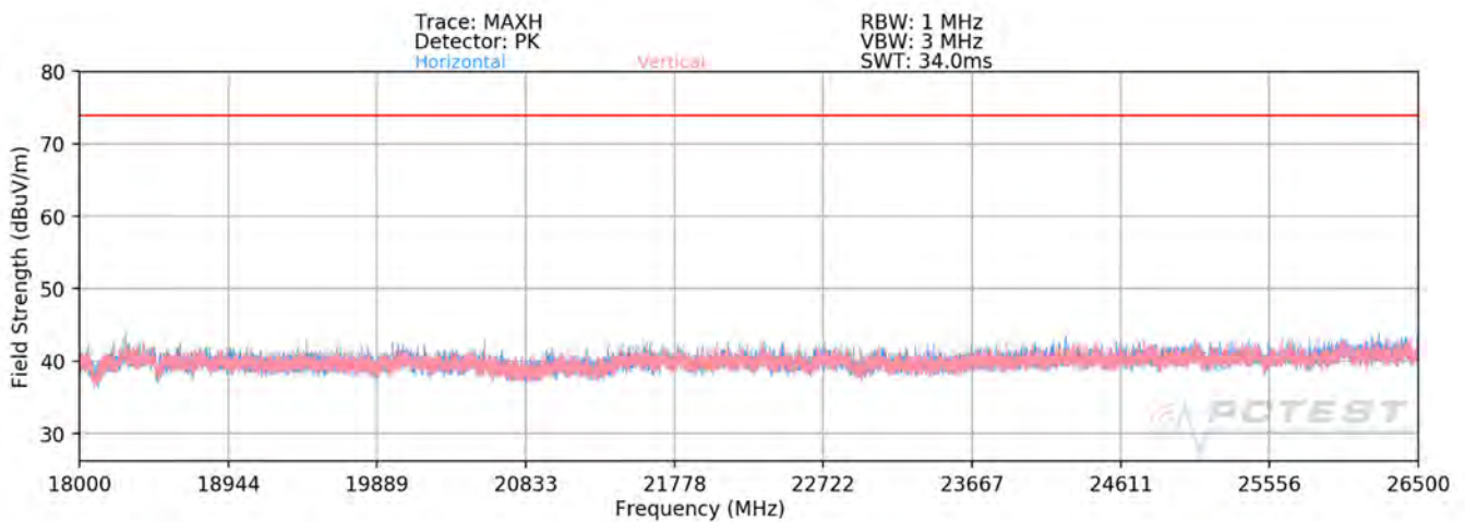
Plot 7-88. Radiated Spurious Plot above 18GHz MIMO (802.11ax OFDMA – 242 Tones)
