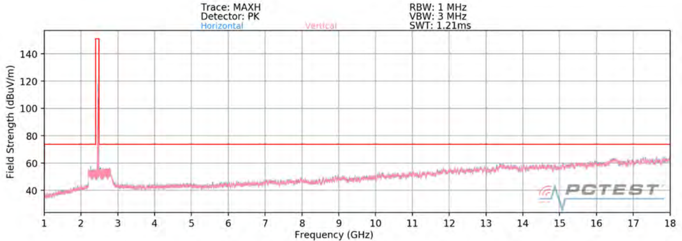
Plot 7-75. Radiated Spurious Plot above 1GHz SISO ANT2 (802.11ax OFDMA – 26 Tones – Ch. 11)
