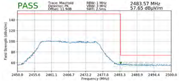
Plot 7-102. Radiated Restricted Upper Band Edge Measurement SISO ANT1 (Peak – 242 Tones)
