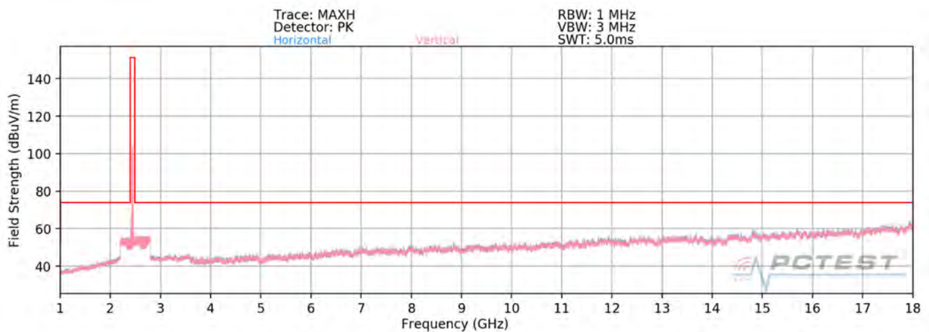
Plot 7-85. Radiated Spurious Plot above 1GHz MIMO (802.11ax OFDMA – 242 Tones – Ch. 6)
