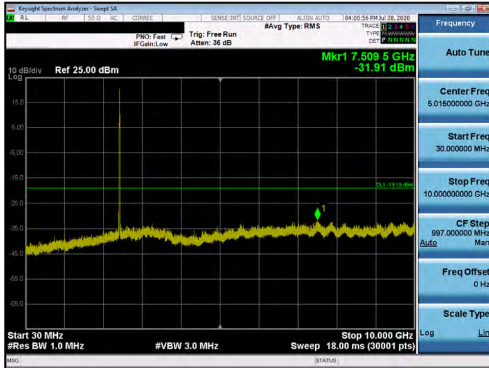
Plot 7-43. Conducted Spurious Plot SISO ANT1 (802.11ax OFDMA – 26 Tones – Ch. 6)
