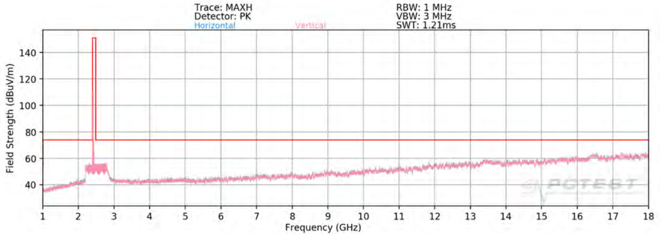
Plot 7-81. Radiated Spurious Plot above 1GHz MIMO (802.11ax OFDMA – 26 Tones – Ch. 1)
