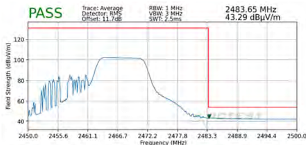
Plot 7-91. Radiated Restricted Upper Band Edge Measurement SISO ANT1 (Average – 106 Tones)
