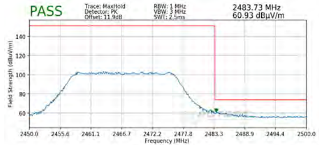
Plot 7-118. Radiated Restricted Upper Band Edge Measurement SISO ANT2 (Peak – 242 Tones)
