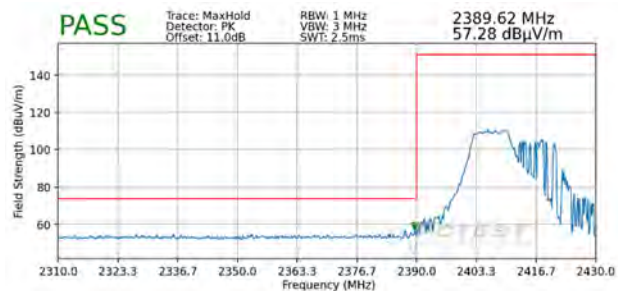
Plot 7-90. Radiated Restricted Lower Band Edge Measurement SISO ANT1 (Peak – 106 Tones)
