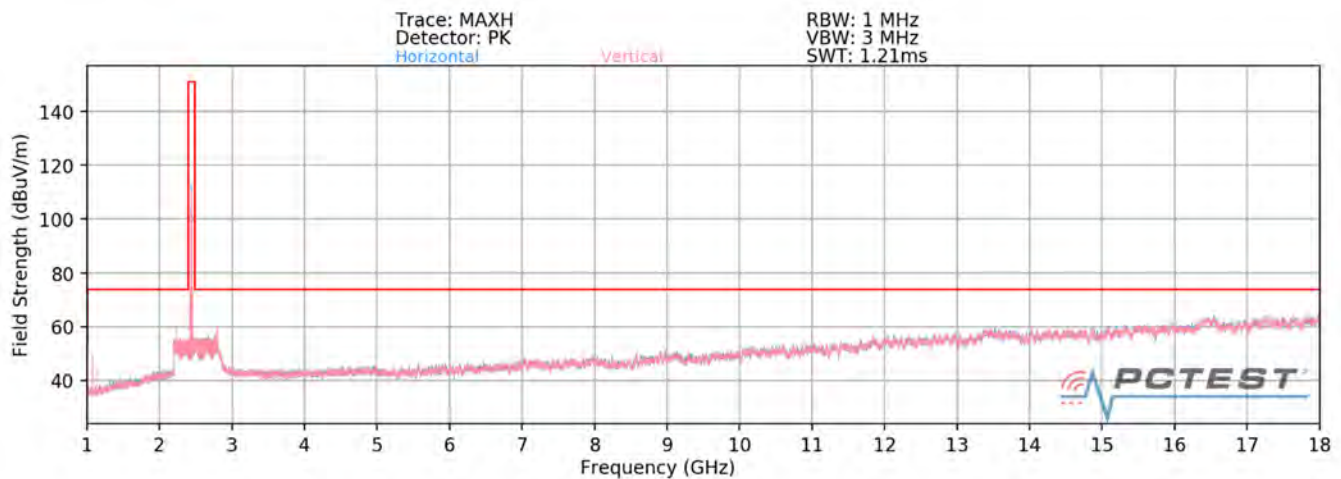
Plot 7-74. Radiated Spurious Plot above 1GHz SISO ANT2 (802.11ax OFDMA – 26 Tones – Ch. 6)
