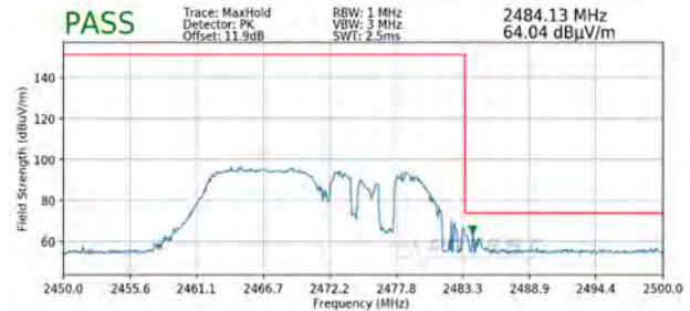
Plot 7-128. Radiated Restricted Upper Band Edge Measurement MIMO (Peak – 106 Tones)
