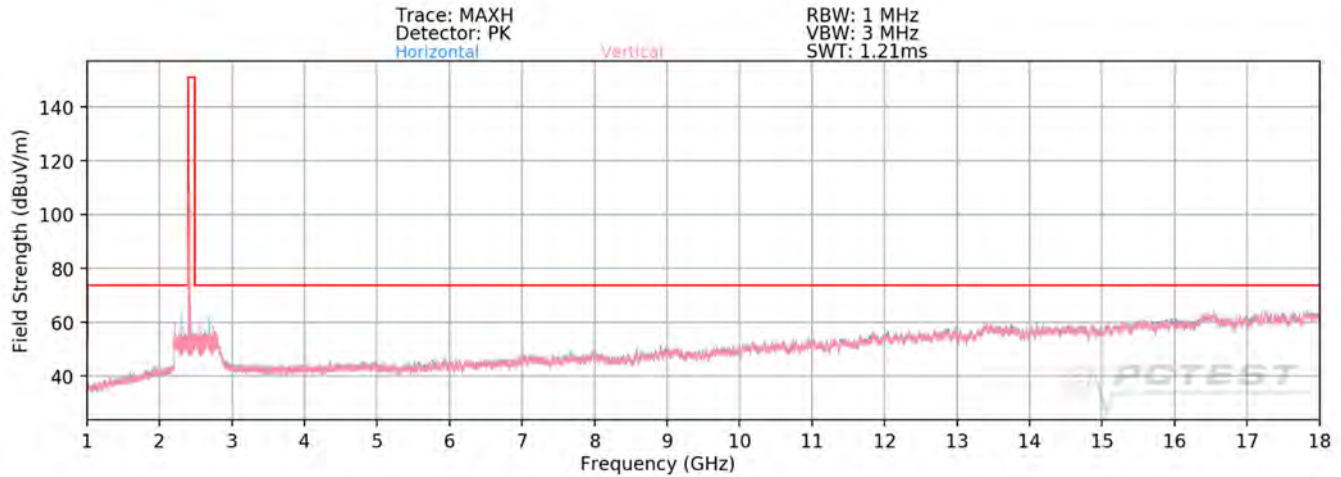
Plot 7-73. Radiated Spurious Plot above 1GHz SISO ANT2 (802.11ax OFDMA – 26 Tones – Ch. 1)
