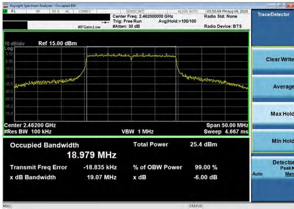
Plot 7-12. 6dB Bandwidth Plot SISO ANT2 (802.11ax OFDMA – 242 Tones – Ch. 11)
