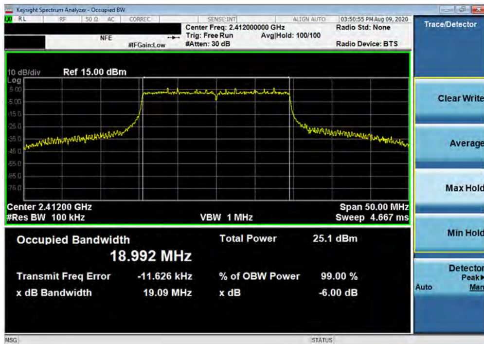
Plot 7-10. 6dB Bandwidth Plot SISO ANT2 (802.11ax OFDMA – 242 Tones – Ch. 1)
