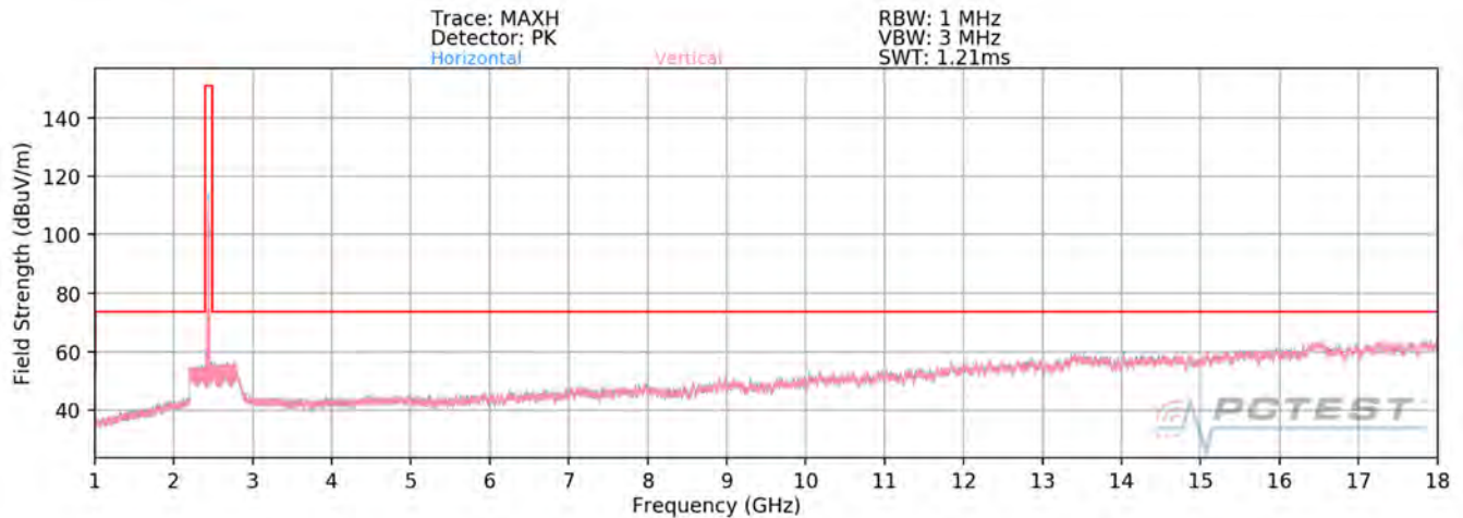
Plot 7-82. Radiated Spurious Plot above 1GHz MIMO (802.11ax OFDMA – 26 Tones – Ch. 6)
