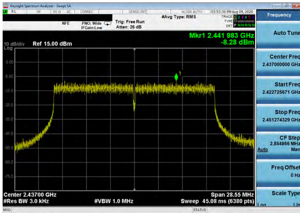
Plot 7-23. Power Spectral Density Plot SISO ANT2 (802.11ax OFDMA – 242 Tones – Ch. 6)
