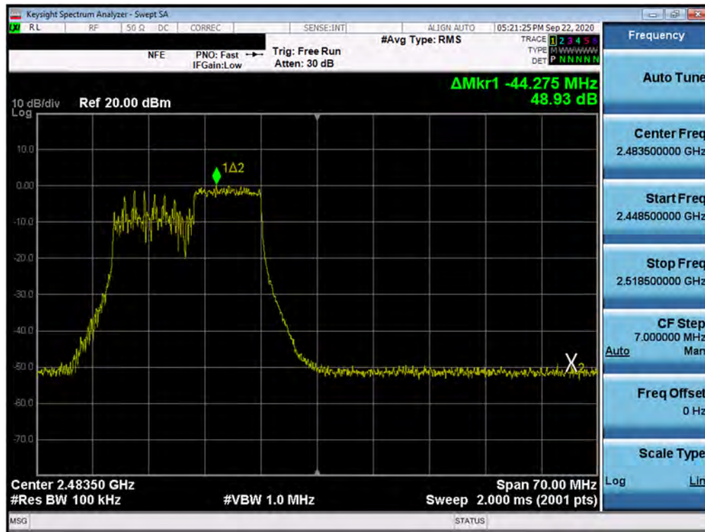
Plot 7-35. Band Edge Plot SISO ANT2 (802.11ax OFDMA - 106 Tones - Ch. 12)
