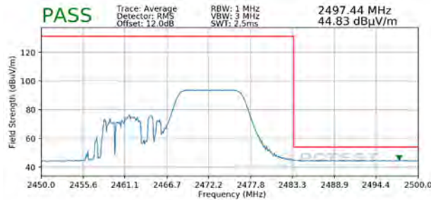
Plot 7-93. Radiated Restricted Upper Band Edge Measurement SISO ANT1 (Average – 106 Tones)
