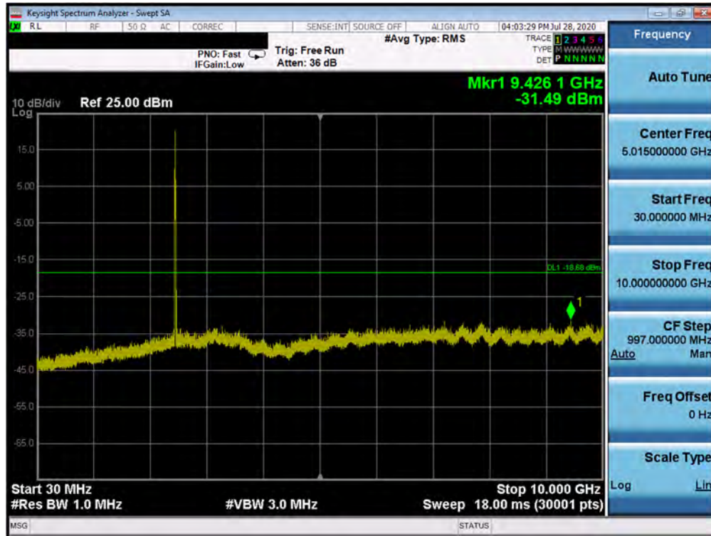
Plot 7-45. Conducted Spurious Plot SISO ANT1 (802.11ax OFDMA – 26 Tones – Ch. 11)
