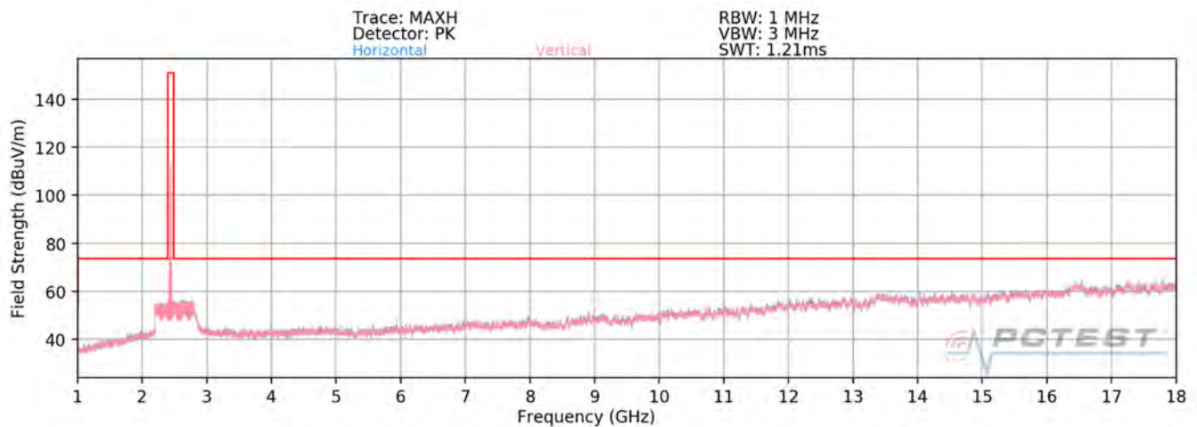
Plot 7-66. Radiated Spurious Plot above 1GHz SISO ANT1 (802.11ax OFDMA – 26 Tones – Ch. 6)
