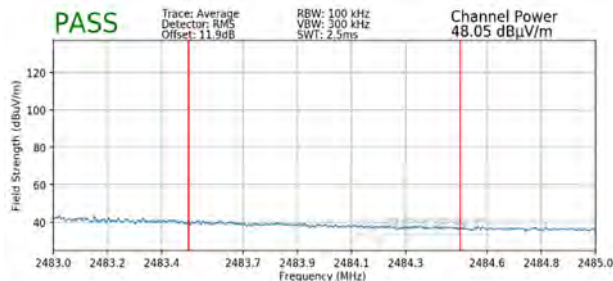
Plot 7-119. Radiated Restricted Upper Band Edge Measurement SISO ANT2 (Average – 242 Tones)
