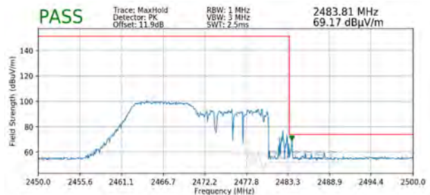
Plot 7-112. Radiated Restricted Upper Band Edge Measurement SISO ANT2 (Peak – 106 Tones)
