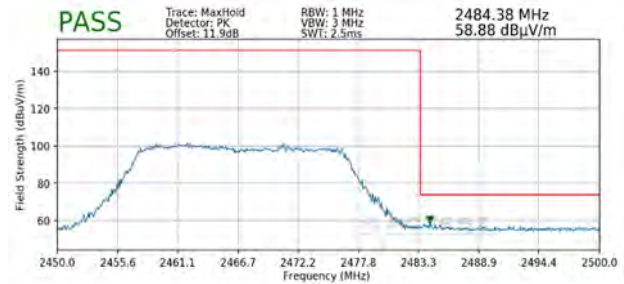
Plot 7-134. Radiated Restricted Upper Band Edge Measurement MIMO (Peak – 242 Tones)
