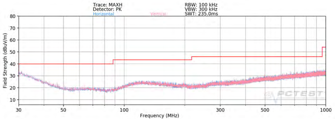
Plot 7-138. Radiated Spurious Plot below 1GHz MIMO (242 Tones)
