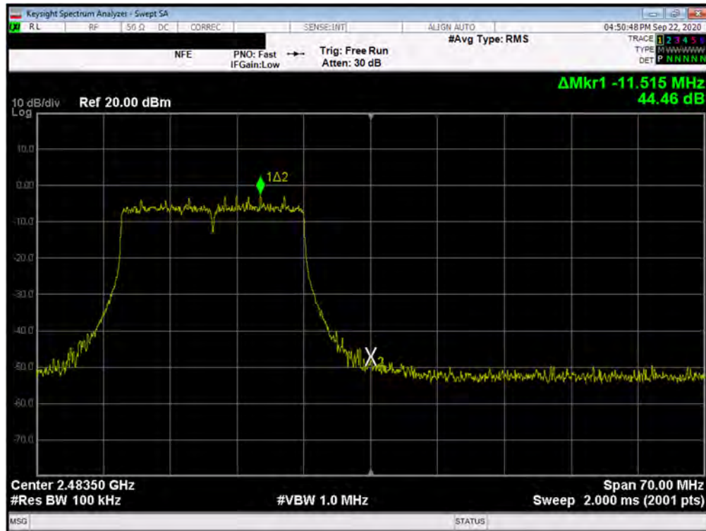
Plot 7-39. Band Edge Plot SISO ANT2 (802.11ax OFDMA - 242 Tones - Ch. 12)
