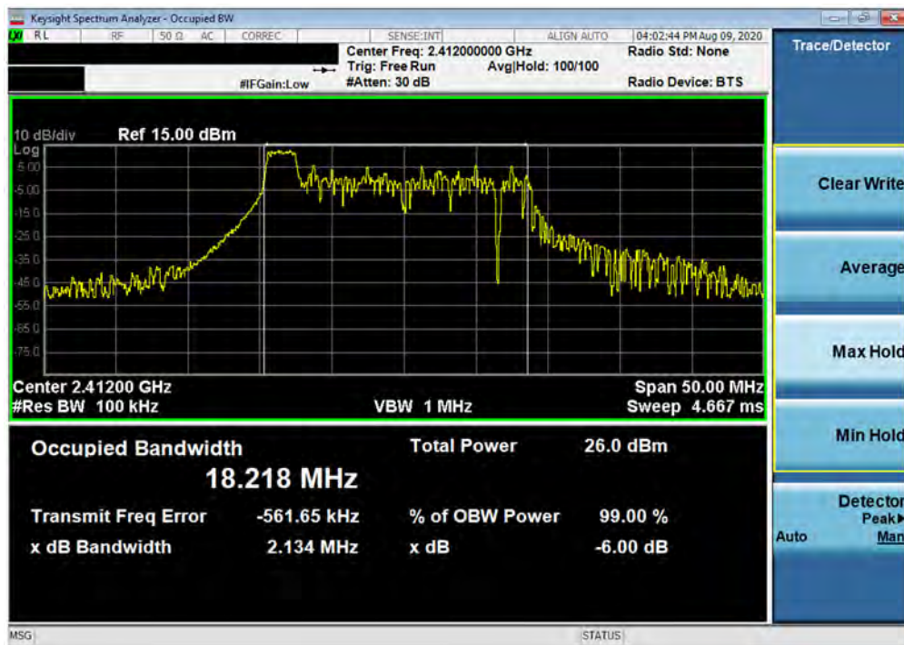
Plot 7-7. 6dB Bandwidth Plot SISO ANT2 (802.11ax OFDMA – 26 Tones – Ch. 1)
