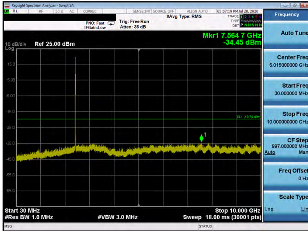
Plot 7-55. Conducted Spurious Plot SISO ANT2 (802.11ax OFDMA – 26 Tones – Ch. 6)
