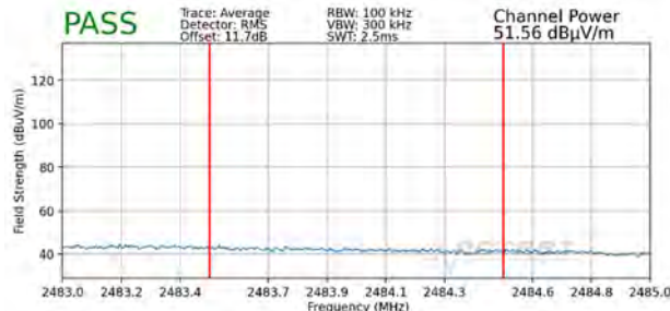
Plot 7-115. Radiated Restricted Upper Band Edge Measurement SISO ANT2 (Average - 242 Tones)
