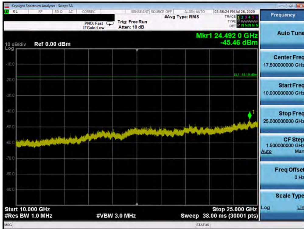
Plot 7-42. Conducted Spurious Plot SISO ANT1 (802.11ax OFDMA – 26 Tones – Ch. 1)
