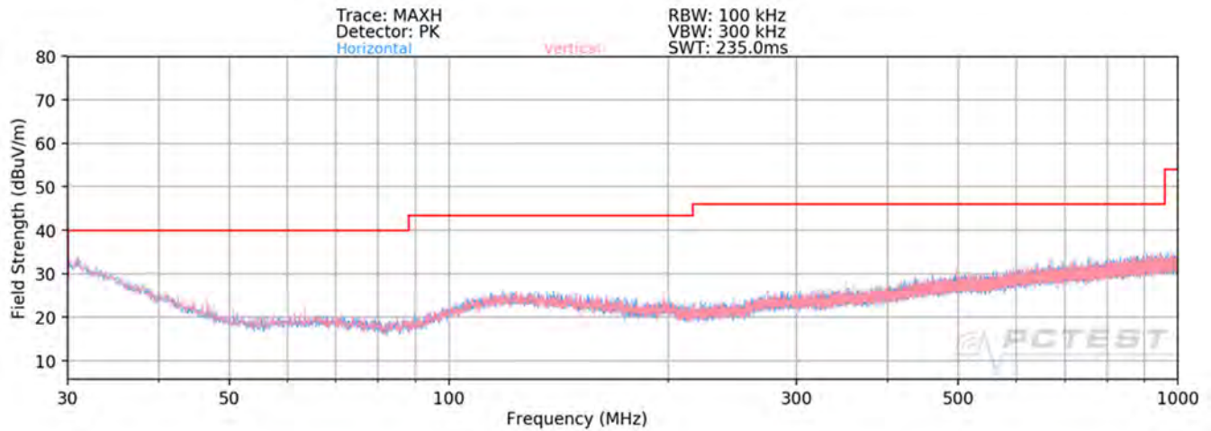
Plot 7-137. Radiated Spurious Plot below 1GHz MIMO (26 Tones)
