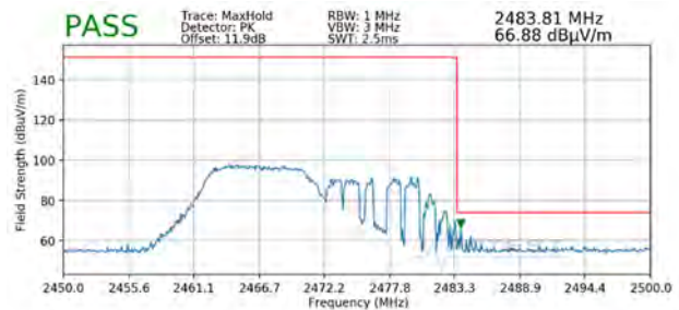
Plot 7-96. Radiated Restricted Upper Band Edge Measurement SISO ANT1 (Peak – 106 Tones)
