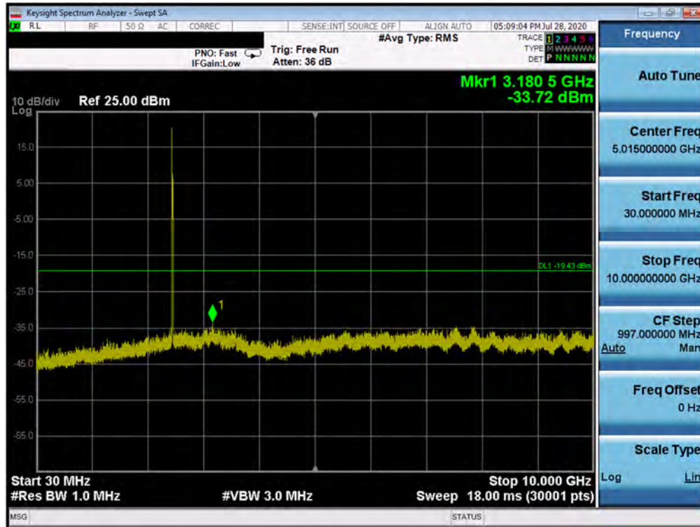
Plot 7-57. Conducted Spurious Plot SISO ANT2 (802.11ax OFDMA – 26 Tones – Ch. 11)
