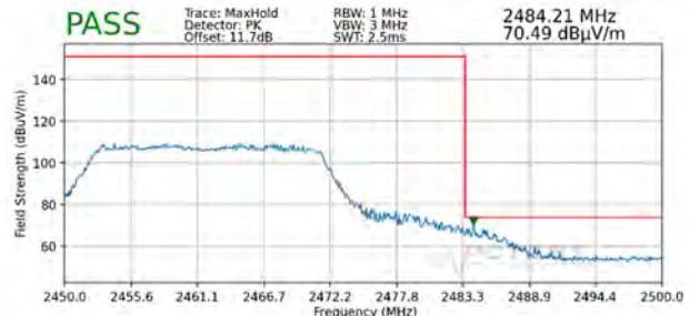
Plot 7-116. Radiated Restricted Upper Band Edge Measurement SISO ANT2 (Peak - 242 Tones)
