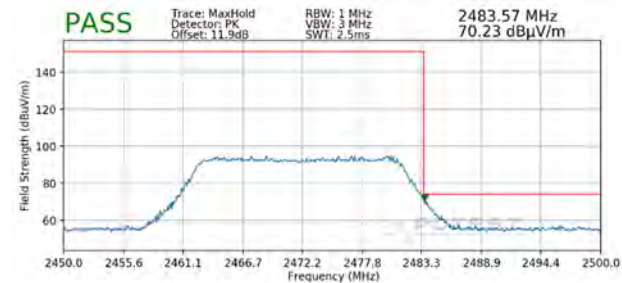
Plot 7-104. Radiated Restricted Upper Band Edge Measurement SISO ANT1 (Peak – 242 Tones)
