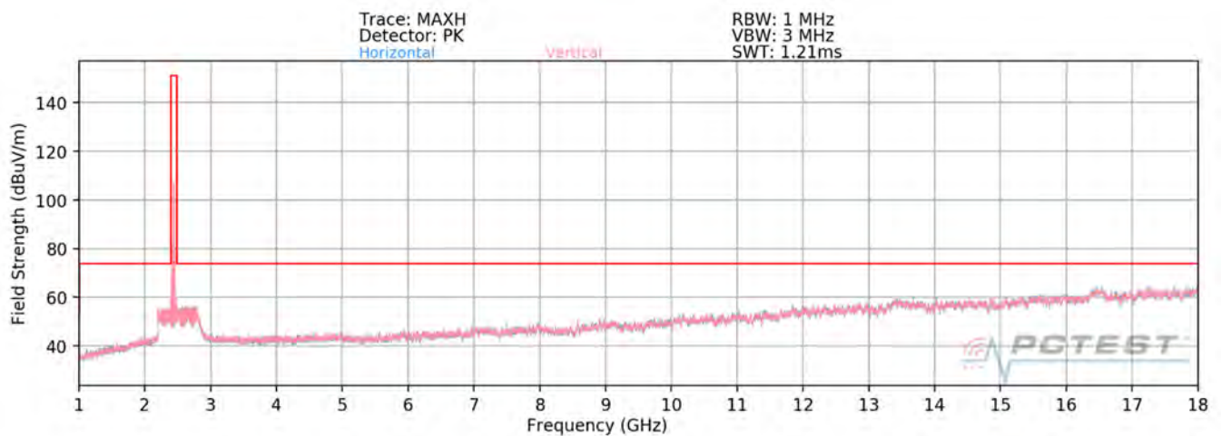
Plot 7-69. Radiated Spurious Plot above 1GHz SISO ANT1 (802.11ax OFDMA – 242 Tones – Ch. 6)
