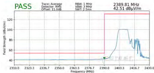
Plot 7-105. Radiated Restricted Lower Band Edge Measurement SISO ANT2 (Average – 106 Tones)
