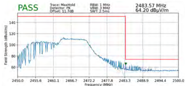
Plot 7-108. Radiated Restricted Upper Band Edge Measurement SISO ANT2 (Peak – 106 Tones)
