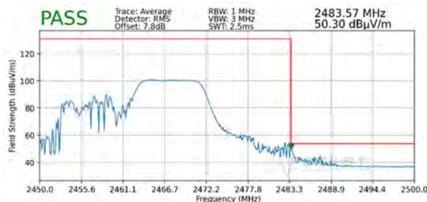
Plot 7-123. Radiated Restricted Upper Band Edge Measurement MIMO (Average – 106 Tones)
