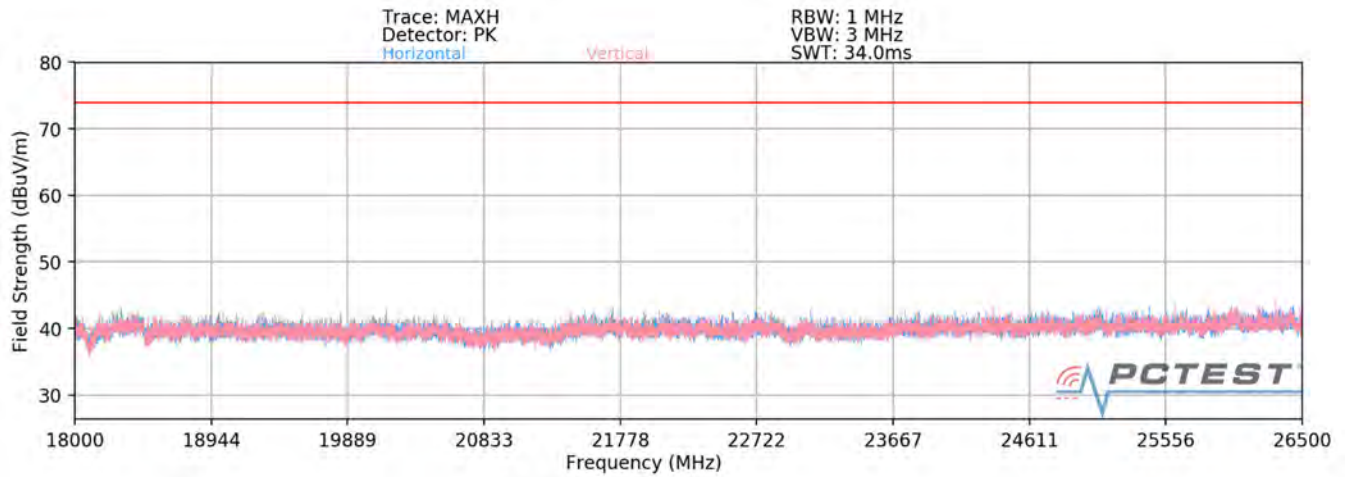
Plot 7-79. Radiated Spurious Plot above 18GHz SISO ANT2 (802.11ax OFDMA – 26 Tones)
