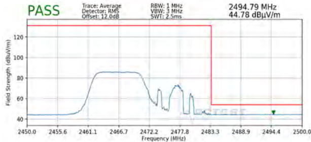
Plot 7-127. Radiated Restricted Upper Band Edge Measurement MIMO (Average – 106 Tones)
