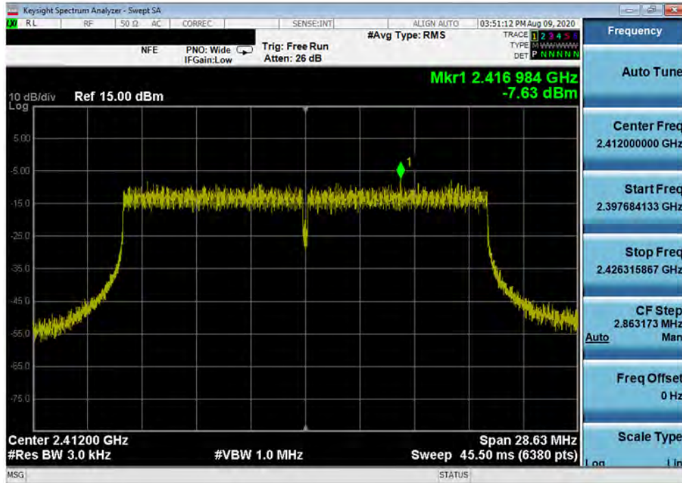
Plot 7-22. Power Spectral Density Plot SISO ANT2 (802.11ax OFDMA – 242 Tones – Ch. 1)
