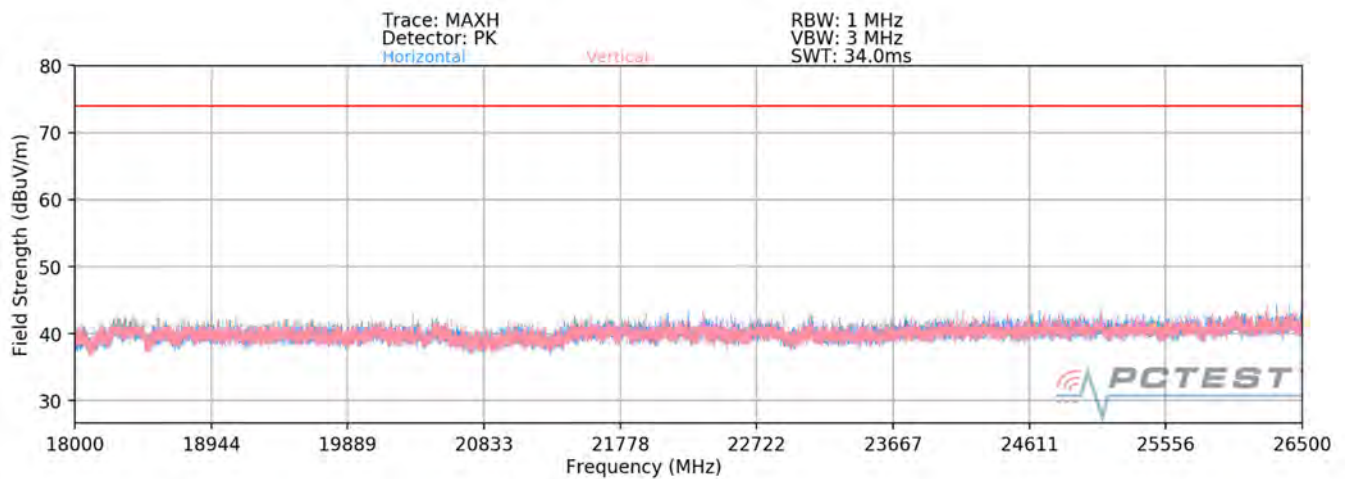
Plot 7-72. Radiated Spurious Plot above 18GHz SISO ANT1 (802.11ax OFDMA – 242 Tones)
