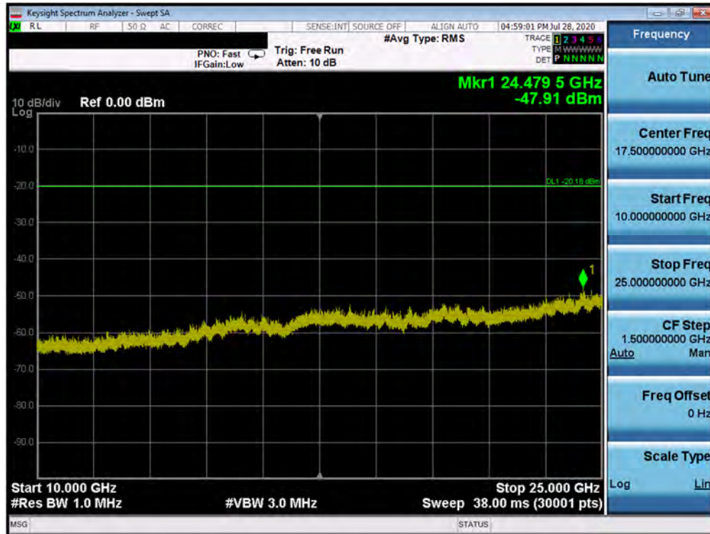
Plot 7-54. Conducted Spurious Plot SISO ANT2 (802.11ax OFDMA – 26 Tones – Ch. 1)
