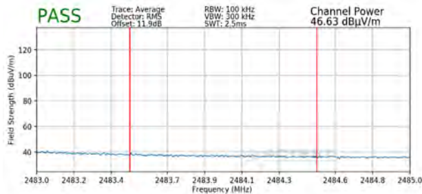
Plot 7-135. Radiated Restricted Upper Band Edge Measurement MIMO (Average – 242 Tones)
