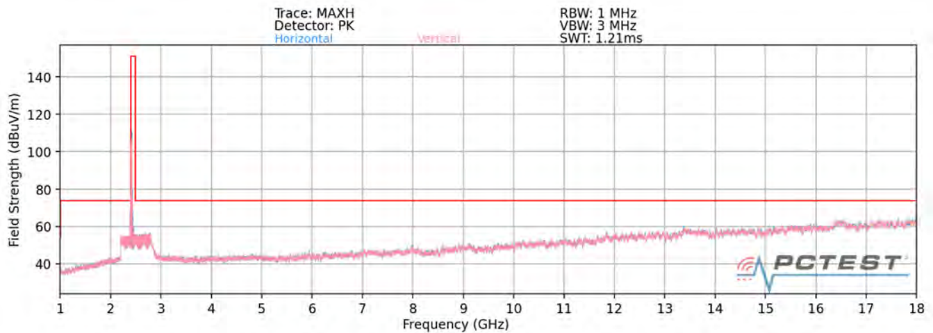
Plot 7-76. Radiated Spurious Plot above 1GHz SISO ANT2 (802.11ax OFDMA – 242 Tones – Ch. 1)
