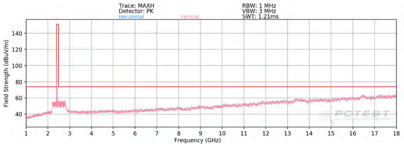
Plot 7-68. Radiated Spurious Plot above 1GHz SISO ANT1 (802.11ax OFDMA – 242 Tones – Ch. 1)
