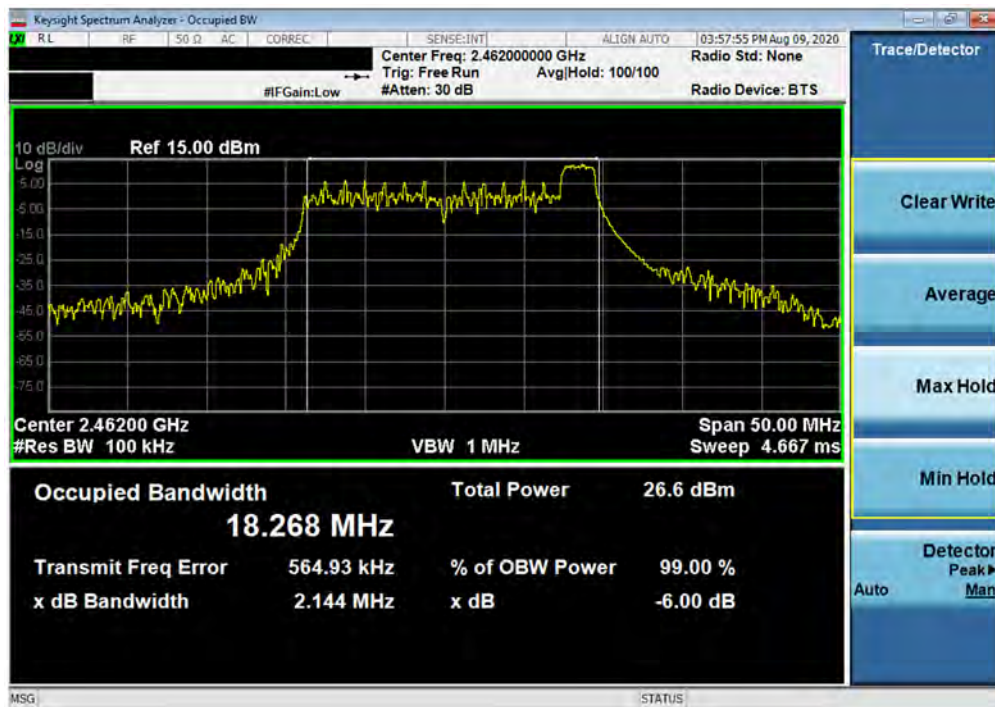
Plot 7-9. 6dB Bandwidth Plot SISO ANT2 (802.11ax OFDMA – 26 Tones – Ch. 11)
