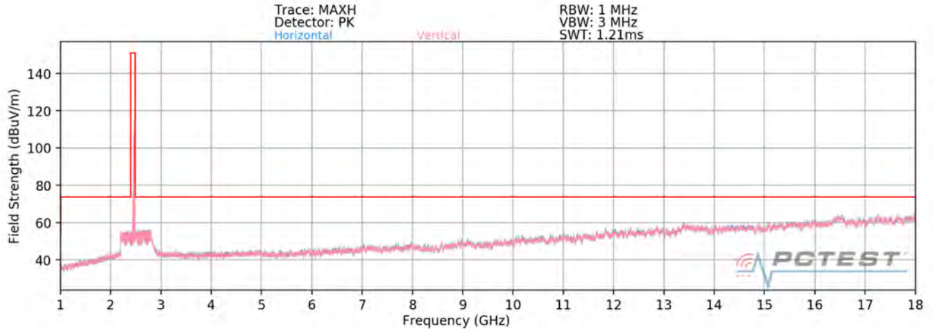
Plot 7-67. Radiated Spurious Plot above 1GHz SISO ANT1 (802.11ax OFDMA – 26 Tones – Ch. 11)
