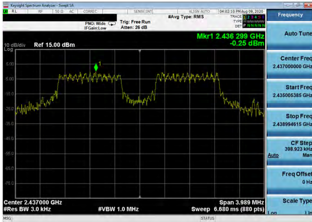
Plot 7-20. Power Spectral Density Plot SISO ANT2 (802.11ax OFDMA – 26 Tones – Ch. 6)
