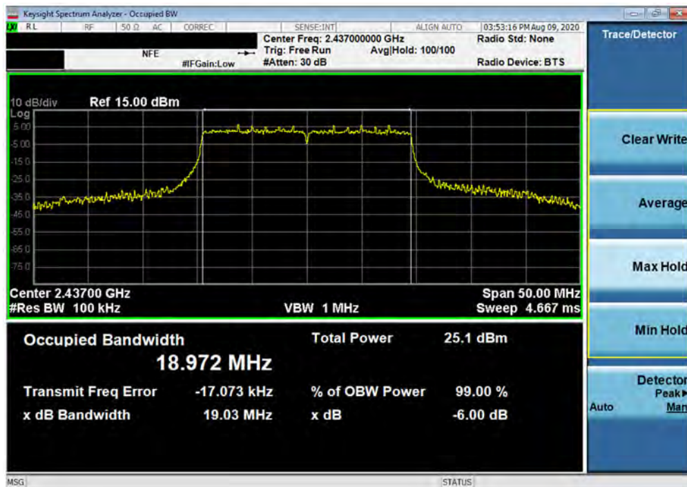
Plot 7-11. 6dB Bandwidth Plot SISO ANT2 (802.11ax OFDMA – 242 Tones – Ch. 6)
