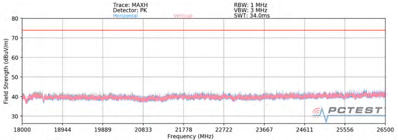
Plot 7-71. Radiated Spurious Plot above 18GHz SISO ANT1 (802.11ax OFDMA – 26 Tones)
