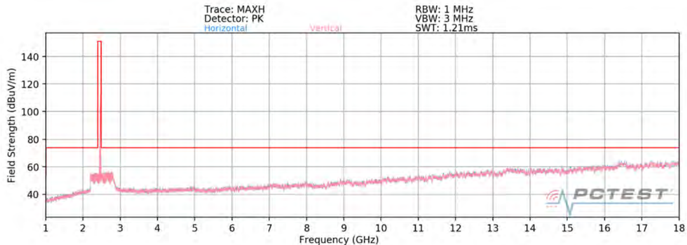
Plot 7-70. Radiated Spurious Plot above 1GHz SISO ANT1 (802.11ax OFDMA – 242 Tones – Ch. 11)
