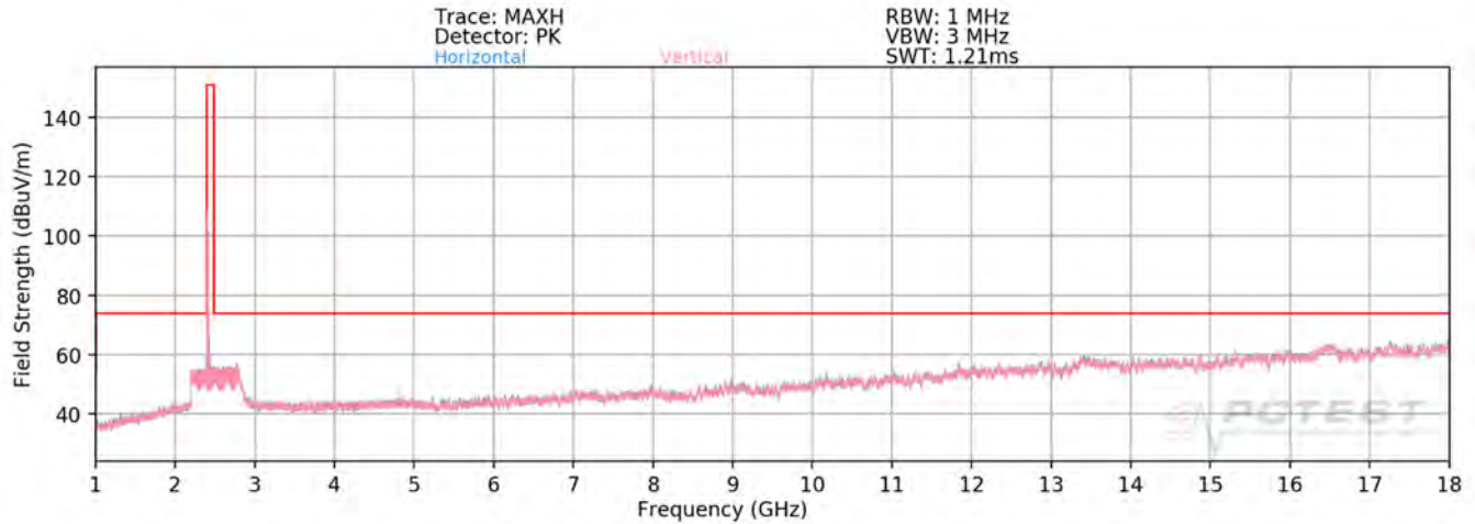
Plot 7-65. Radiated Spurious Plot above 1GHz SISO ANT1 (802.11ax OFDMA – 26 Tones – Ch. 1)
