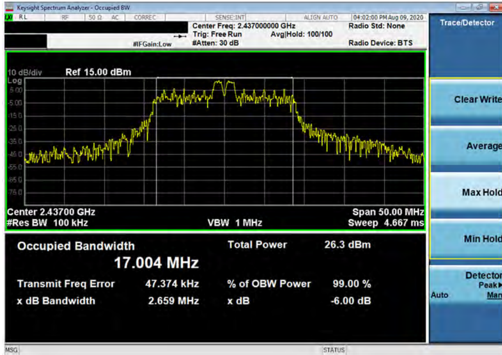
Plot 7-8. 6dB Bandwidth Plot SISO ANT2 (802.11ax OFDMA – 26 Tones – Ch. 6)
