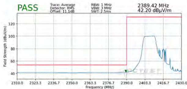
Plot 7-89. Radiated Restricted Lower Band Edge Measurement SISO ANT1 (Average – 106 Tones)
