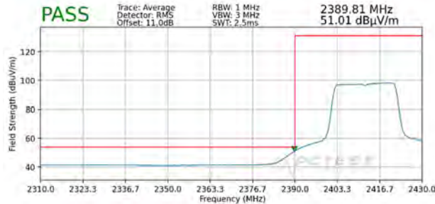
Plot 7-113. Radiated Restricted Lower Band Edge Measurement SISO ANT2 (Average - 242 Tones)
