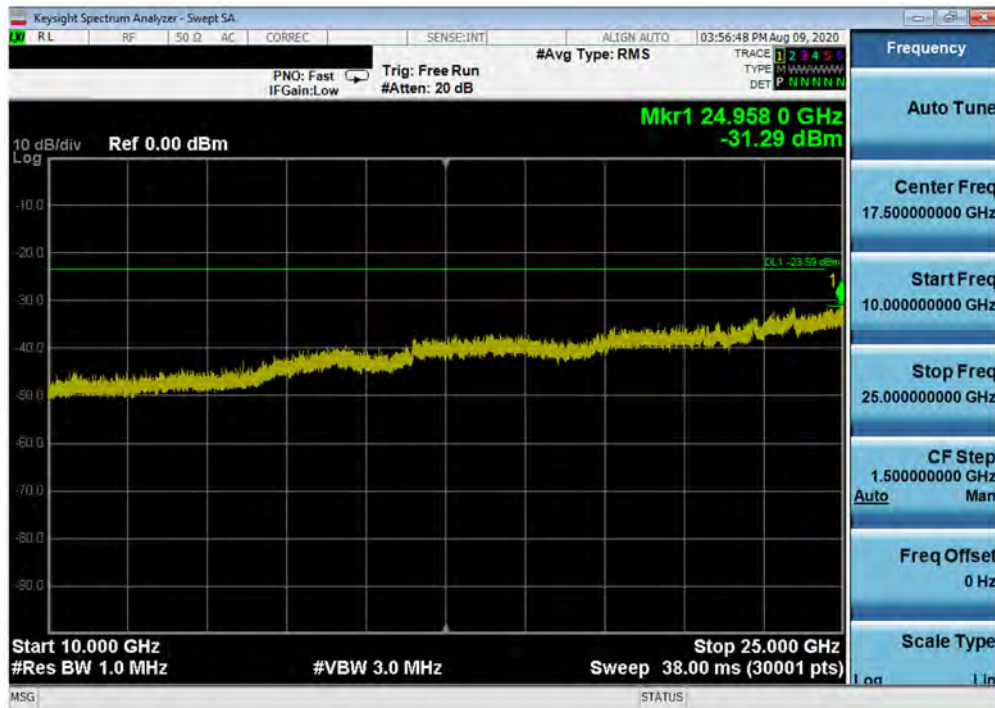
Plot 7-64. Conducted Spurious Plot SISO ANT2 (802.11ax OFDMA – 242 Tones – Ch. 11)
