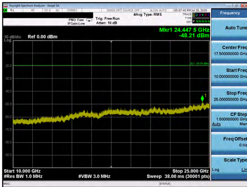
Plot 7-56. Conducted Spurious Plot SISO ANT2 (802.11ax OFDMA – 26 Tones – Ch. 6)
