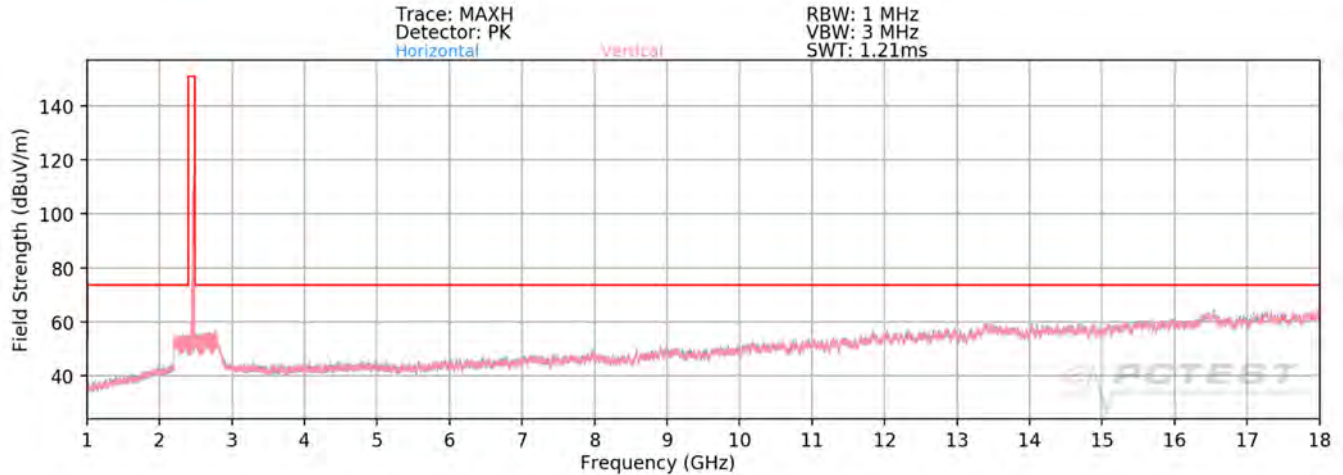
Plot 7-83. Radiated Spurious Plot above 1GHz MIMO (802.11ax OFDMA – 26 Tones – Ch. 11)
