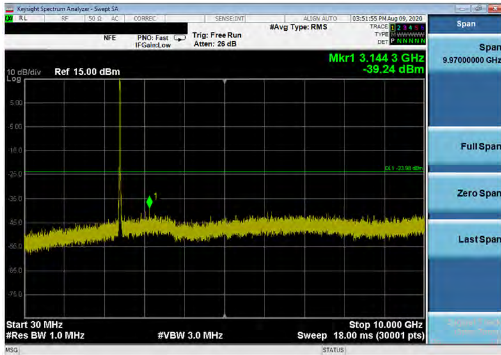
Plot 7-59. Conducted Spurious Plot SISO ANT2 (802.11ax OFDMA – 242 Tones – Ch. 1)
