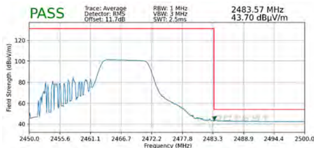
Plot 7-107. Radiated Restricted Upper Band Edge Measurement SISO ANT2 (Average – 106 Tones)
