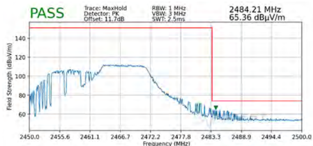
Plot 7-92. Radiated Restricted Upper Band Edge Measurement SISO ANT1 (Peak – 106 Tones)
