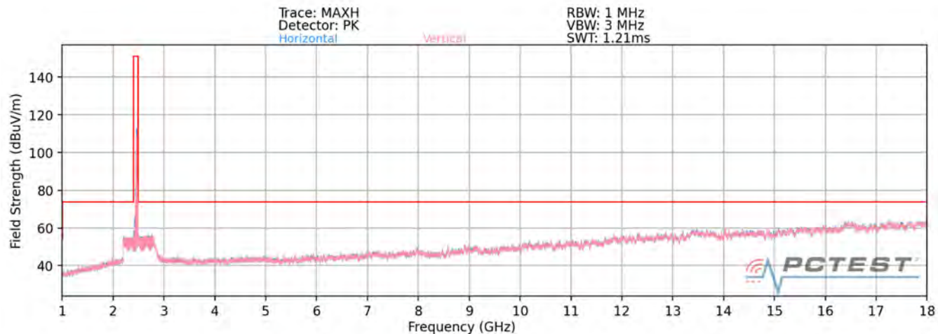
Plot 7-78. Radiated Spurious Plot above 1GHz SISO ANT2 (802.11ax OFDMA – 242 Tones – Ch. 11)
