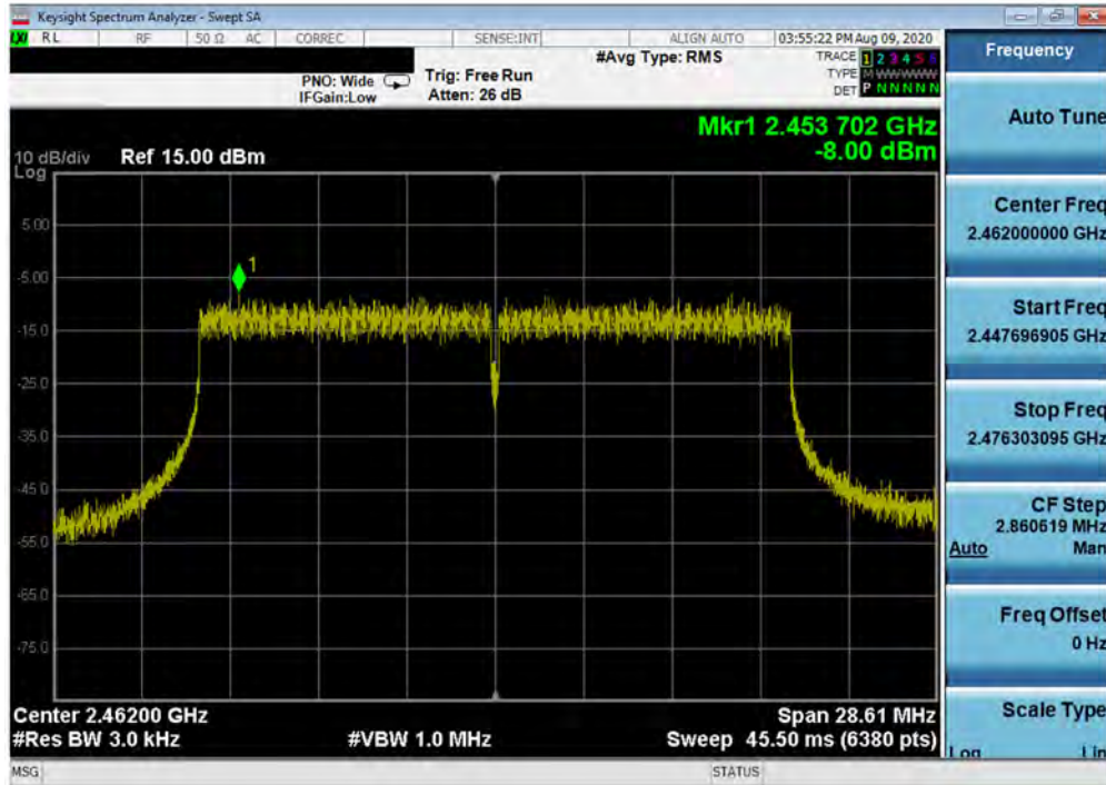
Plot 7-24. Power Spectral Density Plot SISO ANT2 (802.11ax OFDMA – 242 Tones – Ch. 11)
