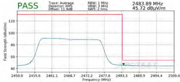
Plot 7-101. Radiated Restricted Upper Band Edge Measurement SISO ANT1 (Average – 242 Tones)
