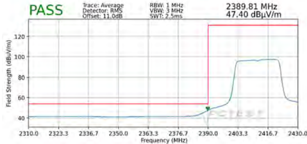
Plot 7-97. Radiated Restricted Lower Band Edge Measurement SISO ANT1 (Average - 242 Tones)
