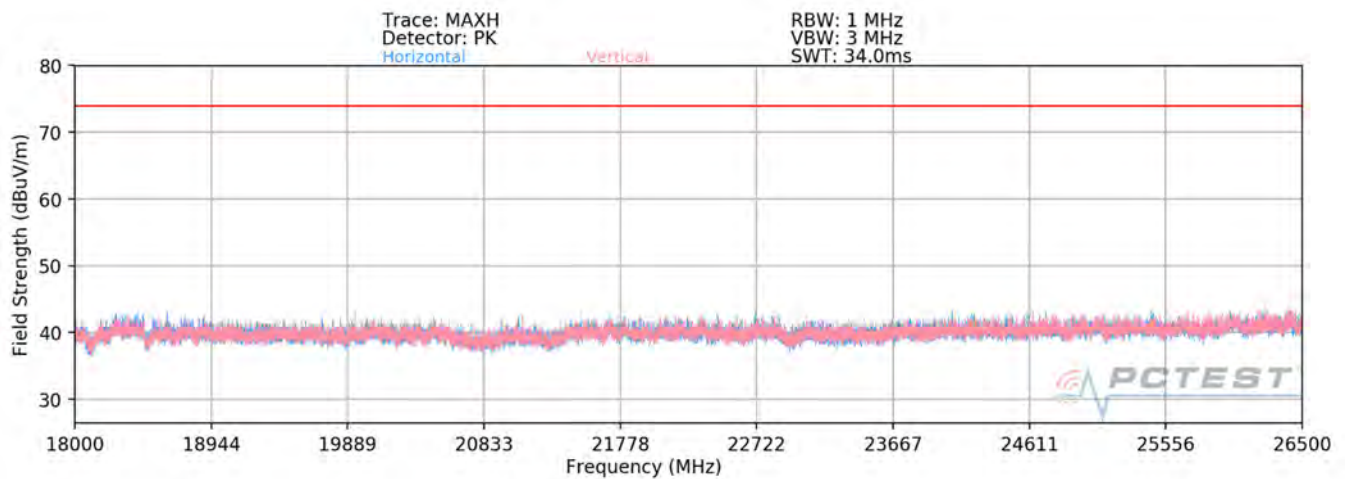
Plot 7-80. Radiated Spurious Plot above 18GHz SISO ANT2 (802.11ax OFDMA – 242 Tones)
