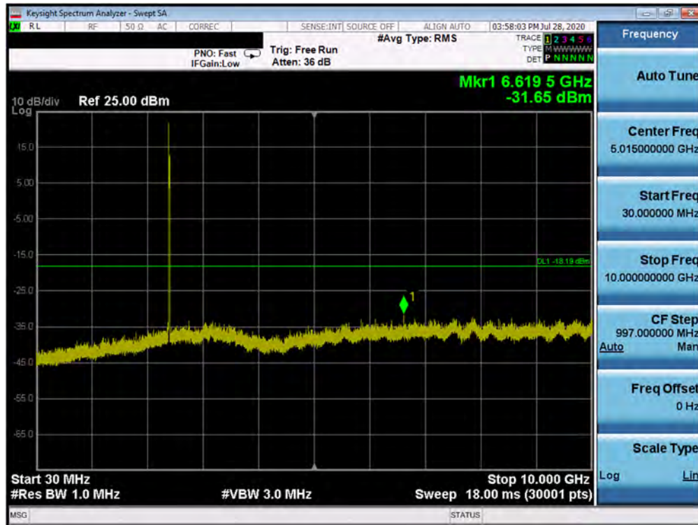
Plot 7-41. Conducted Spurious Plot SISO ANT1 (802.11ax OFDMA – 26 Tones – Ch. 1)
