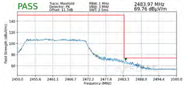
Plot 7-100. Radiated Restricted Upper Band Edge Measurement SISO ANT1 (Peak - 242 Tones)
