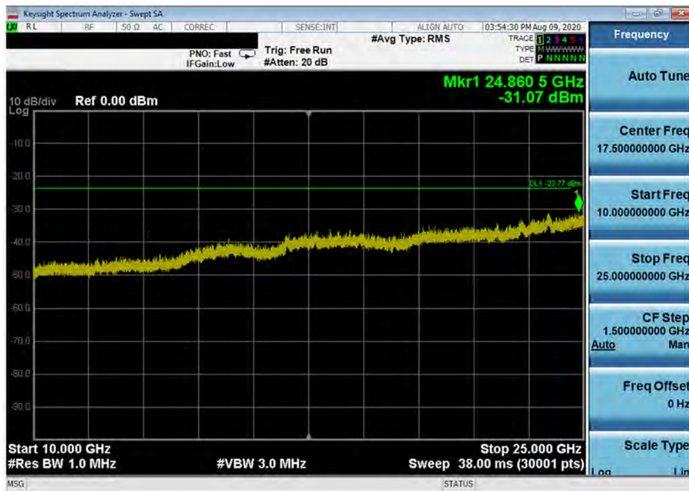
Plot 7-62. Conducted Spurious Plot SISO ANT2 (802.11ax OFDMA – 242 Tones – Ch. 6)
