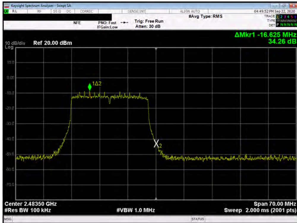
Plot 7-40. Band Edge Plot SISO ANT2 (802.11ax OFDMA - 242 Tones - Ch. 13)
