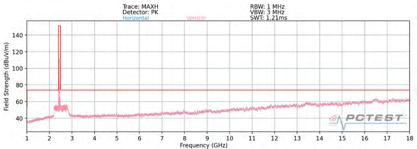
Plot 7-77. Radiated Spurious Plot above 1GHz SISO ANT2 (802.11ax OFDMA – 242 Tones – Ch. 6)
