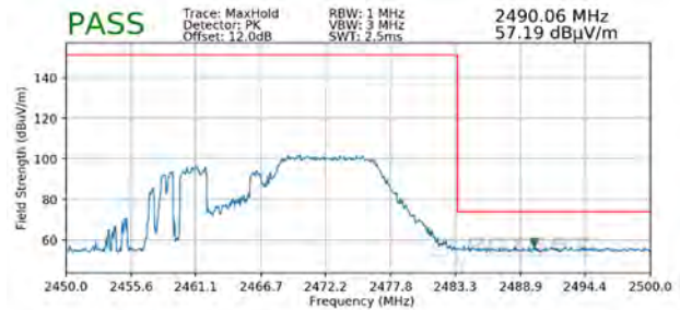
Plot 7-94. Radiated Restricted Upper Band Edge Measurement SISO ANT1 (Peak – 106 Tones)
