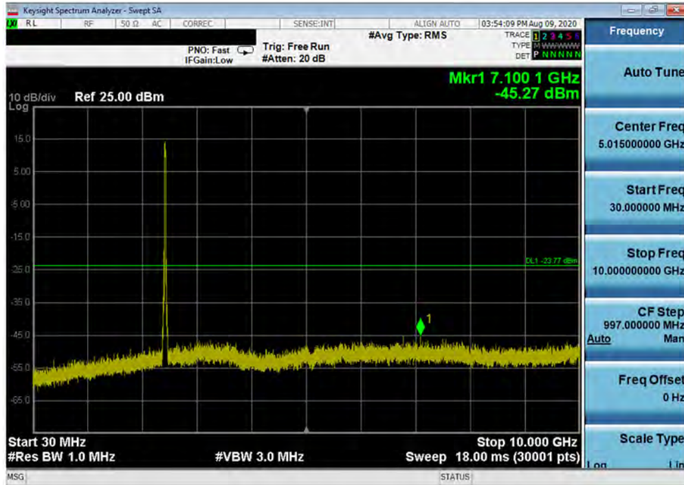
Plot 7-61. Conducted Spurious Plot SISO ANT2 (802.11ax OFDMA – 242 Tones – Ch. 6)
