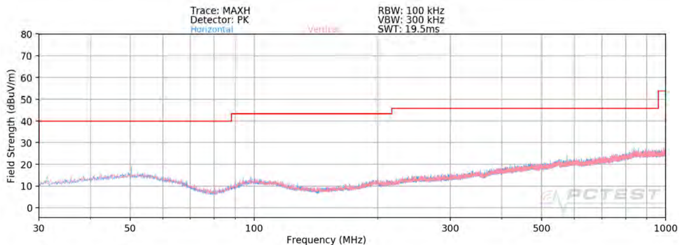
Plot 7-135. Radiated Spurious Plot below 1GHz
