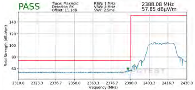
Plot 7-134. Radiated Restricted Band Edge Measurement MIMO with WCP (Peak)
