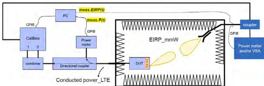
Figure 7-1 mmW NR radiated power measurement setup – Test Setup Photo 8
