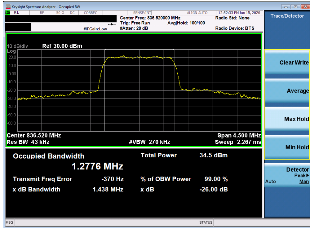
Plot 7-5. Occupied Bandwidth Plot (Cellular CDMA Mode)
