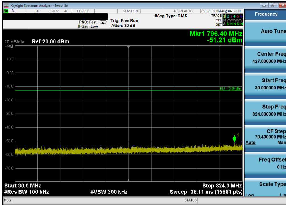
Plot 7-16. Conducted Spurious Plot (Cellular GPRS Mode - High Channel)
