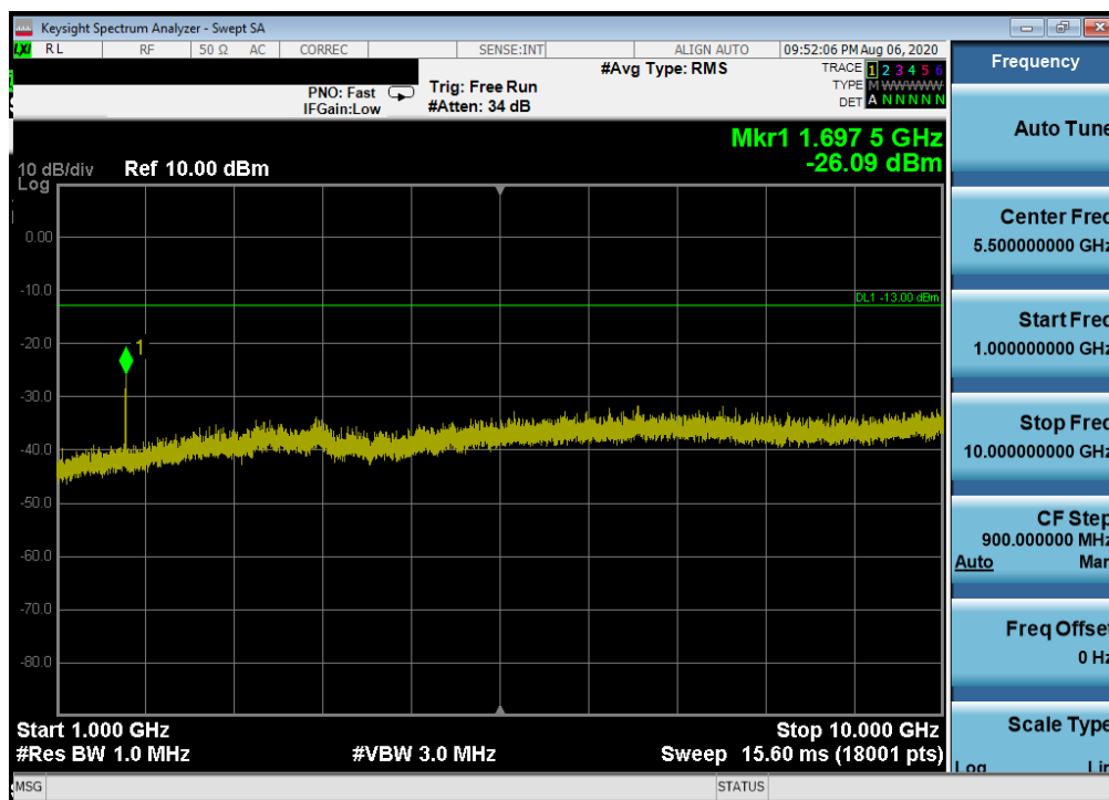
Plot 7-18. Conducted Spurious Plot (Cellular GPRS Mode - High Channel)
