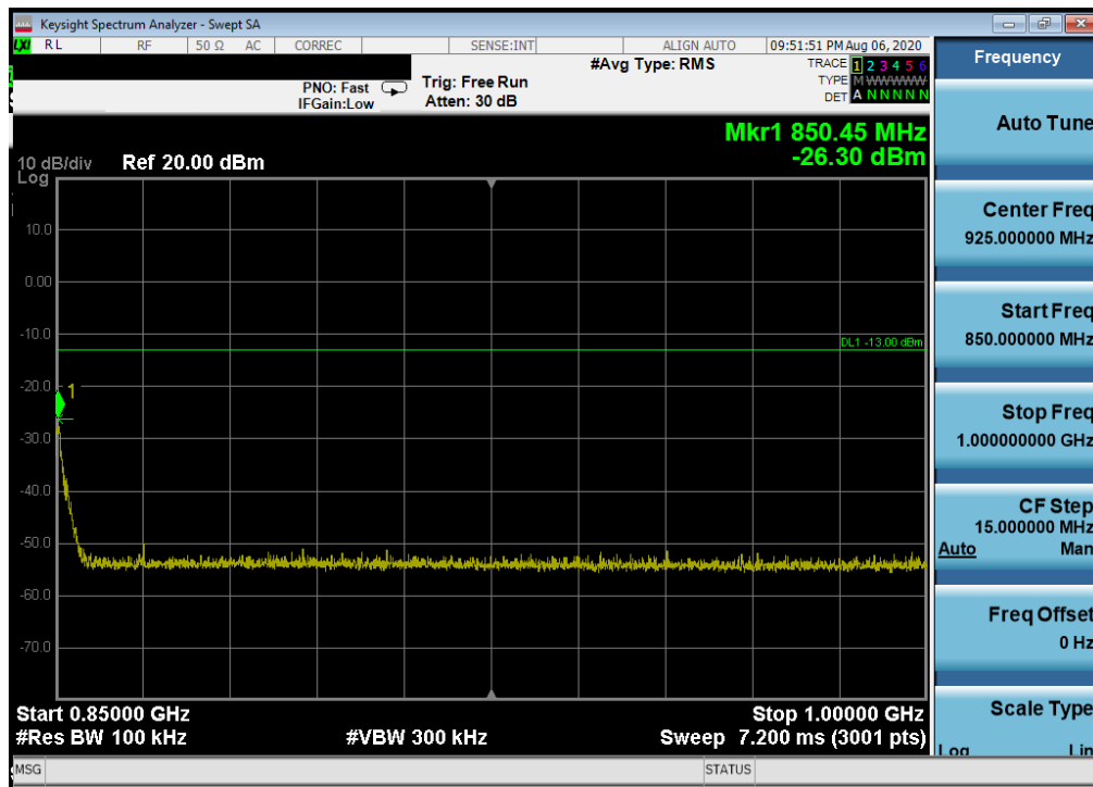
Plot 7-17. Conducted Spurious Plot (Cellular GPRS Mode - High Channel)
