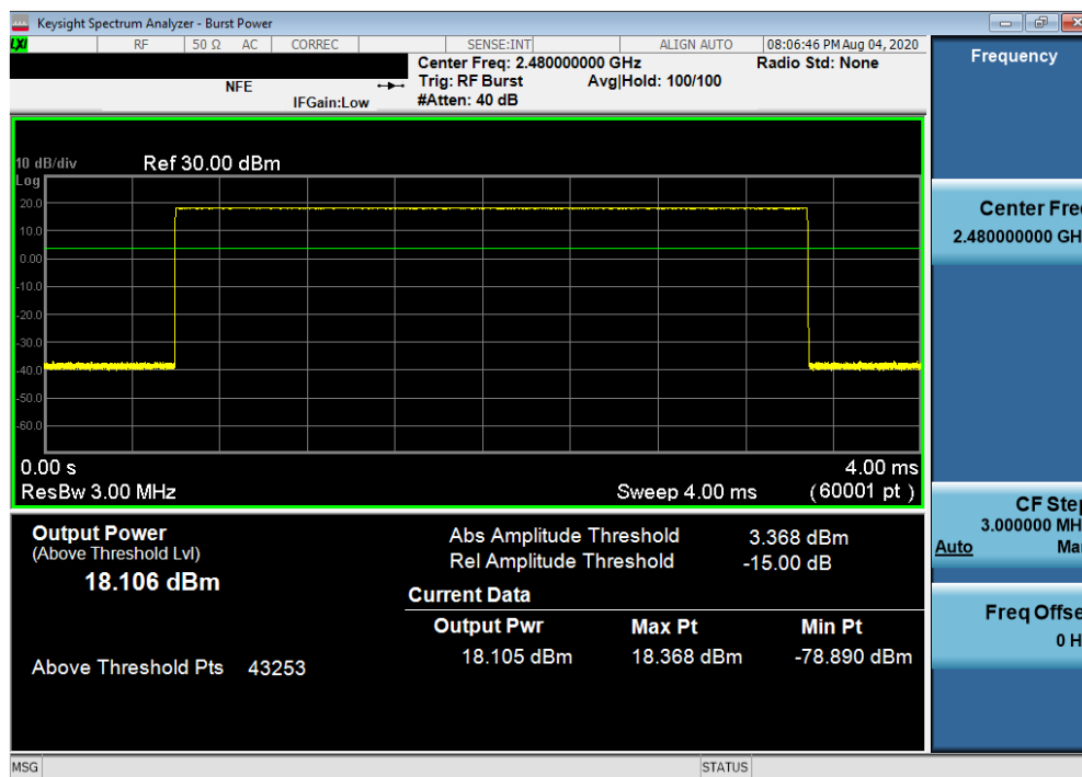
Plot 7-48. Average Conducted Power (1Mbps – Ch. 78)
