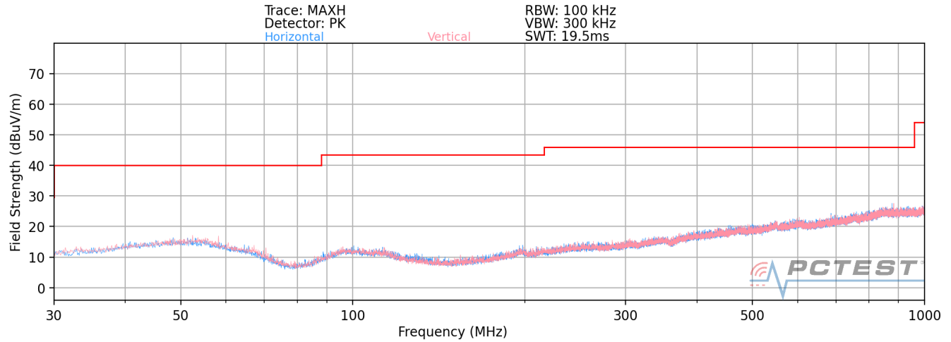
Plot 7-95. Radiated Spurious Plot below 1GHz
