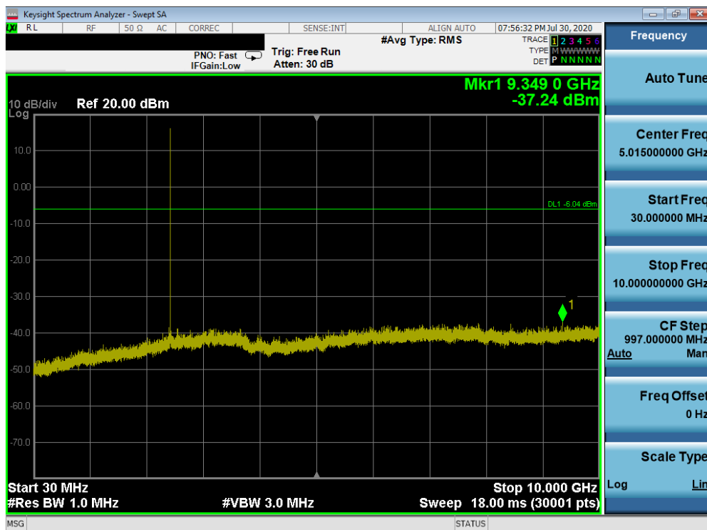
Plot 7-79. Conducted Spurious Plot (Bluetooth, 1Mbps – Ch. 39)
