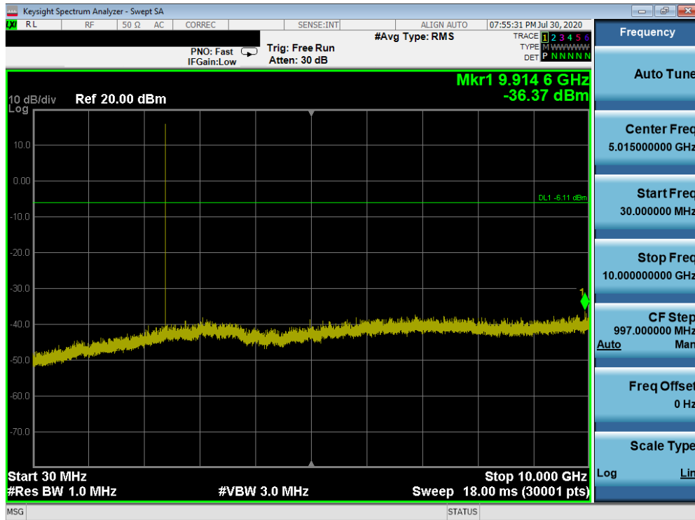
Plot 7-77. Conducted Spurious Plot (Bluetooth, 1Mbps - Ch. 0)
