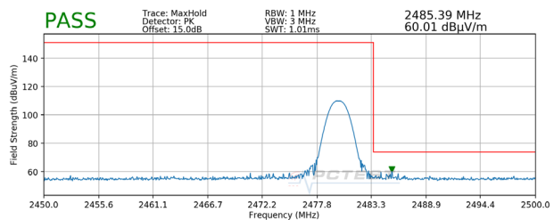
Plot 7-90. Radiated Restricted Upper Band Edge Measurement with WCP (Peak) – ANT1
