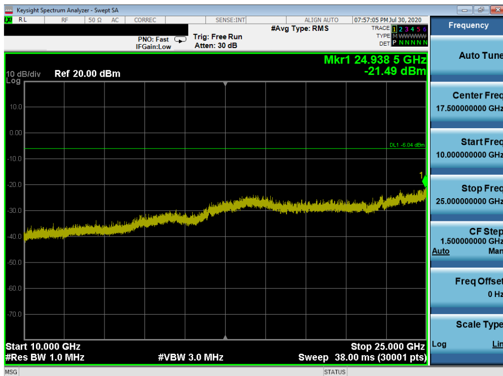
Plot 7-80. Conducted Spurious Plot (Bluetooth, 1Mbps – Ch. 39)
