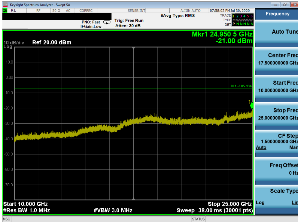
Plot 7-82. Conducted Spurious Plot (Bluetooth, 1Mbps – Ch. 78)
