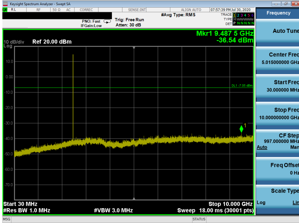
Plot 7-81. Conducted Spurious Plot (Bluetooth, 1Mbps – Ch. 78)
