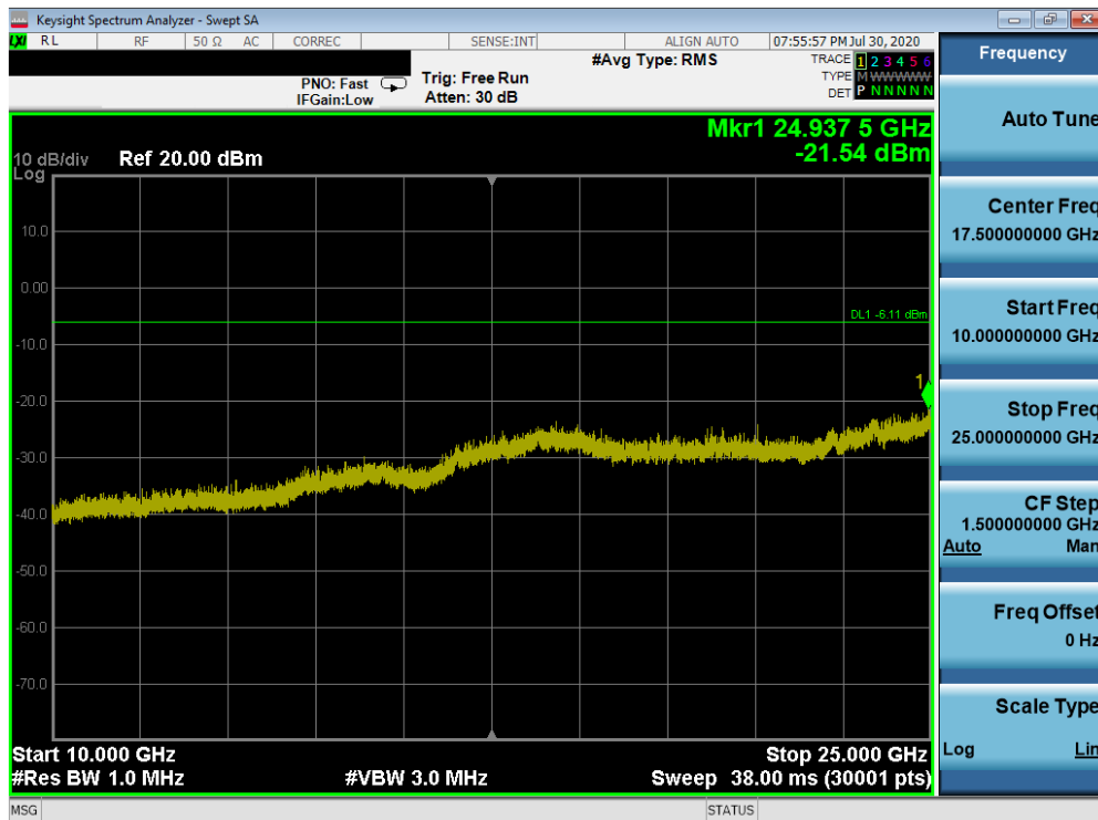
Plot 7-78. Conducted Spurious Plot (Bluetooth, 1Mbps - Ch. 0)
