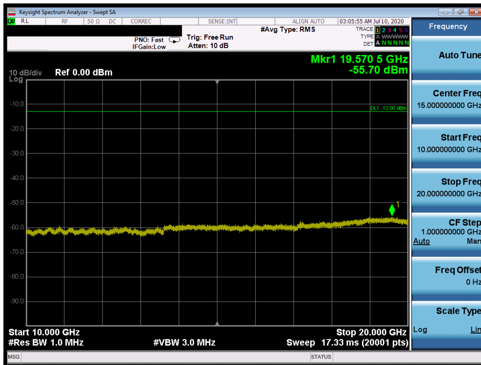
Plot 7-332. Conducted Spurious Plot (Band 25/2 - 20.0MHz QPSK - RB Size 1, RB Offset 0 - Low Channel)
