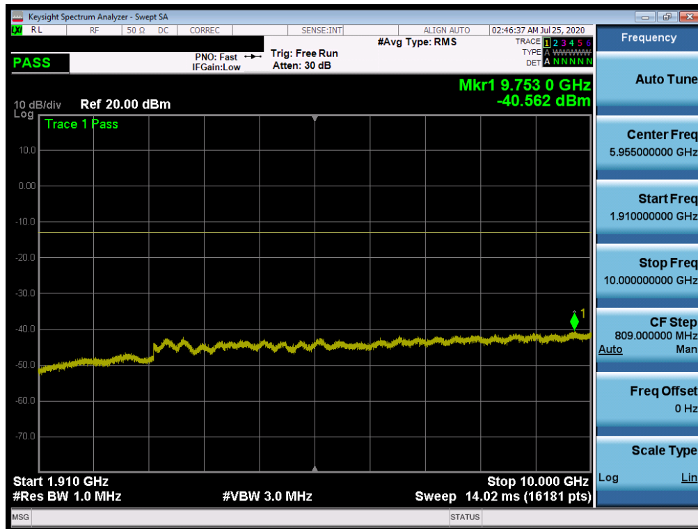
Plot 7-340. Conducted Spurious Plot (NR Band n25/2 - 20.0MHz - RB Size 1, RB Offset 0 - Low Channel)
