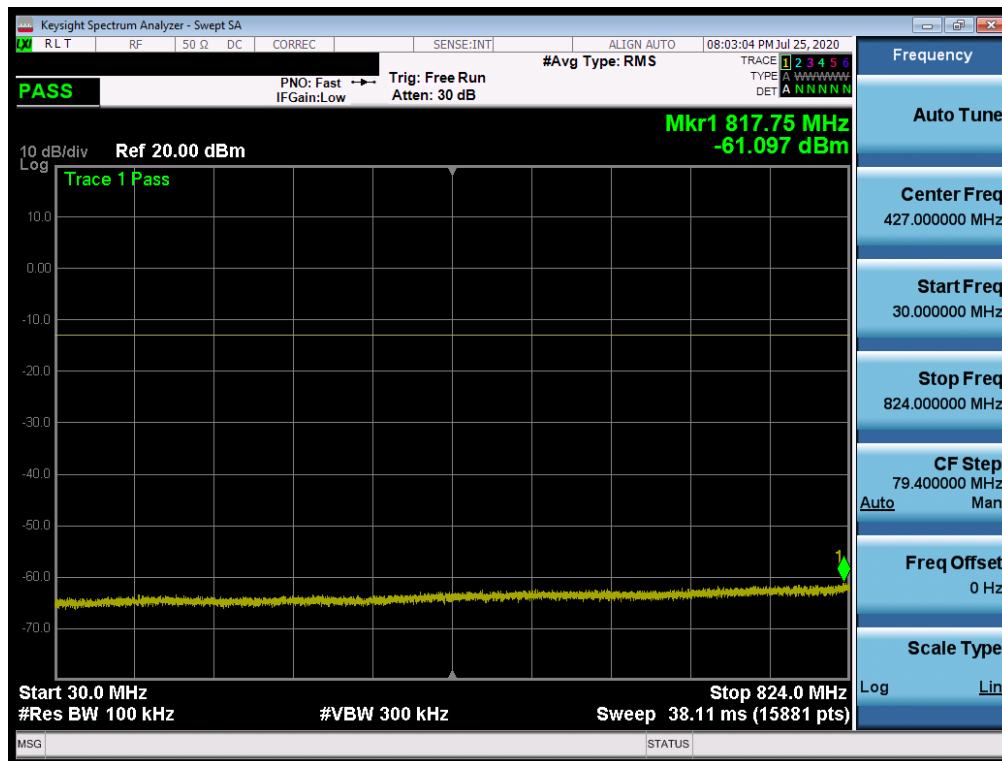
Plot 7-309. Conducted Spurious Plot (NR Band n5 - 20.0MHz - RB Size 1, RB Offset 0 - High Channel)
