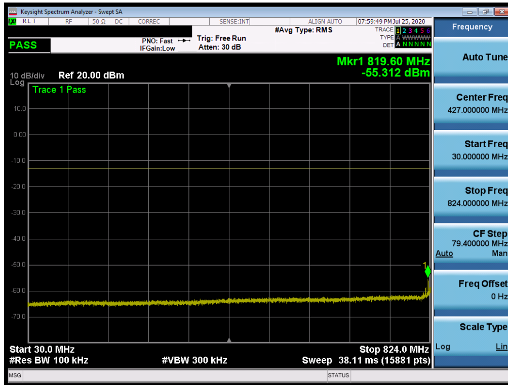
Plot 7-303. Conducted Spurious Plot (NR Band n5 - 20.0MHz - RB Size 1, RB Offset 0 - Low Channel)
