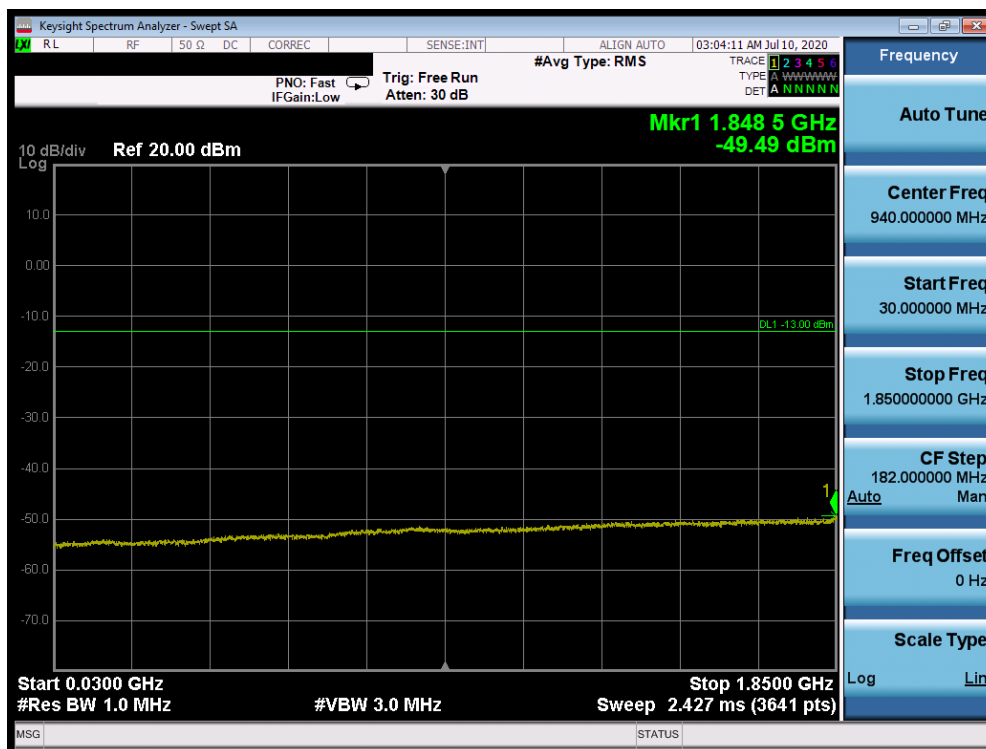
Plot 7-333. Conducted Spurious Plot (Band 25/2 - 20.0MHz QPSK - RB Size 1, RB Offset 0 - Mid Channel)
