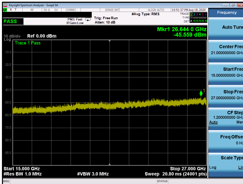
Plot 7-374. Conducted Spurious Plot (NR Band n41 - 100.0MHz - RB Size 1, RB Offset 0 - Mid Channel)
