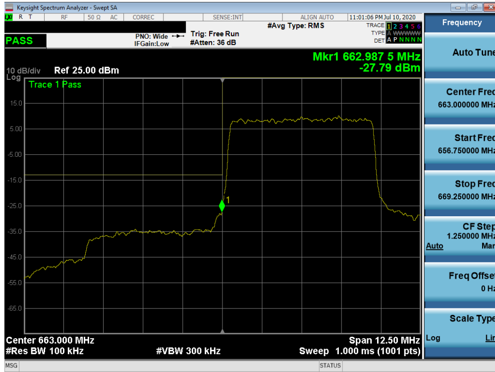
Plot 7-386. Lower Band Edge Plot (NR Band n71 – 5.0MHz - Full RB)
