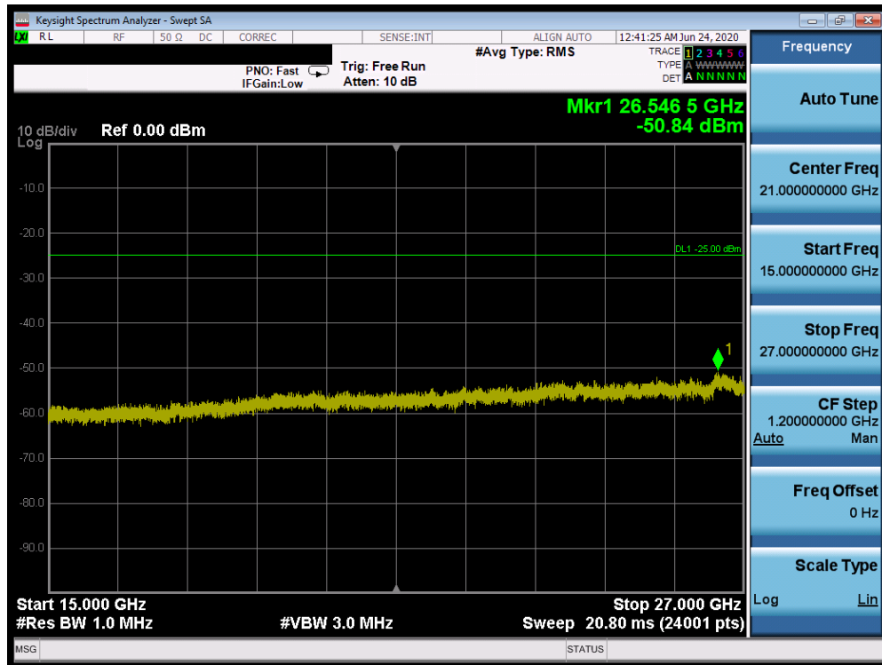
Plot 7-359. Conducted Spurious Plot (Band 7 - 20.0MHz QPSK - RB Size 1, RB Offset 0 - High Channel)
