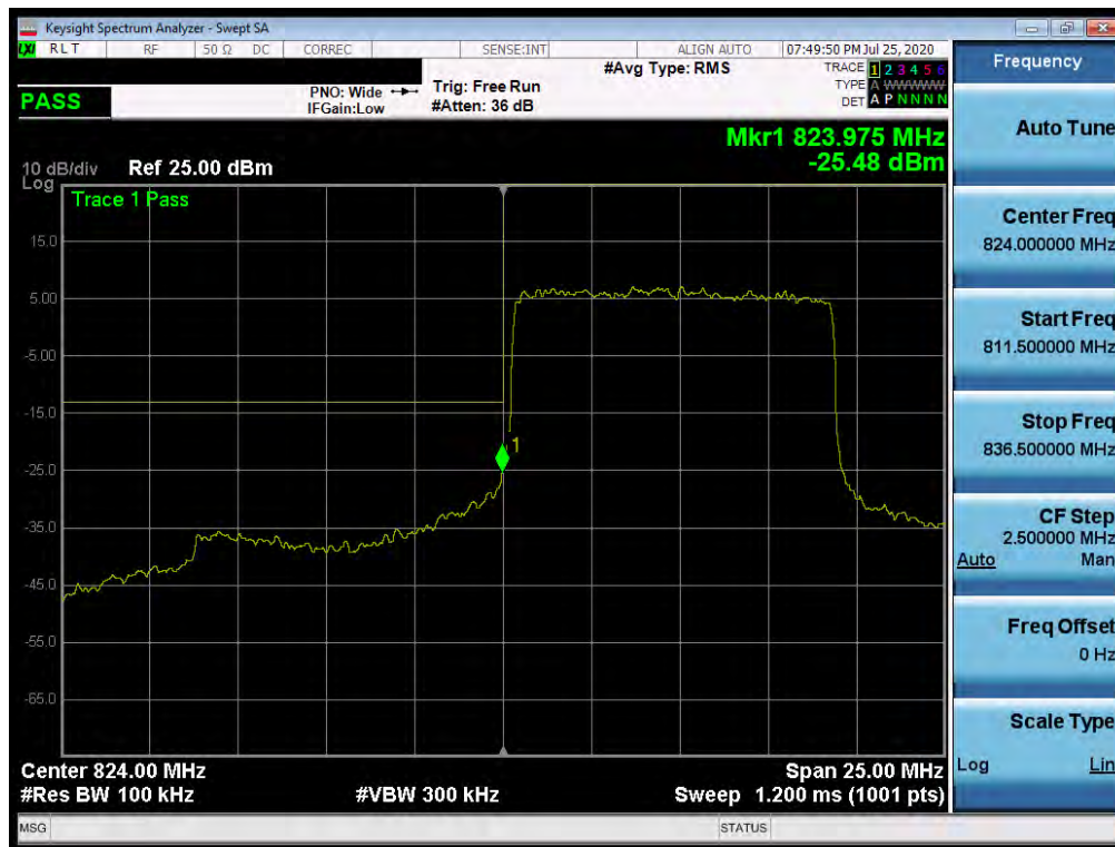
Plot 7-420. Lower Band Edge Plot (NR Band n5 - 10.0MHz - Full RB)
