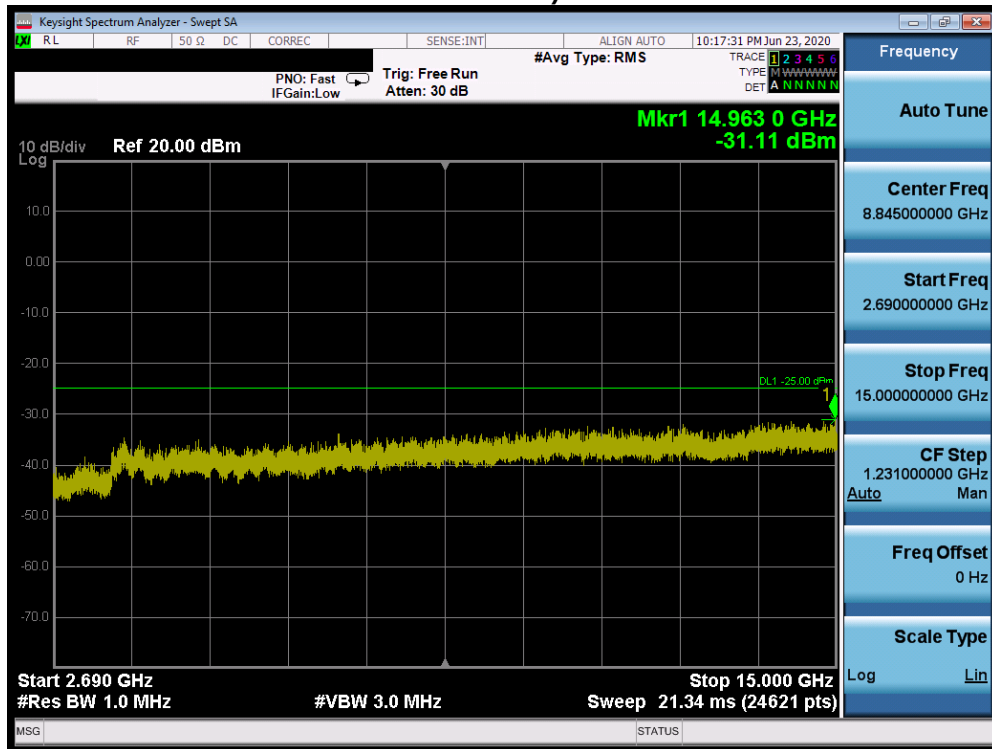
Plot 7-361. Conducted Spurious Plot (Band 41 PC2 - 20.0MHz QPSK - RB Size 1, RB Offset 0 - Low Channel)
