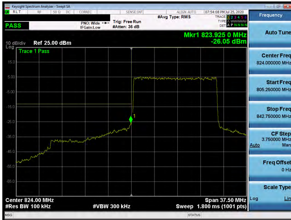
Plot 7-422. Lower Band Edge Plot (NR Band n5 - 15.0MHz - Full RB)
