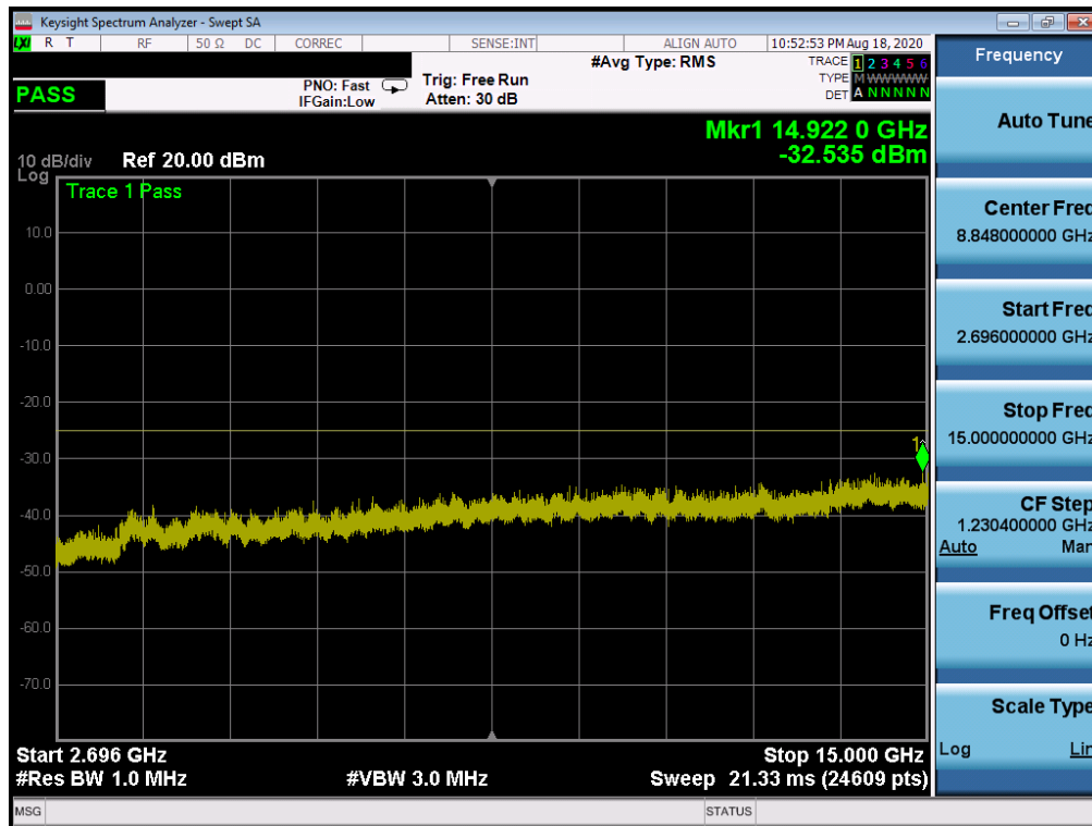
Plot 7-370. Conducted Spurious Plot (NR Band n41 - 100.0MHz - RB Size 1, RB Offset 0 - Low Channel)
