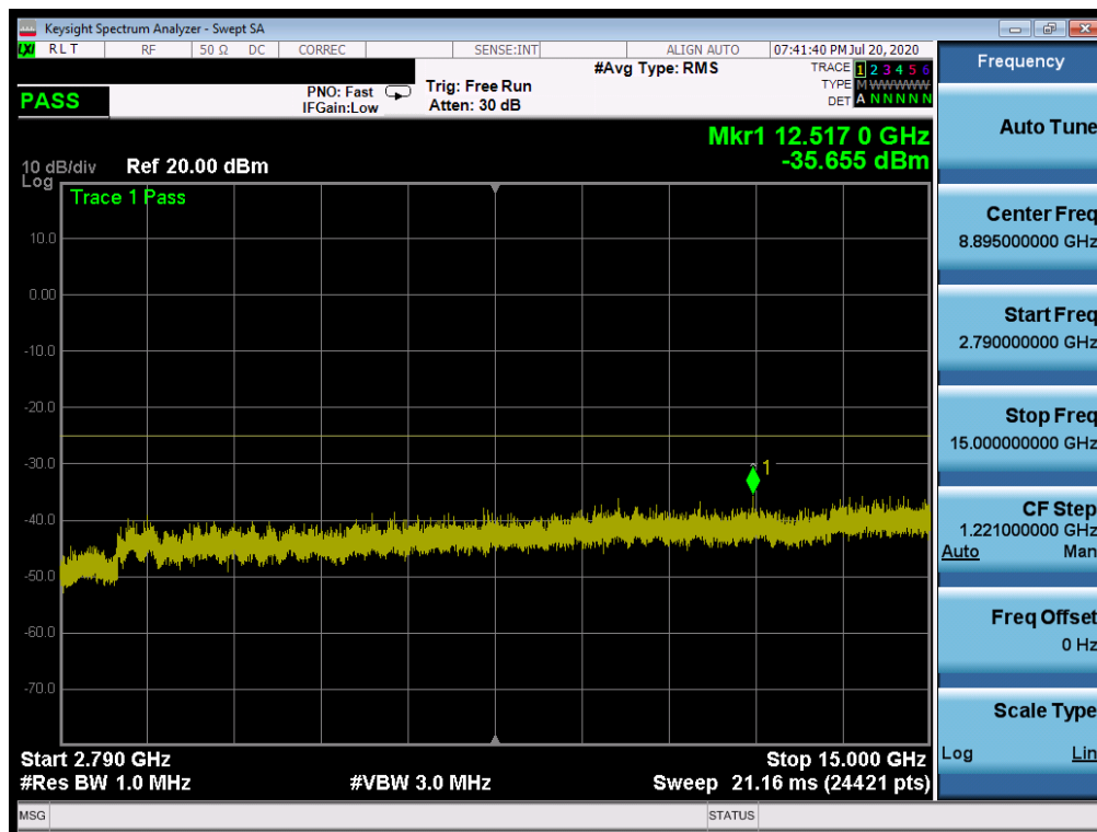
Plot 7-376. Conducted Spurious Plot (NR Band n41 - 100.0MHz - RB Size 1, RB Offset 0 - High Channel)
