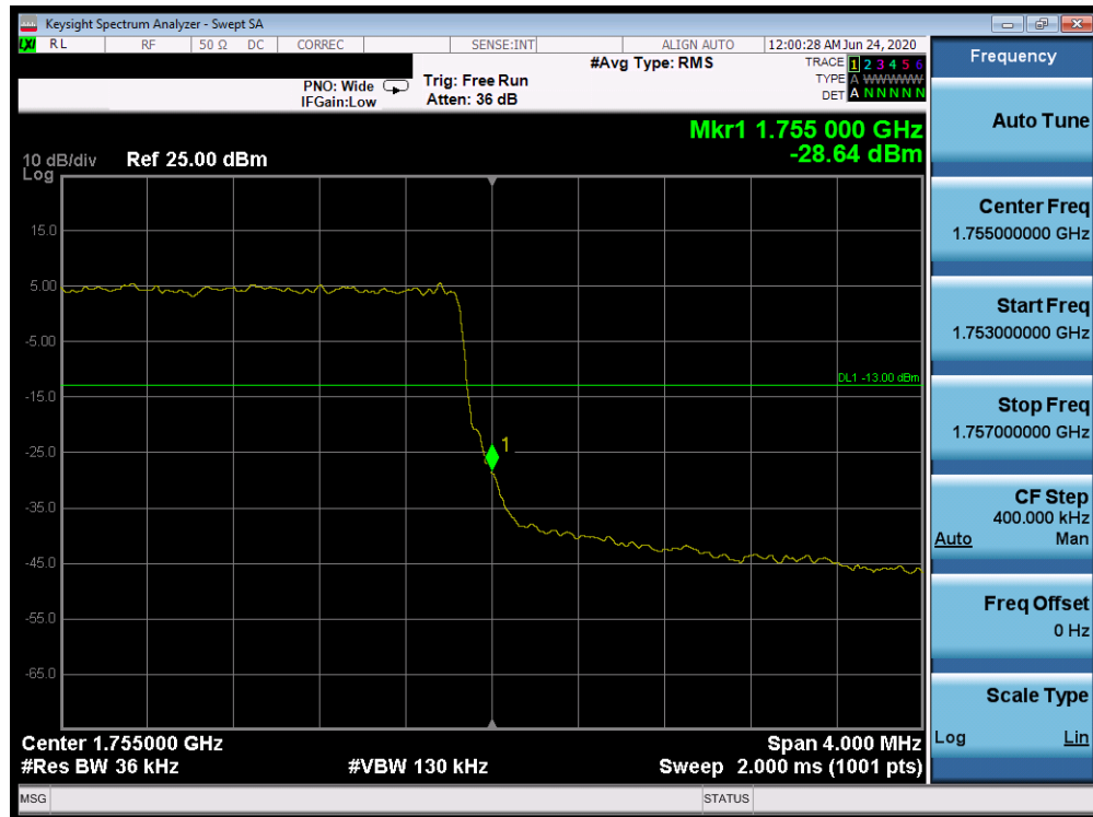
Plot 7-434. Upper Band Edge Plot (Band 4 - 3.0MHz QPSK - Full RB Configuration)
