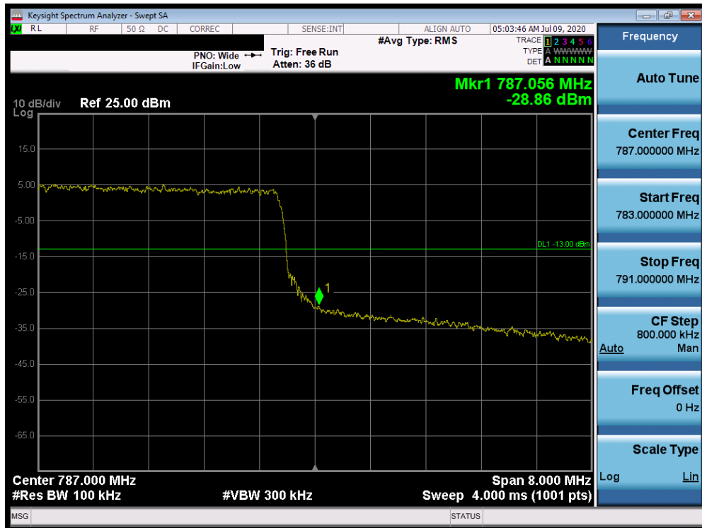
Plot 7-408. Upper Band Edge Plot (Band 13 - 10.0MHz QPSK - Full RB Configuration)
