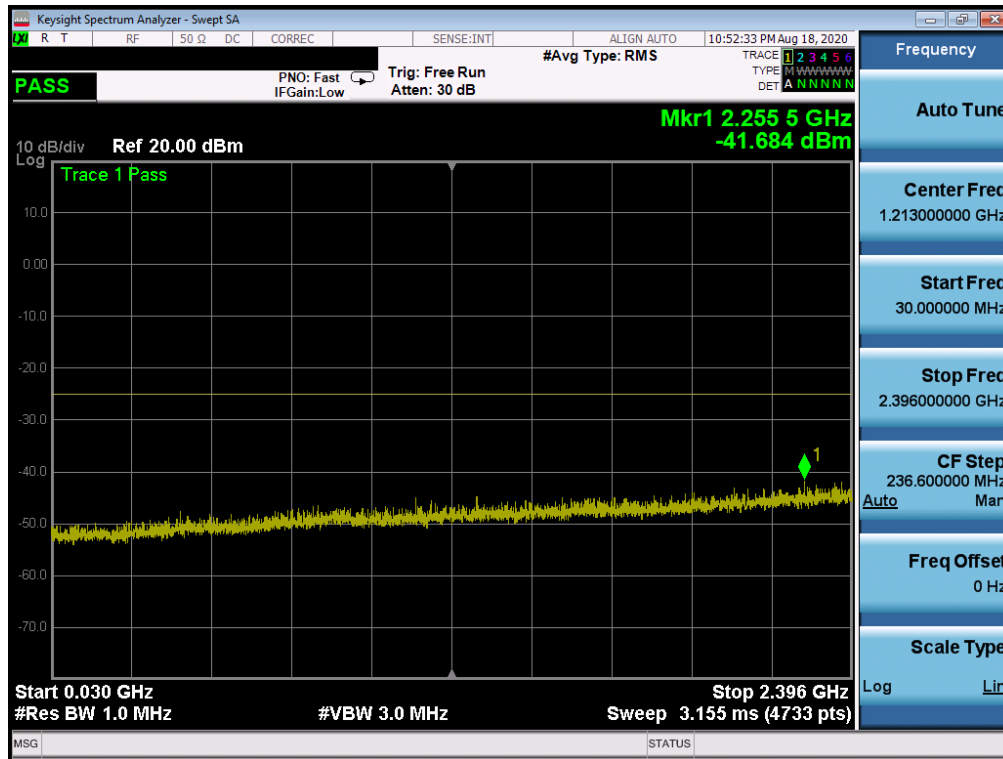
Plot 7-369. Conducted Spurious Plot (NR Band n41 -100.0MHz - RB Size 1, RB Offset 0 - Low Channel)
