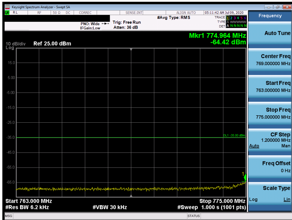
Plot 7-403. Lower Emission Mask Plot (Band 13 - 5.0MHz QPSK - Full RB Configuration)
