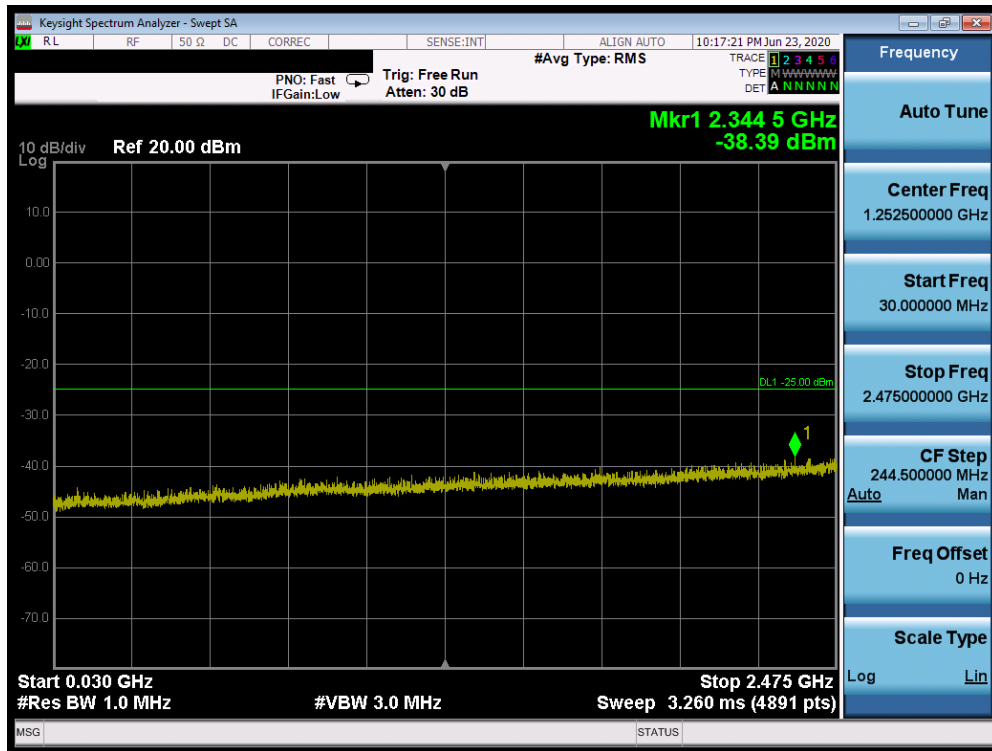
Plot 7-360. Conducted Spurious Plot (Band 41 PC2 - 20.0MHz QPSK - RB Size 1, RB Offset 0 - Low Channel)
