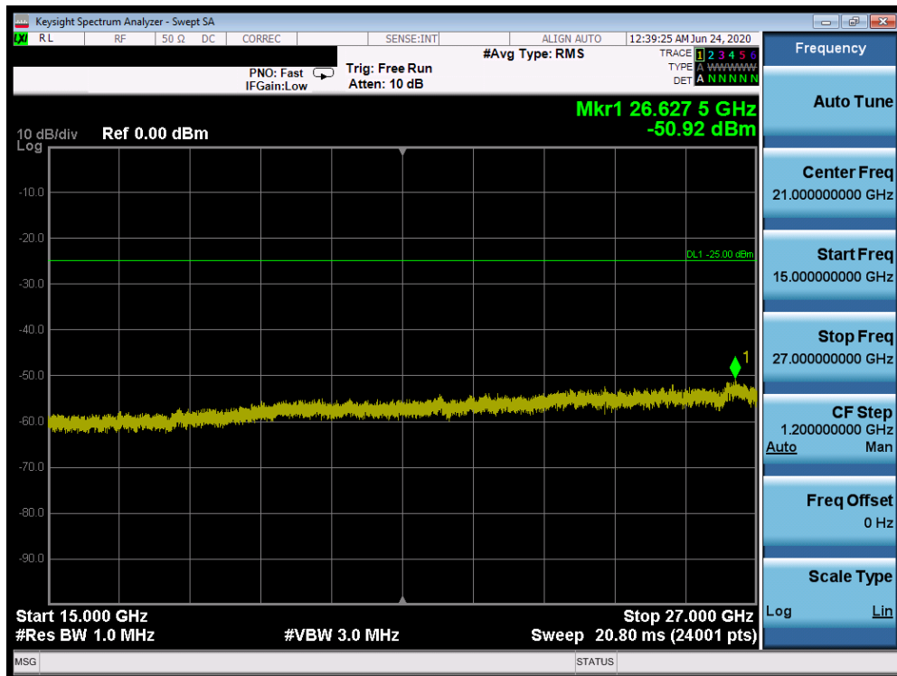
Plot 7-356. Conducted Spurious Plot (Band 7 - 20.0MHz QPSK - RB Size 1, RB Offset 0 - Mid Channel)
