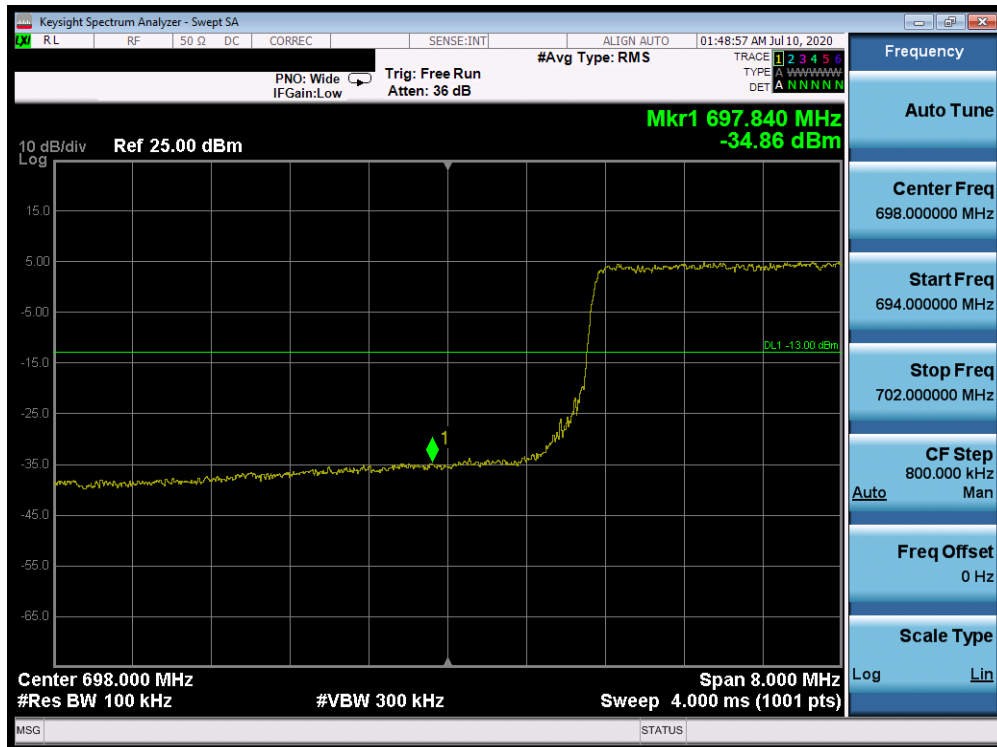
Plot 7-400. Lower Band Edge Plot (Band 12 - 10.0MHz QPSK - Full RB Configuration)
