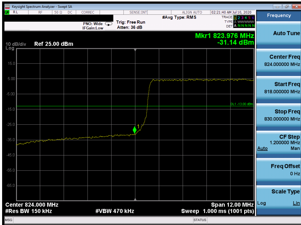
Plot 7-416. Lower Band Edge Plot (Band 26 - 15.0MHz QPSK - Full RB Configuration)
