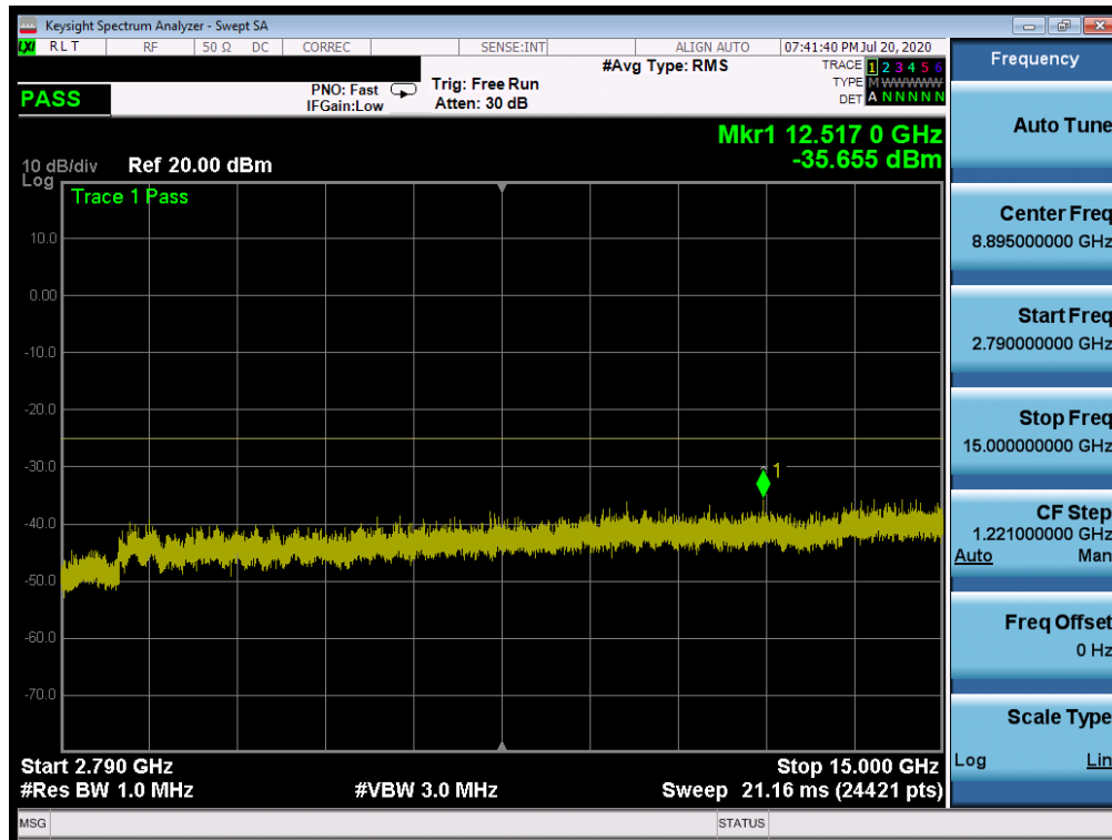
Plot 7-373. Conducted Spurious Plot (NR Band n41 - 100.0MHz - RB Size 1, RB Offset 0 - Mid Channel)
