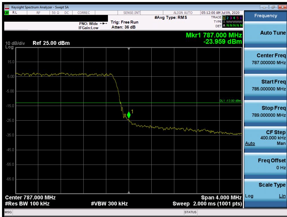
Plot 7-404. Upper Band Edge Plot (Band 13 - 5.0MHz QPSK - Full RB Configuration)
