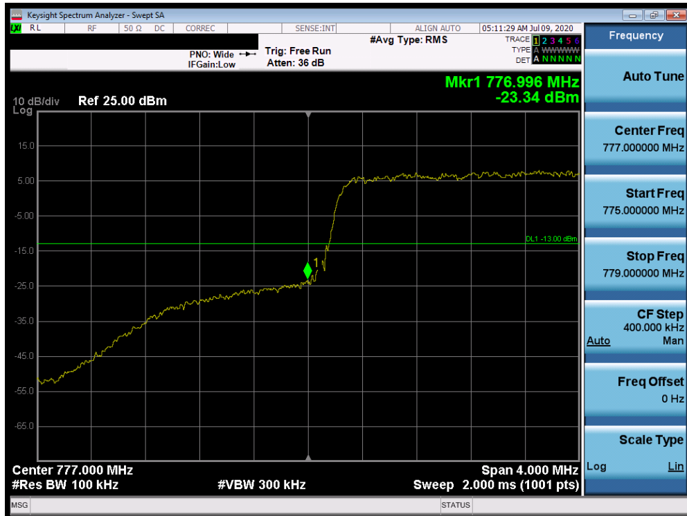
Plot 7-402. Lower Band Edge Plot (Band 13 - 5.0MHz QPSK - Full RB Configuration)
