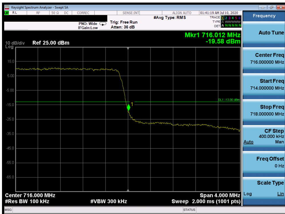
Plot 7-397. Upper Band Edge Plot (Band 12 - 3.0MHz QPSK - Full RB Configuration)
