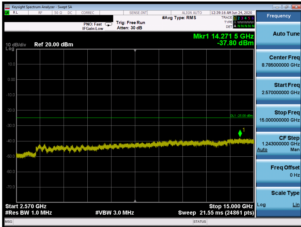
Plot 7-355. Conducted Spurious Plot (Band 7 - 20.0MHz QPSK - RB Size 1, RB Offset 0 - Mid Channel)
