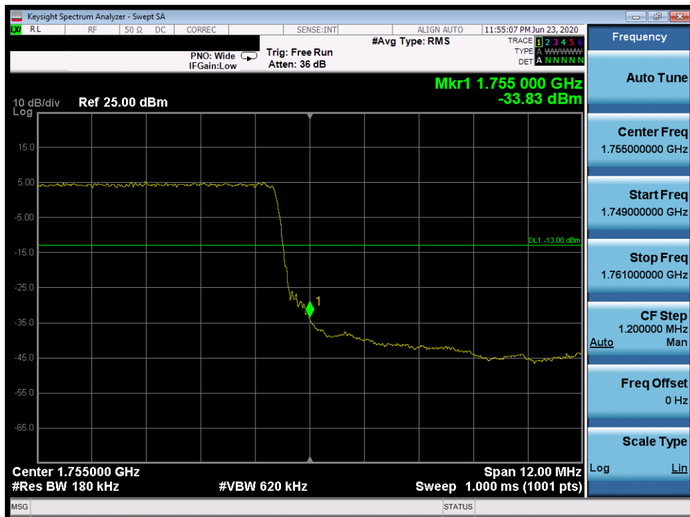
Plot 7-452. Upper Band Edge Plot (Band 4 - 15.0MHz QPSK - Full RB Configuration)
