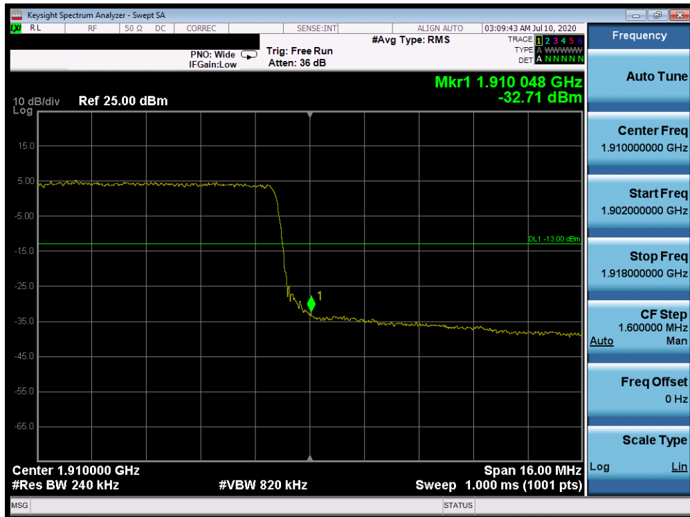
Plot 7-510. Upper Band Edge Plot (Band 2 - 20.0MHz QPSK - Full RB Configuration)
