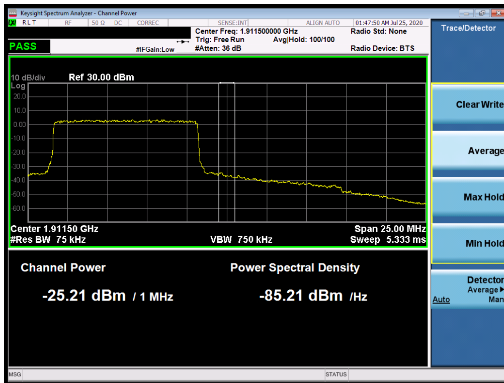
Plot 7-523. Upper Extended Band Edge Plot (NR Band n2 – 10.0MHz - Full RB)
