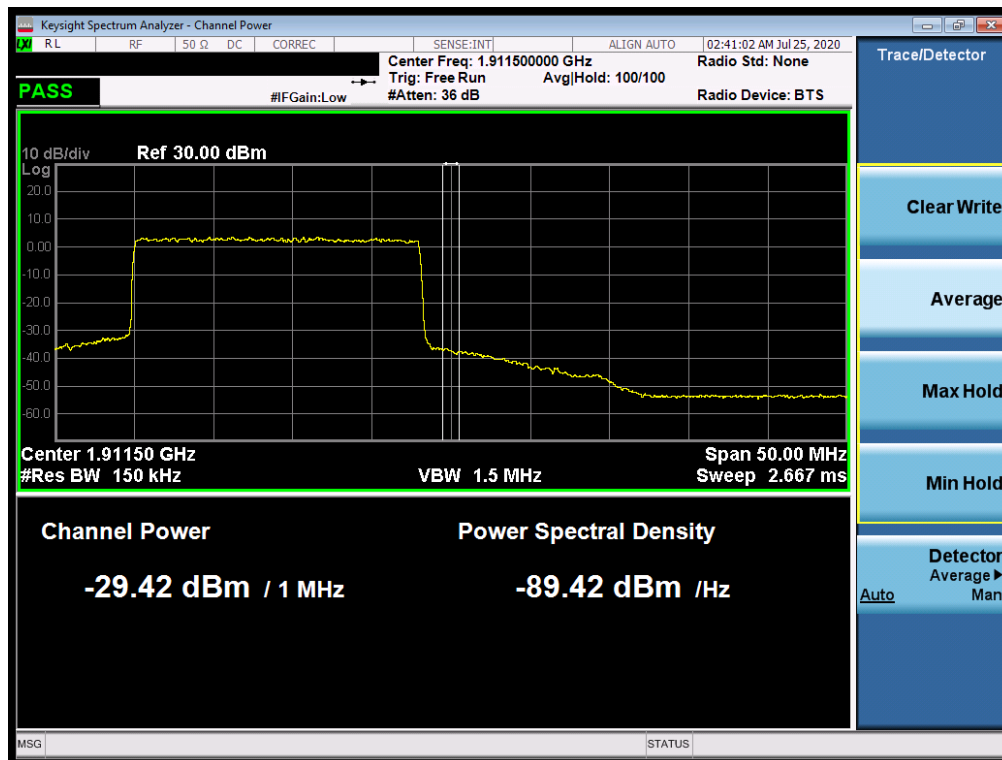
Plot 7-535. Upper Extended Band Edge Plot (NR Band n2 – 20.0MHz - Full RB)
