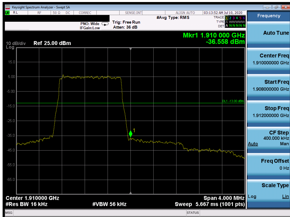
Plot 7-480. Upper Band Edge Plot (Band 2 - 1.4MHz QPSK - Full RB Configuration)
