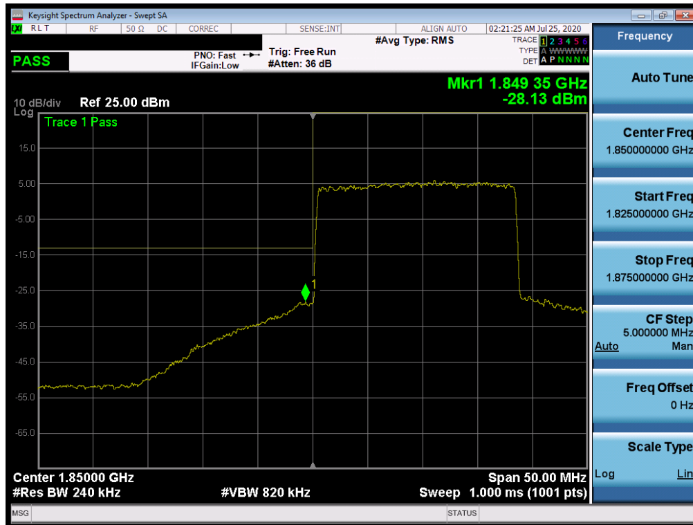
Plot 7-532. Lower Band Edge Plot (NR Band n25/2 – 20.0MHz - Full RB)
