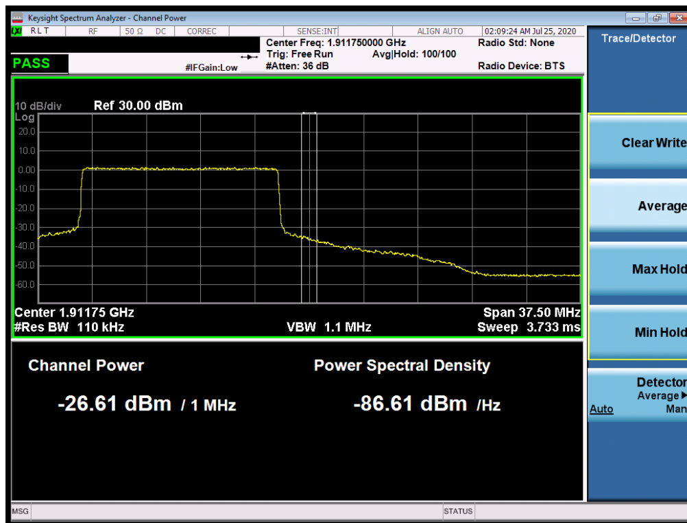
Plot 7-529. Upper Extended Band Edge Plot (NR Band n2 – 15.0MHz - Full RB)
