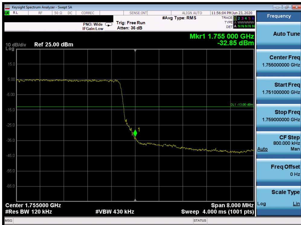
Plot 7-446. Upper Band Edge Plot (Band 4 - 10.0MHz QPSK - Full RB Configuration)
