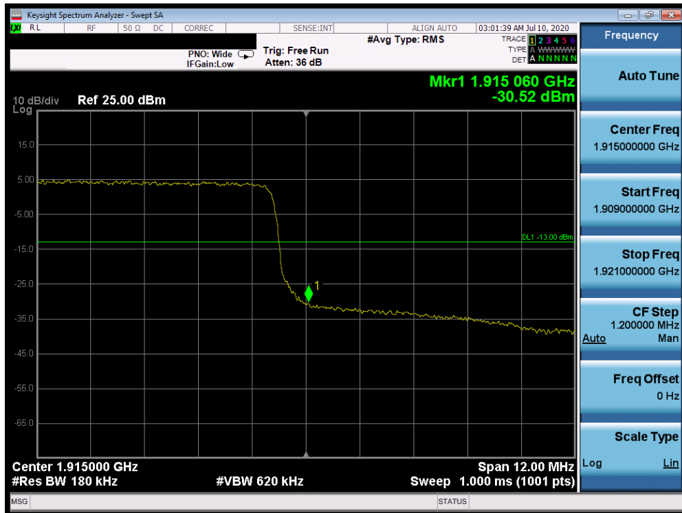
Plot 7-506. Upper Band Edge Plot (Band 25 - 15.0MHz QPSK - Full RB Configuration)
