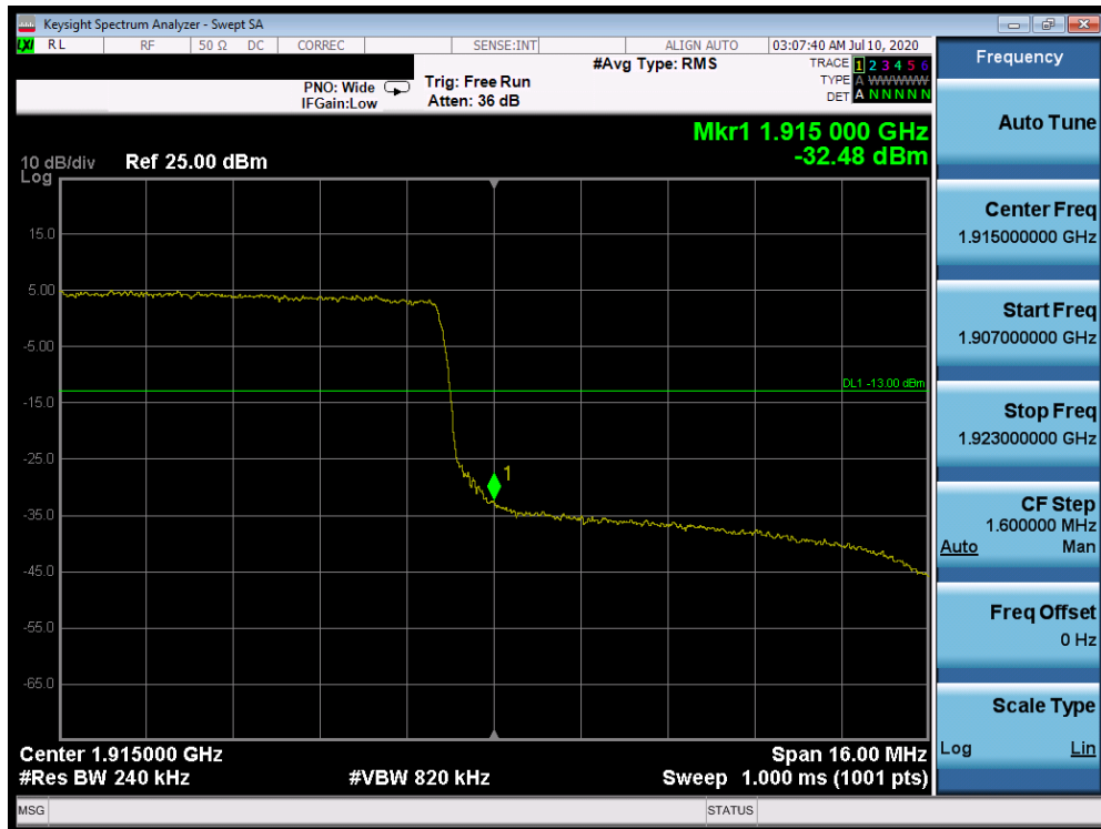
Plot 7-512. Upper Band Edge Plot (Band 25 - 20.0MHz QPSK - Full RB Configuration)
