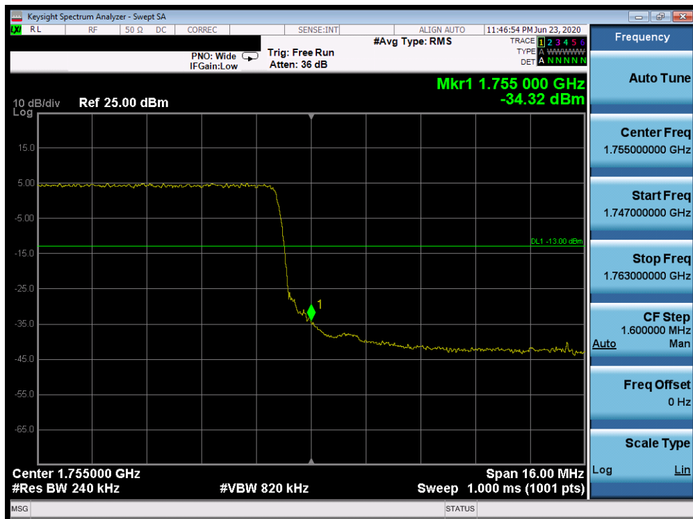
Plot 7-458. Upper Band Edge Plot (Band 4 - 20.0MHz QPSK - Full RB Configuration)
