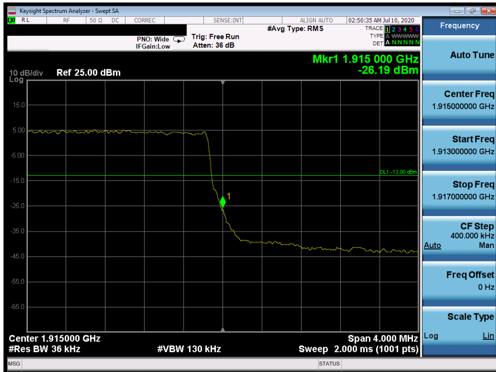
Plot 7-488. Upper Band Edge Plot (Band 25 - 3.0MHz QPSK - Full RB Configuration)
