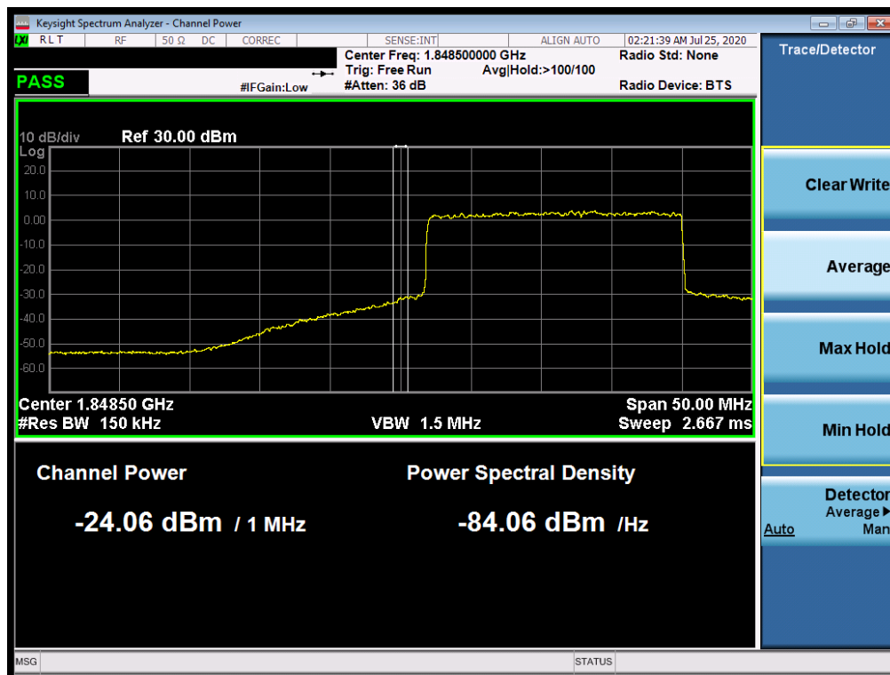
Plot 7-533. Lower Extended Band Edge Plot (NR Band n25/2 – 20.0MHz - Full RB)
