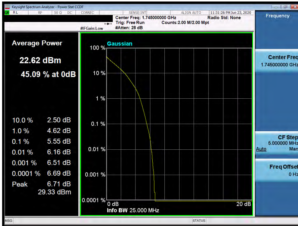
Plot 7-644. PAR Plot (Band 66/4 - 15.0MHz QPSK - Full RB Configuration)
