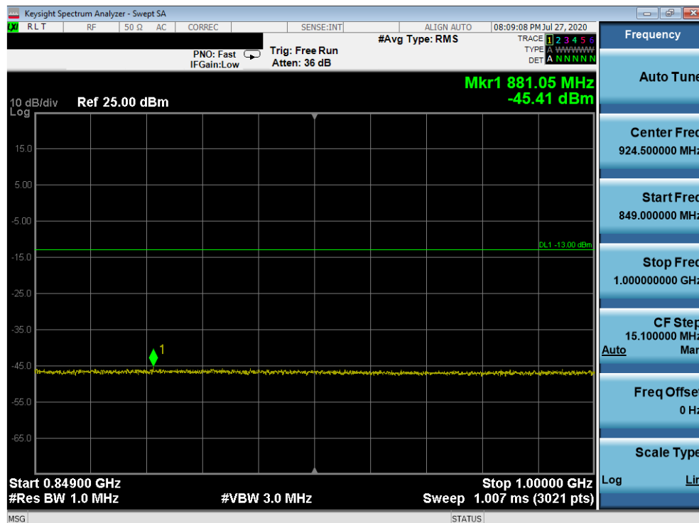
Plot 7-674. Conducted Spurious Plot (Band 5 – 10.0MHz QPSK – PCC 1/49 SCC 1/0 – Low Channel)
