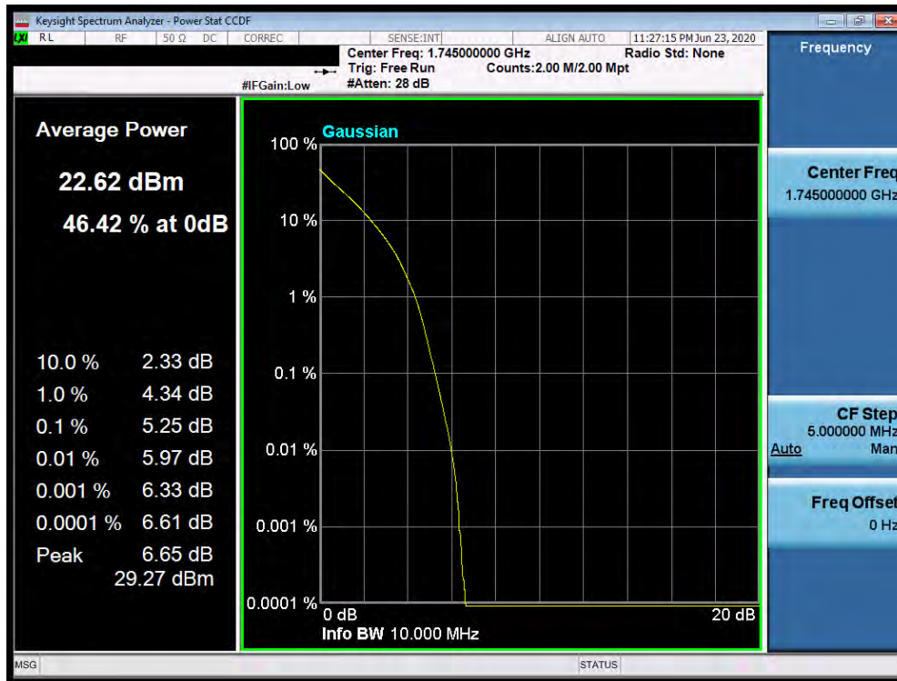
Plot 7-640. PAR Plot (Band 66/4 - 10.0MHz QPSK - Full RB Configuration)
