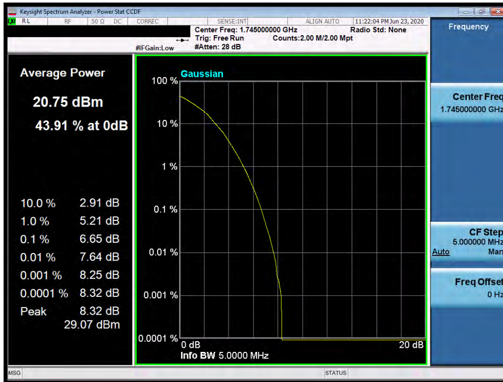
Plot 7-638. PAR Plot (Band 66/4 - 5.0MHz 64-QAM - Full RB Configuration)
