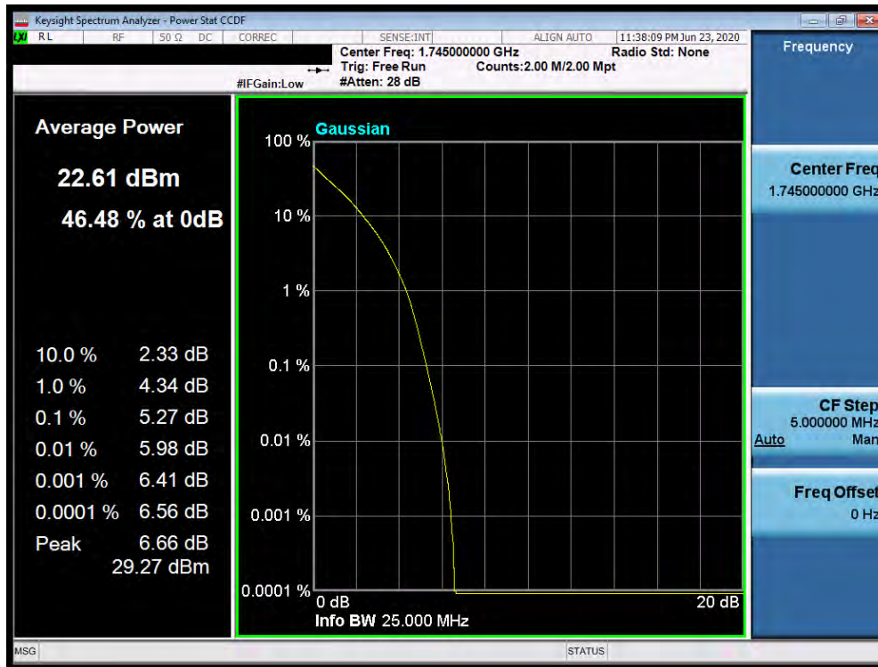
Plot 7-648. PAR Plot (Band 66/4 - 20.0MHz QPSK - Full RB Configuration)
