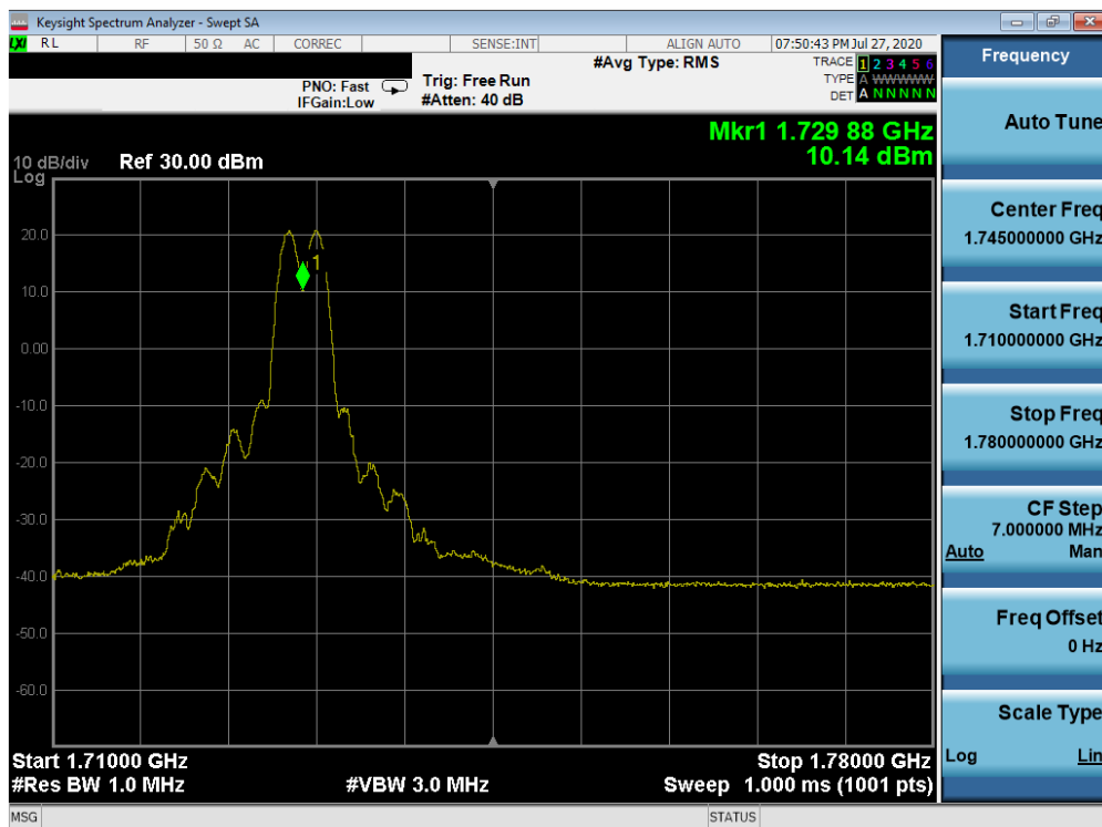
Plot 7-683. Conducted Spurious Plot (Band 66 – 20.0MHz QPSK – PCC 1/99 SCC 1/0 – Low Channel)
