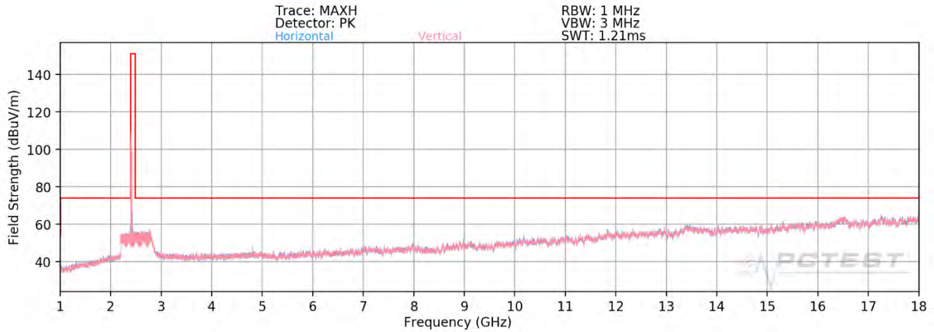
Plot 7-57. Radiated Spurious Plot above 1GHz SISO ANT1 (802.11ax OFDMA – 26 Tones – Ch. 1)
