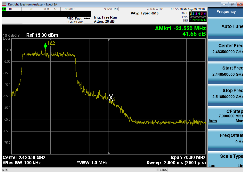
Plot 7-32. Band Edge Plot SISO ANT2 (802.11ax OFDMA – 242 Tones – Ch. 11)
