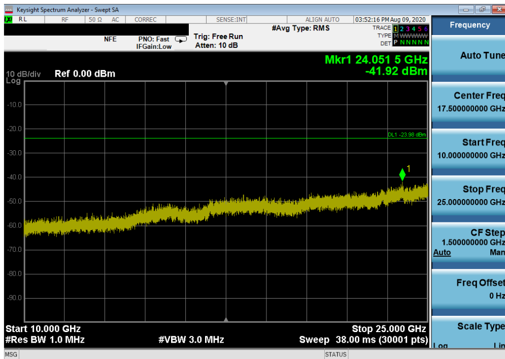
Plot 7-52. Conducted Spurious Plot SISO ANT2 (802.11ax OFDMA – 242 Tones – Ch. 1)
