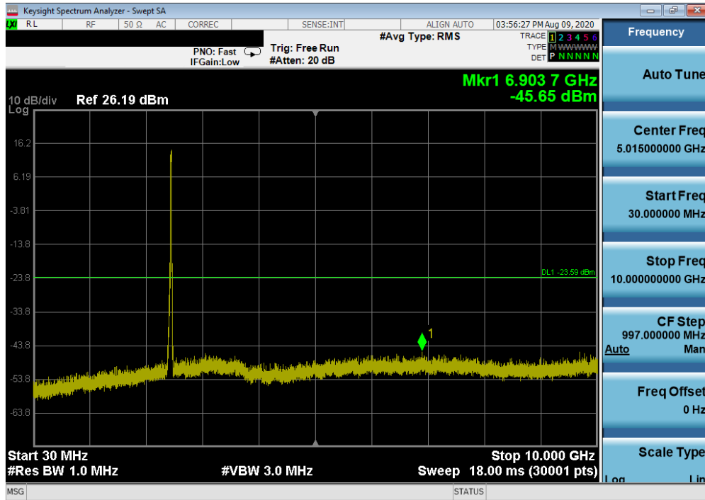
Plot 7-55. Conducted Spurious Plot SISO ANT2 (802.11ax OFDMA – 242 Tones – Ch. 11)
