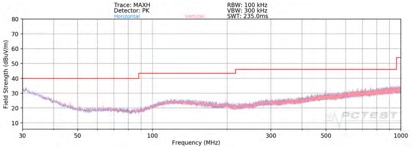
Plot 7-105. Radiated Spurious Plot below 1GHz MIMO (26 Tones)
