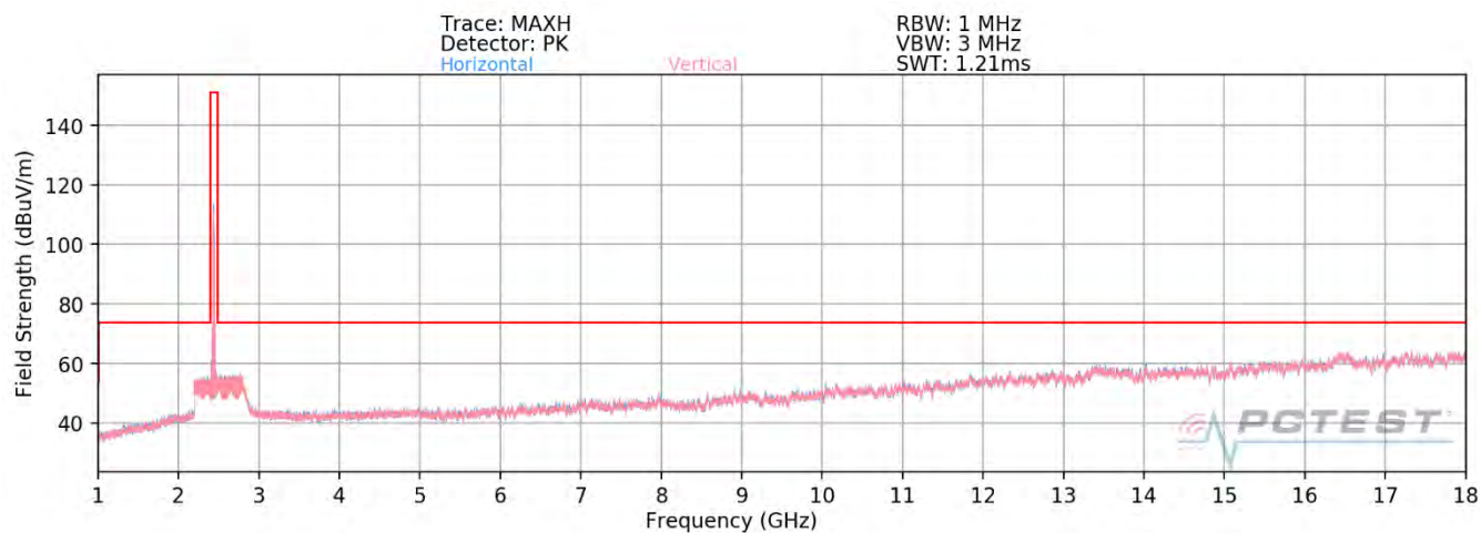
Plot 7-74. Radiated Spurious Plot above 1GHz MIMO (802.11ax OFDMA – 26 Tones – Ch. 6)
