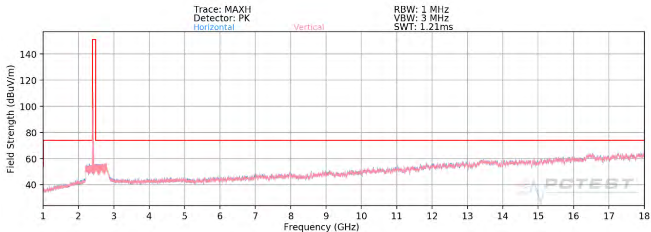
Plot 7-73. Radiated Spurious Plot above 1GHz MIMO (802.11ax OFDMA – 26 Tones – Ch. 1)
