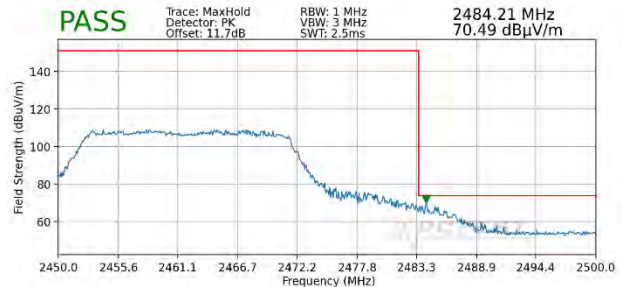
Plot 7-96. Radiated Restricted Upper Band Edge Measurement SISO ANT2 (Peak – 242 Tones)
