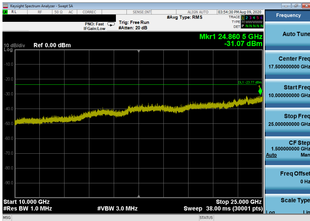
Plot 7-54. Conducted Spurious Plot SISO ANT2 (802.11ax OFDMA – 242 Tones – Ch. 6)
