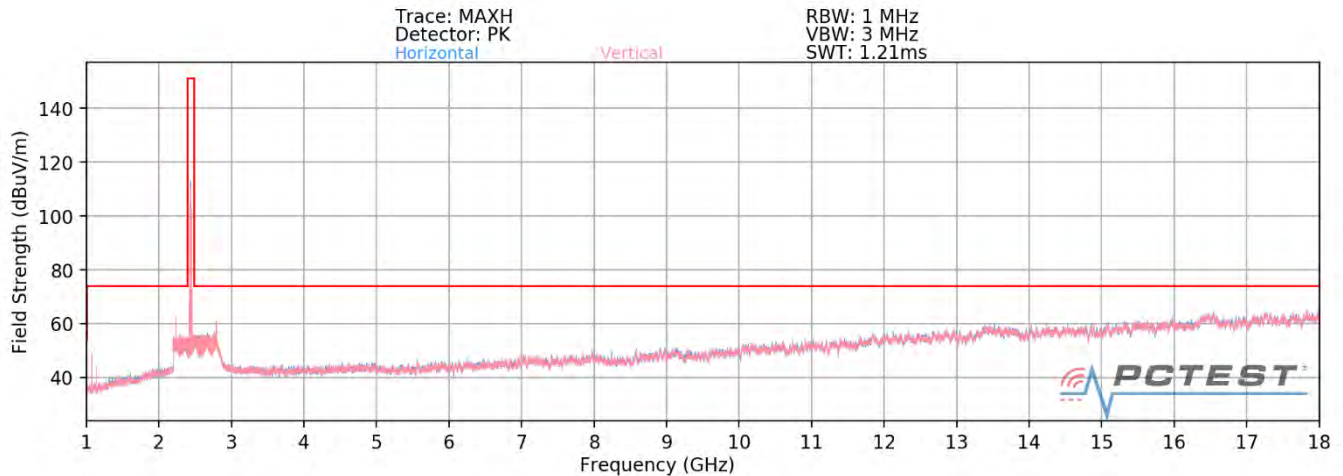
Plot 7-66. Radiated Spurious Plot above 1GHz SISO ANT2 (802.11ax OFDMA – 26 Tones – Ch. 6)
