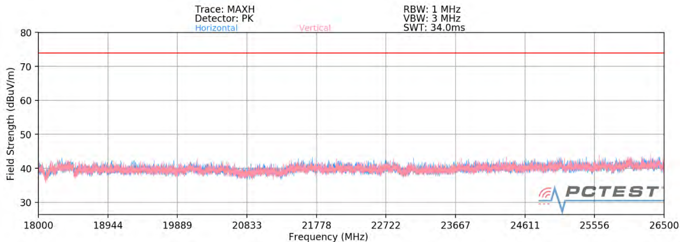
Plot 7-71. Radiated Spurious Plot above 18GHz SISO ANT2 (802.11ax OFDMA – 26 Tones)
