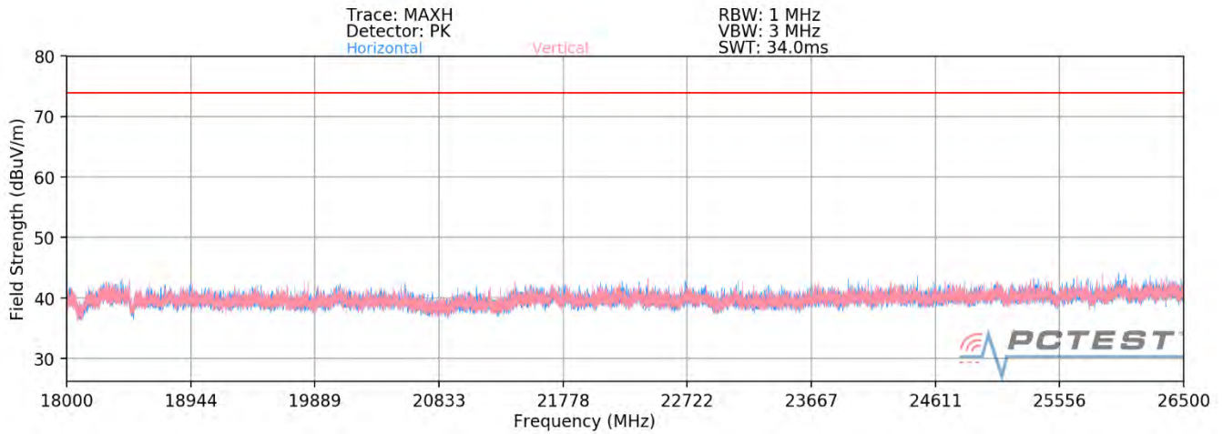
Plot 7-63. Radiated Spurious Plot above 18GHz SISO ANT1 (802.11ax OFDMA – 26 Tones)
