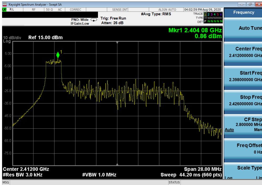
Plot 7-19. Power Spectral Density Plot SISO ANT2 (802.11ax OFDMA – 26 Tones – Ch. 1)
