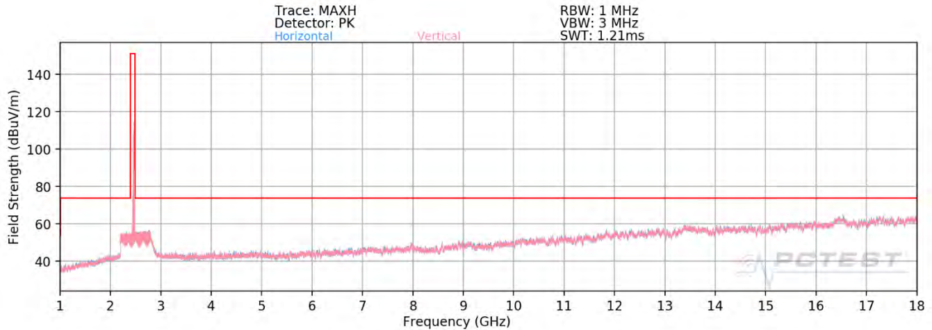
Plot 7-75. Radiated Spurious Plot above 1GHz MIMO (802.11ax OFDMA – 26 Tones – Ch. 11)
