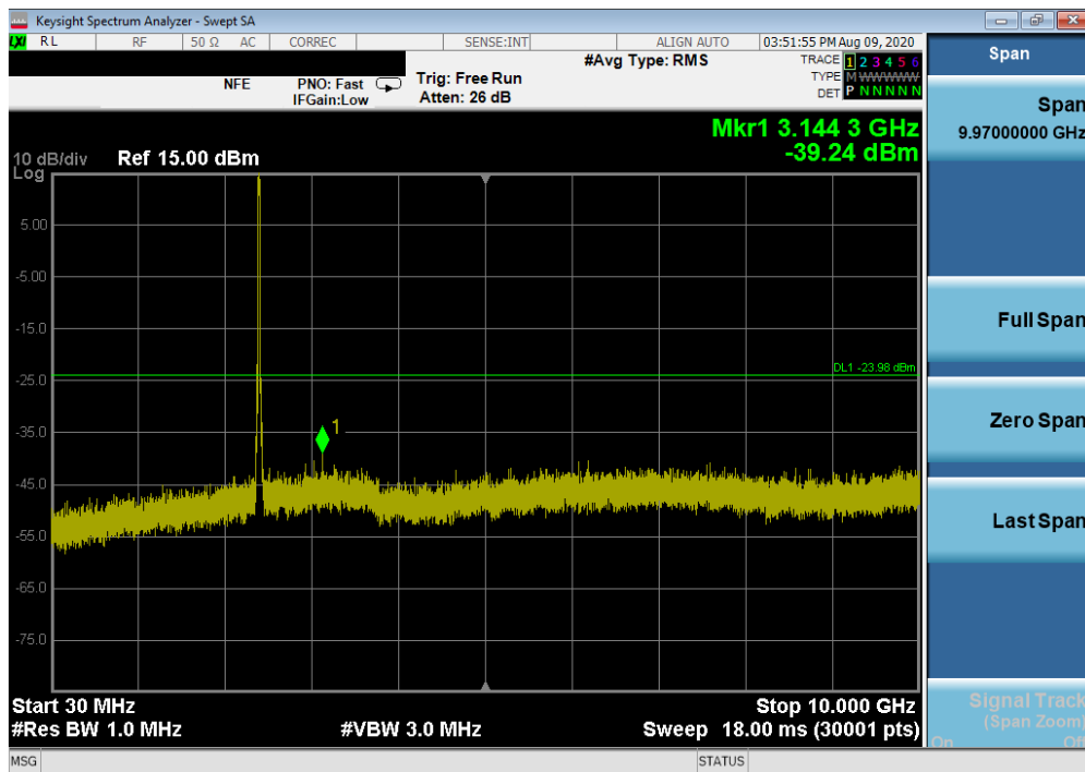
Plot 7-51. Conducted Spurious Plot SISO ANT2 (802.11ax OFDMA – 242 Tones – Ch. 1)
