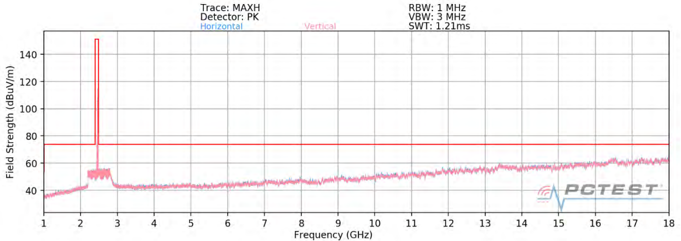
Plot 7-59. Radiated Spurious Plot above 1GHz SISO ANT1 (802.11ax OFDMA – 26 Tones – Ch. 11)
