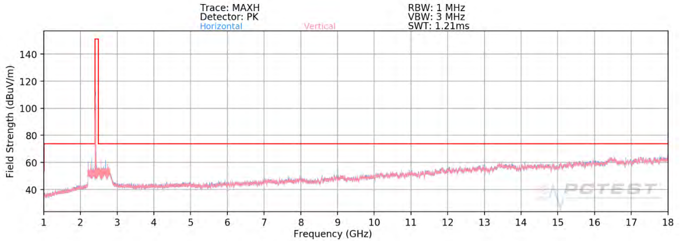
Plot 7-65. Radiated Spurious Plot above 1GHz SISO ANT2 (802.11ax OFDMA – 26 Tones – Ch. 1)
