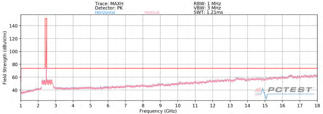
Plot 7-67. Radiated Spurious Plot above 1GHz SISO ANT2 (802.11ax OFDMA – 26 Tones – Ch. 11)
