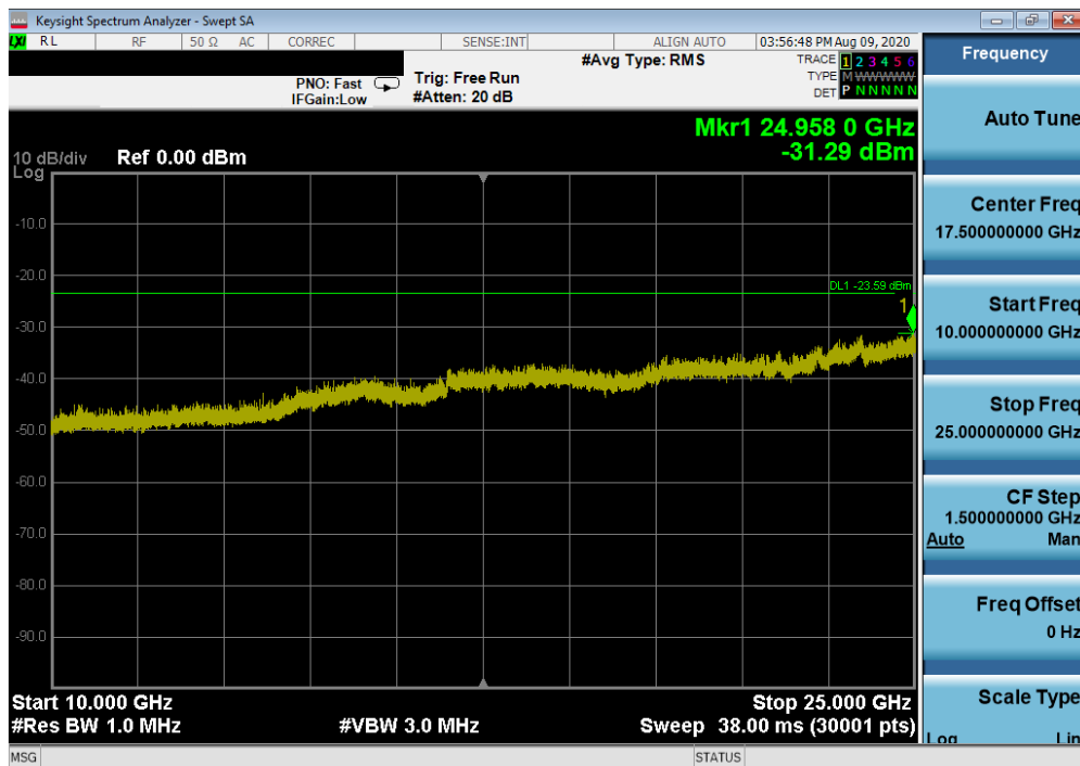
Plot 7-56. Conducted Spurious Plot SISO ANT2 (802.11ax OFDMA – 242 Tones – Ch. 11)
