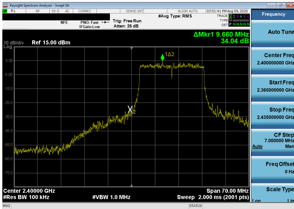
Plot 7-31. Band Edge Plot SISO ANT2 (802.11ax OFDMA – 242 Tones – Ch. 1)
