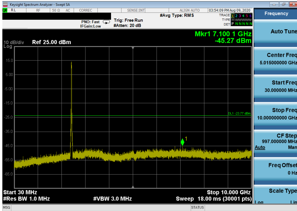
Plot 7-53. Conducted Spurious Plot SISO ANT2 (802.11ax OFDMA – 242 Tones – Ch. 6)
