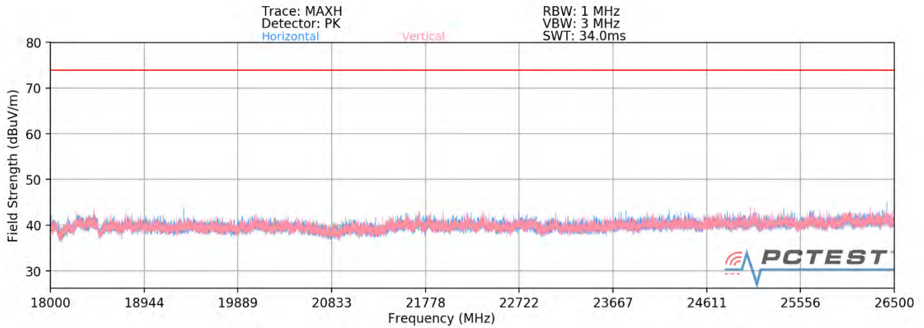
Plot 7-79. Radiated Spurious Plot above 18GHz MIMO (802.11ax OFDMA – 26 Tones)
