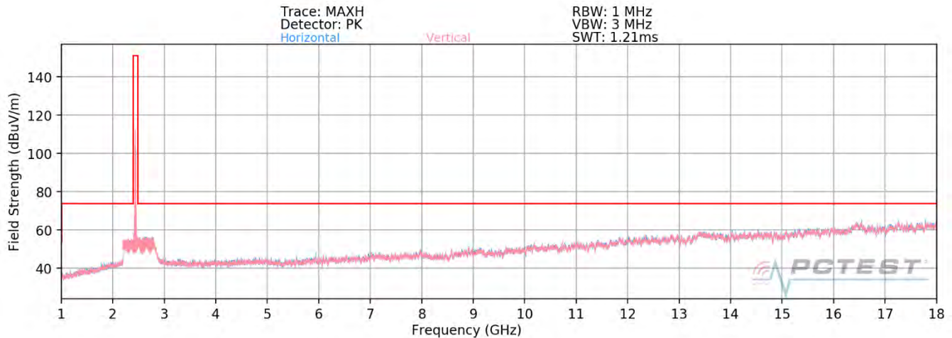
Plot 7-58. Radiated Spurious Plot above 1GHz SISO ANT1 (802.11ax OFDMA – 26 Tones – Ch. 6)
