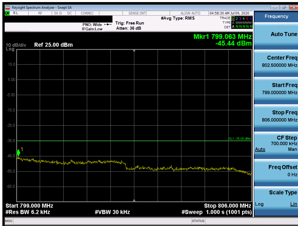
Plot 7-56. Upper Emission Mask Plot (LTE Band 14, 5MHz QPSK - RB Size 25)
