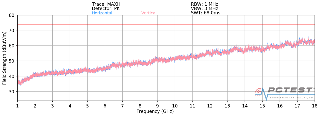
Plot 7-10. Radiated Spurious Plot above 1GHz [Radiated Test Config. 5]
