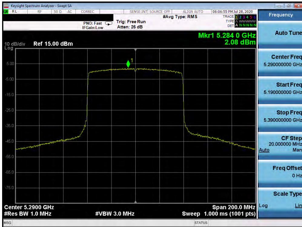
Plot 7-165. Power Spectral Density Plot SISO ANT1 (80MHz BW 802.11ax (UNII Band 2A) – Ch. 58)
