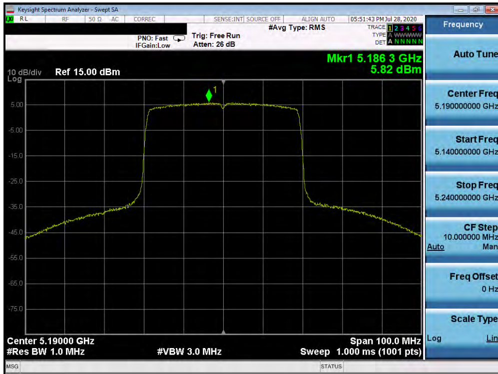
Plot 7-147. Power Spectral Density Plot SISO ANT1 (40MHz BW 802.11ax (UNII Band 1) – Ch. 38)
