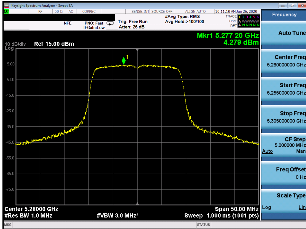
Plot 7-155. Power Spectral Density Plot SISO ANT1 (20MHz BW 802.11n (UNII Band 2A) – Ch. 56)
