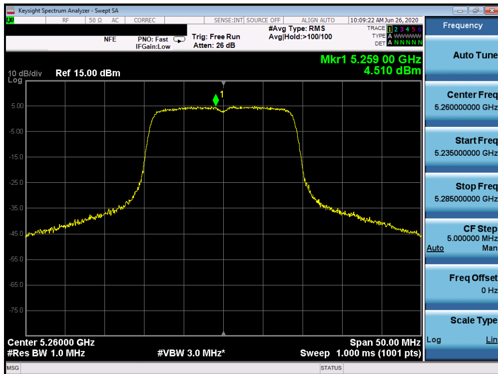
Plot 7-154. Power Spectral Density Plot SISO ANT1 (20MHz BW 802.11n (UNII Band 2A) – Ch. 52)
