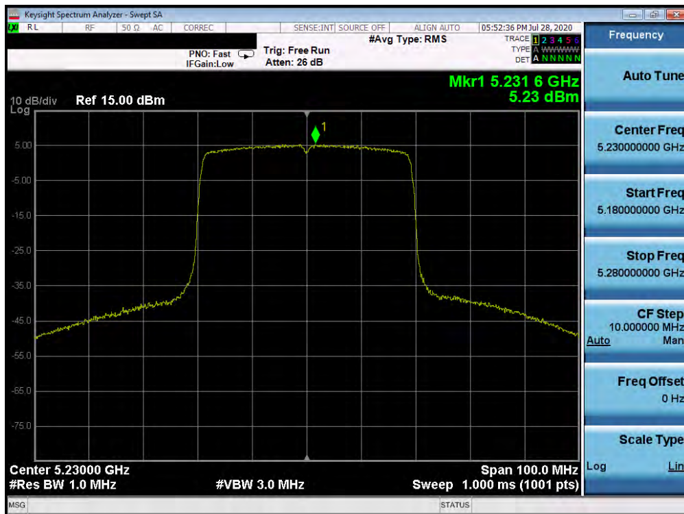
Plot 7-148. Power Spectral Density Plot SISO ANT1 (40MHz BW 802.11ax (UNII Band 1) – Ch. 46)
