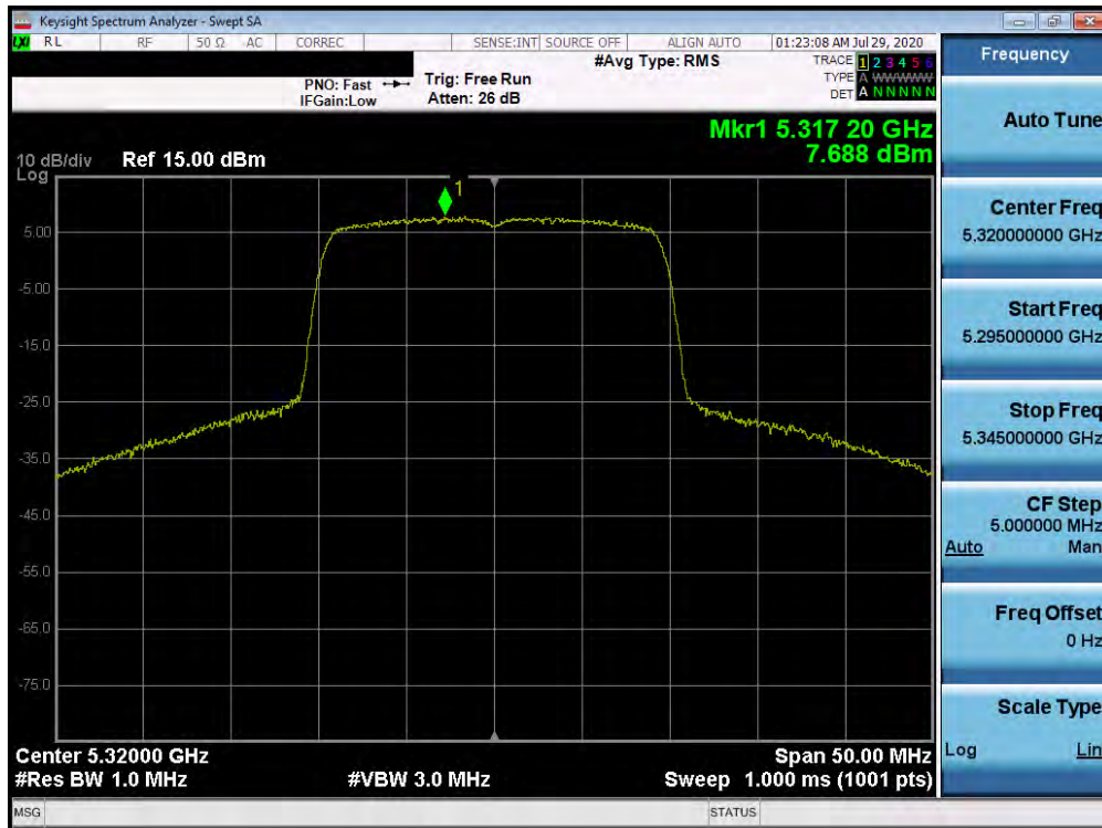
Plot 7-159. Power Spectral Density Plot SISO ANT1 (20MHz BW 802.11ax (UNII Band 2A) – Ch. 64)
