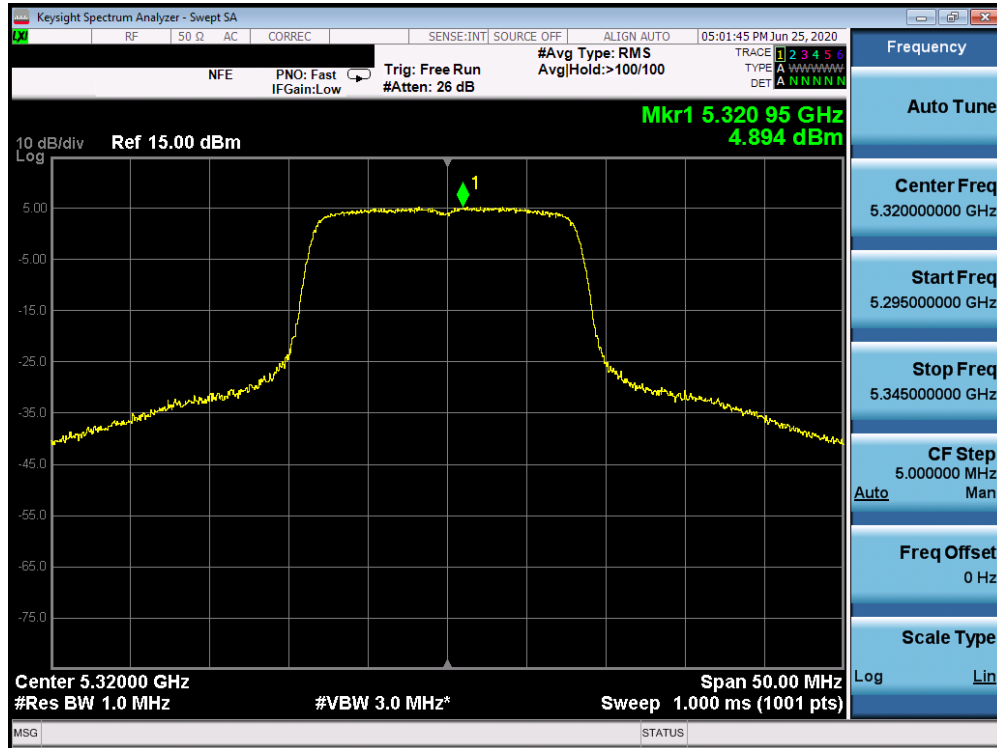
Plot 7-153. Power Spectral Density Plot SISO ANT1 (802.11a (UNII Band 2A) – Ch. 64)
