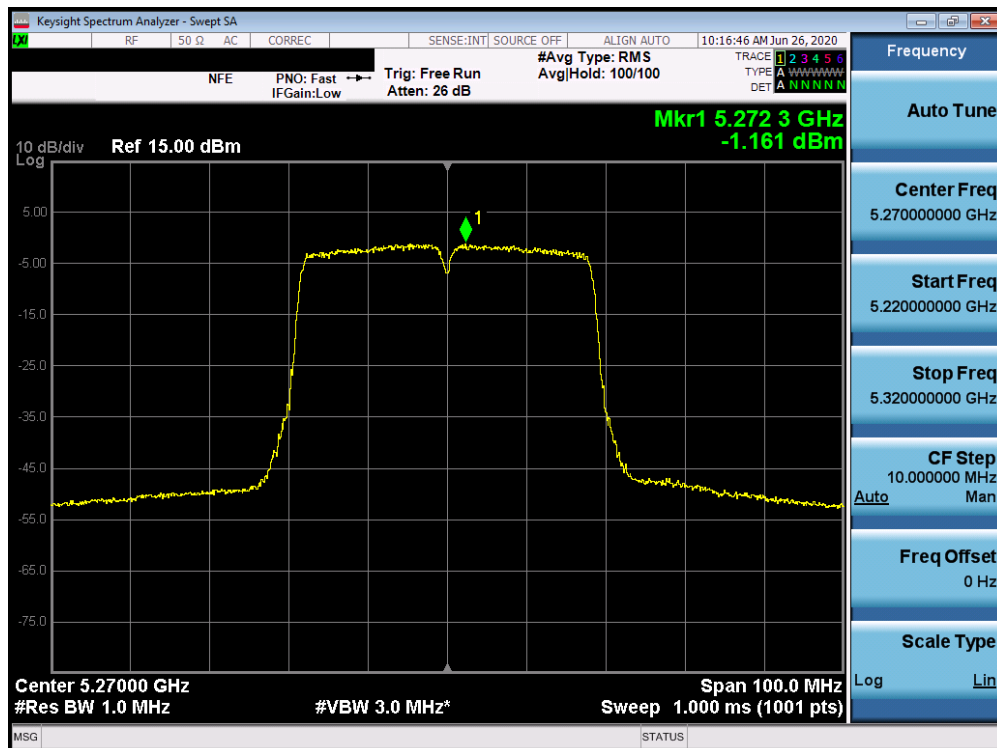
Plot 7-160. Power Spectral Density Plot SISO ANT1 (40MHz BW 802.11n (UNII Band 2A) – Ch. 54)
