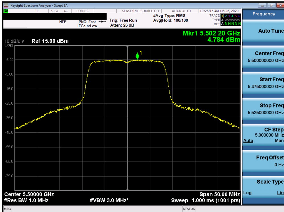
Plot 7-166. Power Spectral Density Plot SISO ANT1 (802.11a (UNII Band 2C) – Ch. 100)
