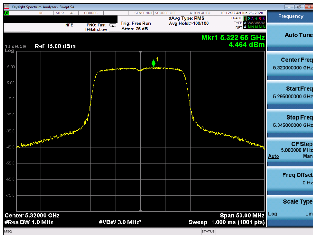
Plot 7-156. Power Spectral Density Plot SISO ANT1 (20MHz BW 802.11n (UNII Band 2A) – Ch. 64)
