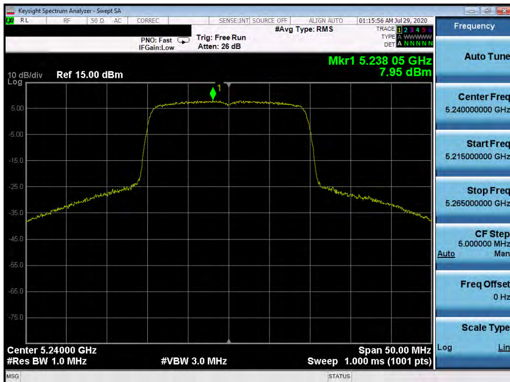
Plot 7-144. Power Spectral Density Plot SISO ANT1 (20MHz BW 802.11ax (UNII Band 1) – Ch. 48)
