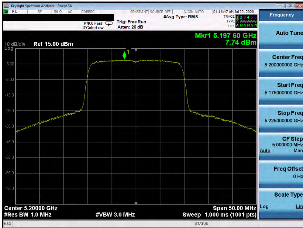
Plot 7-143. Power Spectral Density Plot SISO ANT1 (20MHz BW 802.11ax (UNII Band 1) – Ch. 40)
