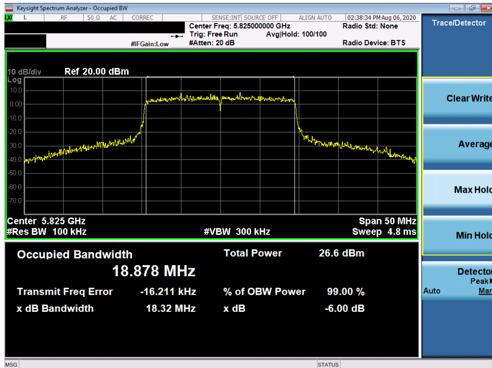
Plot 7-129. 6dB Bandwidth Plot SISO ANT2 (20MHz BW 802.11ax (UNII Band 3) – Ch. 165)
