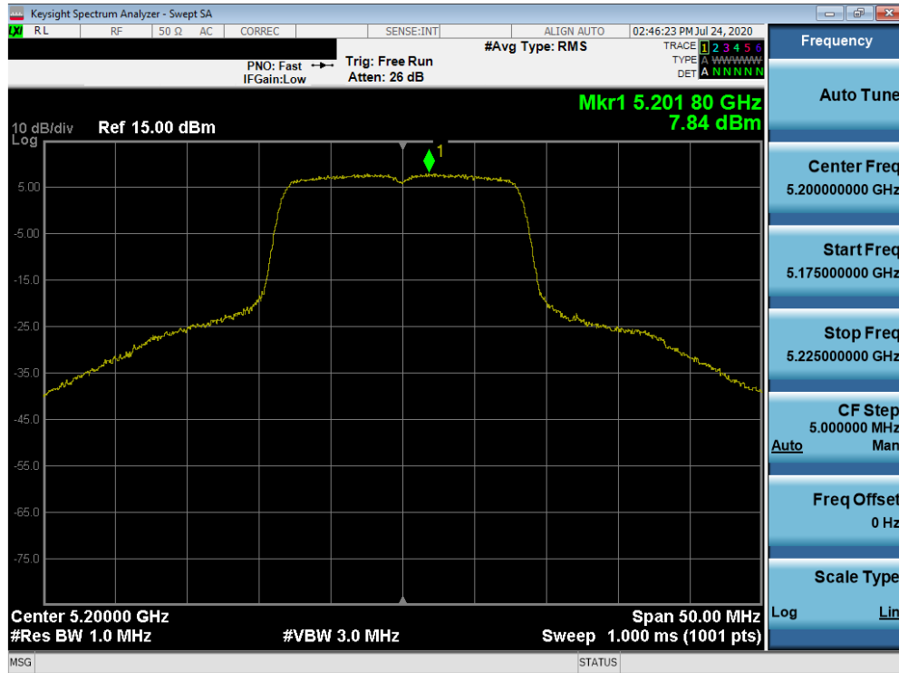
Plot 7-203. Power Spectral Density Plot SISO ANT2 (802.11a (UNII Band 1) – Ch. 40)
