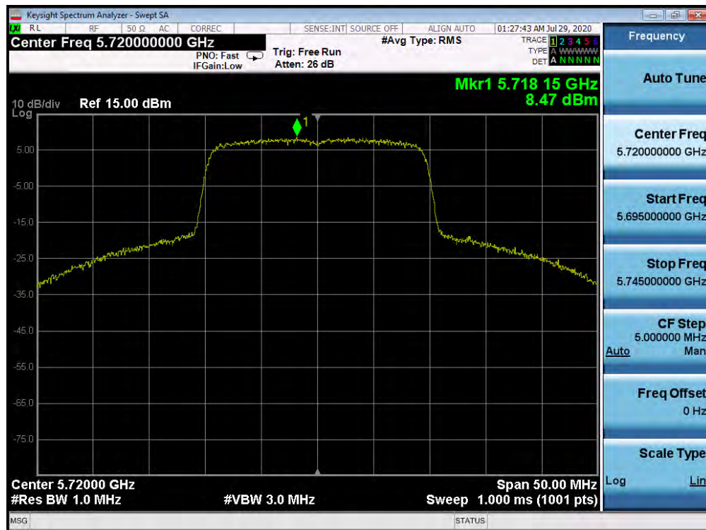
Plot 7-174. Power Spectral Density Plot SISO ANT1 (20MHz BW 802.11ax (UNII Band 2C) – Ch. 144)
