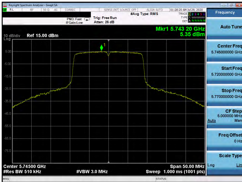
Plot 7-193. Power Spectral Density Plot SISO ANT1 (20MHz BW 802.11ax (UNII Band 3) – Ch. 149)
