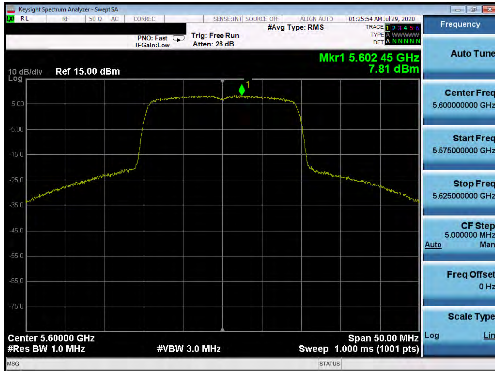
Plot 7-173. Power Spectral Density Plot SISO ANT1 (20MHz BW 802.11ax (UNII Band 2C) – Ch. 120)
