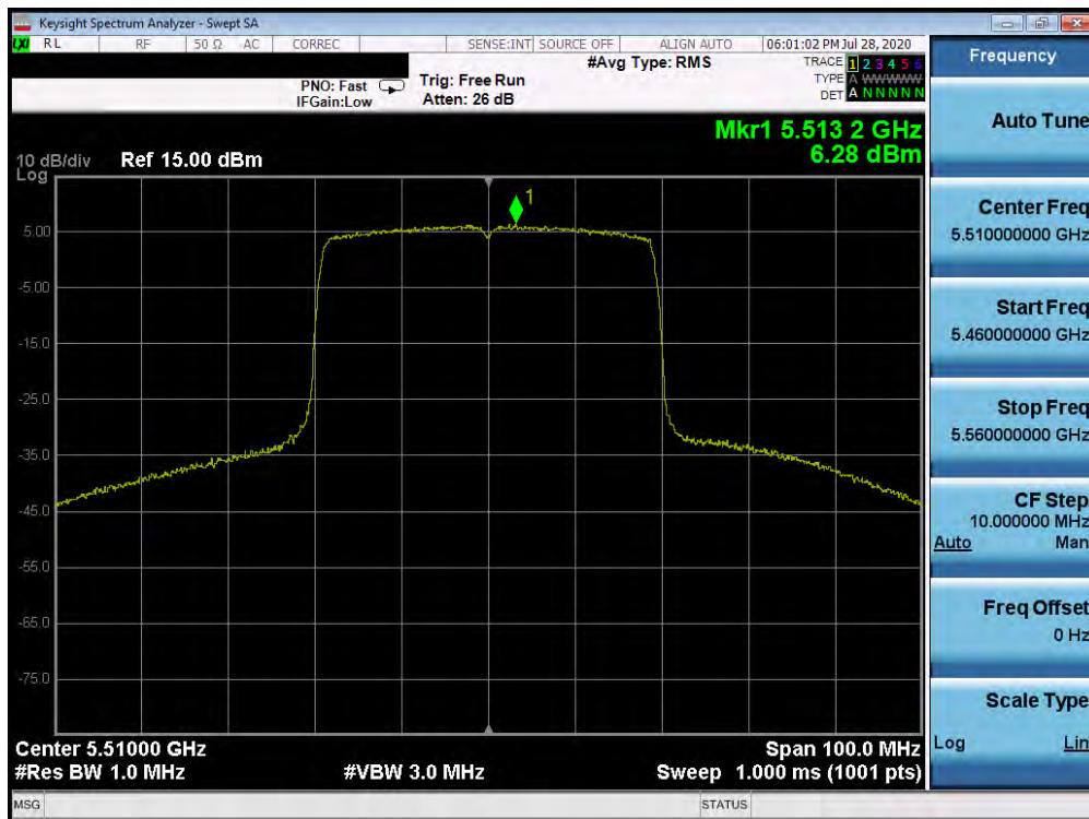
Plot 7-178. Power Spectral Density Plot SISO ANT1 (40MHz BW 802.11ax (UNII Band 2C) – Ch. 102)
