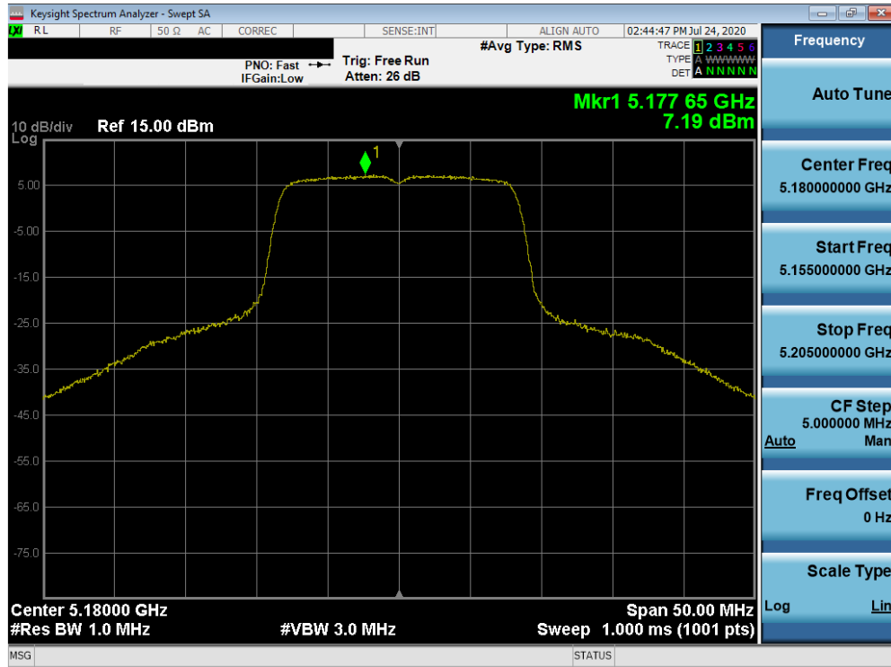
Plot 7-202. Power Spectral Density Plot SISO ANT2 (802.11a (UNII Band 1) – Ch. 36)
