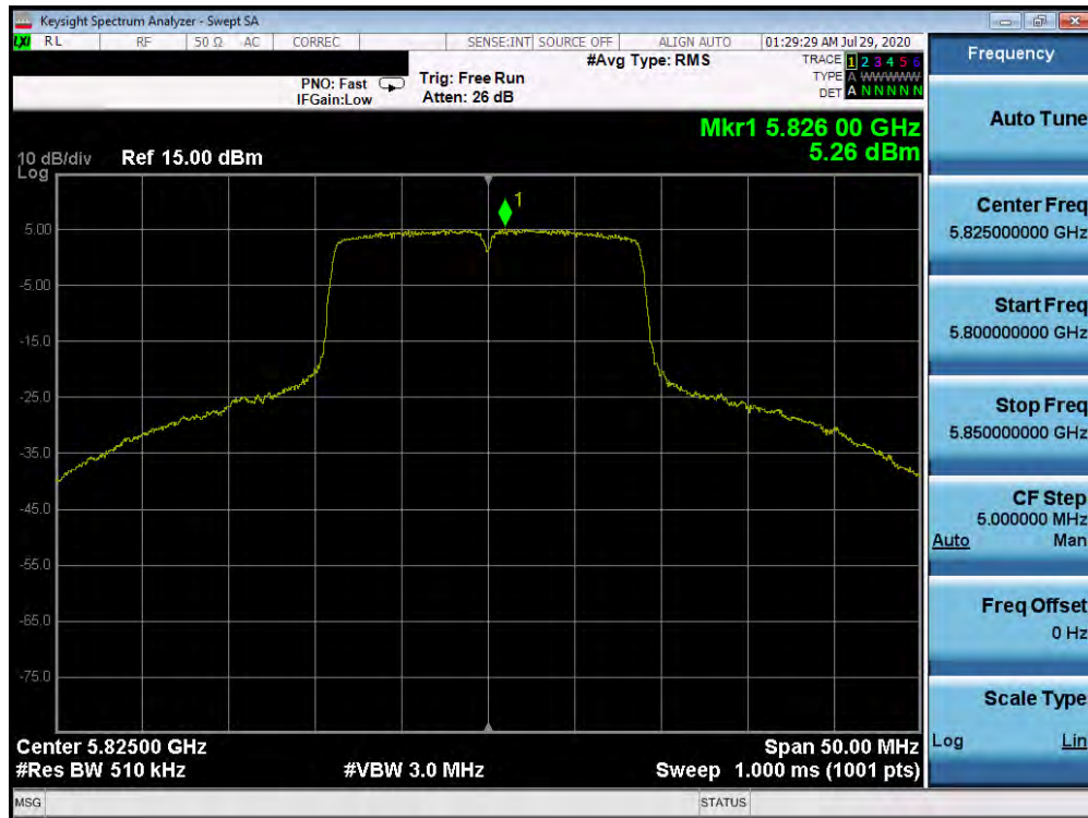
Plot 7-192. Power Spectral Density Plot SISO ANT1 (20MHz BW 802.11n (UNII Band 3) – Ch. 165)
