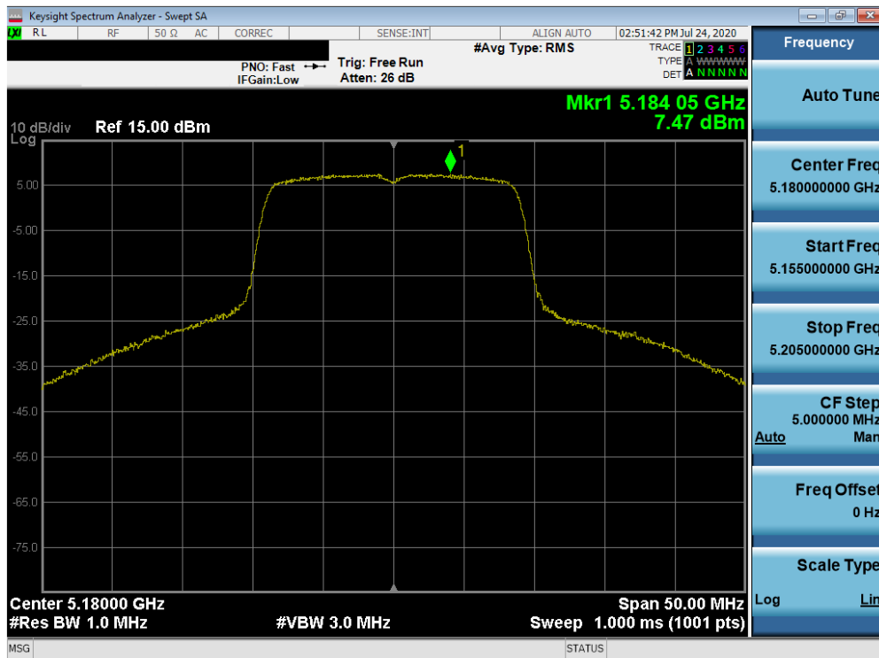
Plot 7-205. Power Spectral Density Plot SISO ANT2 (20MHz BW 802.11n (UNII Band 1) – Ch. 36)
