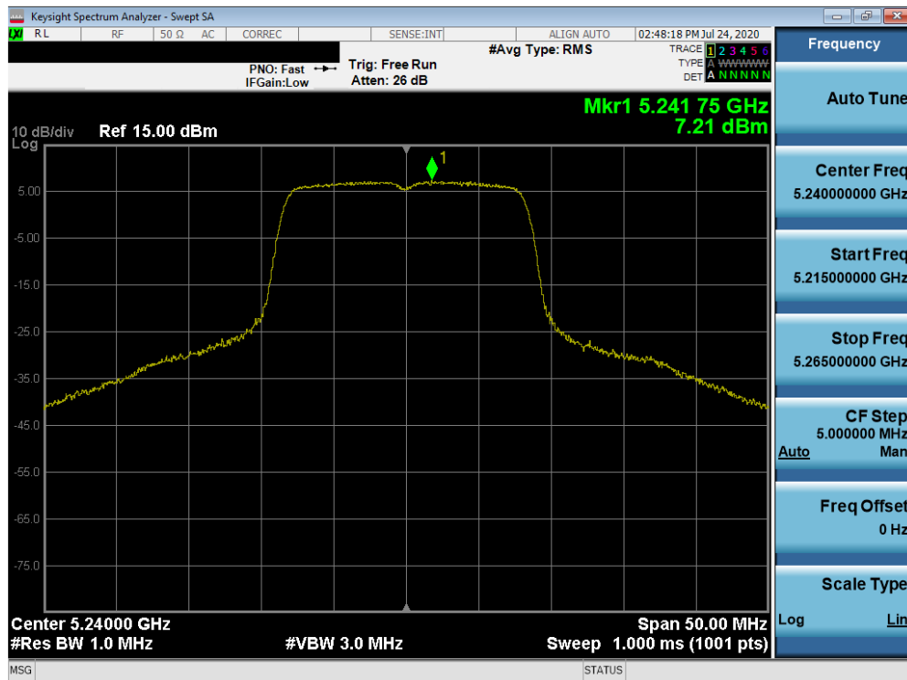
Plot 7-204. Power Spectral Density Plot SISO ANT2 (802.11a (UNII Band 1) – Ch. 48)
