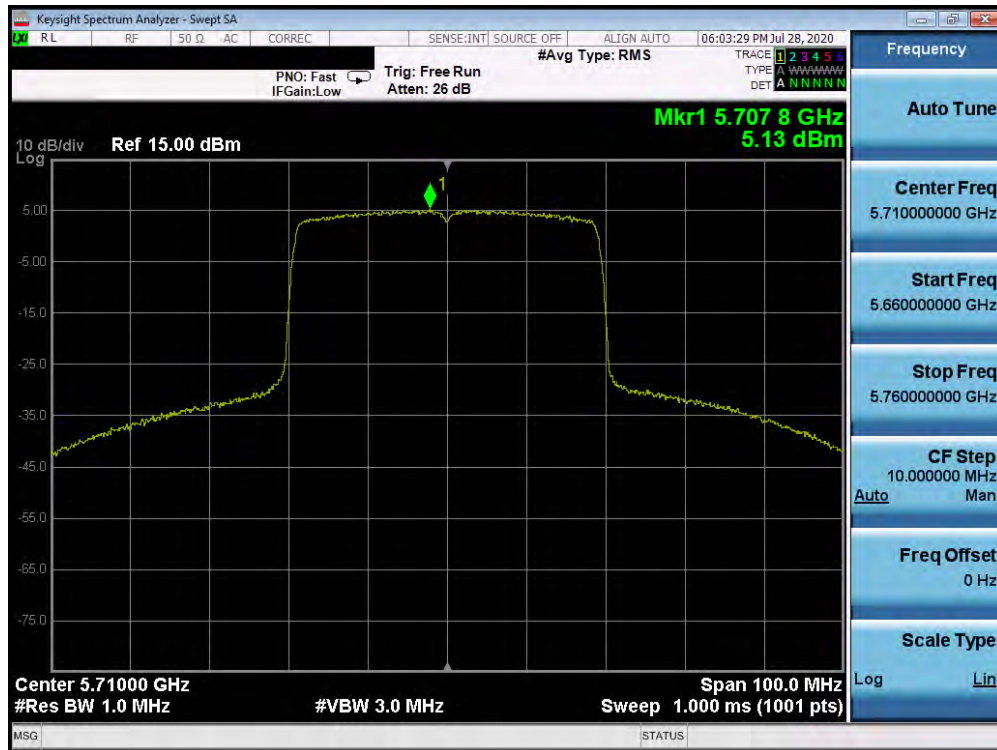
Plot 7-177. Power Spectral Density Plot SISO ANT1 (40MHz BW 802.11n (UNII Band 2C) – Ch. 142)
