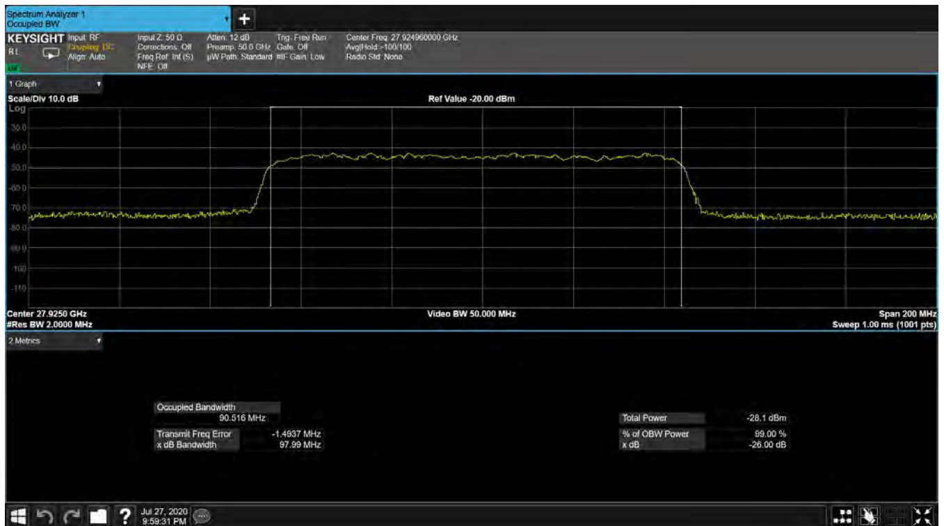
Plot 7-1. Ant 1 Occupied Bandwidth Plot (100MHz-1CC – pi/2-BPSK – Mid Channel)
