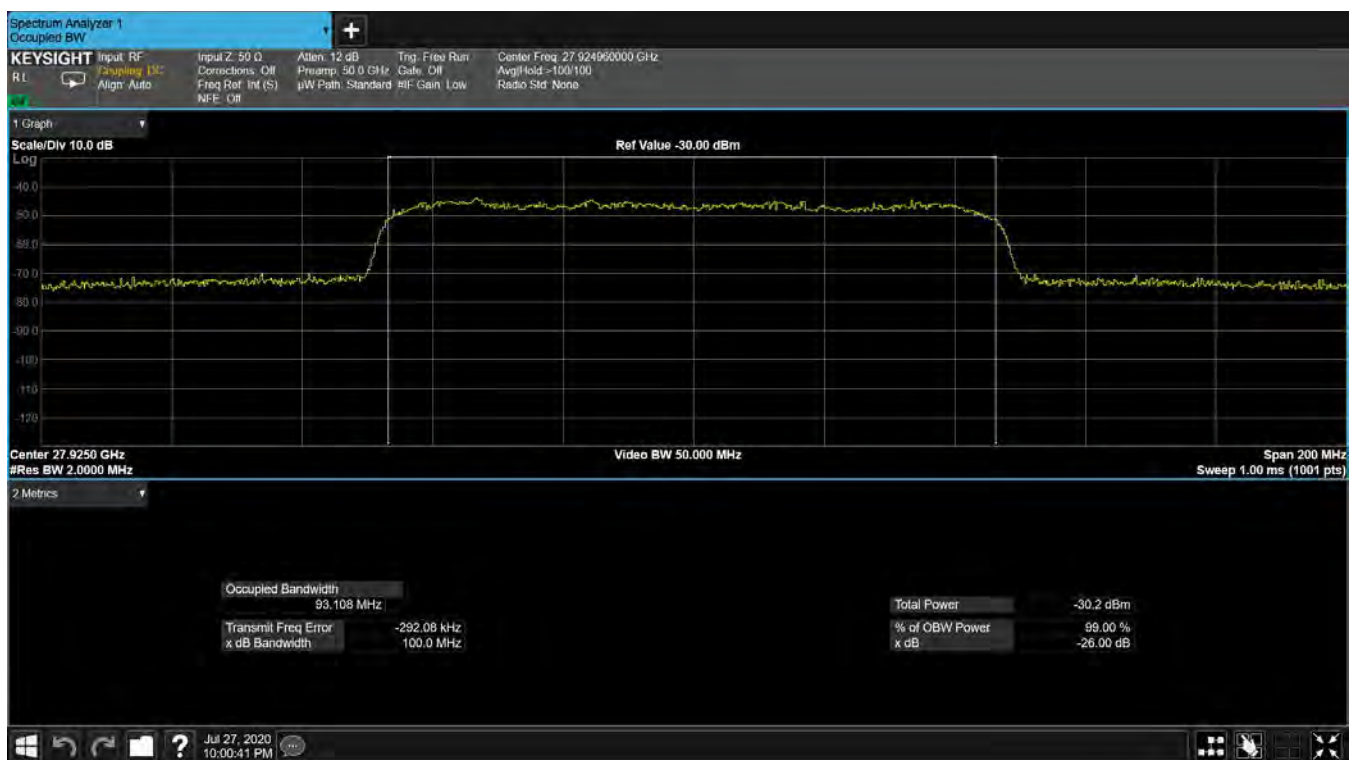
Plot 7-2. Ant 1 Occupied Bandwidth Plot (100MHz-1CC – QPSK – Mid Channel)
