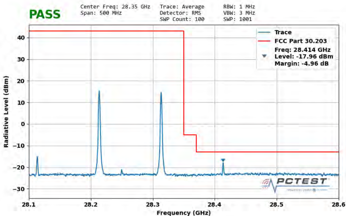
Plot 7-70. Ant 3 Upper Band Edge (100MHz-2CC – QPSK 1 RB)
