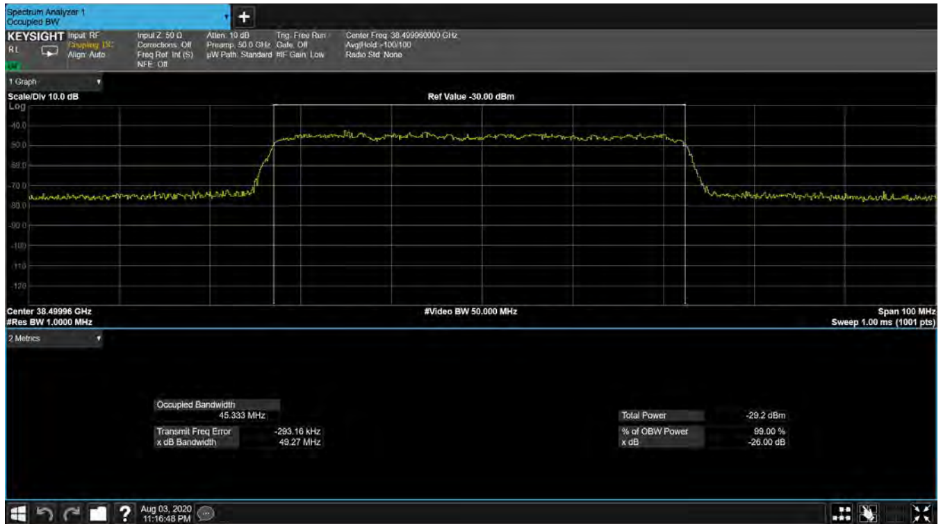
Plot 7-27. Ant 1 Occupied Bandwidth Plot (50MHz-1CC – 16QAM – Mid Channel)
