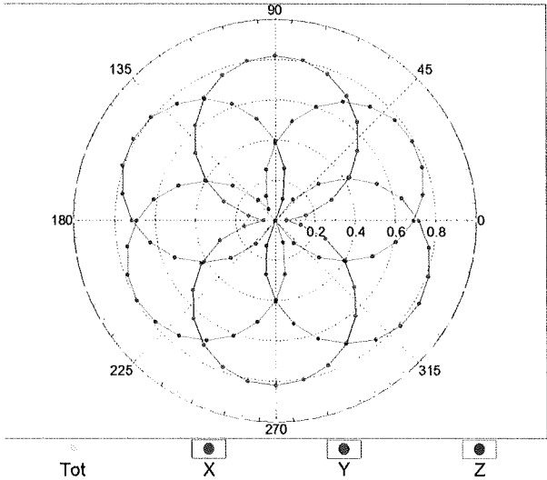
f=600 MHz,TEM
