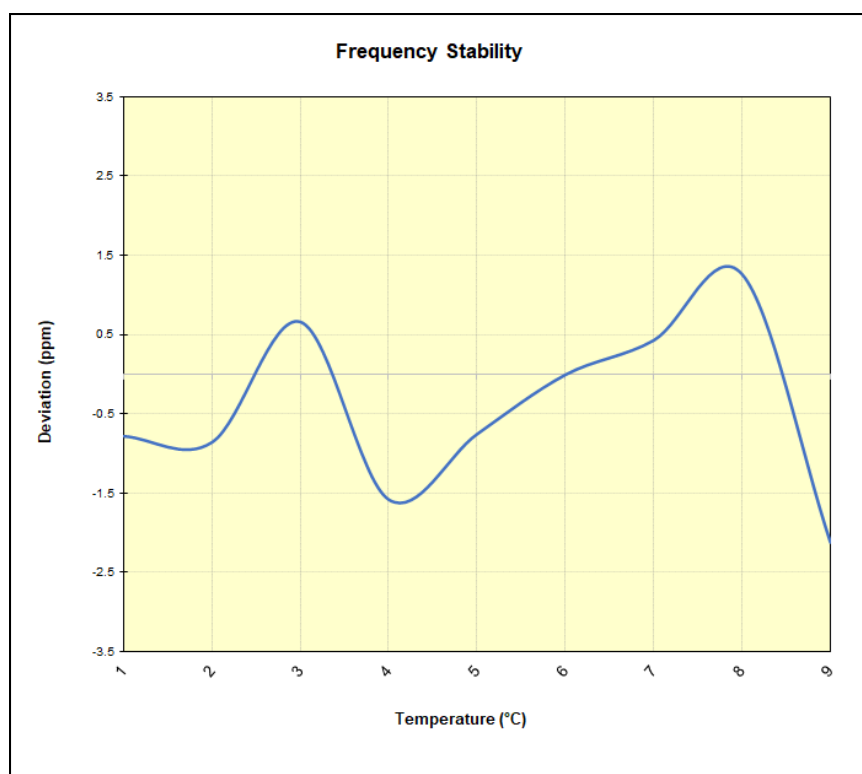
Plot 7-25. LTE Band 26 Frequency Stability Chart
