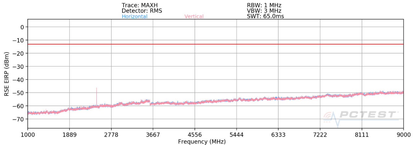
Plot 7-22. Radiated Spurious Plot (LTE Band 26 – AntA + AntB)- OPEN
