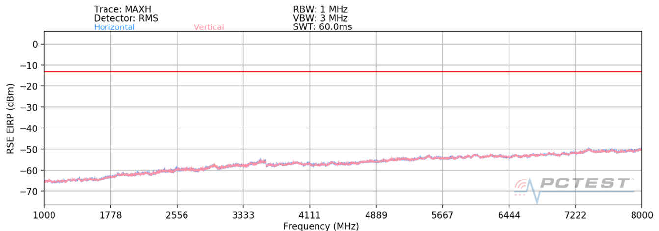
Plot 7-2. Radiated Spurious Plot above 1GHz - OPEN
