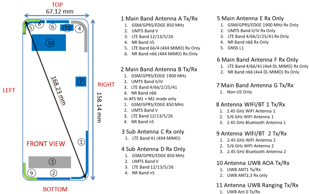
Figure C-1 DUT Antenna Locations – Closed
