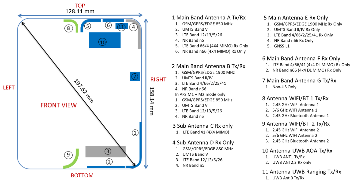
Figure C-2 DUT Antenna Locations - Open
