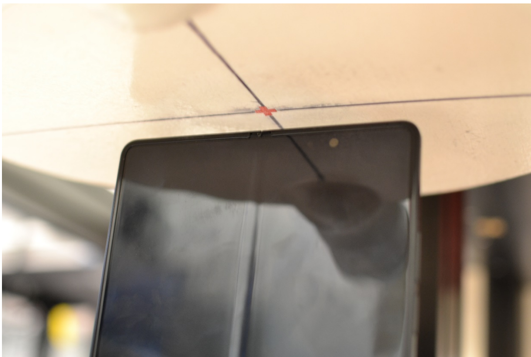
Figure C-16 SAR Test Setup Photo – UMPC Body, Top Edge at 10mm
