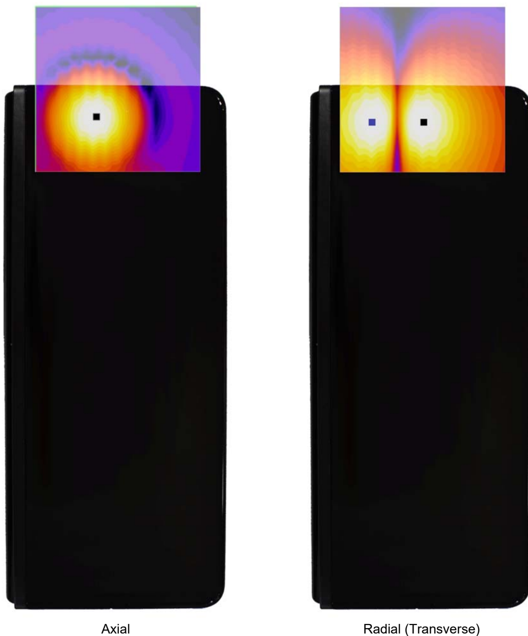
Figure 16-3 T-Coil Scan Overlay Magnetic Field Distributions
