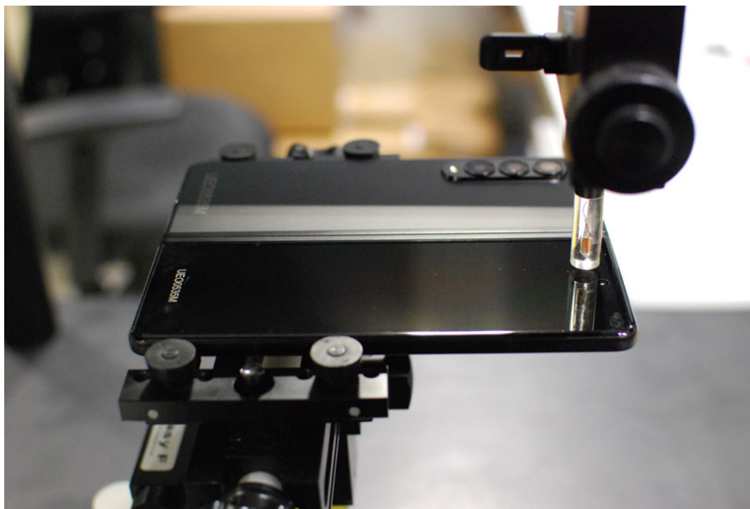
Figure 13-3 Test Setup for Wireless Device (FLAT – BACK)
