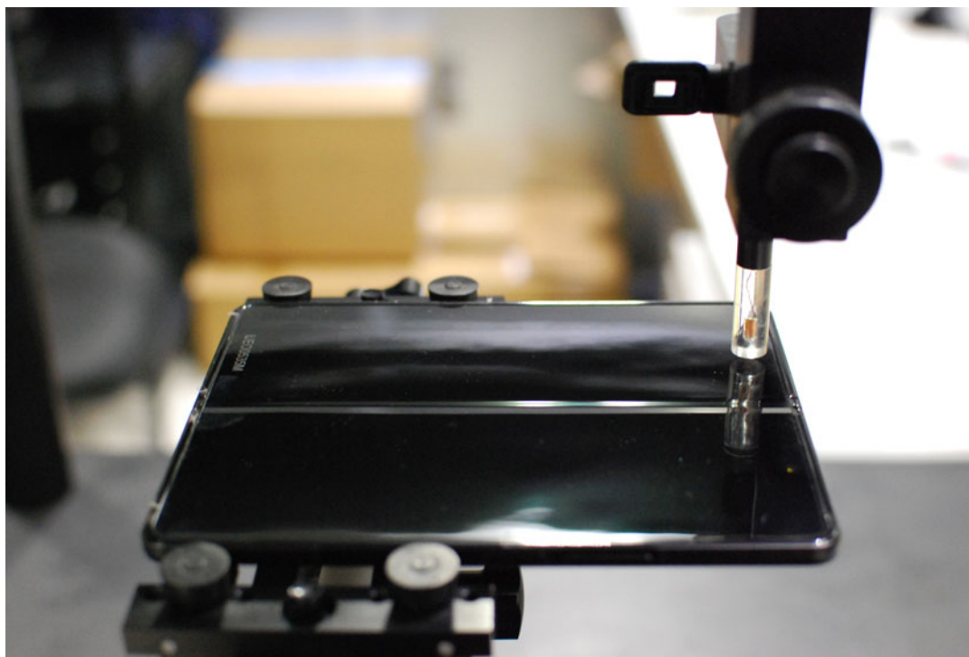
Figure 13-1 Test Setup for Wireless Device (FLAT – FRONT)
