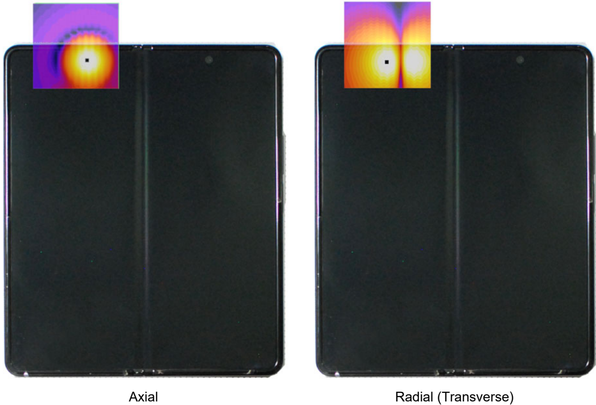
Figure 13-5 T-Coil Scan Overlay Magnetic Field Distributions (FLAT – FRONT)
