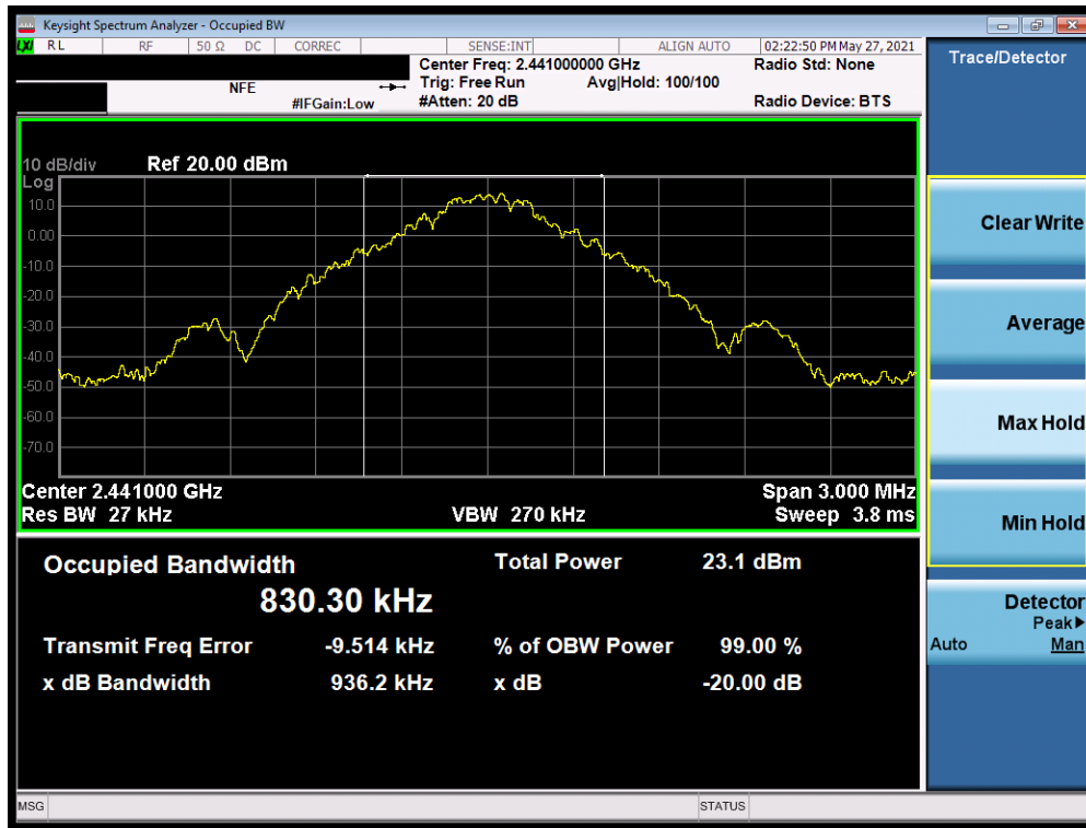
Plot 7-2. 20dB Bandwidth Plot (Bluetooth, 1Mbps – Ch. 39) Antenna 0
