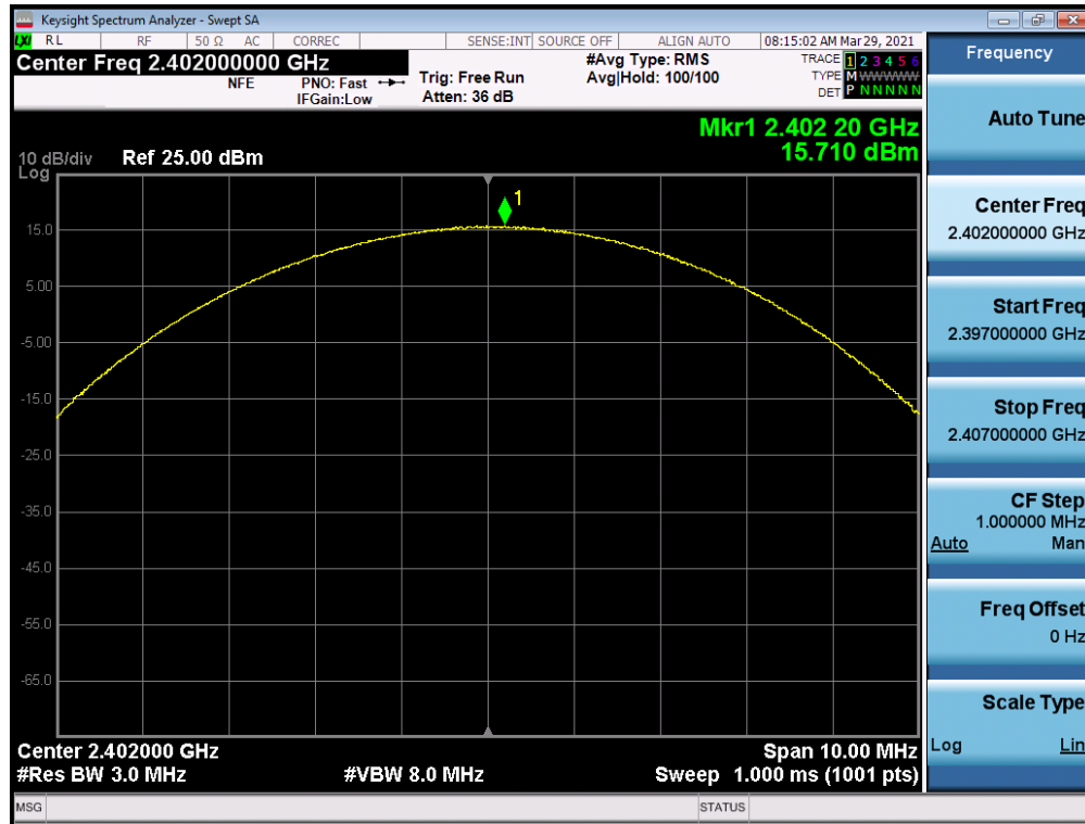
Plot 7-70. Peak Conducted Power (3Mbps – Ch. 0) Antenna 1 iPA
