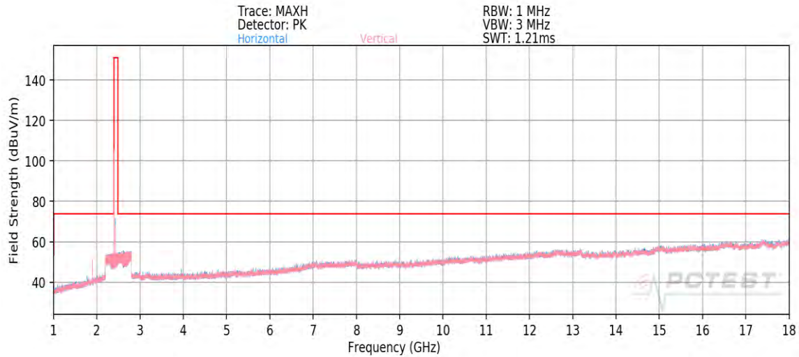
Plot 7-115. Radiated Spurious Plot above 1GHz (BT– Ch. 0)
