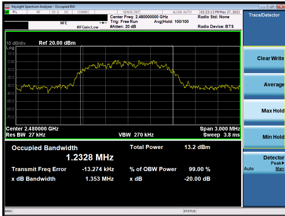
Plot 7-6. 20dB Bandwidth Plot (Bluetooth, 2Mbps – Ch. 78) Antenna 0
