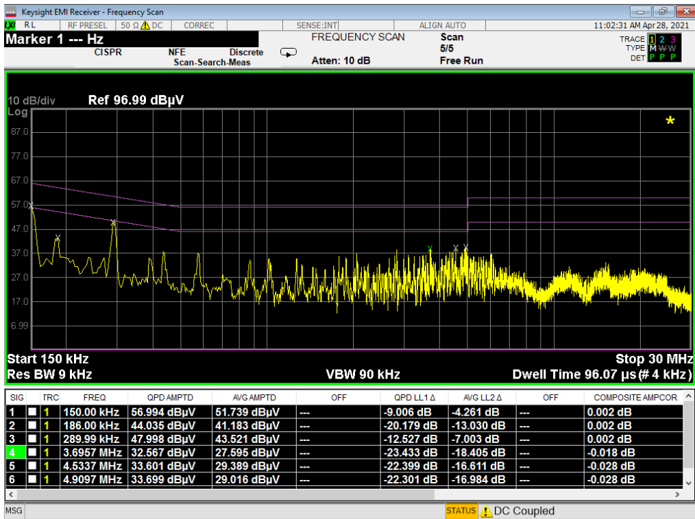
Plot 7-124. Line-Conducted Test Plot (N)
