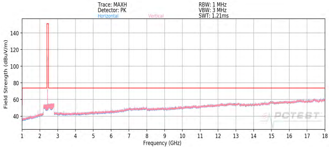
Plot 7-116. Radiated Spurious Plot above 1GHz (BT– Ch. 39)
