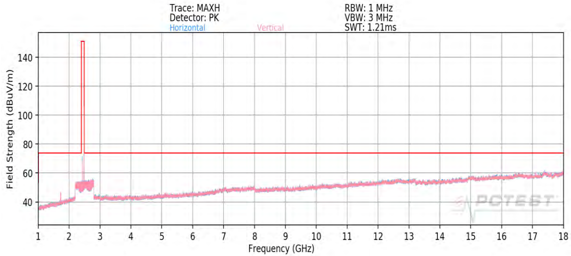
Plot 7-117. Radiated Spurious Plot above 1GHz (BT– Ch. 78)
