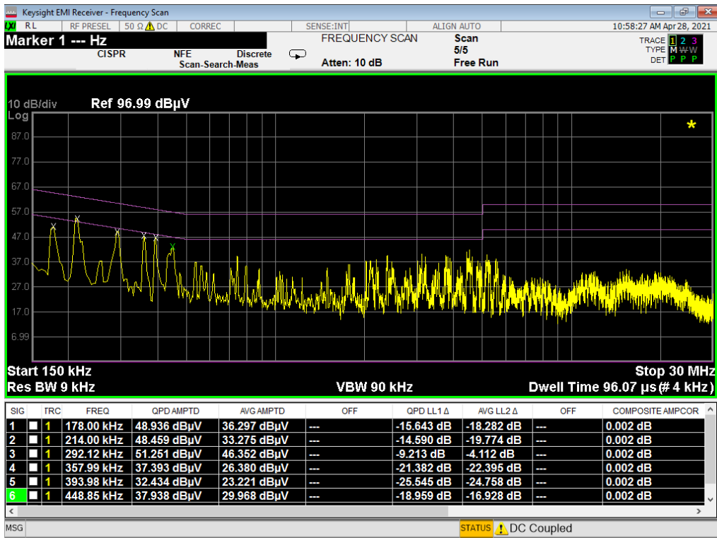
Plot 7-123. Line-Conducted Test Plot (L1)
