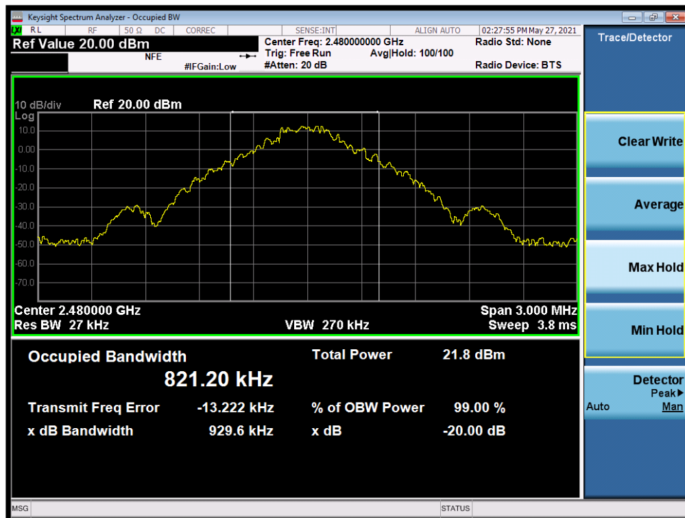
Plot 7-12. 20dB Bandwidth Plot (Bluetooth, 1Mbps – Ch. 78) Antenna 1
