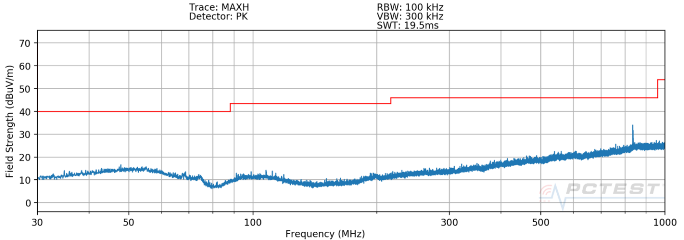
Plot 7-4. Radiated Spurious Plot 30MHz – 1GHz (Pol. H) - Open
