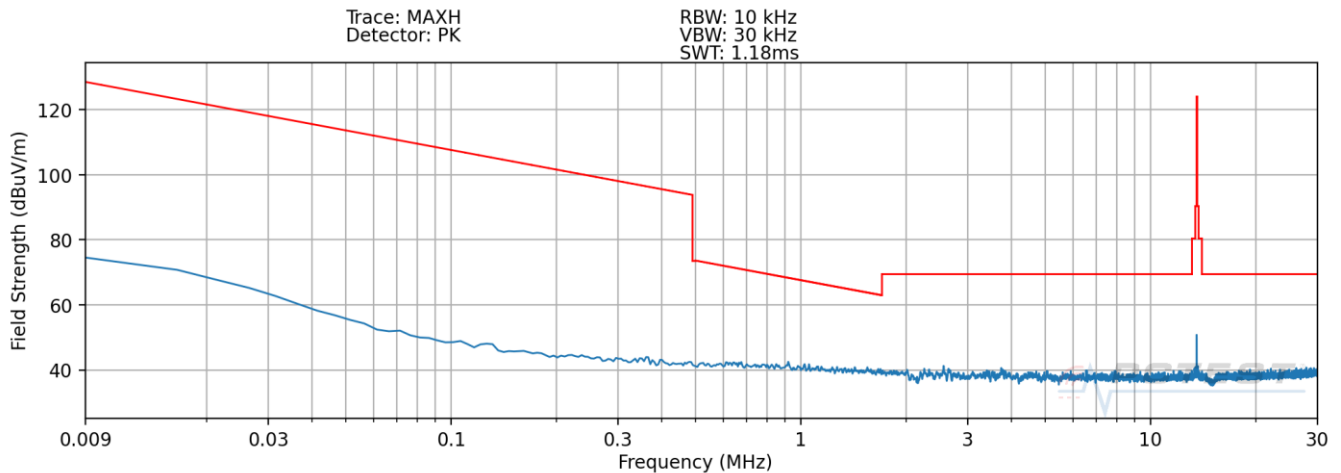
Plot 7-7. Radiated Spurious Plot 9kHz – 30MHz (Pol. Y) - Closed
