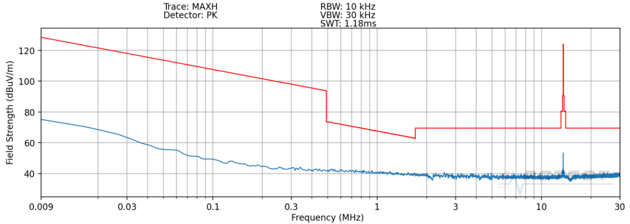
Plot 7-1. Radiated Spurious Plot 9kHz – 30MHz (Pol. X) - Open
