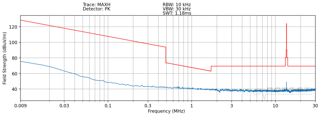
Plot 7-8. Radiated Spurious Plot 9kHz – 30MHz (Pol. Z) - Closed
