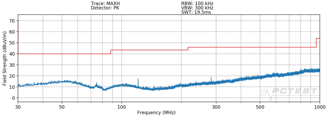
Plot 7-9. Radiated Spurious Plot 30MHz – 1GHz (Pol. H) - Closed
