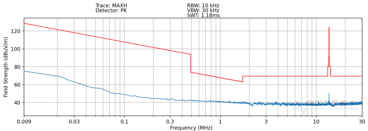
Plot 7-3. Radiated Spurious Plot 9kHz – 30MHz (Pol. Z) - Open
