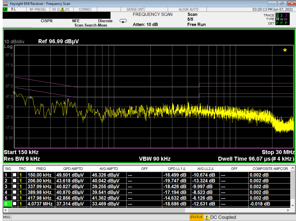
Plot 7-13. Line-Conducted Test Plot (L1) with WCP
