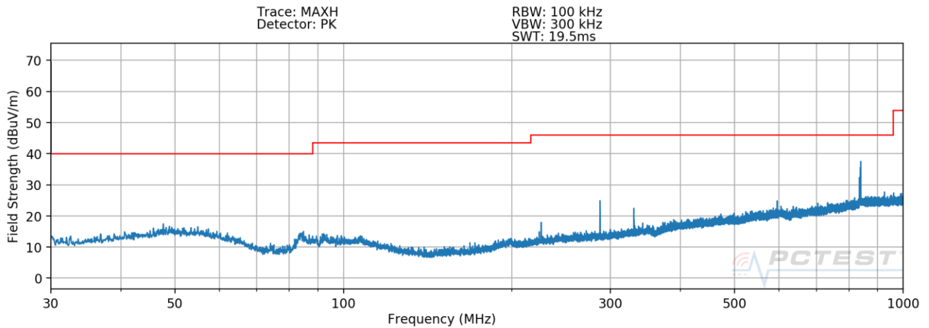
Plot 7-10. Radiated Spurious Plot 30MHz – 1GHz (Pol. V) - Closed
