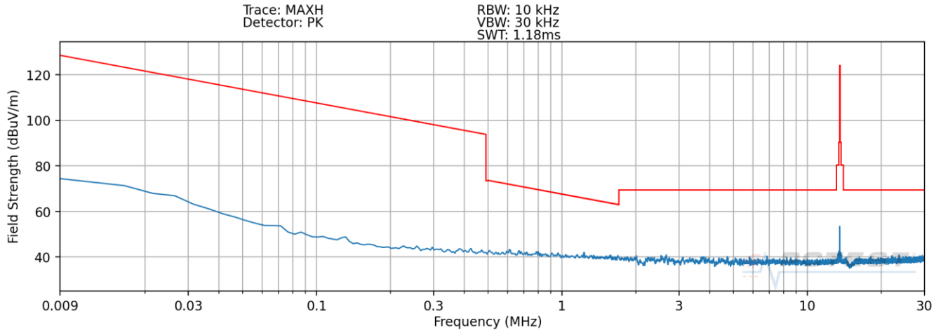
Plot 7-6. Radiated Spurious Plot 9kHz – 30MHz (Pol. X) - Closed
