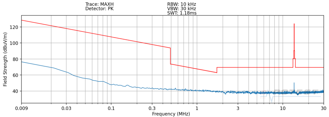
Plot 7-2. Radiated Spurious Plot 9kHz – 30MHz (Pol. Y) - Open
