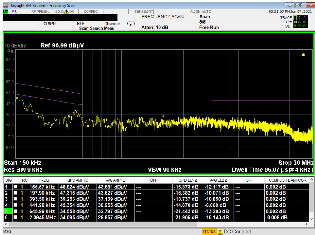
Plot 7-14. Line-Conducted Test Plot (N) with WCP
