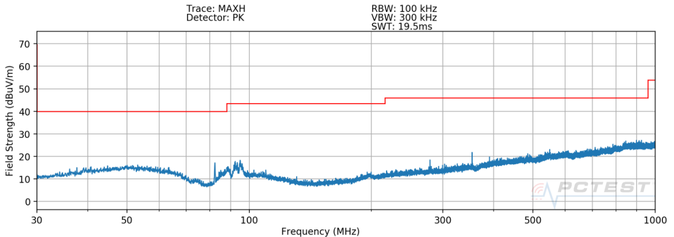
Plot 7-5. Radiated Spurious Plot 30MHz – 1GHz (Pol. V) - Open
