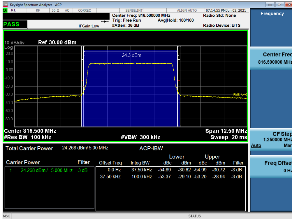
Plot 7-39. Channel Edge Plot (LTE Band 26 - 5MHz QPSK - Low Channel)
