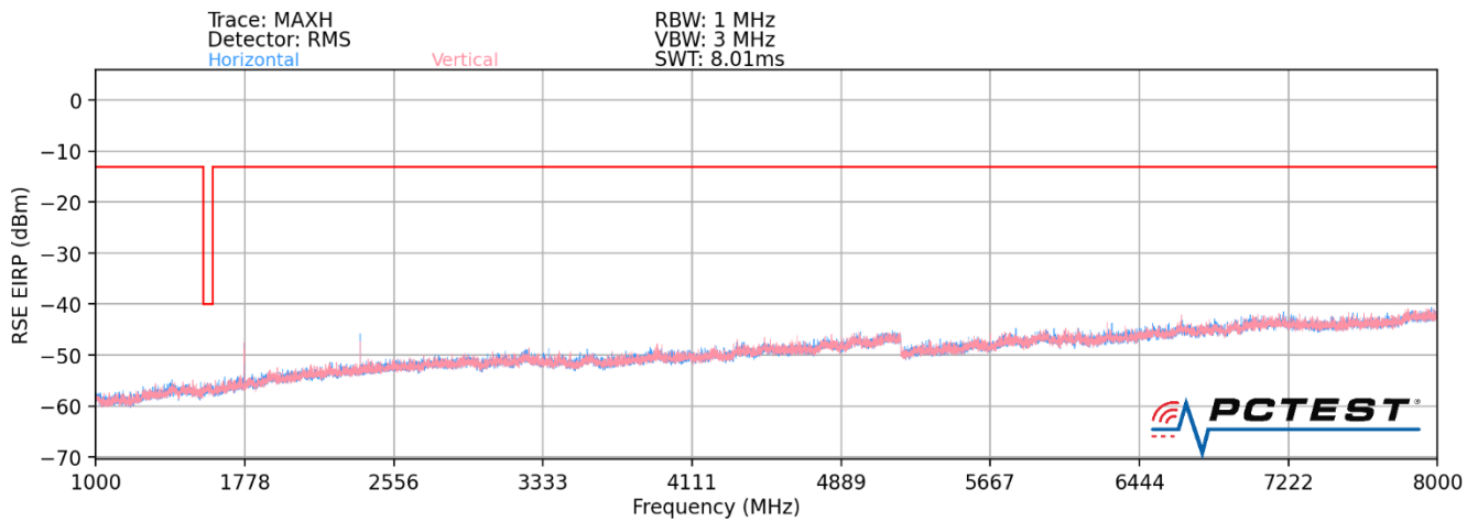
Plot 7-48. Radiated Spurious Plot (LTE Band 14) - CLOSE
