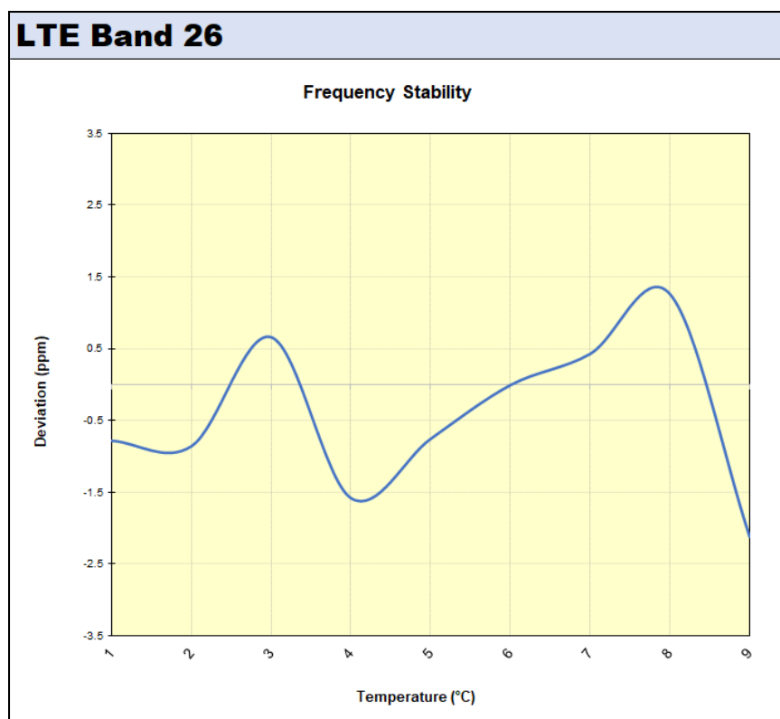
Plot 7-54. LTE Band 26 Frequency Stability Chart
