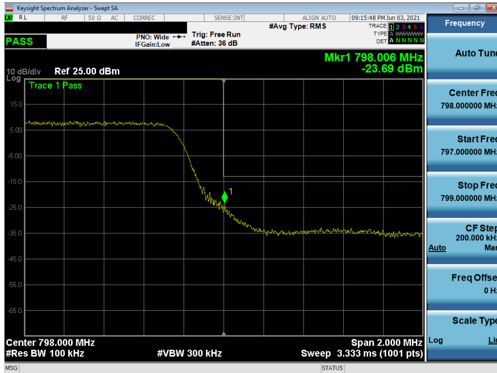
Plot 7-35. Upper Band Edge Plot (LTE Band 14, 5MHz QPSK - RB Size 25)
