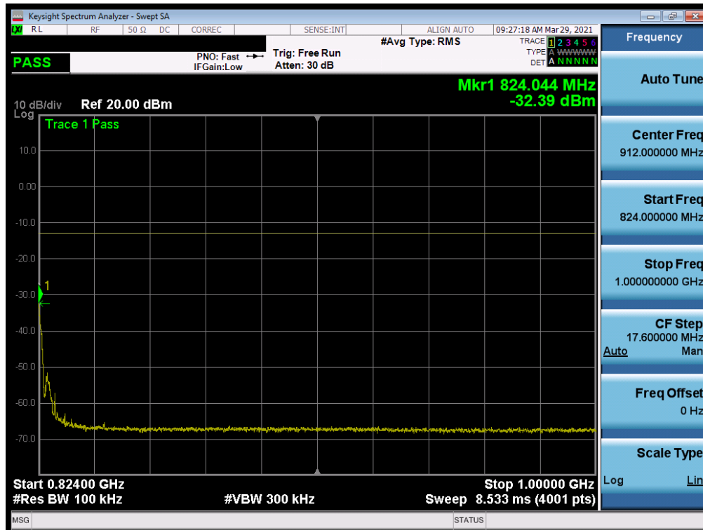
Plot 7-21. Conducted Spurious Plot (LTE Band 26 - 15MHz QPSK - RB Size 1, RB Offset 0)
