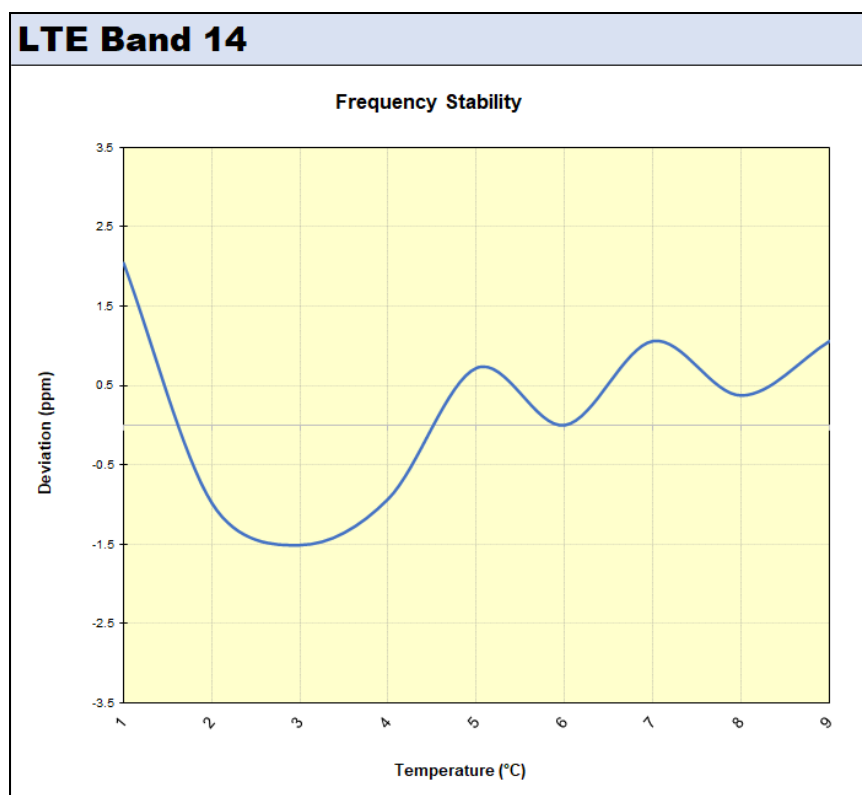
Plot 7-53. LTE Band 14 Frequency Stability Chart
