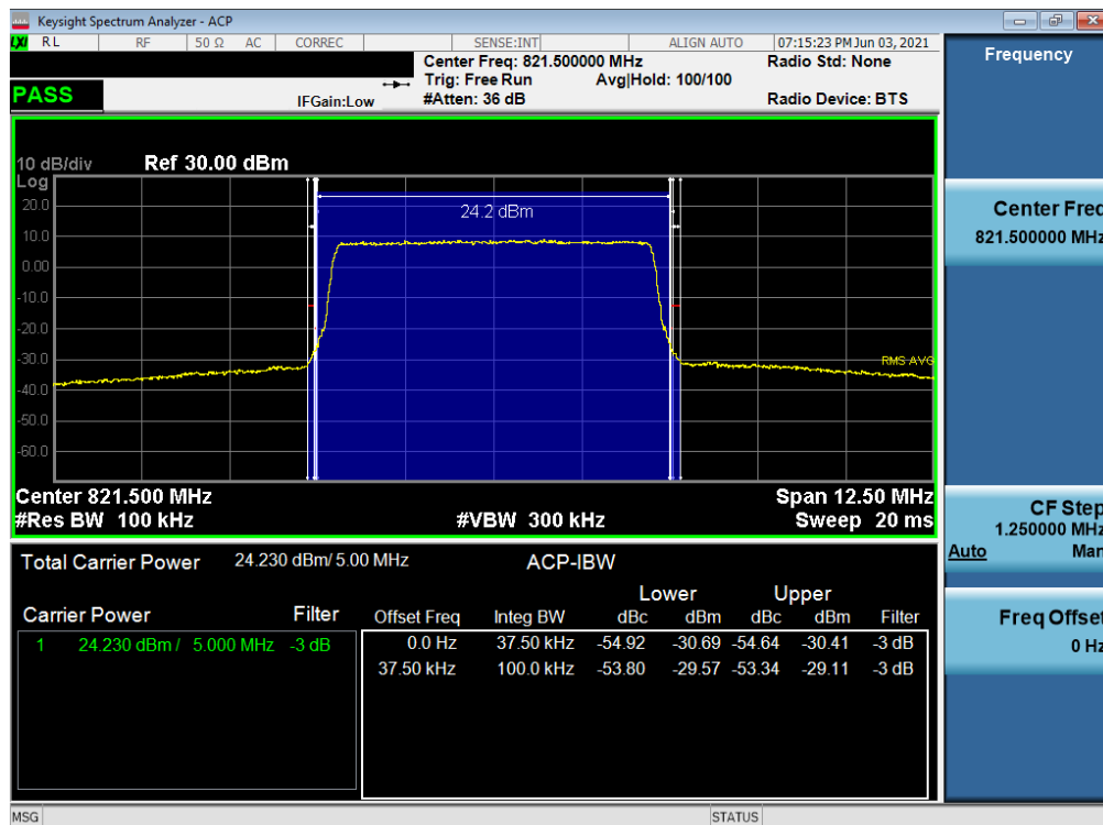
Plot 7-40. Channel Edge Plot (LTE Band 26 - 5MHz QPSK - High Channel)
