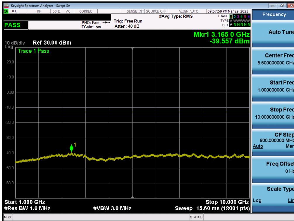
Plot 7-25. Conducted Spurious Plot (CDMA Ch. 476- Low Channel)
