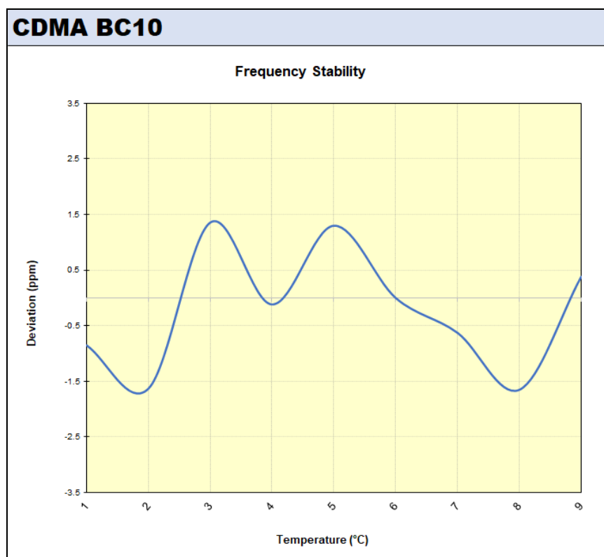
Plot 7-55. CDMA BC10 Frequency Stability Chart
