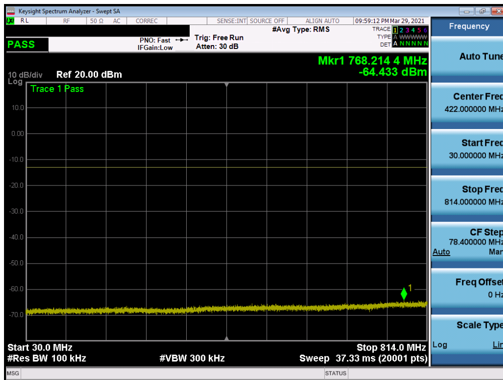
Plot 7-26. Conducted Spurious Plot (CDMA Ch. 684- High Channel)
