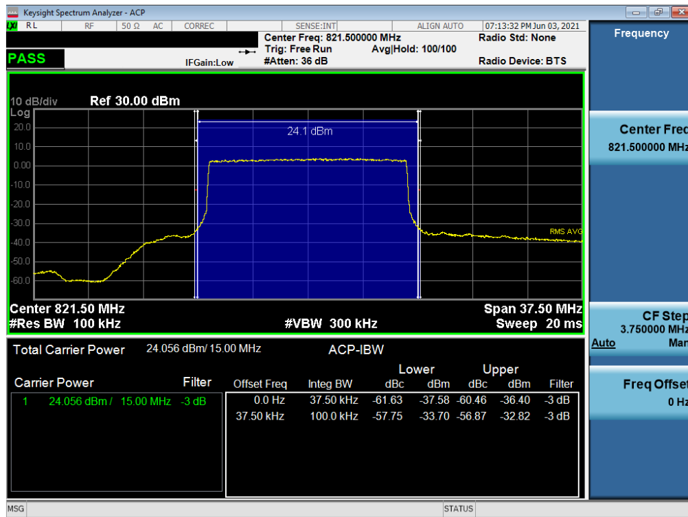
Plot 7-37. Channel Edge Plot (LTE Band 26 - 15MHz QPSK - Mid Channel)
