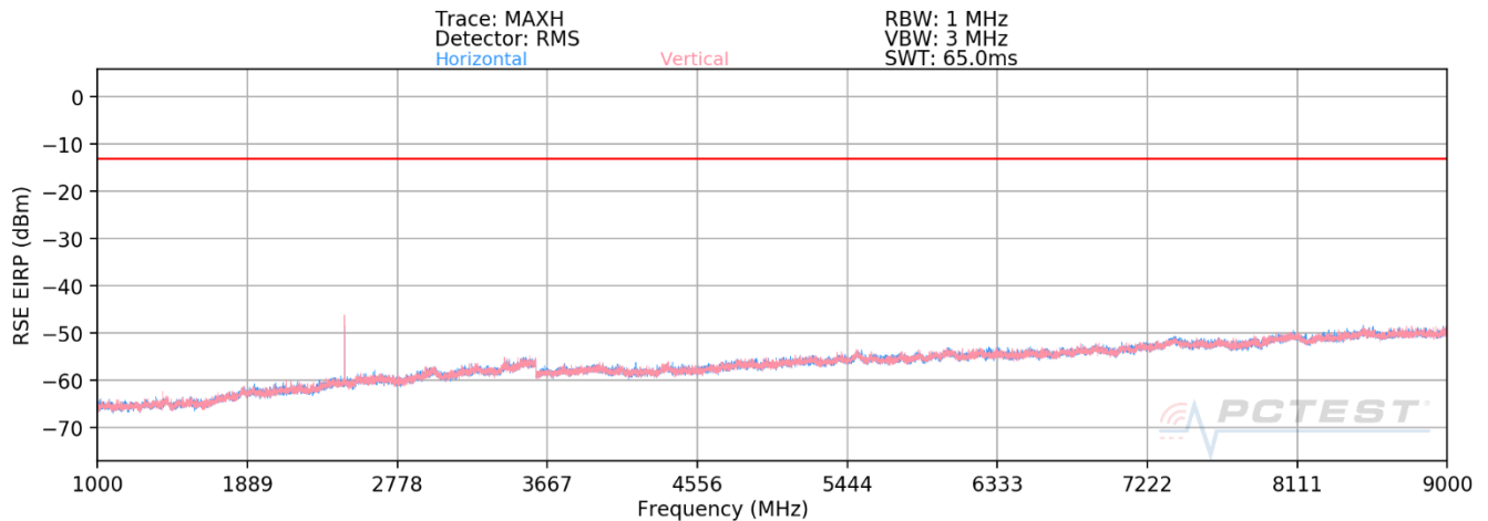
Plot 7-49. Radiated Spurious Plot (LTE Band 26 – AntA + AntB)- OPEN
