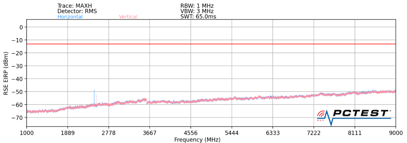
Plot 7-50. Radiated Spurious Plot (LTE Band 26 – AntA + AntB)- CLOSE
