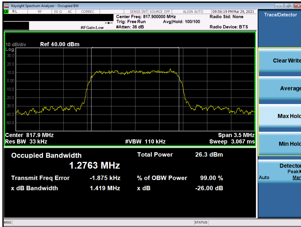
Plot 7-15. Occupied Bandwidth Plot (CDMA, Ch. 476)
