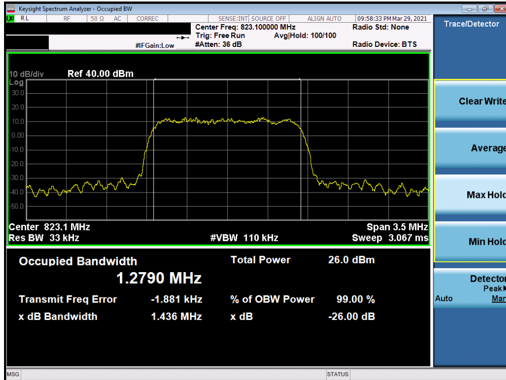
Plot 7-16. Occupied Bandwidth Plot (CDMA, Ch. 684)
