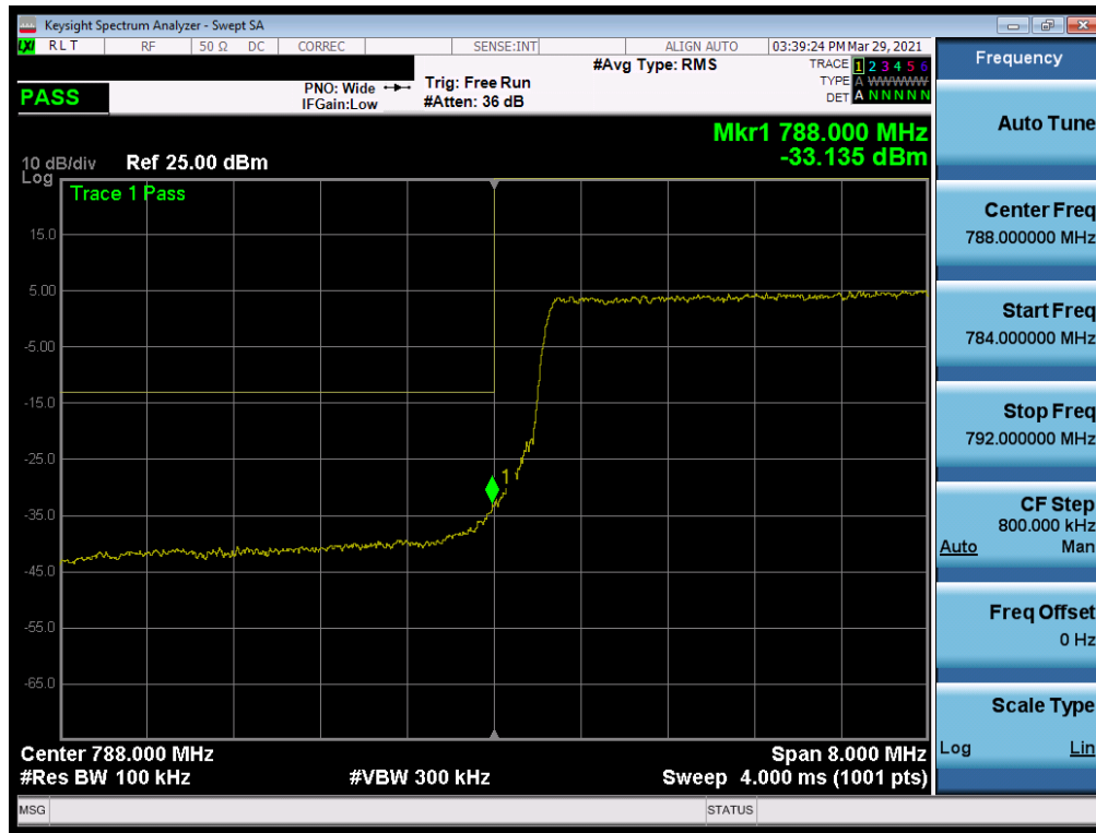
Plot 7-29. Lower Band Edge Plot (LTE Band 14, 10MHz QPSK - RB Size 50)
