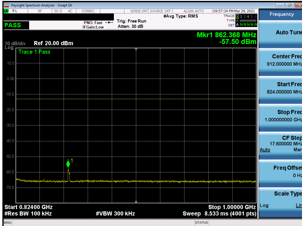
Plot 7-24. Conducted Spurious Plot (CDMA Ch. 476- Low Channel)
