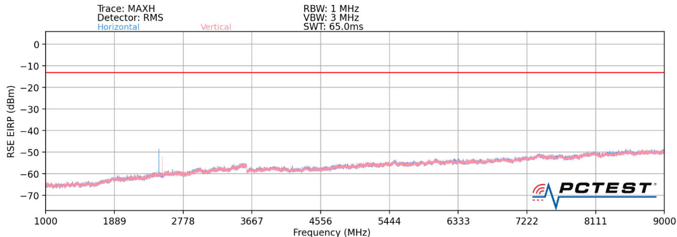
Plot 7-51. Radiated Spurious Plot (LTE Band 26 – AntA)- CLOSE
