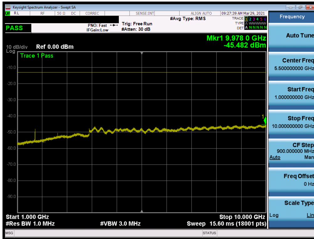
Plot 7-22. Conducted Spurious Plot (LTE Band 26 - 15MHz QPSK - RB Size 1, RB Offset 0)
