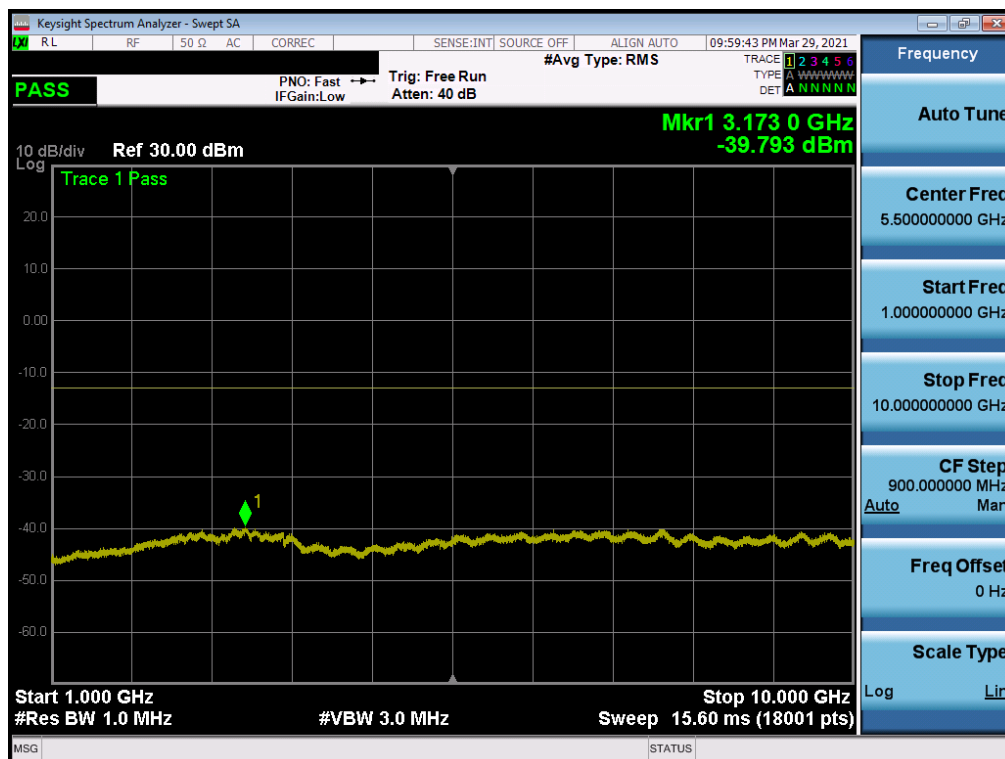
Plot 7-28. Conducted Spurious Plot (CDMA Ch. 684- High Channel)
