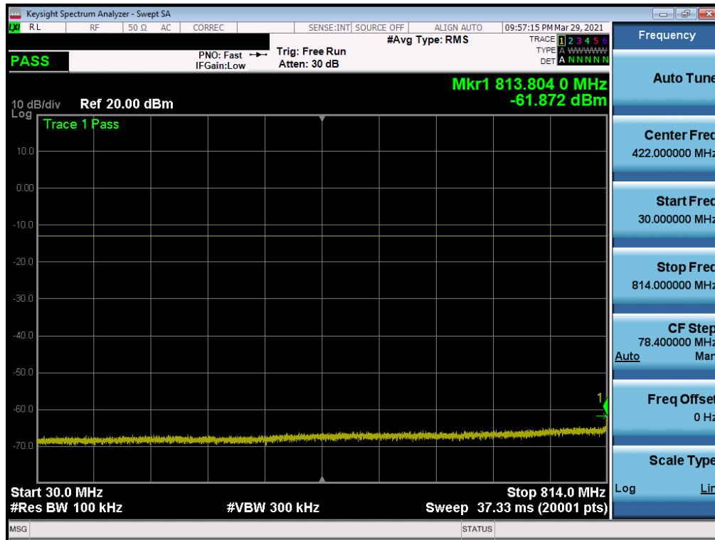
Plot 7-23. Conducted Spurious Plot (CDMA Ch. 476- Low Channel)
