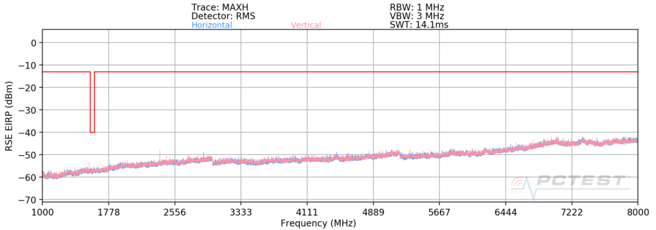
Plot 7-47. Radiated Spurious Plot (LTE Band 14) – OPEN
