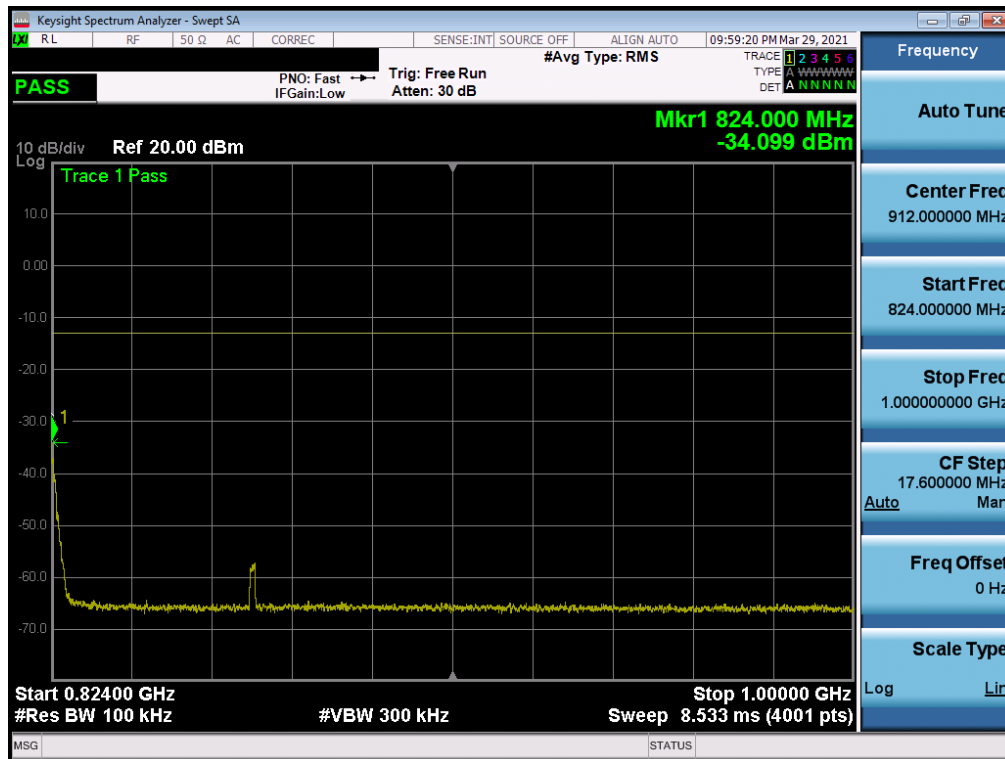
Plot 7-27. Conducted Spurious Plot (CDMA Ch. 684- High Channel)
