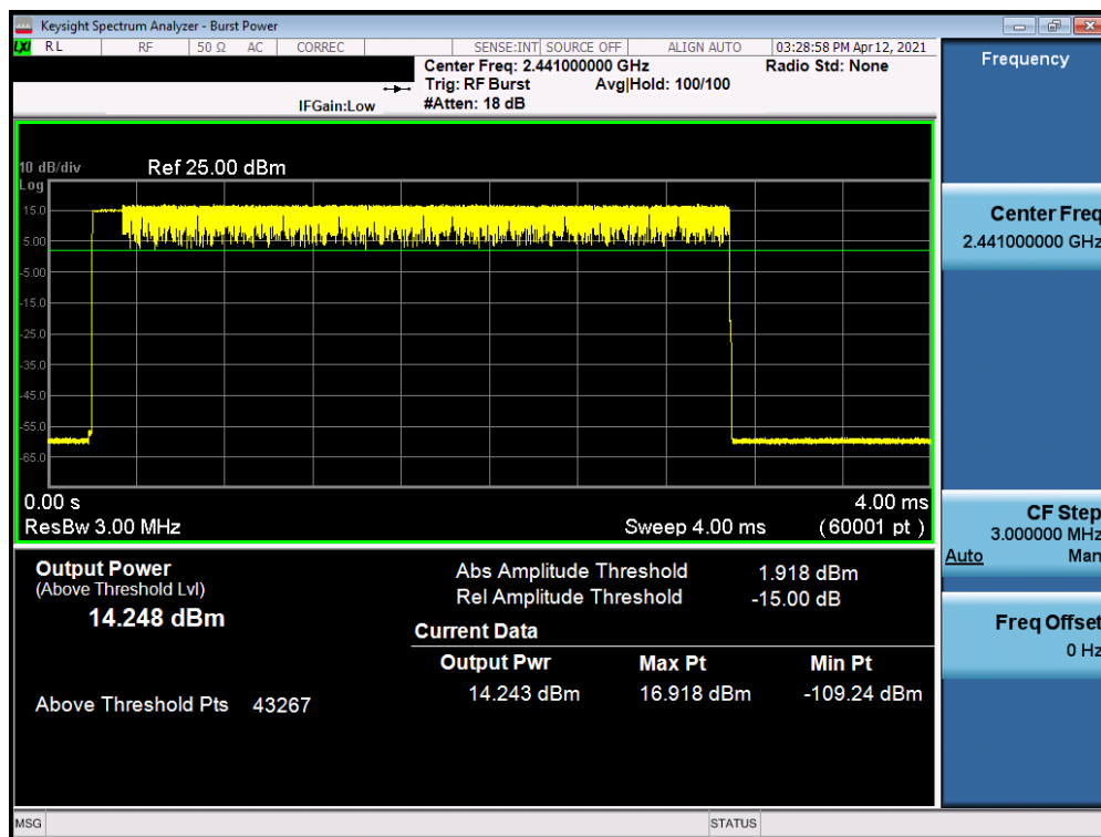
Plot 7-44. Average Conducted Power (2Mbps – Ch. 39) Antenna 0 - ePA
